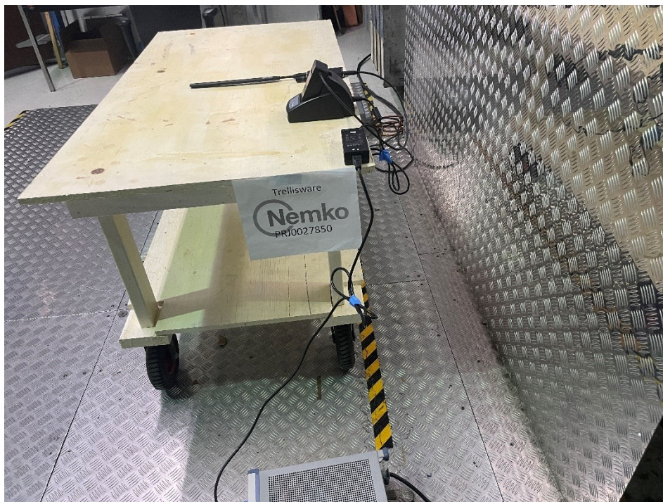
Figure 9 – Test setup, side view.
