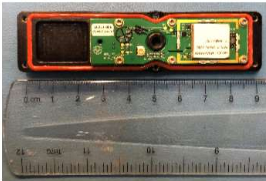
Figure 6: TW-1760 PCB, shield-can removed
