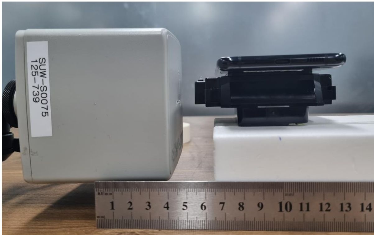
Right position (6cm test distance between Probe's center to DUT's surface)
