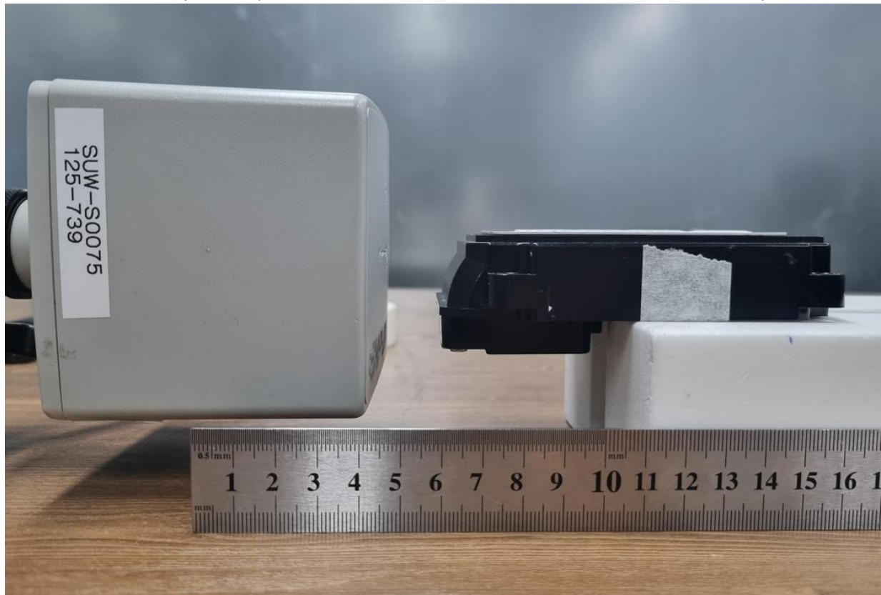
Bottom position (6cm test distance between Probe's center to DUT's surface)
