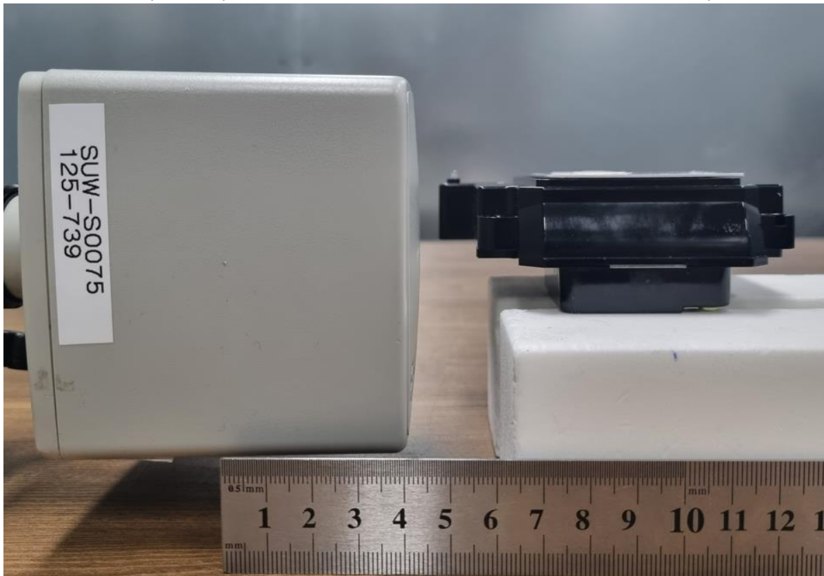
Right position (6cm test distance between Probe's center to DUT's surface)
