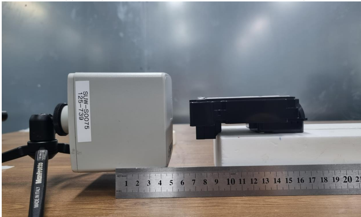
Bottom position (6cm test distance between Probe's center to DUT's surface)
