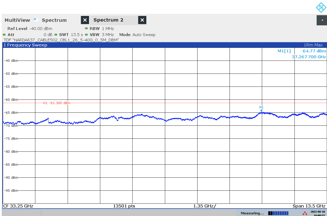
Plot 11: 26.5 GHz to 40.0 GHz (EUT2)
