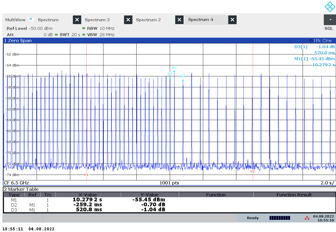
Plot 14: Emissions of the EUT, only at the beginning with associated receiver (EUT3)
