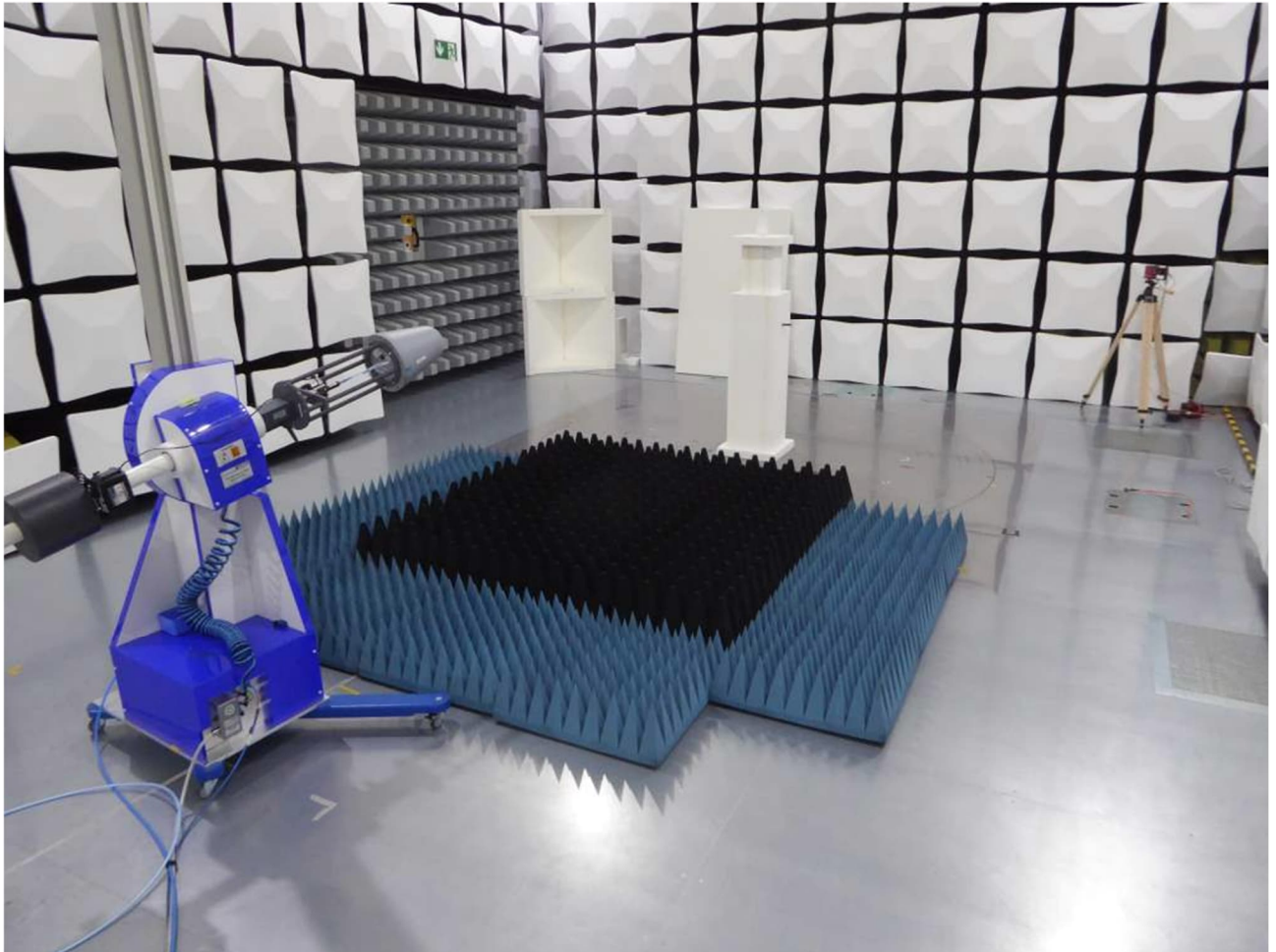
Test setup semi anechoic chamber with ground absorbers 1 GHz – 10 GHz
