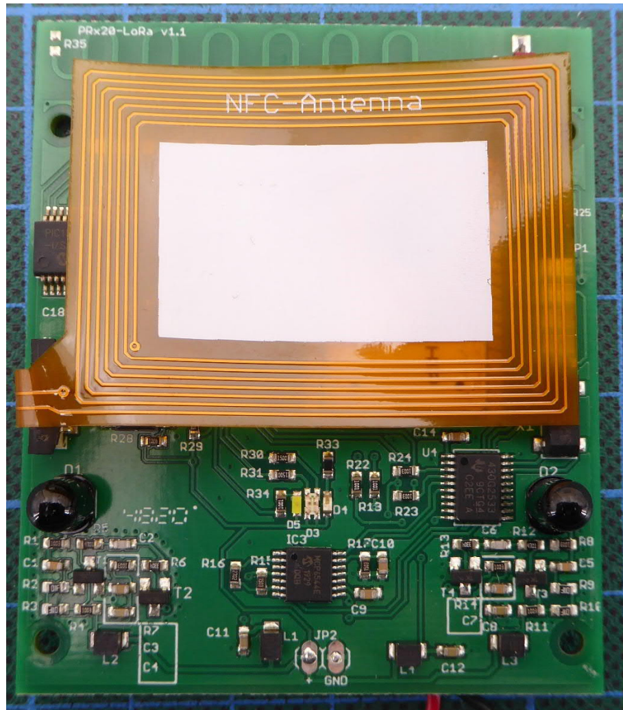
Receiver PCB Top view1
