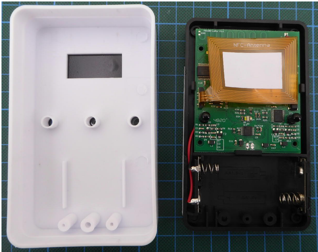
Receiver opened
