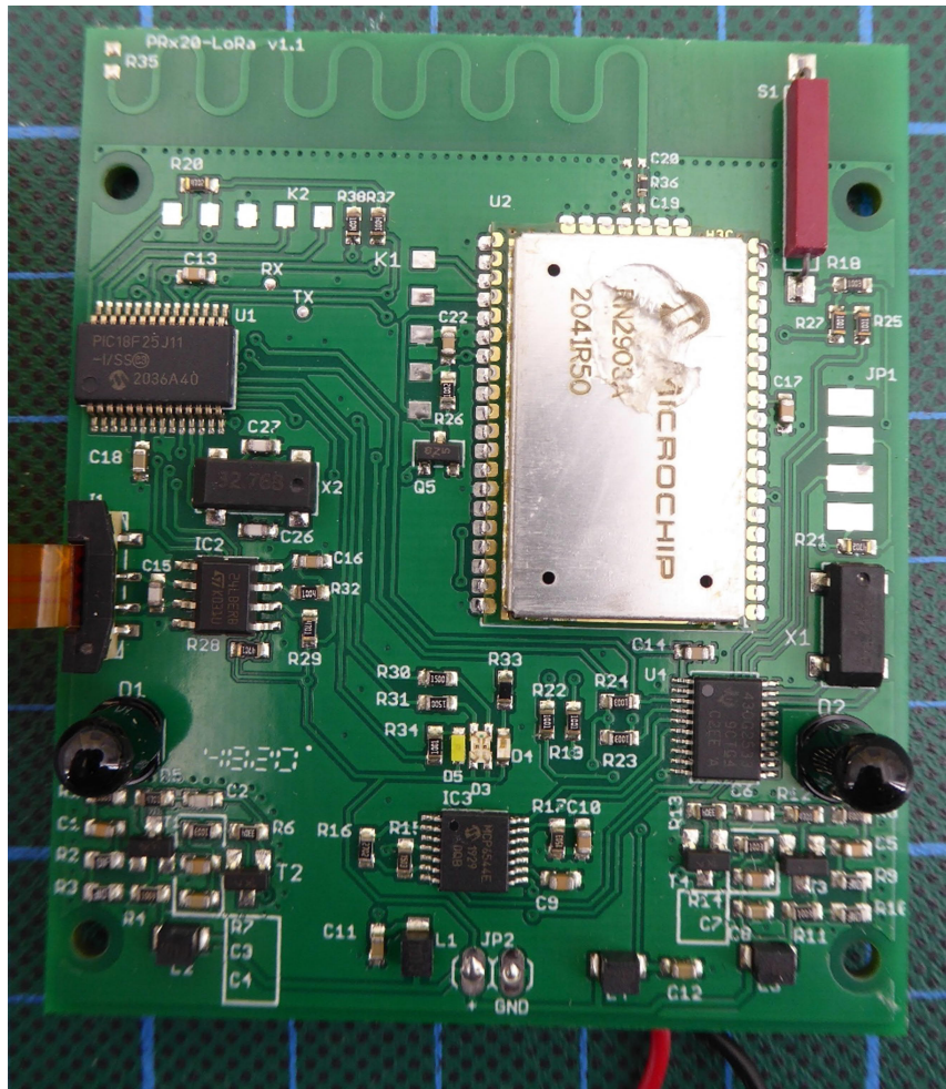
Receiver PCB Top view2 Integrated LoRA-WAN not yet finally labelled
