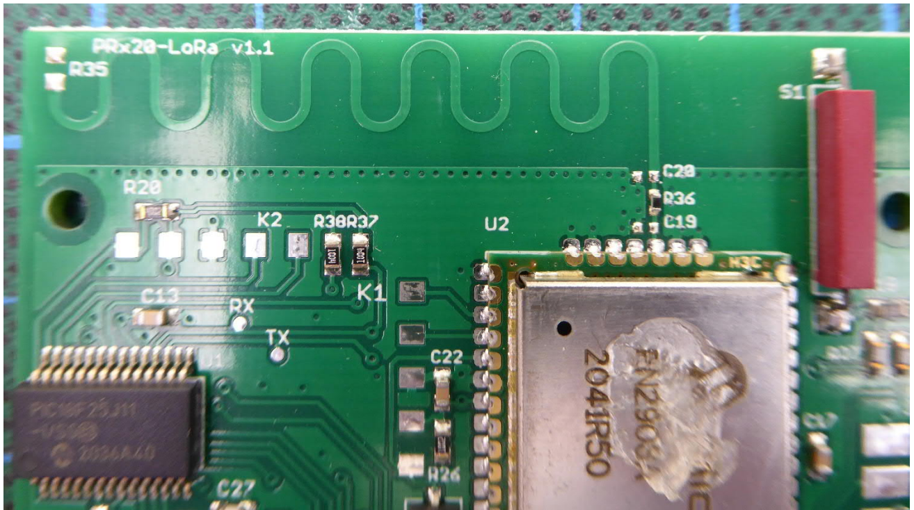
Radio part Detail view
