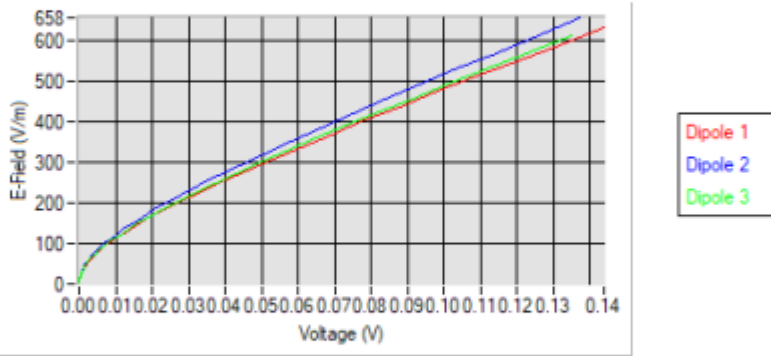
Calibration curves
