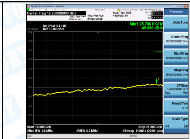
Band4-10MHz-QPSK-20350-1-0-High-12000-26500--45.9-PASS
