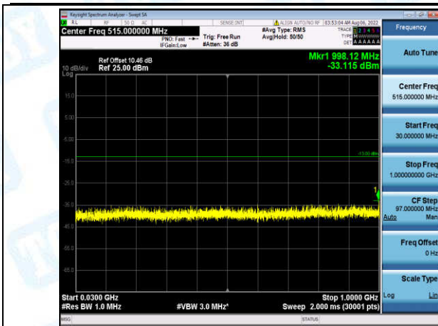
Band4-20MHz-QPSK-20175-1-0-Low-30-1000--33.12-PASS
