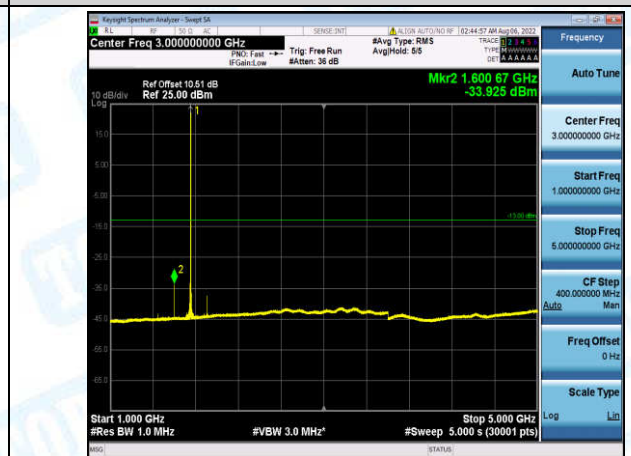
Band4-10MHz-16QAM-20350-1-0-High-1000-5000--33.93-PASS
