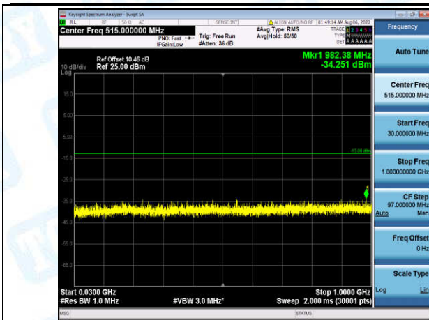
Band4-5MHz-QPSK-20175-1-0-Low-30-1000--34.25-PASS
