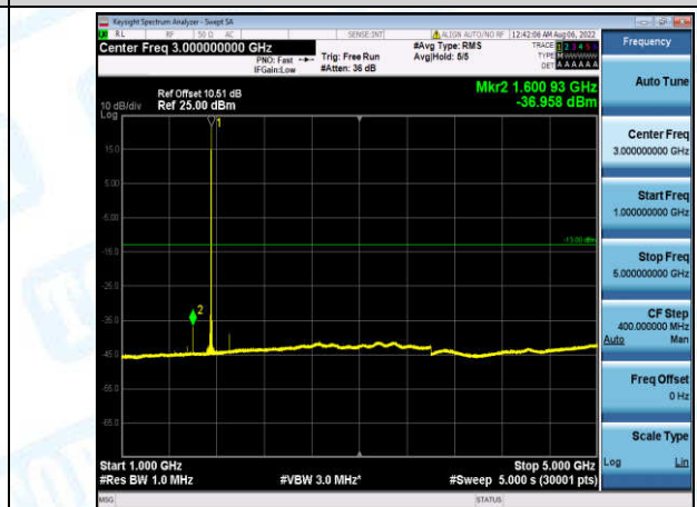
Band4-3MHz-16QAM-20385-1-0-High-1000-5000--36.96-PASS
