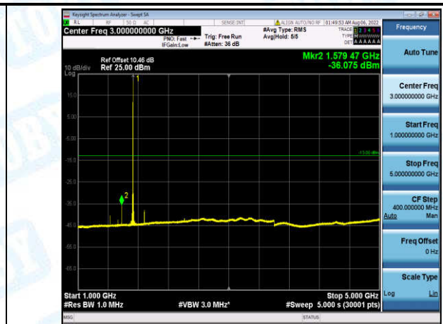
Band4-5MHz-QPSK-20175-1-0-Low-1000-5000--36.08-PASS
