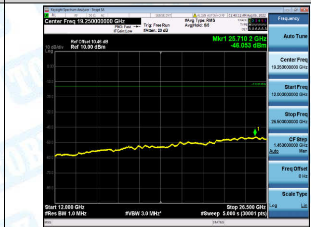
Band4-10MHz-QPSK-20175-1-0-Low-12000-26500--46.05-PASS
