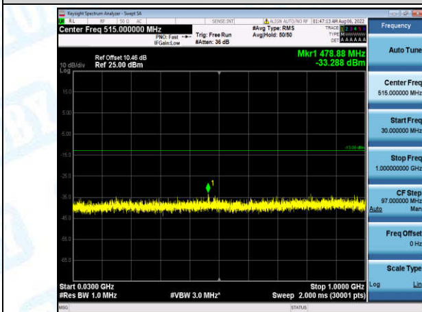
Band4-5MHz-16QAM-19975-1-0-Low-30-1000--33.29-PASS
