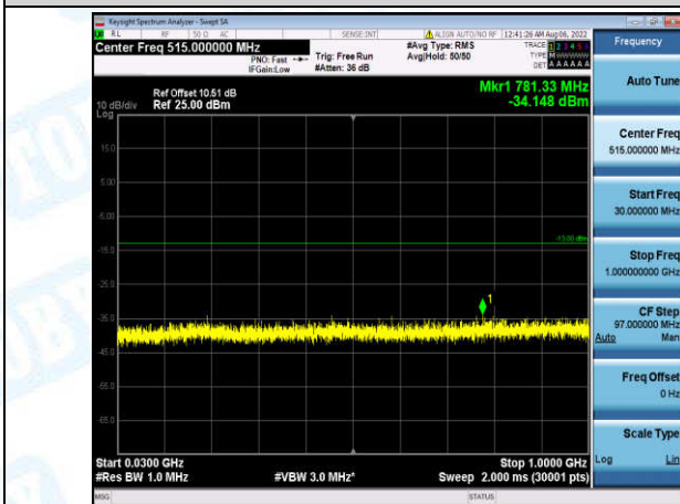
Band4-3MHz-16QAM-20385-1-0-High-30-1000--34.15-PASS
