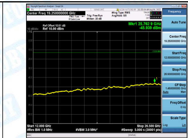
Band4-5MHz-QPSK-20375-1-0-High-12000-26500--45.94-PASS
