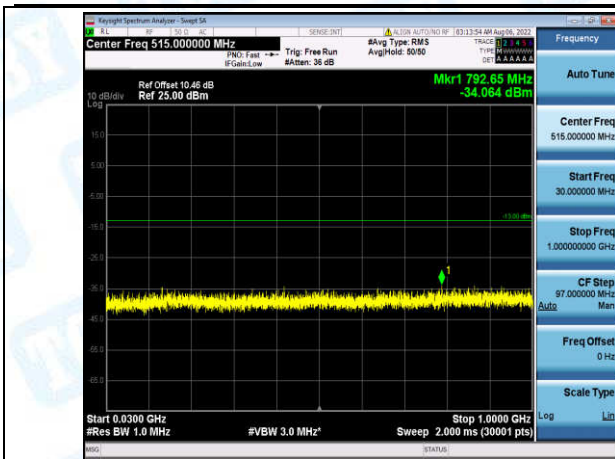
Band4-15MHz-QPSK-20175-1-0-Low-30-1000--34.06-PASS
