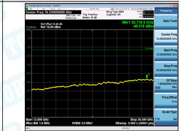
Band4-5MHz-QPSK-20175-1-0-Low-12000-26500--46.02-PASS
