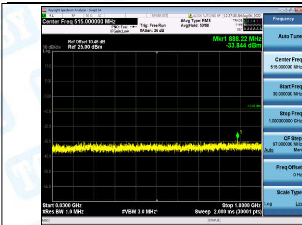
Band4-3MHz-16QAM-20175-1-0-Low-30-1000--33.84-PASS
