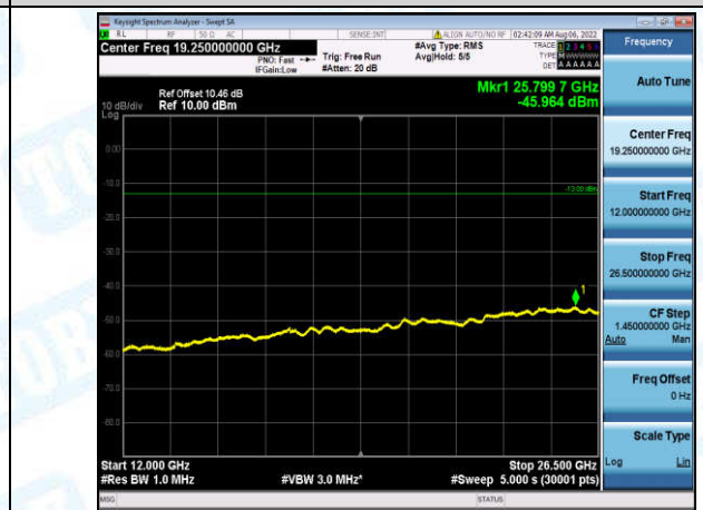
Band4-10MHz-16QAM-20175-1-0-Low-12000-26500--45.96-PASS
