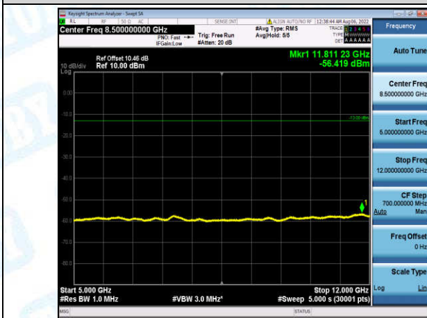
Band4-3MHz-16QAM-20175-1-0-Low-5000-12000--56.42-PASS
