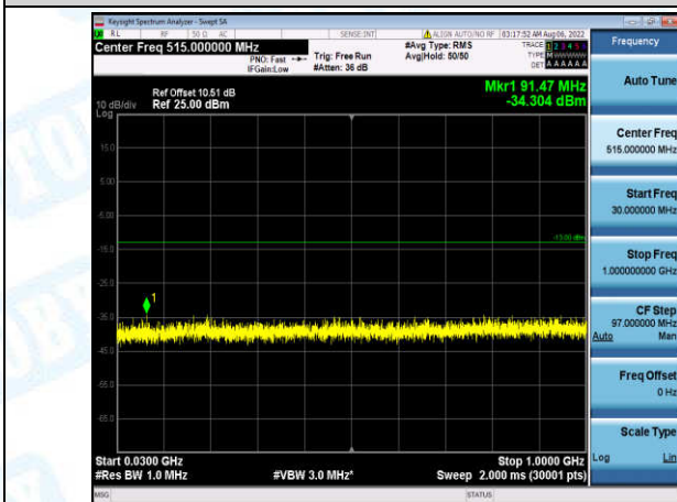
Band4-15MHz-QPSK-20325-1-0-High-30-1000--34.3-PASS
