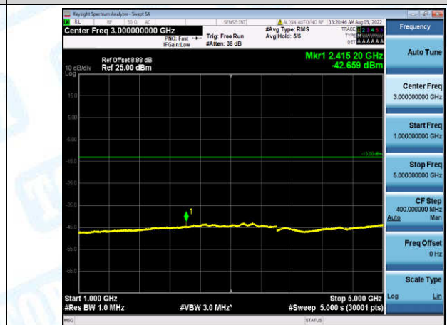
Band5-1.4MHz-QPSK-20643-1-0-High-1000-5000--42.66-PASS
