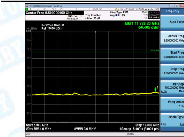
Band4-5MHz-QPSK-20175-1-0-Low-5000-12000--56.47-PASS
