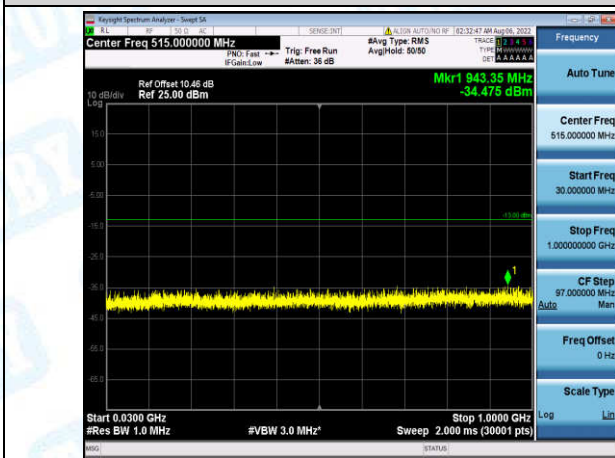
Band4-10MHz-16QAM-20000-1-0-Low-30-1000--34.48-PASS
