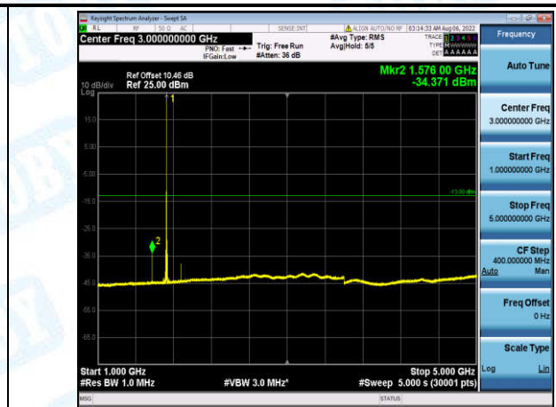
Band4-15MHz-QPSK-20175-1-0-Low-1000-5000--34.37-PASS
