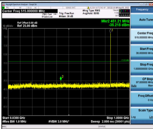
Band5-1.4MHz-16QAM-20643-1-0-High-30-1000--35.22-PASS
