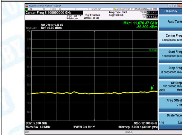
Band4-15MHz-QPSK-20175-1-0-Low-5000-12000--56.4-PASS
