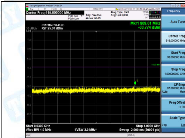
Band4-5MHz-16QAM-20175-1-0-Low-30-1000--33.77-PASS
