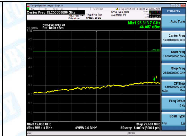
Band4-20MHz-16QAM-20300-1-0-High-12000-26500--46.06-PASS
