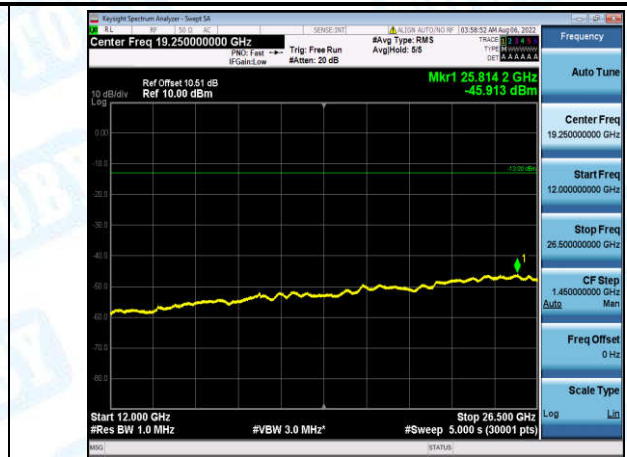
Band4-20MHz-QPSK-20300-1-0-High-12000-26500--45.91-PASS
