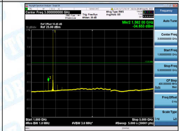
Band4-10MHz-QPSK-20000-1-0-Low-1000-5000--34.65-PASS
