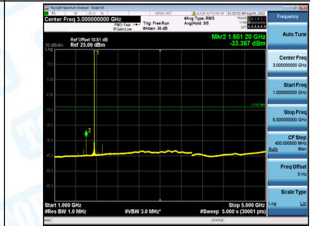
Band4-5MHz-16QAM-20375-1-0-High-1000-5000--33.37-PASS
