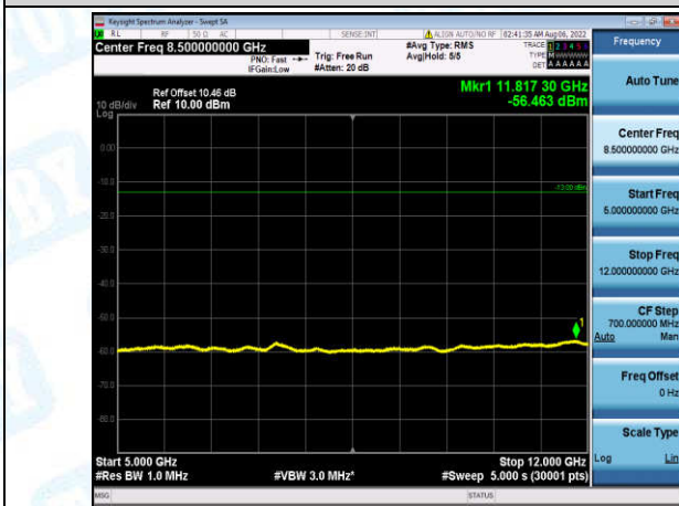
Band4-10MHz-16QAM-20175-1-0-Low-5000-12000--56.46-PASS
