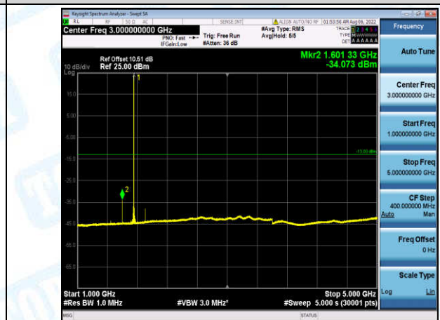
Band4-5MHz-QPSK-20375-1-0-High-1000-5000--34.07-PASS
