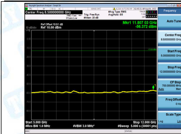
Band4-10MHz-16QAM-20350-1-0-High-5000-12000--56.37-PASS
