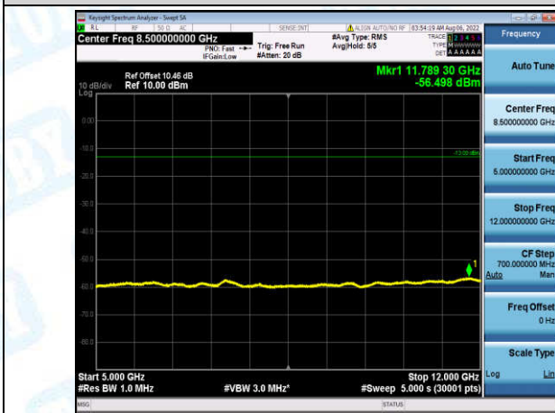
Band4-20MHz-QPSK-20175-1-0-Low-5000-12000--56.5-PASS
