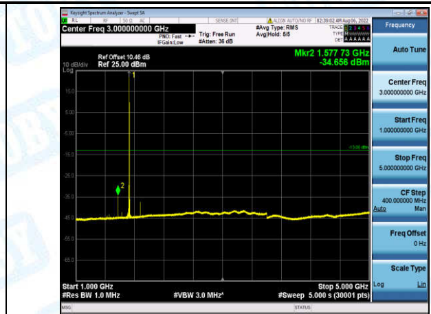
Band4-10MHz-QPSK-20175-1-0-Low-1000-5000--34.66-PASS
