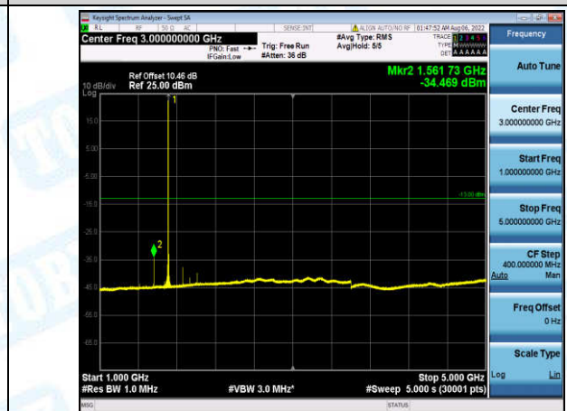
Band4-5MHz-16QAM-19975-1-0-Low-1000-5000--34.47-PASS
