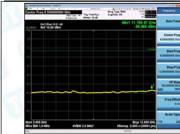
Band4-20MHz-16QAM-20300-1-0-High-5000-12000--56.47-PASS
