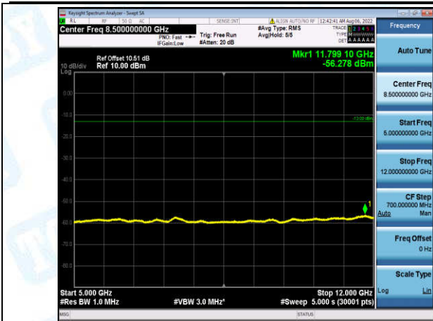
Band4-3MHz-16QAM-20385-1-0-High-5000-12000--56.28-PASS
