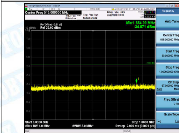
Band4-20MHz-QPSK-20300-1-0-High-30-1000--34.07-PASS
