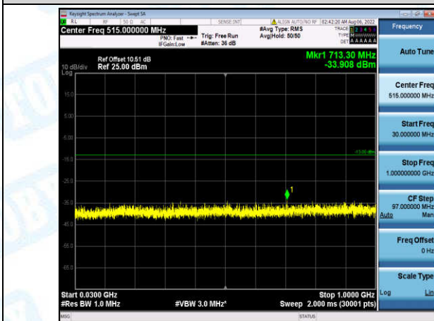
Band4-10MHz-QPSK-20350-1-0-High-30-1000--33.91-PASS
