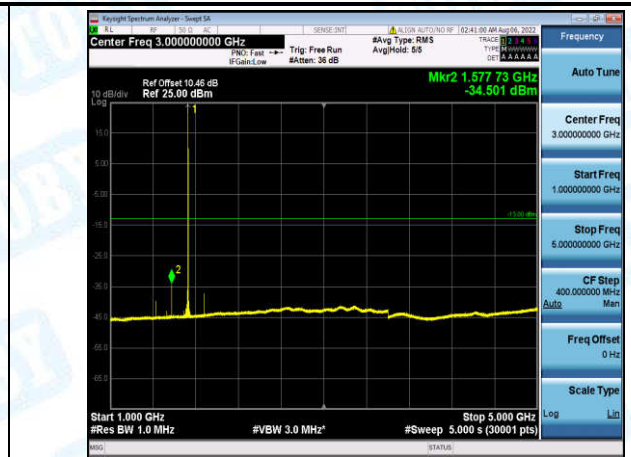
Band4-10MHz-16QAM-20175-1-0-Low-1000-5000--34.5-PASS
