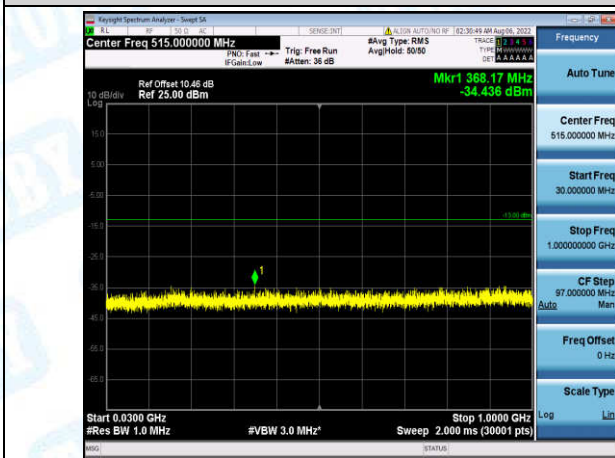
Band4-10MHz-QPSK-20000-1-0-Low-30-1000--34.44-PASS
