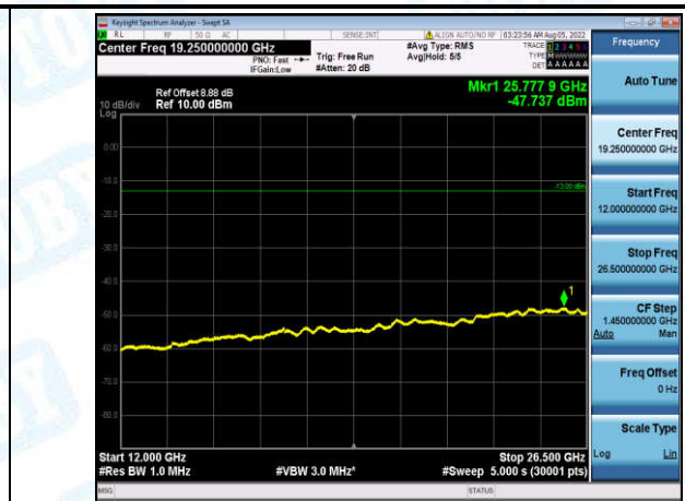
Band5-1.4MHz-16QAM-20643-1-0-High-12000-26500--47.74-PASS
