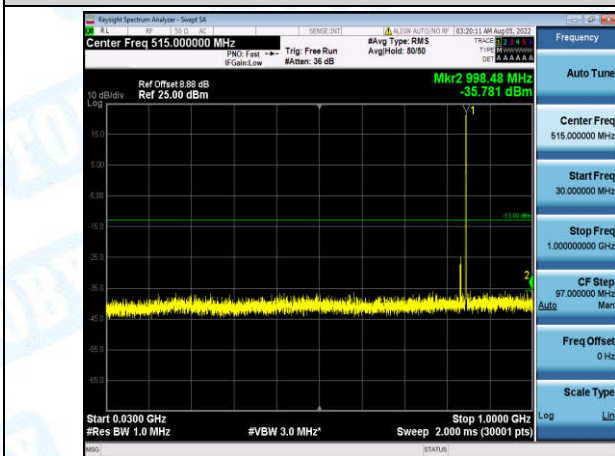
Band5-1.4MHz-QPSK-20643-1-0-High-30-1000--35.78-PASS
