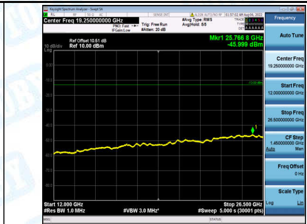
Band4-5MHz-16QAM-20375-1-0-High-12000-26500--46-PASS
