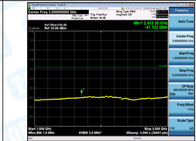
Band5-1.4MHz-16QAM-20643-1-0-High-1000-5000--41.12-PASS
