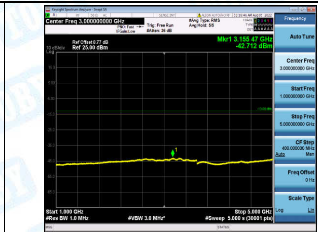
Band5-1.4MHz-QPSK-20525-1-0-Low-1000-5000--42.71-PASS
