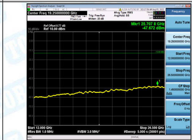
Band5-1.4MHz-QPSK-20525-1-0-Low-12000-26500--47.67-PASS
