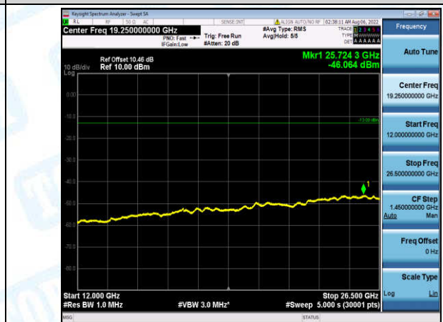
Band4-10MHz-16QAM-20000-1-0-Low-12000-26500--46.06-PASS
