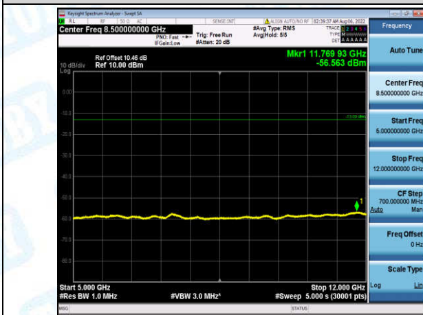
Band4-10MHz-QPSK-20175-1-0-Low-5000-12000--56.56-PASS
