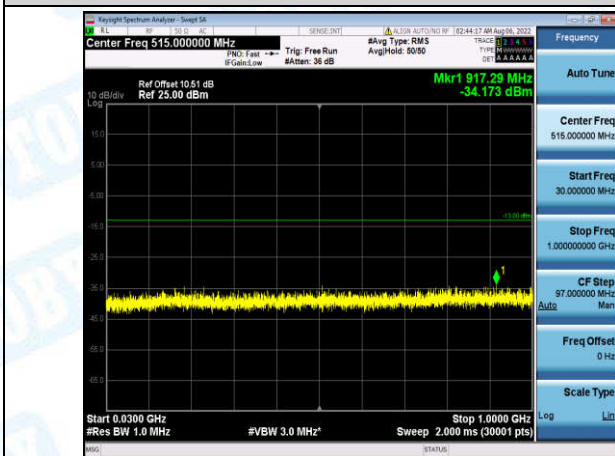
Band4-10MHz-16QAM-20350-1-0-High-30-1000--34.17-PASS
