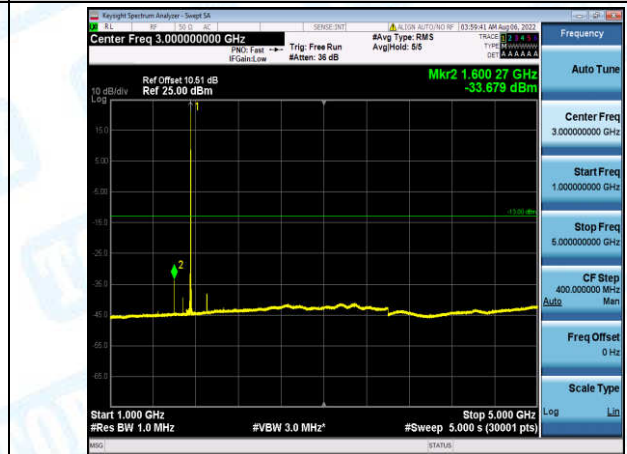
Band4-20MHz-16QAM-20300-1-0-High-1000-5000--33.68-PASS
