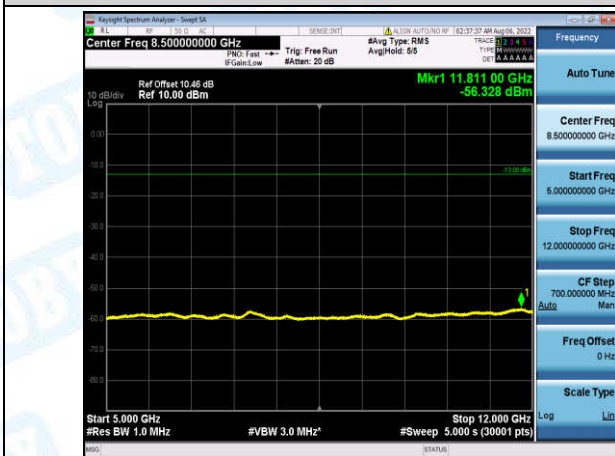
Band4-10MHz-16QAM-20000-1-0-Low-5000-12000--56.33-PASS
