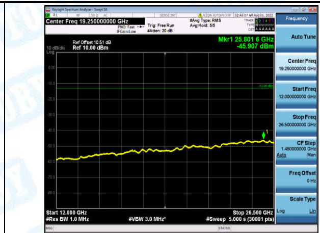
Band4-10MHz-16QAM-20350-1-0-High-12000-26500--45.91-PASS
