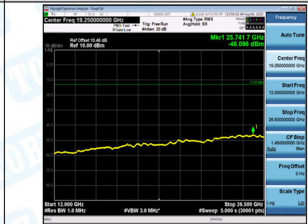
Band4-20MHz-16QAM-20175-1-0-Low-12000-26500--46.1-PASS
