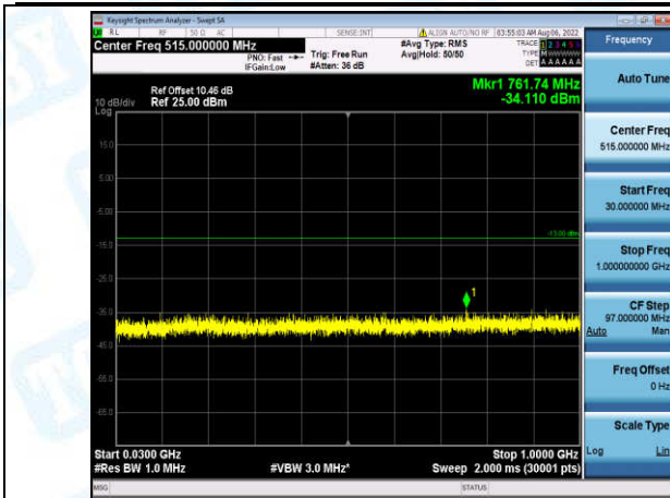
Band4-20MHz-16QAM-20175-1-0-Low-30-1000--34.11-PASS
