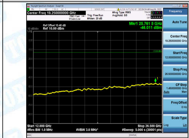
Band4-20MHz-QPSK-20175-1-0-Low-12000-26500--46.01-PASS
