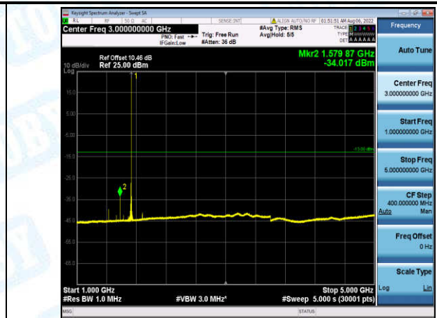
Band4-5MHz-16QAM-20175-1-0-Low-1000-5000--34.02-PASS
