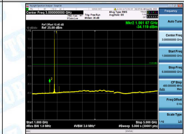
Band4-10MHz-16QAM-20000-1-0-Low-1000-5000--34.12-PASS
