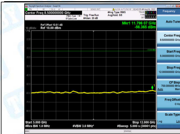
Band4-10MHz-QPSK-20350-1-0-High-5000-12000--56.37-PASS
