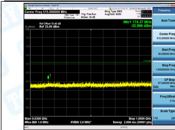
Band4-10MHz-16QAM-20175-1-0-Low-30-1000--32.9-PASS
