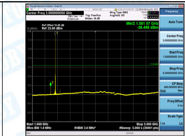
Band4-3MHz-16QAM-20175-1-0-Low-1000-5000--36.5-PASS
