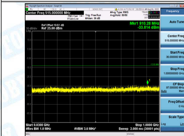
Band4-5MHz-QPSK-20375-1-0-High-30-1000--33.81-PASS
