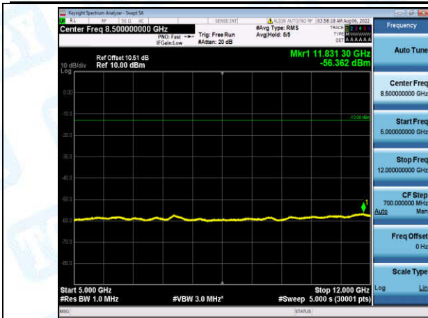
Band4-20MHz-QPSK-20300-1-0-High-5000-12000--56.36-PASS
