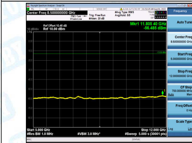
Band4-5MHz-16QAM-20175-1-0-Low-5000-12000--56.49-PASS
