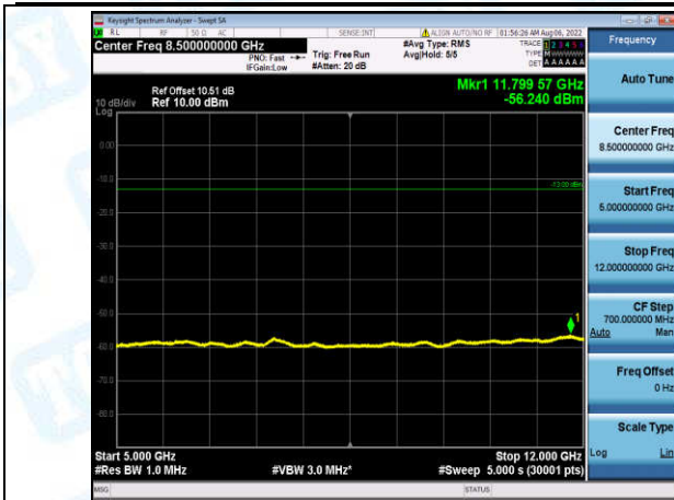
Band4-5MHz-16QAM-20375-1-0-High-5000-12000--56.24-PASS
