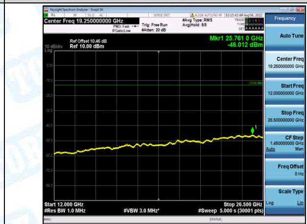
Band4-15MHz-QPSK-20175-1-0-Low-12000-26500--46.01-PASS
