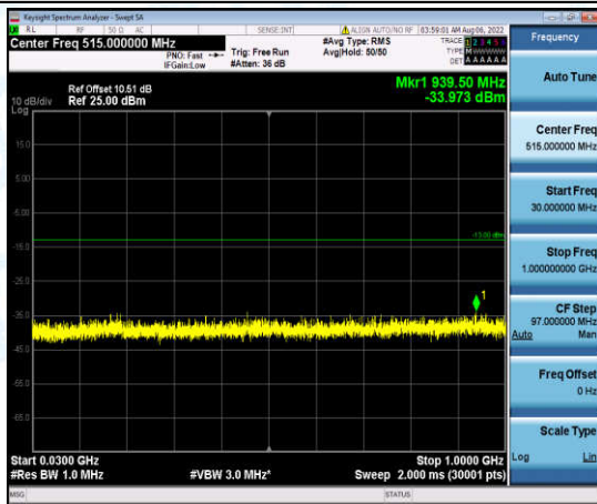
Band4-20MHz-16QAM-20300-1-0-High-30-1000--33.97-PASS
