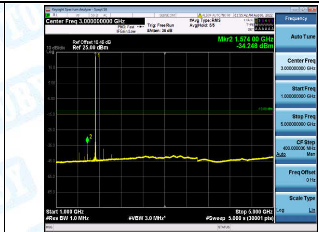
Band4-20MHz-16QAM-20175-1-0-Low-1000-5000--34.25-PASS
