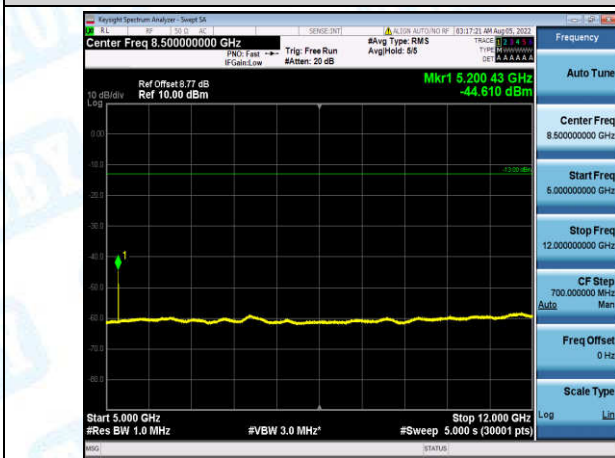
Band5-1.4MHz-QPSK-20525-1-0-Low-5000-12000--44.61-PASS
