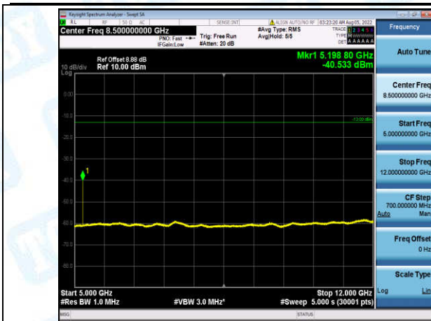
Band5-1.4MHz-16QAM-20643-1-0-High-5000-12000--40.53-PASS
