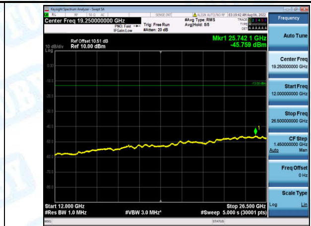
Band4-15MHz-QPSK-20325-1-0-High-12000-26500--45.76-PASS
