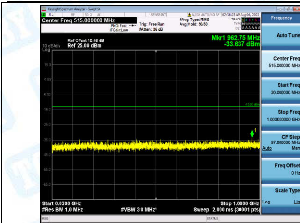
Band4-10MHz-QPSK-20175-1-0-Low-30-1000--33.64-PASS
