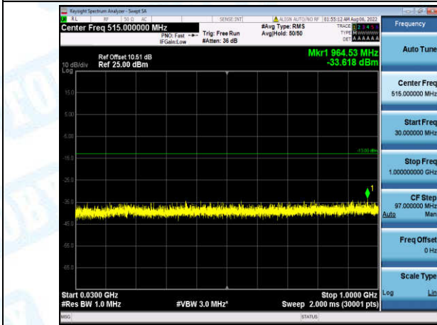
Band4-5MHz-16QAM-20375-1-0-High-30-1000--33.62-PASS
