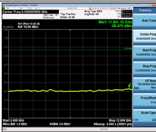
Band4-20MHz-16QAM-20175-1-0-Low-5000-12000--56.47-PASS
