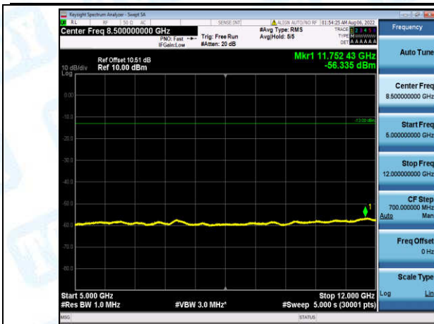
Band4-5MHz-QPSK-20375-1-0-High-5000-12000--56.34-PASS
