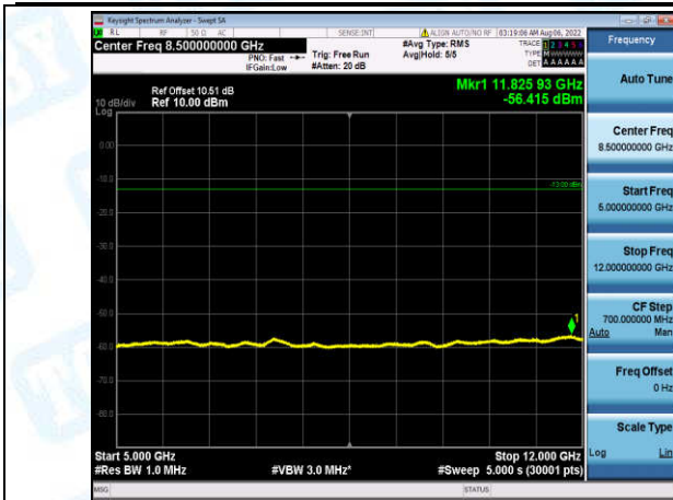
Band4-15MHz-QPSK-20325-1-0-High-5000-12000--56.42-PASS
