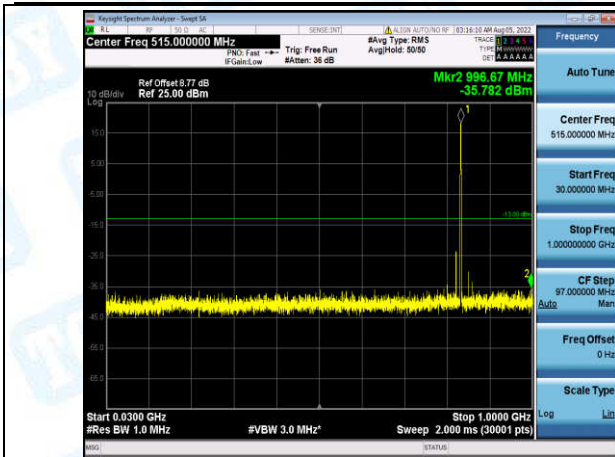
Band5-1.4MHz-QPSK-20525-1-0-Low-30-1000--35.78-PASS
