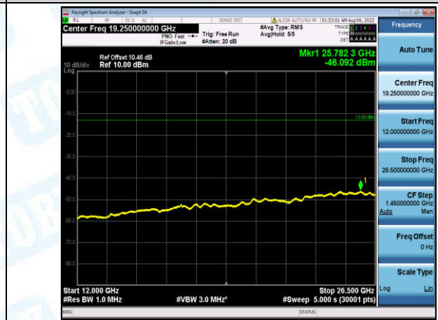
Band4-5MHz-16QAM-20175-1-0-Low-12000-26500--46.09-PASS
