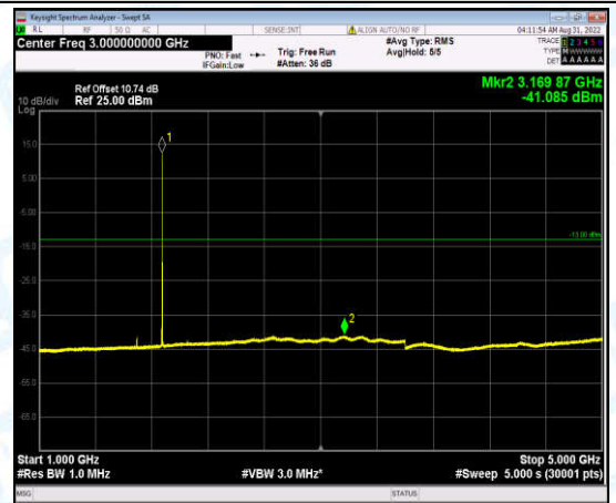
Band2-15MHz-QPSK-19150-1-0-High-1000-5000--41.09-PASS
