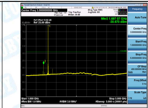
Band2-10MHz-QPSK-18900-1-0-Low-1000-5000--30.67-PASS
