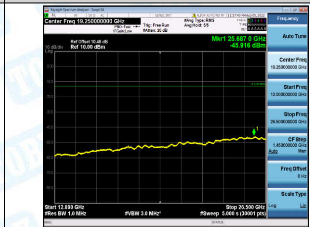
Band4-1.4MHz-QPSK-20175-1-0-Low-12000-26500--45.92-PASS
