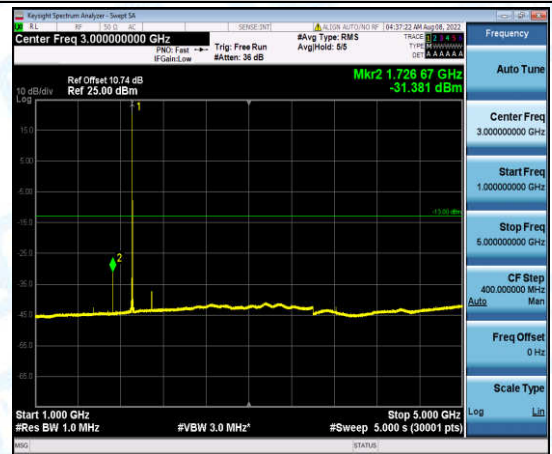
Band2-10MHz-QPSK-19150-1-0-High-1000-5000--31.38-PASS
