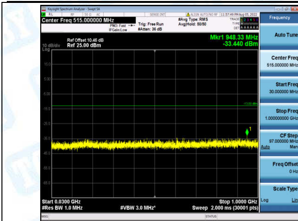
Band4-1.4MHz-16QAM-20175-1-0-Low-30-1000--33.44-PASS
