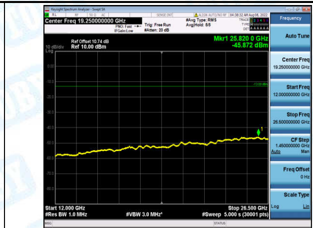
Band2-10MHz-QPSK-19150-1-0-High-12000-26500--45.87-PASS
