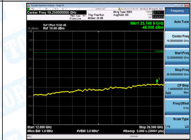
Band2-10MHz-16QAM-18900-1-0-Low-12000-26500--46.06-PASS
