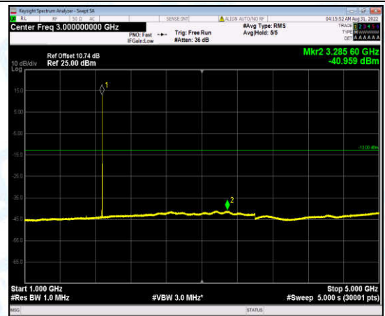
Band2-15MHz-16QAM-19150-1-0-High-1000-5000--40.96-PASS
