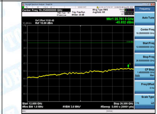
Band2-5MHz-16QAM-18900-1-0-Low-12000-26500--45.83-PASS
