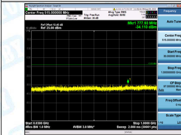
Band4-1.4MHz-16QAM-19957-1-0-Low-30-1000--34.11-PASS
