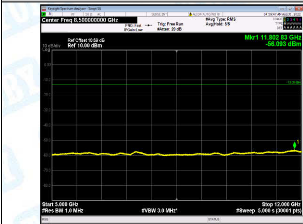
Band2-20MHz-16QAM-18900-1-0-Low-5000-12000--56.09-PASS
