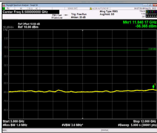
Band2-15MHz-16QAM-18900-1-0-Low-5000-12000--56.37-PASS
