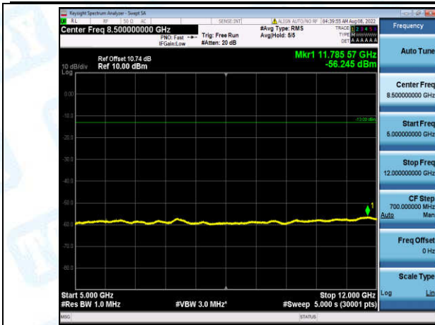
Band2-10MHz-16QAM-19150-1-0-High-5000-12000--56.25-PASS
