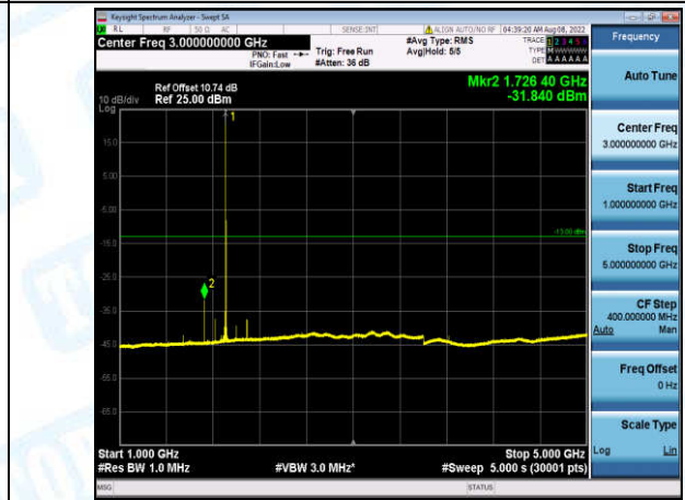
Band2-10MHz-16QAM-19150-1-0-High-1000-5000--31.84-PASS
