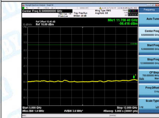
Band4-3MHz-QPSK-20175-1-0-Low-5000-12000--56.42-PASS
