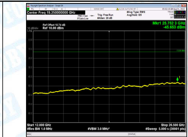
Band2-20MHz-QPSK-19100-1-0-High-12000-26500--45.65-PASS
