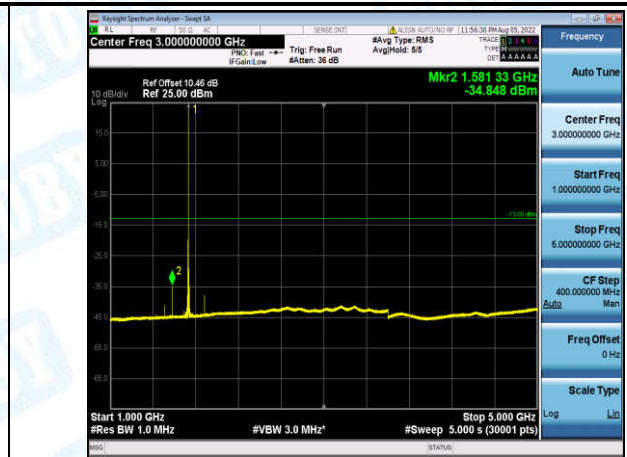
Band4-1.4MHz-QPSK-20175-1-0-Low-1000-5000--34.85-PASS
