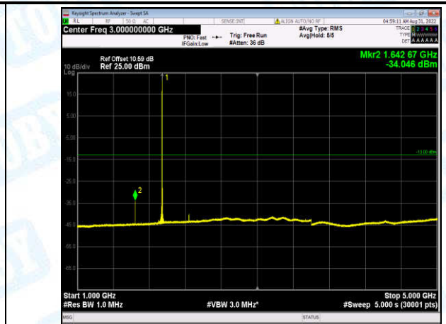
Band2-20MHz-16QAM-18900-1-0-Low-1000-5000--34.05-PASS
