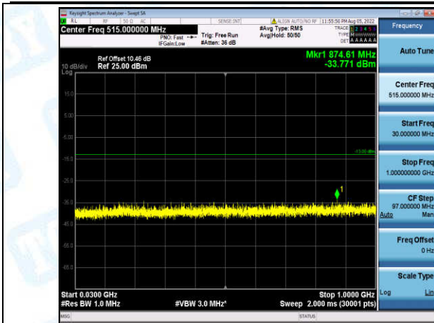
Band4-1.4MHz-QPSK-20175-1-0-Low-30-1000--33.77-PASS
