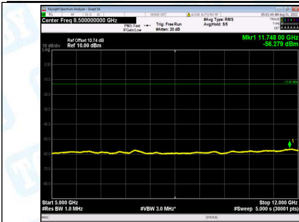
Band2-20MHz-QPSK-19100-1-0-High-5000-12000--56.28-PASS
