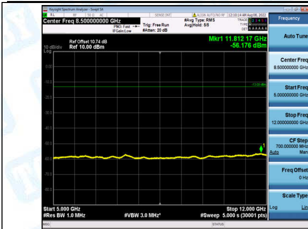
Band2-5MHz-16QAM-19175-1-0-High-5000-12000--56.18-PASS
