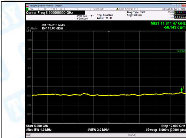
Band2-15MHz-16QAM-19150-1-0-High-5000-12000--56.14-PASS
