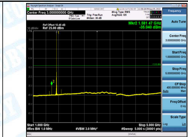
Band4-1.4MHz-16QAM-20175-1-0-Low-1000-5000--35.04-PASS
