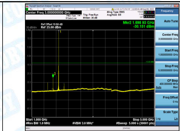
Band2-5MHz-QPSK-18900-1-0-Low-1000-5000--30.15-PASS
