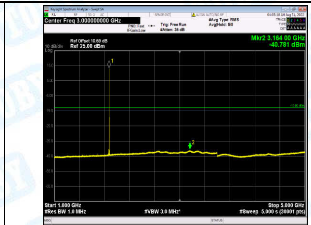
Band2-15MHz-QPSK-18900-1-0-Low-1000-5000--40.78-PASS
