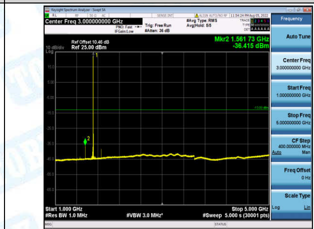
Band4-1.4MHz-16QAM-19957-1-0-Low-1000-5000--36.42-PASS
