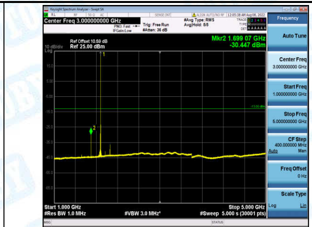
Band2-5MHz-16QAM-18900-1-0-Low-1000-5000--30.45-PASS
