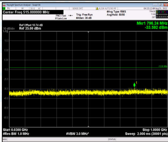
Band2-15MHz-16QAM-19150-1-0-High-30-1000--33.59-PASS
