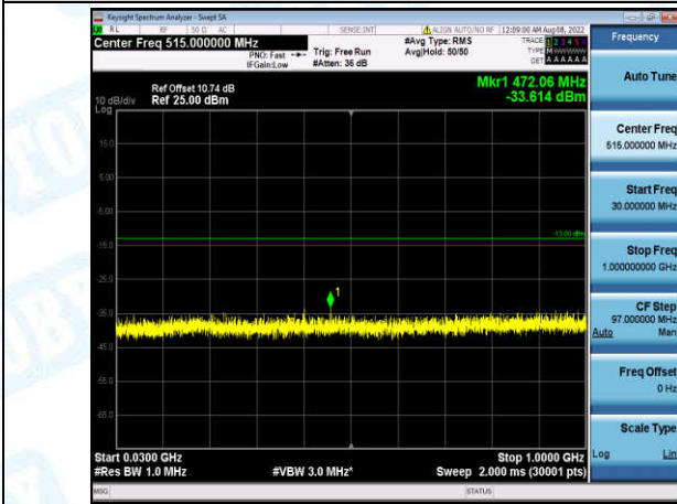
Band2-5MHz-16QAM-19175-1-0-High-30-1000--33.61-PASS
