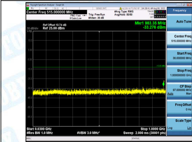
Band2-10MHz-16QAM-19150-1-0-High-30-1000--33.28-PASS
