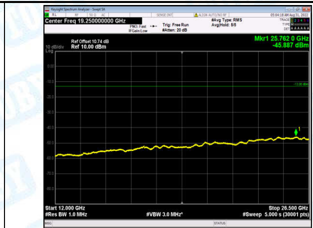
Band2-20MHz-16QAM-19100-1-0-High-12000-26500--45.89-PASS
