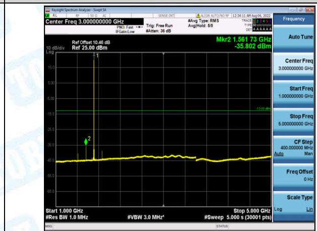
Band4-3MHz-16QAM-19965-1-0-Low-1000-5000--35.8-PASS
