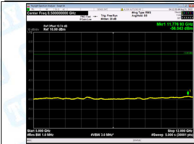
Band2-15MHz-QPSK-19150-1-0-High-5000-12000--56.04-PASS
