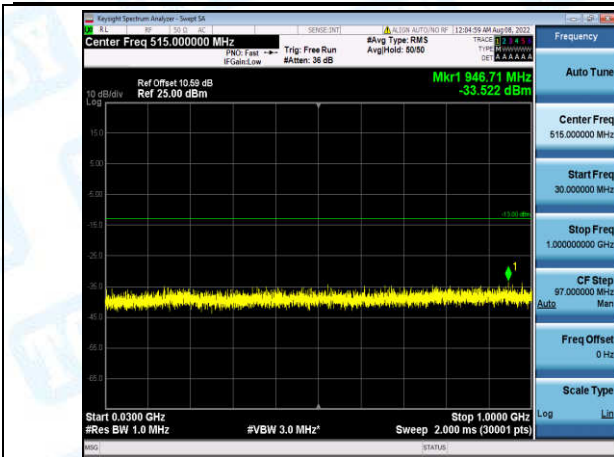
Band2-5MHz-16QAM-18900-1-0-Low-30-1000--33.52-PASS
