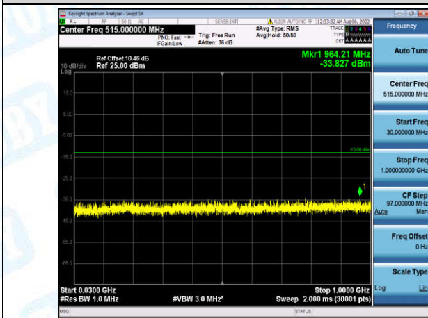
Band4-3MHz-16QAM-19965-1-0-Low-30-1000--33.83-PASS
