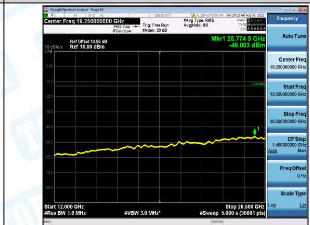
Band2-10MHz-QPSK-18650-1-0-Low-12000-26500--46-PASS
