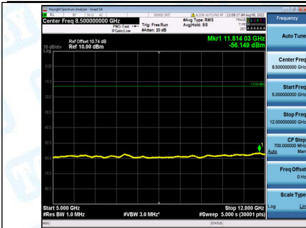
Band2-5MHz-QPSK-19175-1-0-High-5000-12000--56.15-PASS
