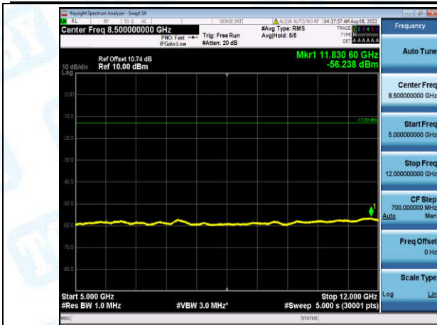
Band2-10MHz-QPSK-19150-1-0-High-5000-12000--56.24-PASS
