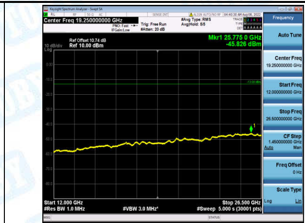
Band2-10MHz-16QAM-19150-1-0-High-12000-26500--45.83-PASS
