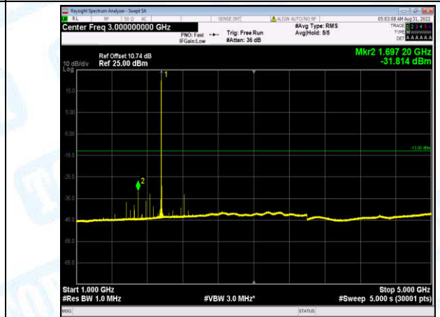
Band2-20MHz-16QAM-19100-1-0-High-1000-5000--31.81-PASS
