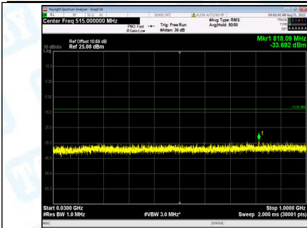
Band2-15MHz-16QAM-18900-1-0-Low-30-1000--33.69-PASS
