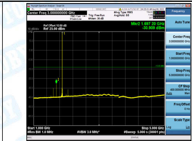
Band2-10MHz-16QAM-18900-1-0-Low-1000-5000--30.91-PASS
