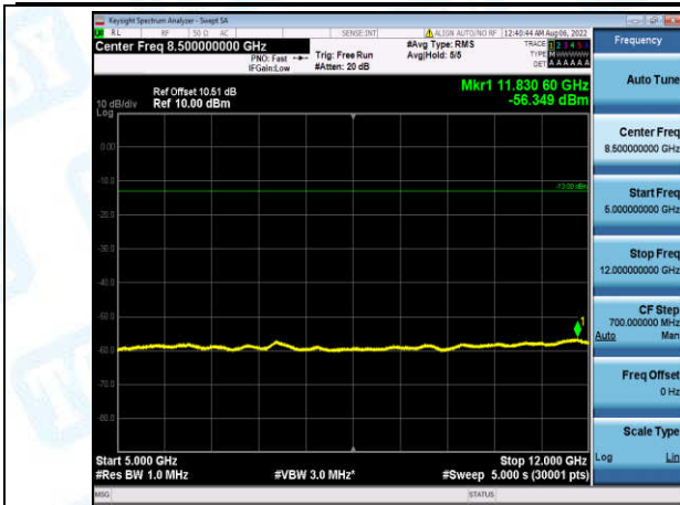
Band4-3MHz-QPSK-20385-1-0-High-5000-12000--56.35-PASS
