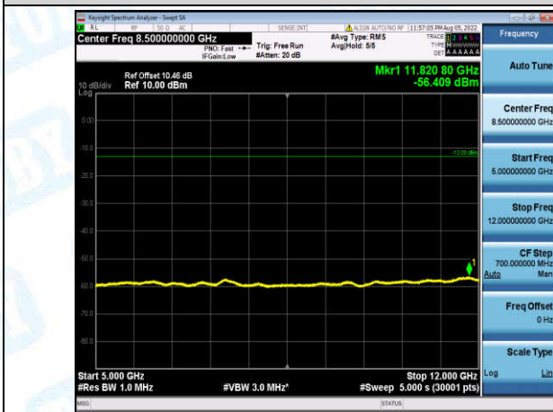
Band4-1.4MHz-QPSK-20175-1-0-Low-5000-12000--56.41-PASS
