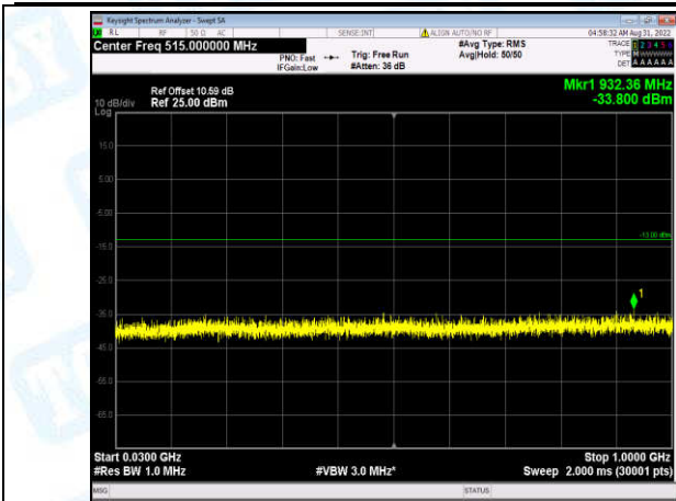
Band2-20MHz-16QAM-18900-1-0-Low-30-1000--33.8-PASS
