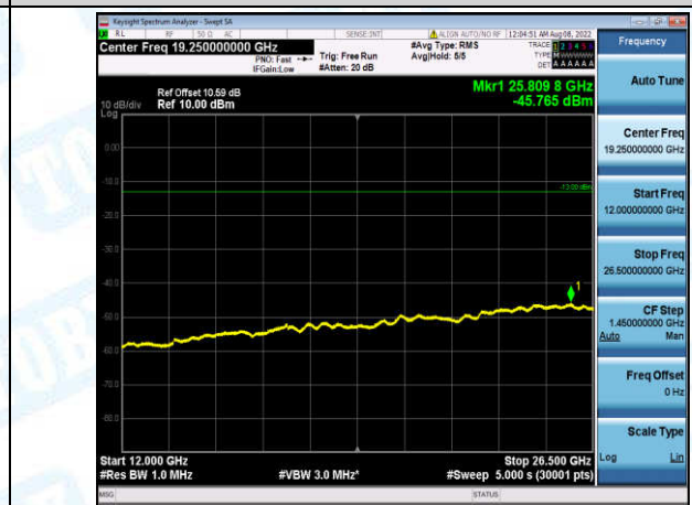
Band2-5MHz-QPSK-18900-1-0-Low-12000-26500--45.77-PASS
