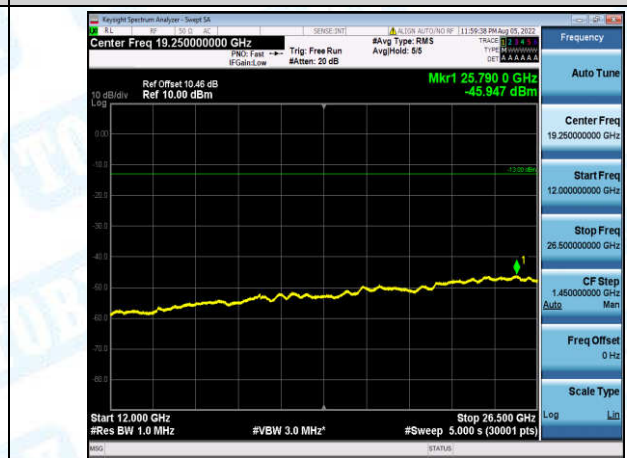
Band4-1.4MHz-16QAM-20175-1-0-Low-12000-26500--45.95-PASS
