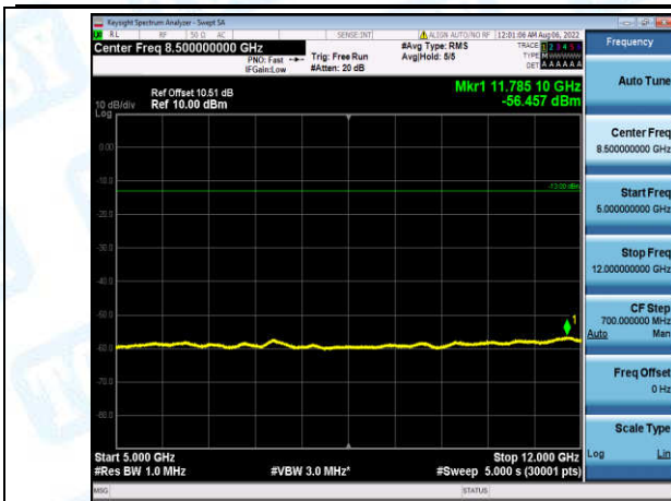
Band4-1.4MHz-QPSK-20393-1-0-High-5000-12000--56.46-PASS
