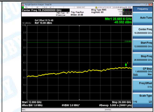
Band2-5MHz-16QAM-19175-1-0-High-12000-26500--45.55-PASS
