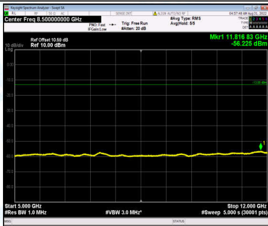
Band2-20MHz-QPSK-18900-1-0-Low-5000-12000--56.23-PASS
