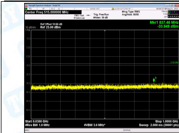
Band2-15MHz-QPSK-18900-1-0-Low-30-1000--33.95-PASS
