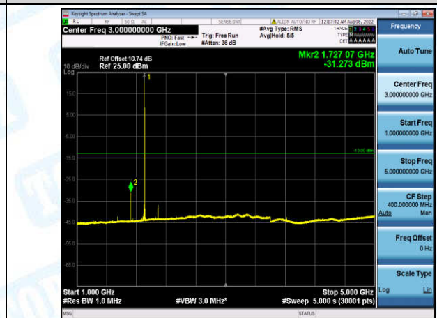
Band2-5MHz-QPSK-19175-1-0-High-1000-5000--31.27-PASS
