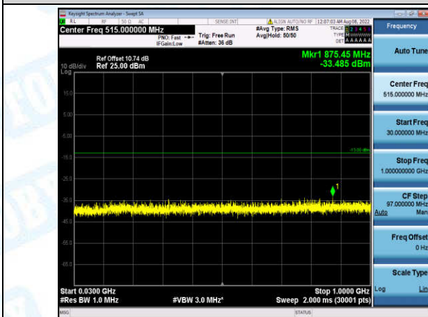
Band2-5MHz-QPSK-19175-1-0-High-30-1000--33.49-PASS
