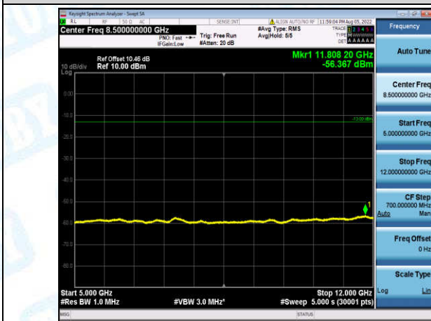
Band4-1.4MHz-16QAM-20175-1-0-Low-5000-12000--56.37-PASS
