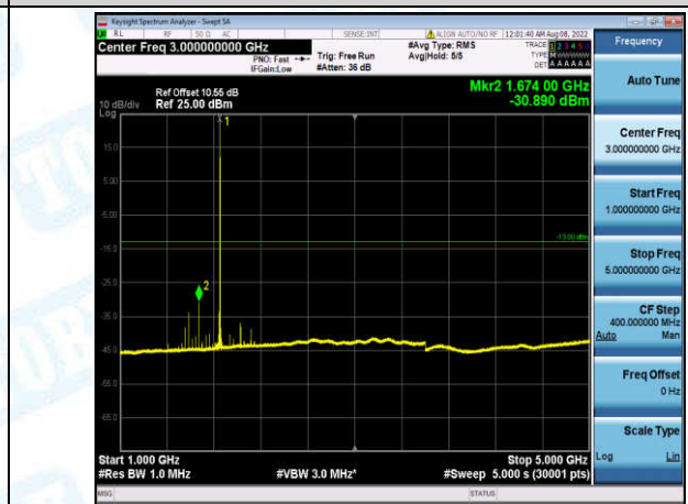
Band2-5MHz-16QAM-18625-1-0-Low-1000-5000--30.89-PASS
