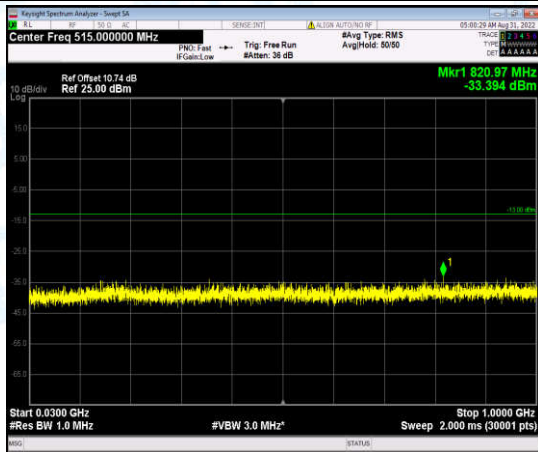
Band2-20MHz-QPSK-19100-1-0-High-30-1000--33.39-PASS
