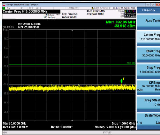
Band2-10MHz-QPSK-19150-1-0-High-30-1000--33.92-PASS
