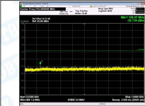
Band2-20MHz-16QAM-19100-1-0-High-30-1000--33.12-PASS
