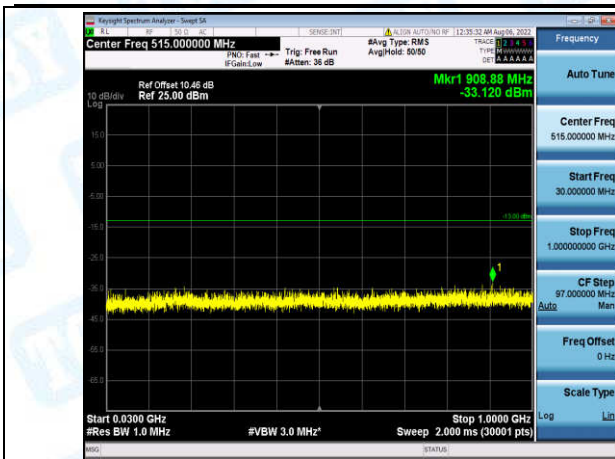
Band4-3MHz-QPSK-20175-1-0-Low-30-1000--33.12-PASS
