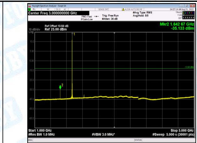
Band2-20MHz-QPSK-18900-1-0-Low-1000-5000--35.13-PASS
