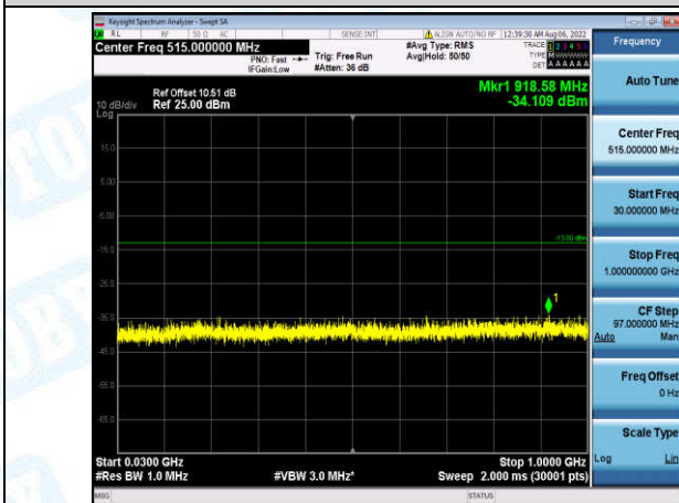
Band4-3MHz-QPSK-20385-1-0-High-30-1000--34.11-PASS
