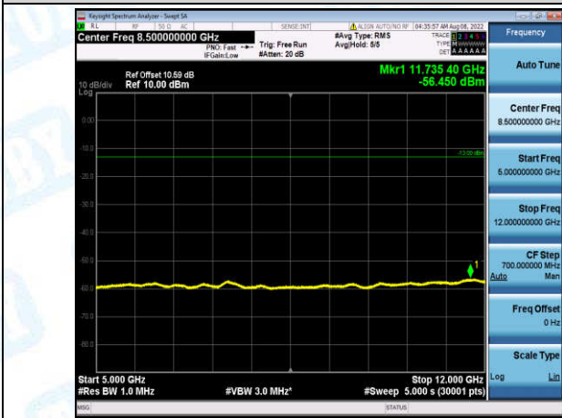
Band2-10MHz-16QAM-18900-1-0-Low-5000-12000--56.45-PASS
