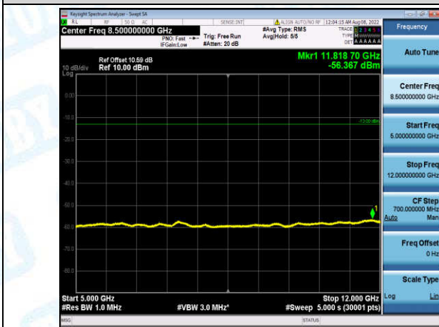
Band2-5MHz-QPSK-18900-1-0-Low-5000-12000--56.37-PASS
