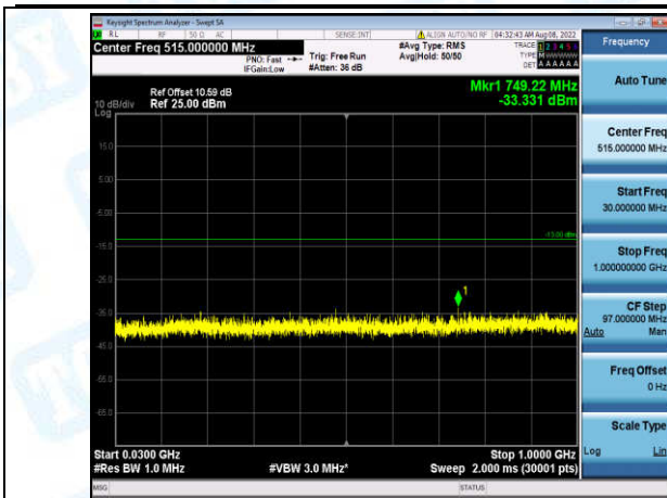
Band2-10MHz-QPSK-18900-1-0-Low-30-1000--33.33-PASS
