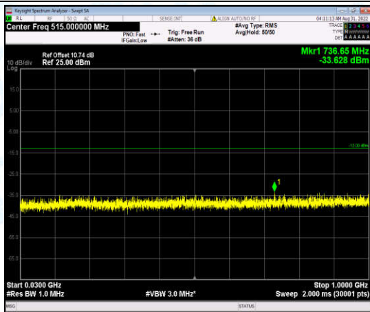
Band2-15MHz-QPSK-19150-1-0-High-30-1000--33.63-PASS
