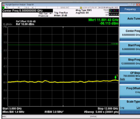
Band2-10MHz-QPSK-18900-1-0-Low-5000-12000--56.11-PASS
