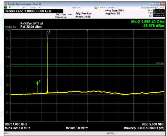
Band2-20MHz-QPSK-19100-1-0-High-1000-5000--35.98-PASS
