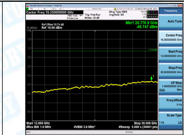
Band2-5MHz-QPSK-19175-1-0-High-12000-26500--45.75-PASS
