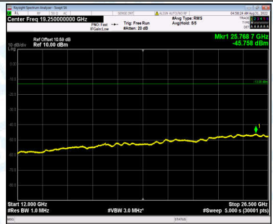
Band2-20MHz-QPSK-18900-1-0-Low-12000-26500--45.76-PASS
