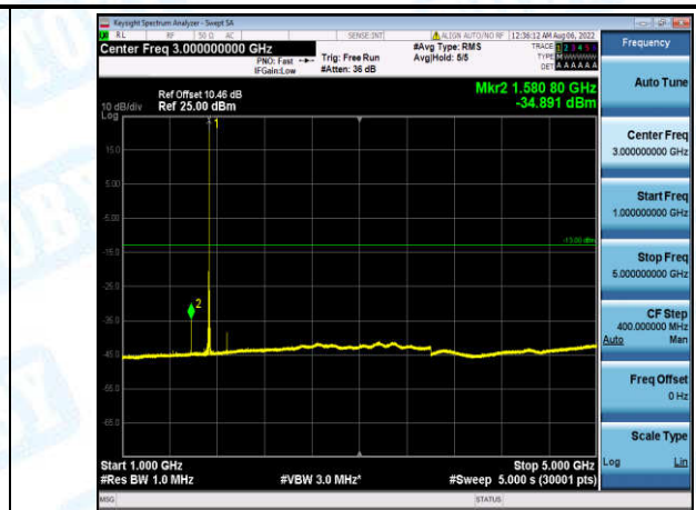
Band4-3MHz-QPSK-20175-1-0-Low-1000-5000--34.89-PASS
