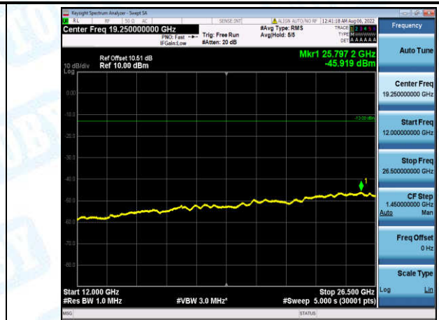
Band4-3MHz-QPSK-20385-1-0-High-12000-26500--45.92-PASS
