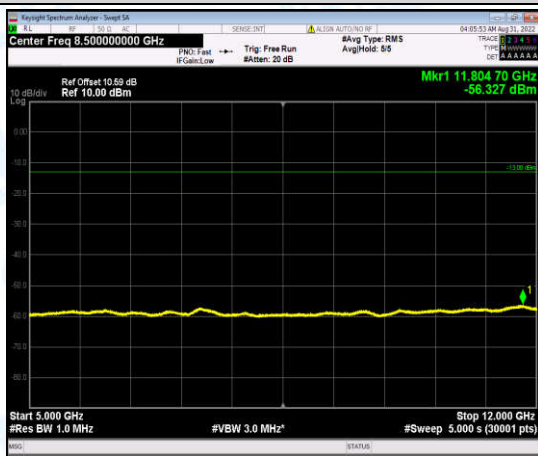
Band2-15MHz-QPSK-18900-1-0-Low-5000-12000--56.33-PASS
