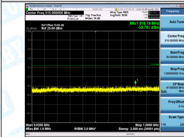
Band2-5MHz-16QAM-18625-1-0-Low-30-1000--33.78-PASS
