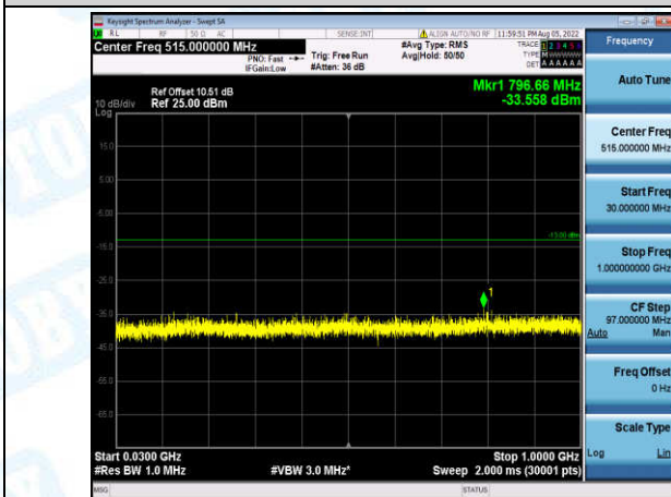
Band4-1.4MHz-QPSK-20393-1-0-High-30-1000--33.56-PASS
