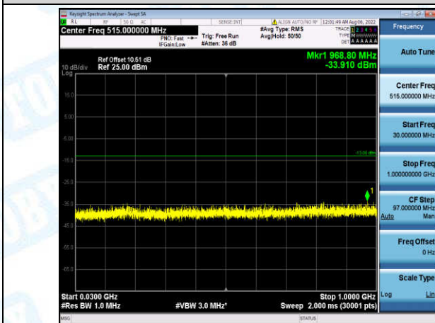
Band4-1.4MHz-16QAM-20393-1-0-High-30-1000--33.91-PASS
