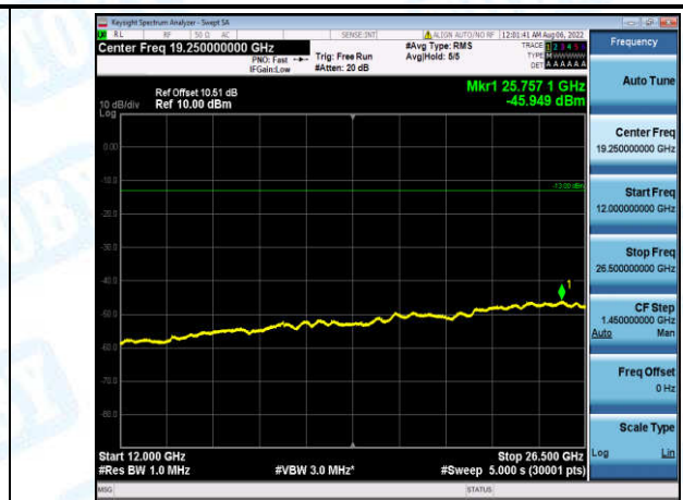
Band4-1.4MHz-QPSK-20393-1-0-High-12000-26500--45.95-PASS
