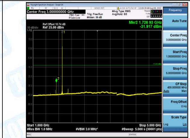
Band2-5MHz-16QAM-19175-1-0-High-1000-5000--31.92-PASS
