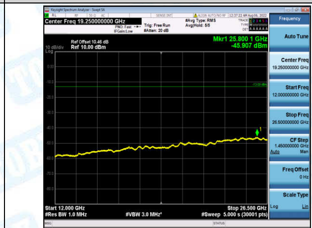
Band4-3MHz-QPSK-20175-1-0-Low-12000-26500--45.91-PASS
