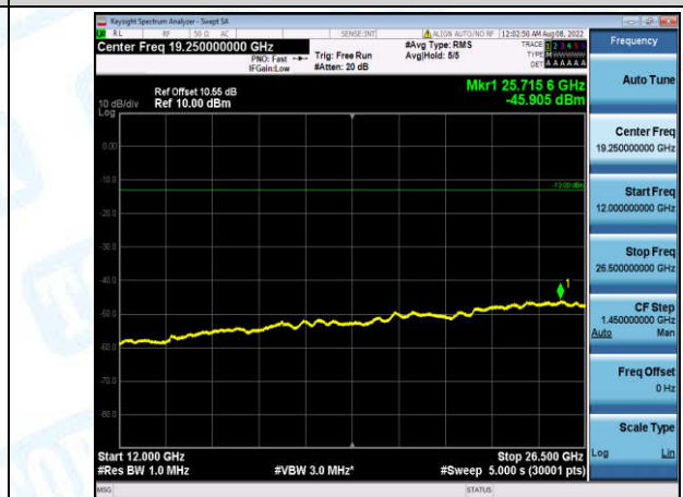
Band2-5MHz-16QAM-18625-1-0-Low-12000-26500--45.91-PASS
