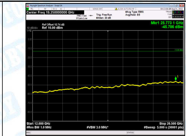
Band2-15MHz-QPSK-19150-1-0-High-12000-26500--45.79-PASS
