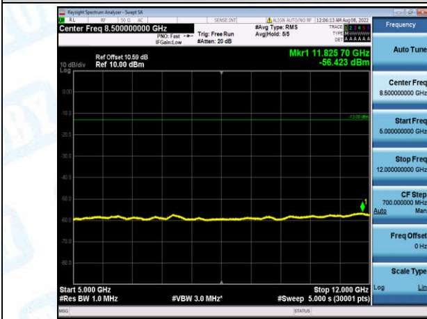
Band2-5MHz-16QAM-18900-1-0-Low-5000-12000--56.42-PASS
