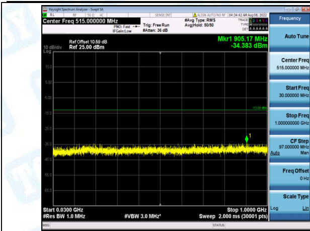
Band2-10MHz-16QAM-18900-1-0-Low-30-1000--34.38-PASS
