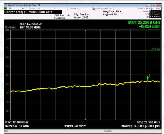
Band2-15MHz-QPSK-18900-1-0-Low-12000-26500--45.82-PASS
