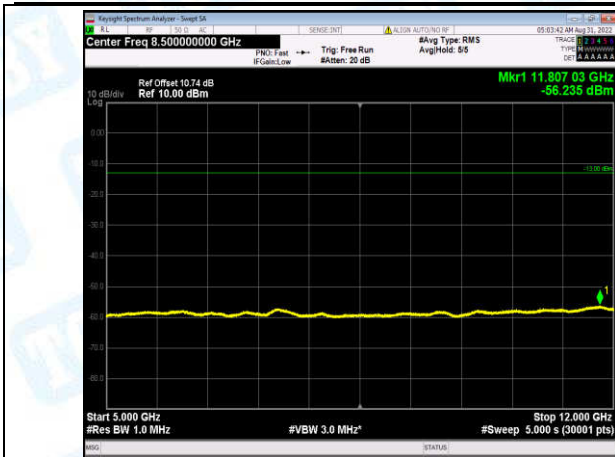
Band2-20MHz-16QAM-19100-1-0-High-5000-12000--56.24-PASS
