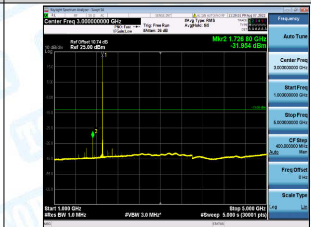
Band2-3MHz-16QAM-19185-1-0-High-1000-5000--31.95-PASS
