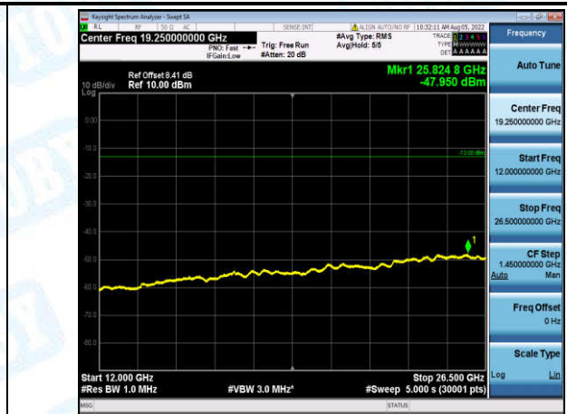
Band12-10MHz-16QAM-23130-1-0-High-12000-26500--47.95-PASS
