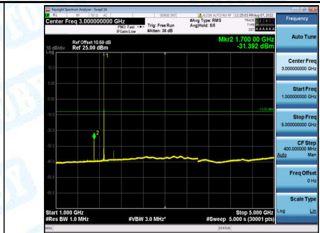
Band2-3MHz-16QAM-18900-1-0-Low-1000-5000--31.39-PASS
