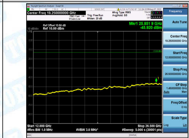
Band2-3MHz-QPSK-18900-1-0-Low-12000-26500--45.92-PASS
