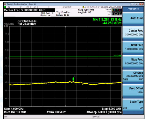
Band12-3MHz-16QAM-23165-1-0-High-1000-5000--43.25-PASS
