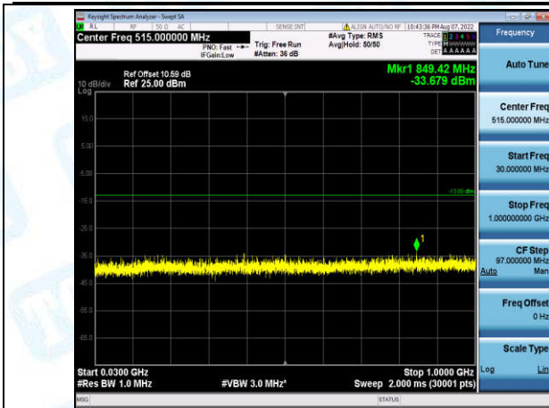
Band2-1.4MHz-16QAM-18900-1-0-Low-30-1000--33.68-PASS
