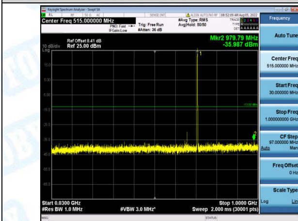
Band12-5MHz-QPSK-23155-1-0-High-30-1000--35.99-PASS
