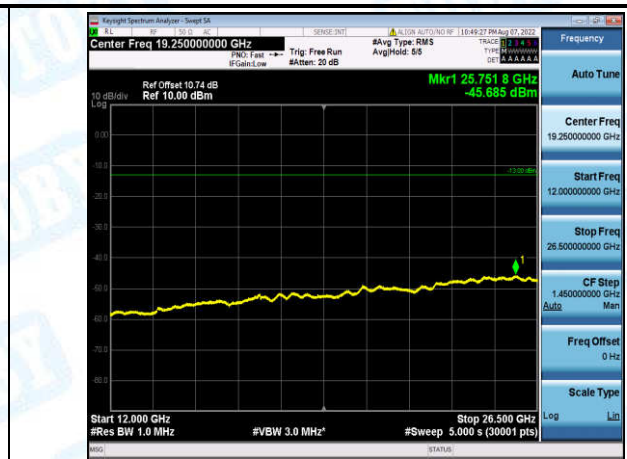
Band2-1.4MHz-16QAM-19193-1-0-High-12000-26500--45.69-PASS
