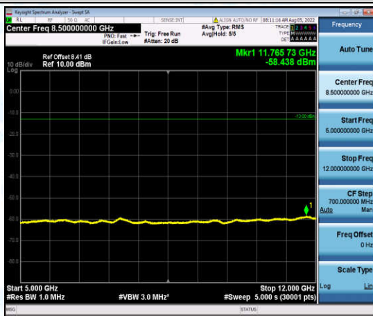
Band12-3MHz-16QAM-23095-1-0-Low-5000-12000--58.44-PASS
