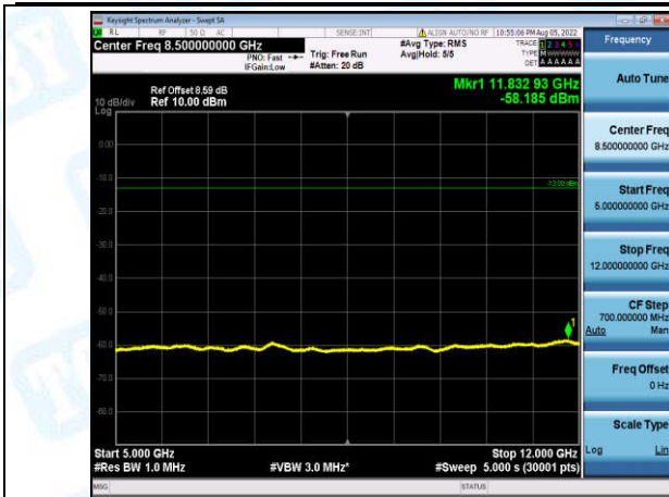
Band13-5MHz-QPSK-23255-1-0-High-5000-12000--58.19-PASS
