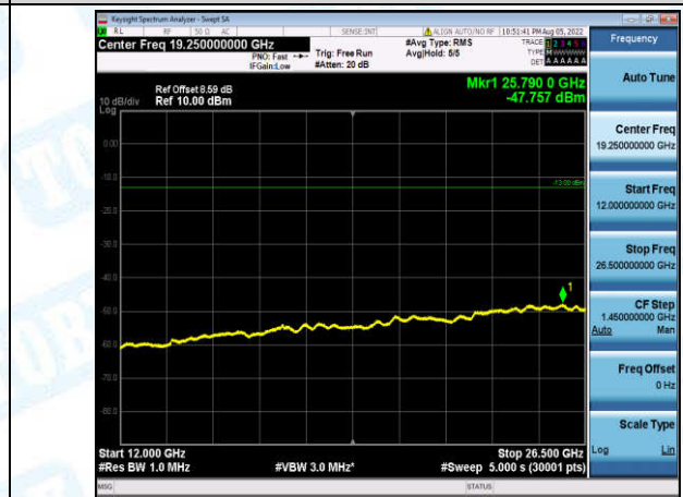
Band13-5MHz-QPSK-23230-1-0-Low-12000-26500--47.76-PASS
