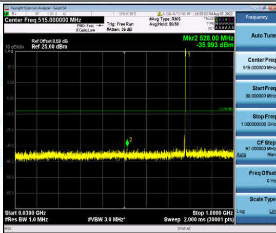
Band13-5MHz-16QAM-23255-1-0-High-30-1000--35.99-PASS
