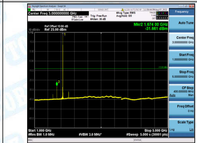
Band2-5MHz-QPSK-18625-1-0-Low-1000-5000--31.66-PASS
