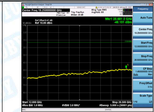
Band12-5MHz-16QAM-23155-1-0-High-12000-26500--48.15-PASS
