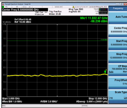
Band13-5MHz-16QAM-23230-1-0-Low-5000-12000--58.24-PASS
