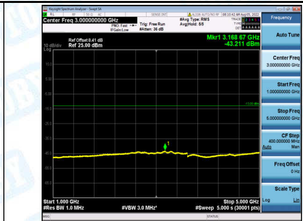
Band12-3MHz-16QAM-23095-1-0-Low-1000-5000--43.21-PASS
