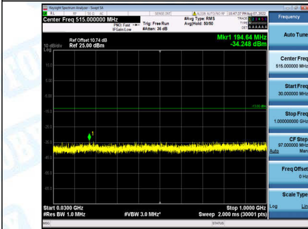
Band2-1.4MHz-16QAM-19193-1-0-High-30-1000--34.25-PASS
