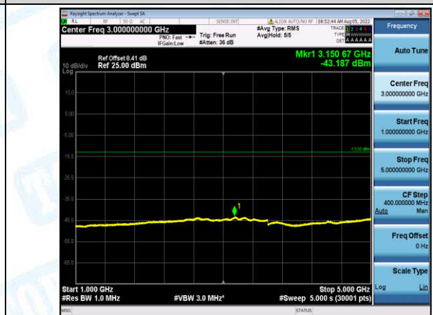
Band12-5MHz-QPSK-23155-1-0-High-1000-5000--43.19-PASS
