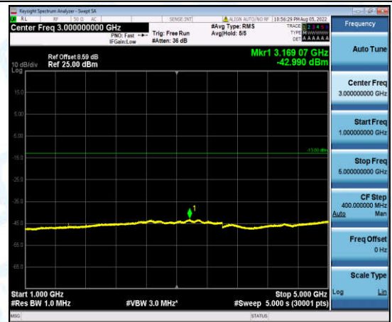
Band13-5MHz-16QAM-23255-1-0-High-1000-5000--42.99-PASS
