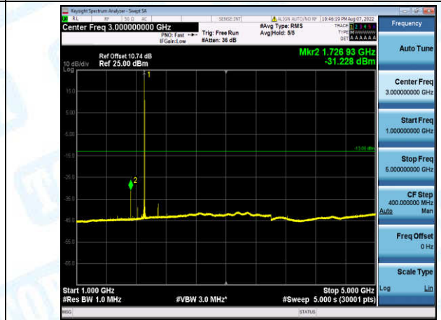
Band2-1.4MHz-QPSK-19193-1-0-High-1000-5000--31.23-PASS
