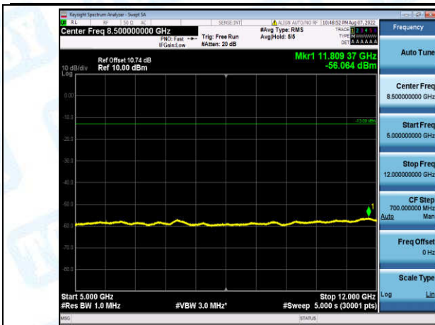
Band2-1.4MHz-16QAM-19193-1-0-High-5000-12000--56.06-PASS
