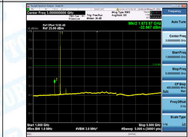
Band2-1.4MHz-16QAM-18607-1-0-Low-1000-5000--32.67-PASS
