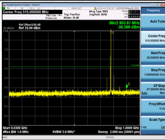
Band13-5MHz-QPSK-23255-1-0-High-30-1000--36.39-PASS
