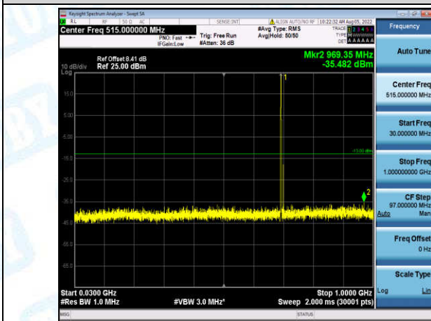
Band12-10MHz-16QAM-23060-1-0-Low-30-1000--35.48-PASS
