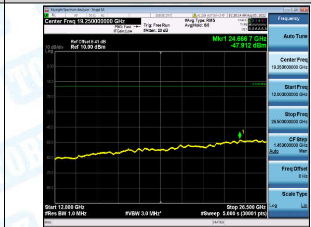
Band12-10MHz-16QAM-23095-1-0-Low-12000-26500--47.91-PASS
