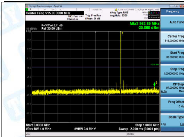
Band12-10MHz-16QAM-23095-1-0-Low-30-1000--35.86-PASS
