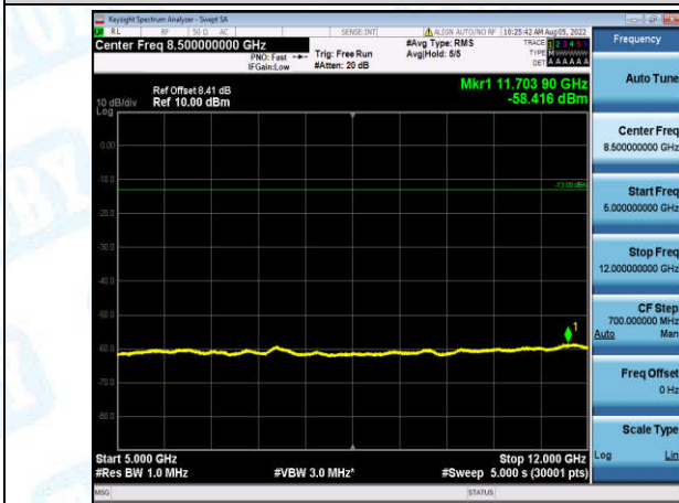
Band12-10MHz-QPSK-23095-1-0-Low-5000-12000--58.42-PASS
