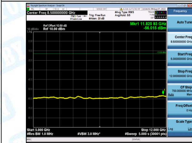
Band2-1.4MHz-16QAM-18900-1-0-Low-5000-12000--56.02-PASS
