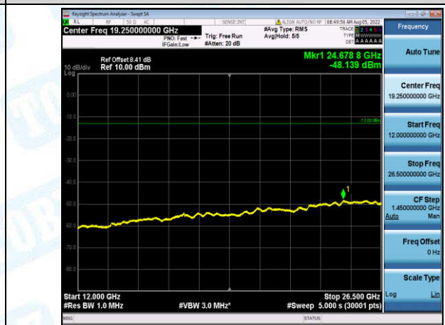
Band12-5MHz-QPSK-23095-1-0-Low-12000-26500--48.14-PASS
