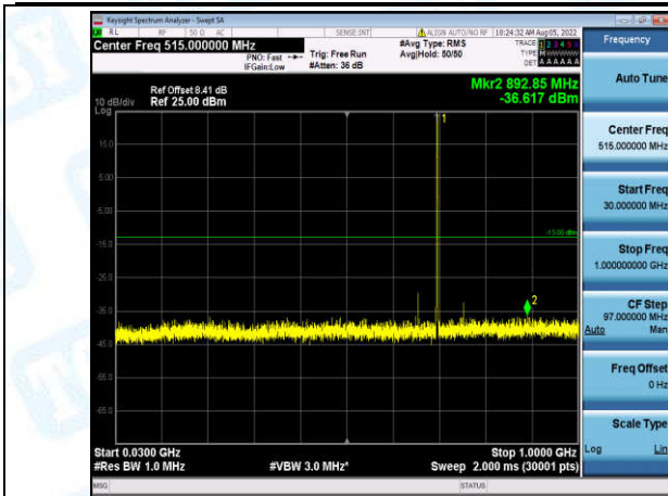
Band12-10MHz-QPSK-23095-1-0-Low-30-1000--36.62-PASS
