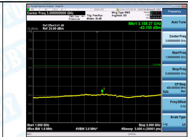
Band12-10MHz-16QAM-23095-1-0-Low-1000-5000--43.11-PASS
