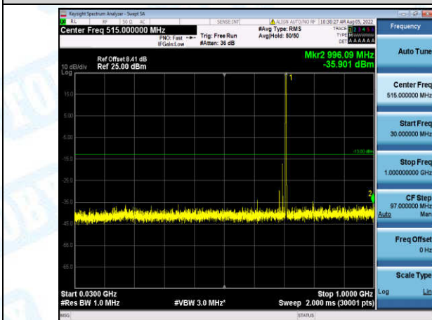
Band12-10MHz-16QAM-23130-1-0-High-30-1000--35.9-PASS
