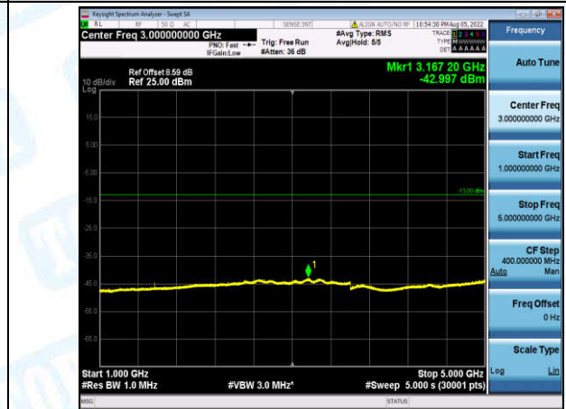
Band13-5MHz-QPSK-23255-1-0-High-1000-5000--43-PASS
