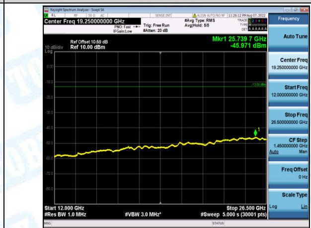
Band2-3MHz-16QAM-18900-1-0-Low-12000-26500--45.97-PASS
