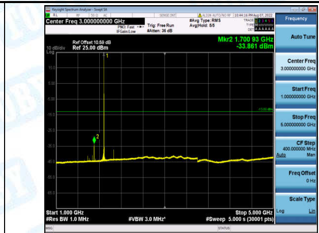
Band2-1.4MHz-16QAM-18900-1-0-Low-1000-5000--33.86-PASS
