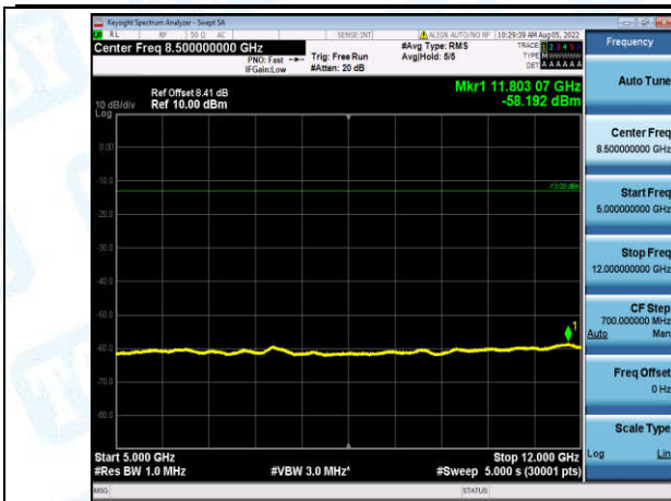
Band12-10MHz-QPSK-23130-1-0-High-5000-12000--58.19-PASS
