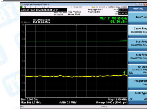
Band13-5MHz-16QAM-23255-1-0-High-5000-12000--58.2-PASS
