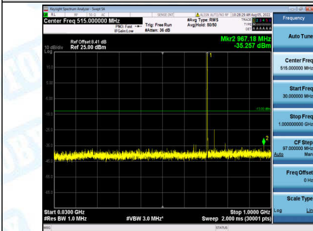
Band12-10MHz-QPSK-23130-1-0-High-30-1000--35.26-PASS
