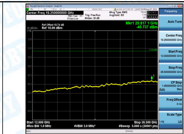
Band2-1.4MHz-QPSK-19193-1-0-High-12000-26500--45.74-PASS
