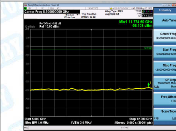
Band2-1.4MHz-QPSK-18900-1-0-Low-5000-12000--56.11-PASS
