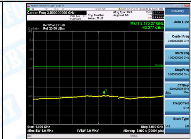
Band12-5MHz-QPSK-23095-1-0-Low-1000-5000--43.28-PASS
