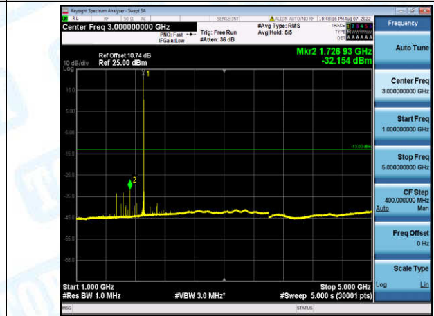
Band2-1.4MHz-16QAM-19193-1-0-High-1000-5000--32.15-PASS
