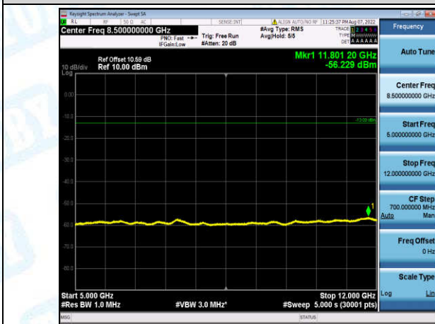
Band2-3MHz-16QAM-18900-1-0-Low-5000-12000--56.23-PASS
