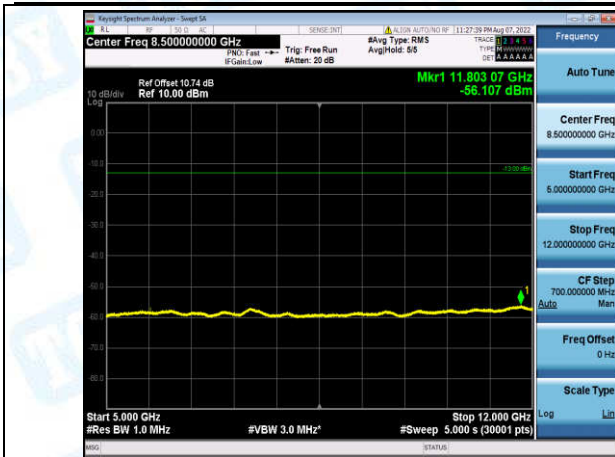
Band2-3MHz-QPSK-19185-1-0-High-5000-12000--56.11-PASS
