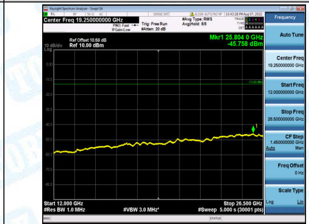
Band2-1.4MHz-QPSK-18900-1-0-Low-12000-26500--45.76-PASS
