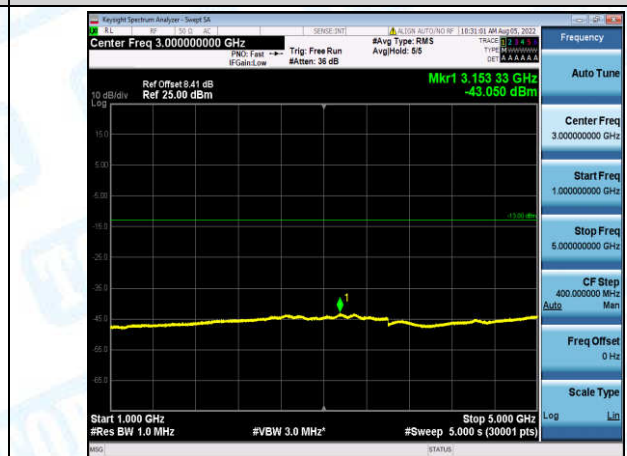
Band12-10MHz-16QAM-23130-1-0-High-1000-5000--43.05-PASS
