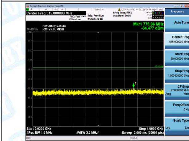
Band2-5MHz-QPSK-18625-1-0-Low-30-1000--34.48-PASS
