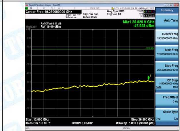
Band12-10MHz-QPSK-23095-1-0-Low-12000-26500--47.93-PASS
