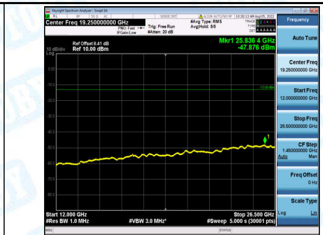
Band12-10MHz-QPSK-23130-1-0-High-12000-26500--47.88-PASS
