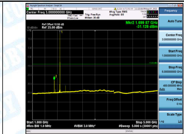
Band2-3MHz-QPSK-18900-1-0-Low-1000-5000--31.13-PASS
