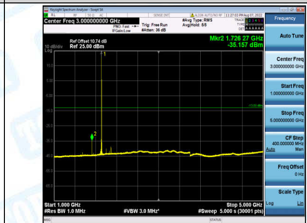
Band2-3MHz-QPSK-19185-1-0-High-1000-5000--35.16-PASS
