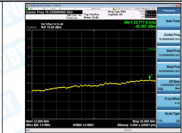
Band2-3MHz-QPSK-19185-1-0-High-12000-26500--45.59-PASS
