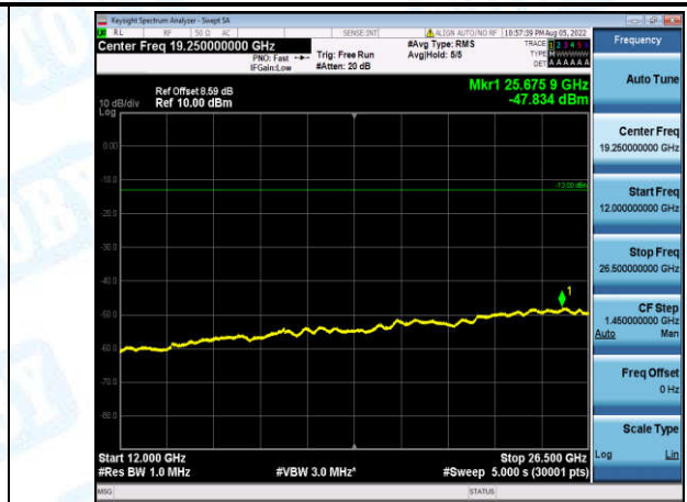
Band13-5MHz-16QAM-23255-1-0-High-12000-26500--47.83-PASS
