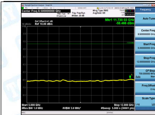
Band12-5MHz-QPSK-23155-1-0-High-5000-12000--58.47-PASS
