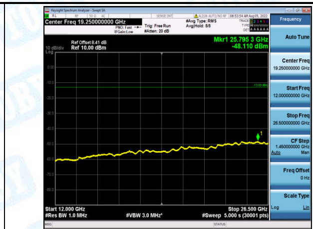
Band12-5MHz-QPSK-23155-1-0-High-12000-26500--48.11-PASS
