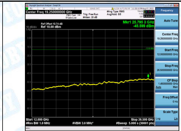
Band2-3MHz-16QAM-19185-1-0-High-12000-26500--45.6-PASS
