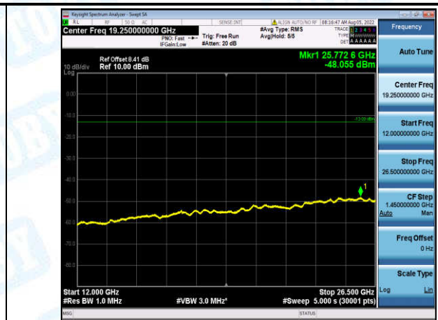
Band12-3MHz-16QAM-23165-1-0-High-12000-26500--48.06-PASS
