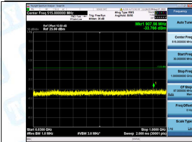
Band2-3MHz-16QAM-18900-1-0-Low-30-1000--33.77-PASS
