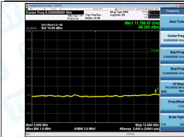
Band12-10MHz-16QAM-23130-1-0-High-5000-12000--58.2-PASS
