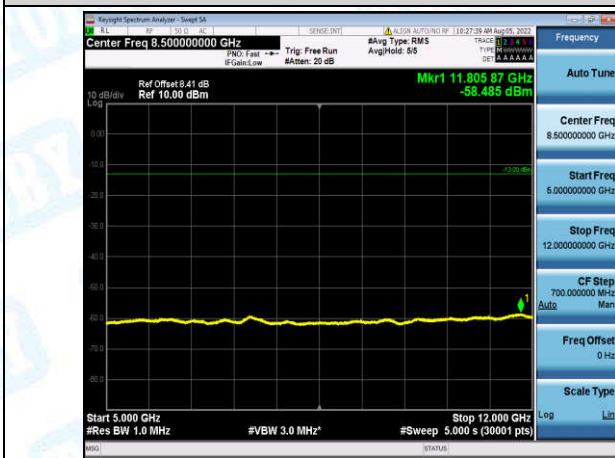
Band12-10MHz-16QAM-23095-1-0-Low-5000-12000--58.49-PASS
