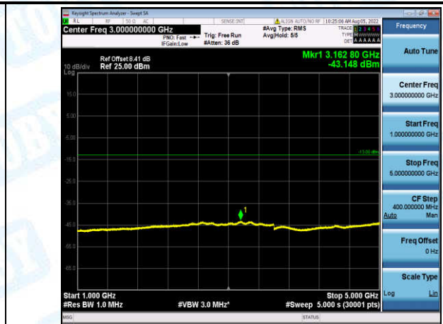
Band12-10MHz-QPSK-23095-1-0-Low-1000-5000--43.15-PASS
