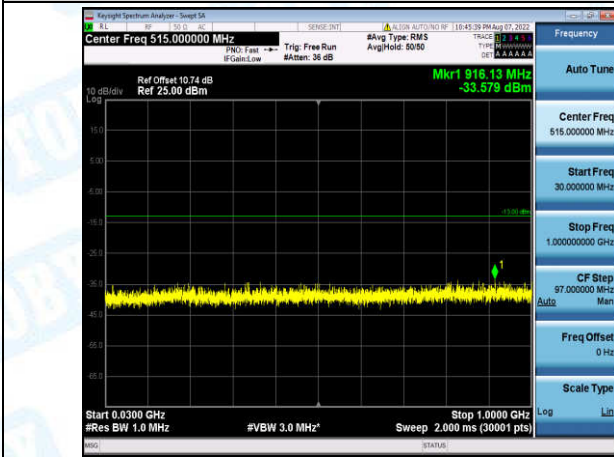
Band2-1.4MHz-QPSK-19193-1-0-High-30-1000--33.58-PASS
