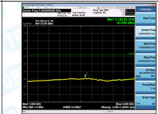
Band12-10MHz-16QAM-23060-1-0-Low-1000-5000--43.06-PASS
