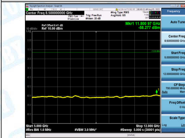
Band12-5MHz-QPSK-23095-1-0-Low-5000-12000--58.28-PASS
