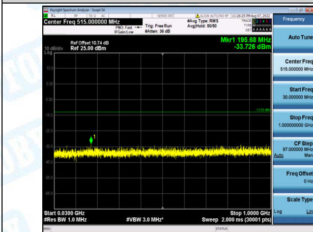
Band2-3MHz-QPSK-19185-1-0-High-30-1000--33.73-PASS
