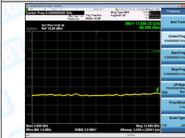
Band2-3MHz-QPSK-18900-1-0-Low-5000-12000--56.4-PASS
