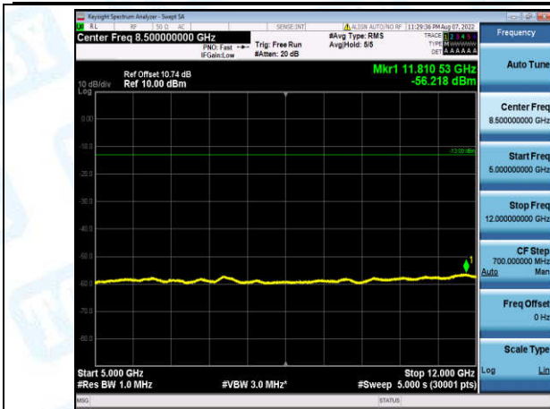
Band2-3MHz-16QAM-19185-1-0-High-5000-12000--56.22-PASS
