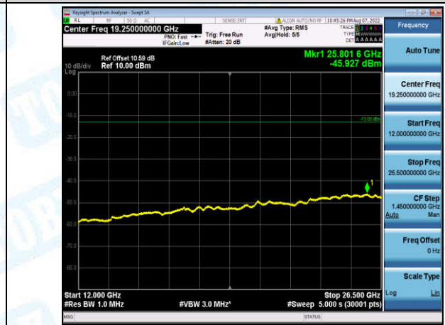
Band2-1.4MHz-16QAM-18900-1-0-Low-12000-26500--45.93-PASS
