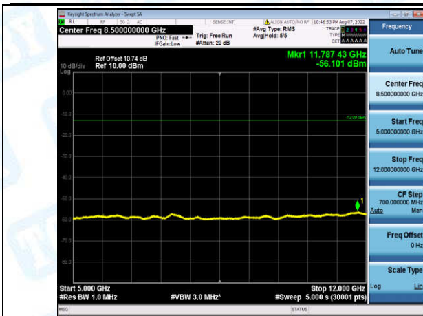
Band2-1.4MHz-QPSK-19193-1-0-High-5000-12000--56.1-PASS
