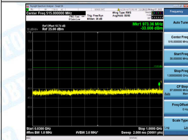
Band2-3MHz-16QAM-19185-1-0-High-30-1000--33.01-PASS
