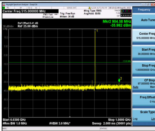
Band12-3MHz-16QAM-23165-1-0-High-30-1000--35.98-PASS
