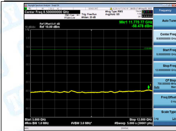
Band12-5MHz-16QAM-23155-1-0-High-5000-12000--58.48-PASS
