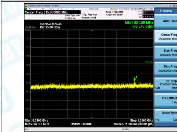
Band2-1.4MHz-16QAM-18607-1-0-Low-30-1000--33.58-PASS
