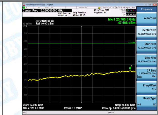
Band13-5MHz-QPSK-23255-1-0-High-12000-26500--47.61-PASS
