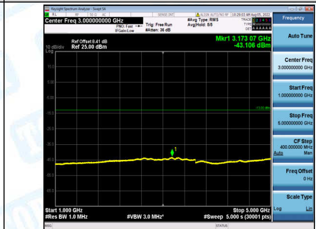
Band12-10MHz-QPSK-23130-1-0-High-1000-5000--43.11-PASS
