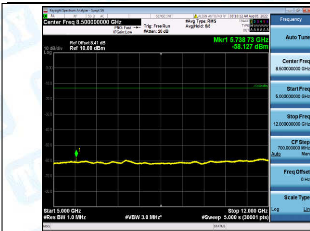
Band12-3MHz-16QAM-23165-1-0-High-5000-12000--58.13-PASS
