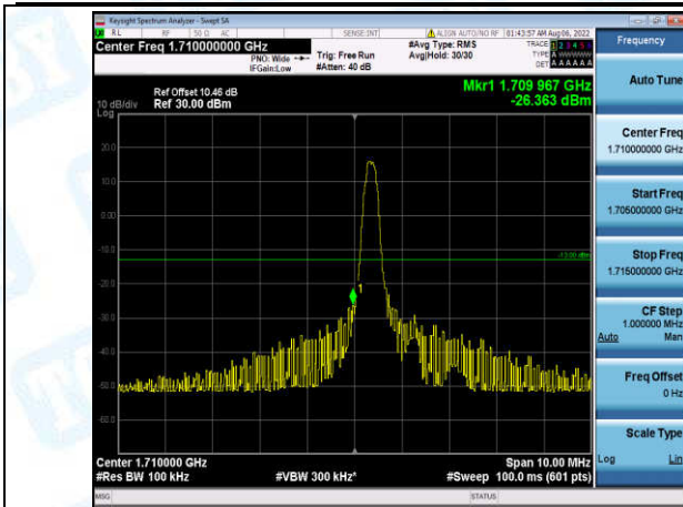
Band4-5MHz-16QAM-19975-1-0-Low--26.36-PASS
