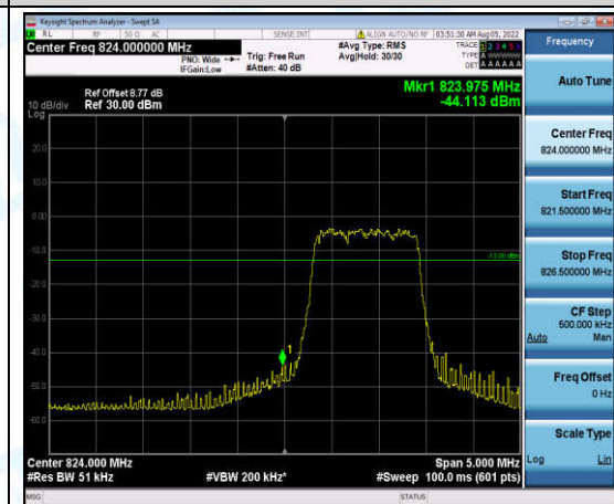
Band5-3MHz-16QAM-20415-6-0-Low--44.11-PASS
