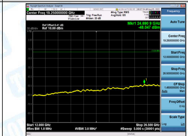
Band12-3MHz-16QAM-23025-1-0-Low-12000-26500--48.05-PASS
