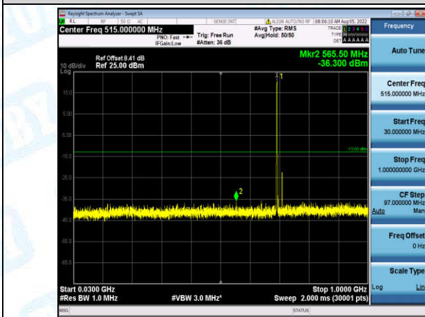
Band12-3MHz-16QAM-23025-1-0-Low-30-1000--36.3-PASS
