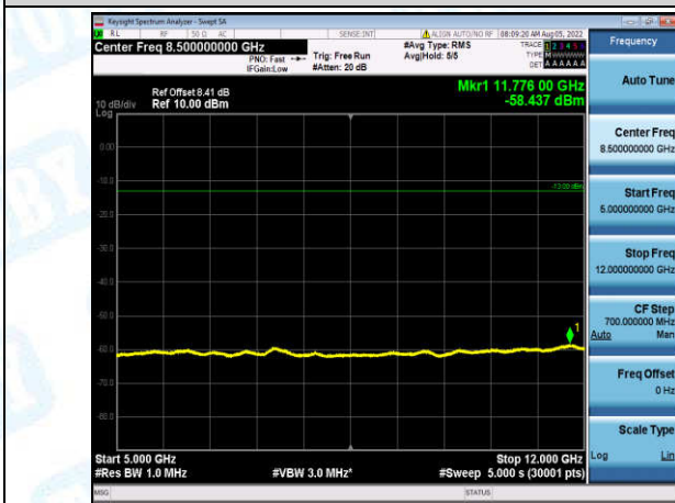
Band12-3MHz-QPSK-23095-1-0-Low-5000-12000--58.44-PASS
