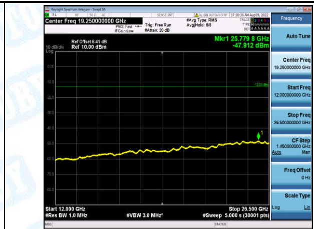
Band12-1.4MHz-QPSK-23173-1-0-High-12000-26500--47.91-PASS
