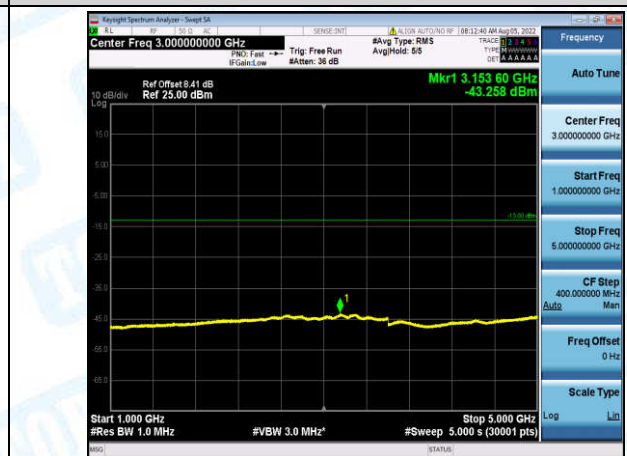
Band12-3MHz-QPSK-23165-1-0-High-1000-5000--43.26-PASS
