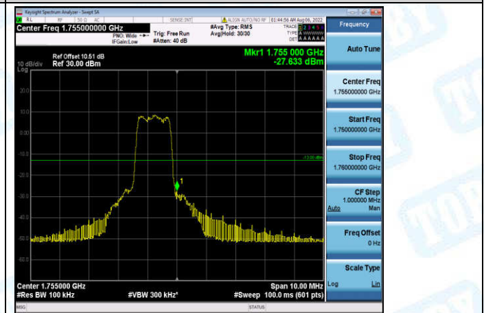
Band4-5MHz-QPSK-20375-6-0-High--27.63-PASS
