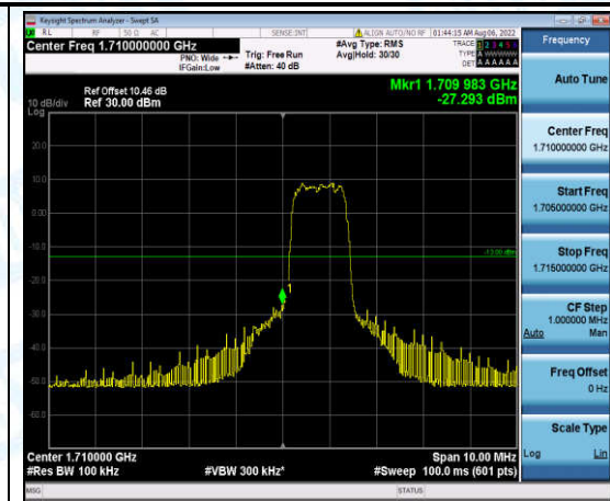
Band4-5MHz-16QAM-19975-6-0-Low--27.29-PASS
