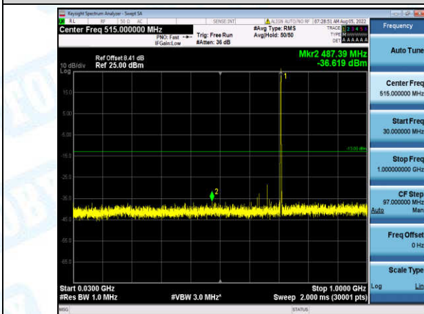
Band12-1.4MHz-QPSK-23173-1-0-High-30-1000--36.62-PASS
