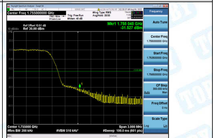
Band4-10MHz-16QAM-20350-6-0-High--31.53-PASS
