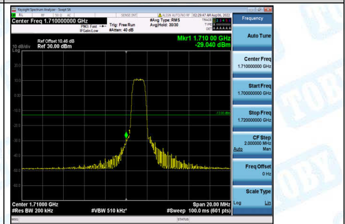
Band4-10MHz-16QAM-20000-6-0-Low--29.04-PASS
