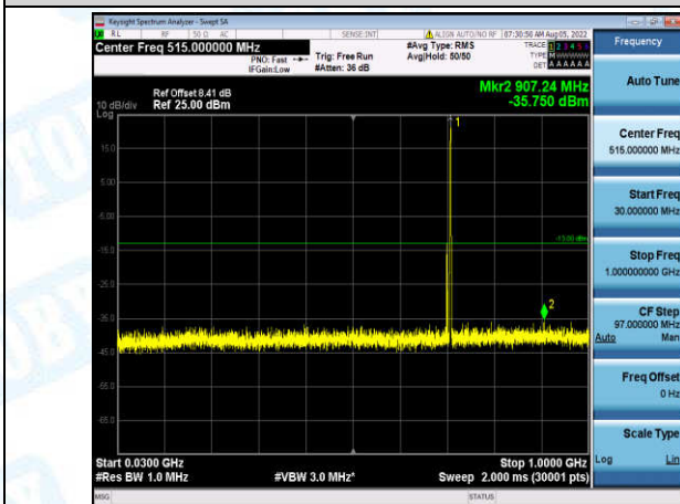
Band12-1.4MHz-16QAM-23173-1-0-High-30-1000--35.75-PASS
