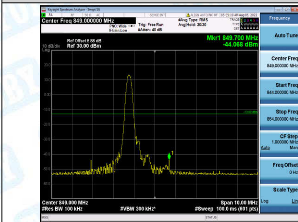
Band5-5MHz-16QAM-20625-1-0-High--44.07-PASS
