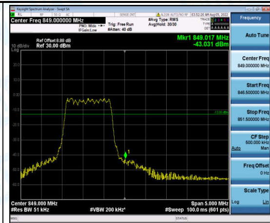
Band5-3MHz-16QAM-20635-6-0-High--43.03-PASS
