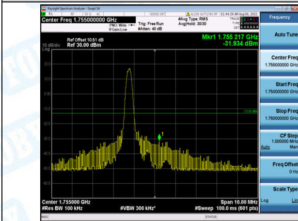
Band4-5MHz-QPSK-20375-1-0-High--31.93-PASS
