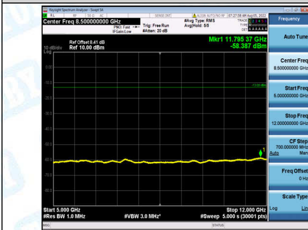
Band12-1.4MHz-16QAM-23095-1-0-Low-5000-12000--58.39-PASS
