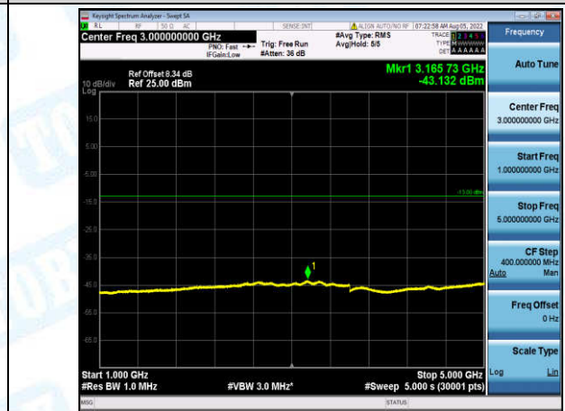
Band12-1.4MHz-16QAM-23017-1-0-Low-1000-5000--43.13-PASS
