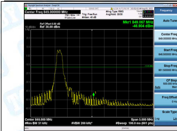
Band5-3MHz-16QAM-20635-1-0-High--46.90-PASS
