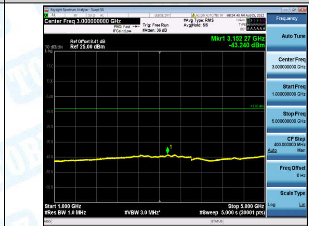
Band12-3MHz-QPSK-23025-1-0-Low-1000-5000--43.24-PASS
