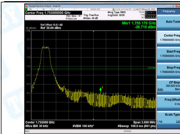
Band4-1.4MHz-QPSK-20393-1-0-High--38.72-PASS
