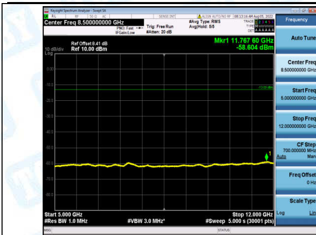
Band12-3MHz-QPSK-23165-1-0-High-5000-12000--58.6-PASS
