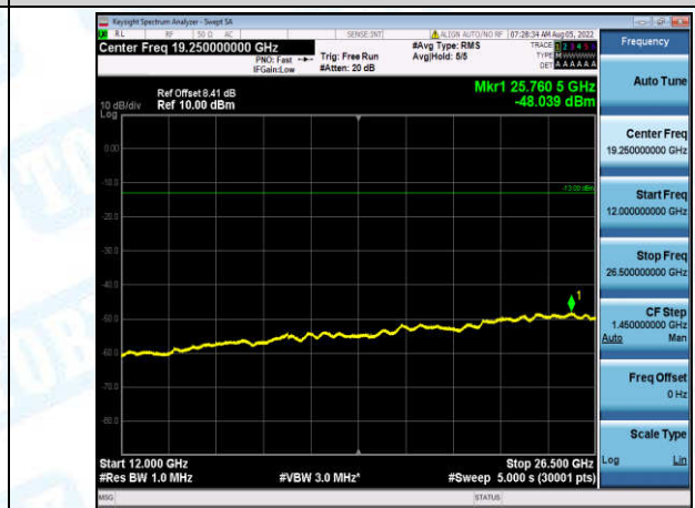
Band12-1.4MHz-16QAM-23095-1-0-Low-12000-26500--48.04-PASS
