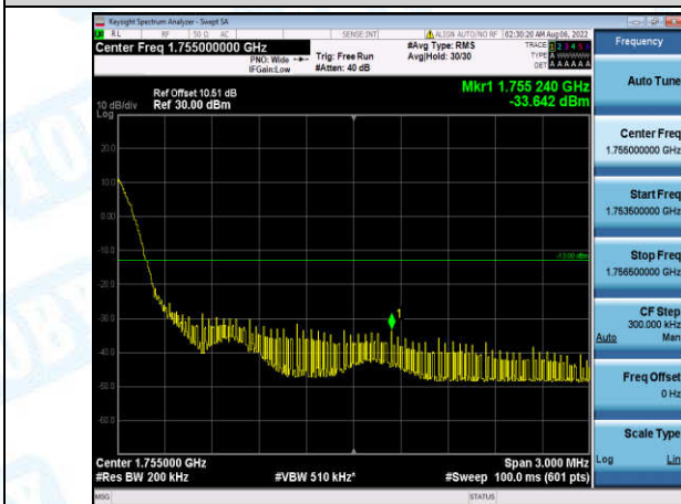
Band4-10MHz-16QAM-20350-1-0-High--33.64-PASS
