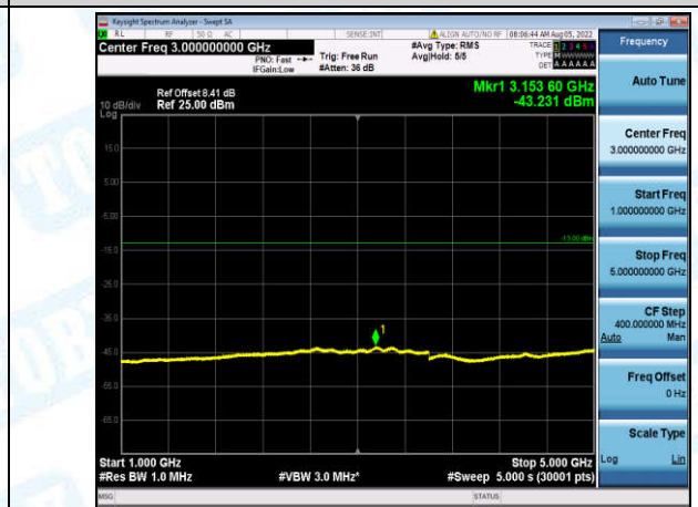
Band12-3MHz-16QAM-23025-1-0-Low-1000-5000--43.23-PASS
