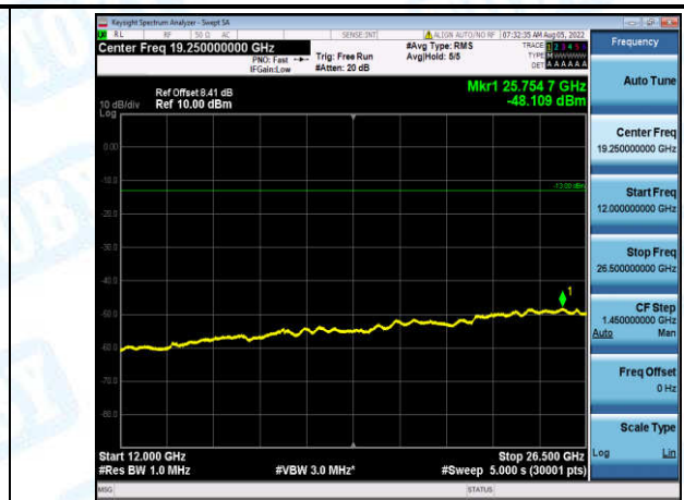
Band12-1.4MHz-16QAM-23173-1-0-High-12000-26500--48.11-PASS
