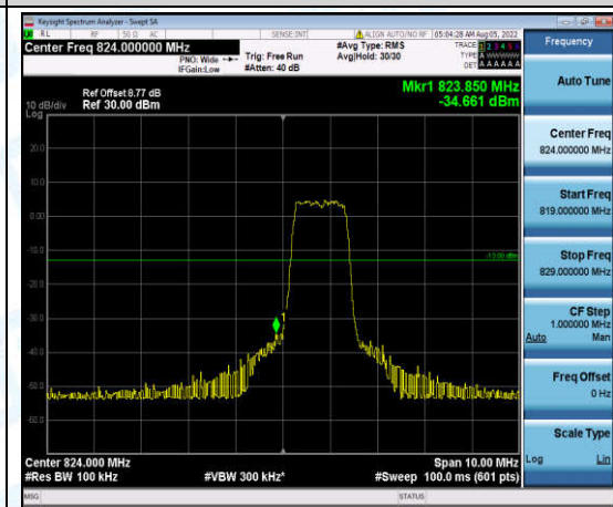
Band5-5MHz-QPSK-20425-6-0-Low--34.66-PASS
