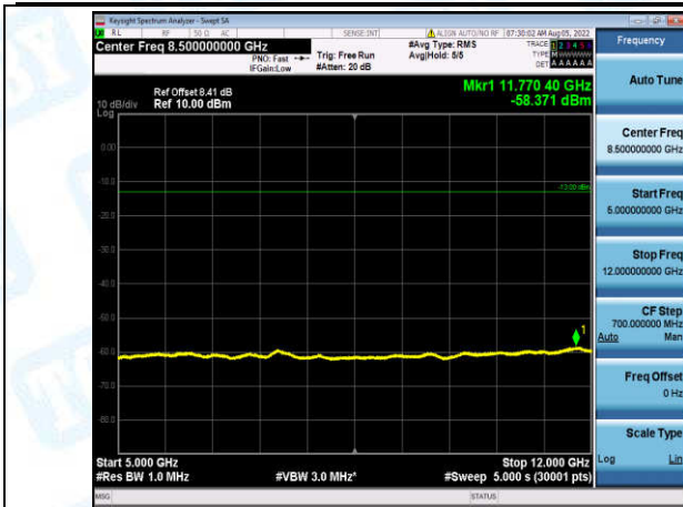
Band12-1.4MHz-QPSK-23173-1-0-High-5000-12000--58.37-PASS
