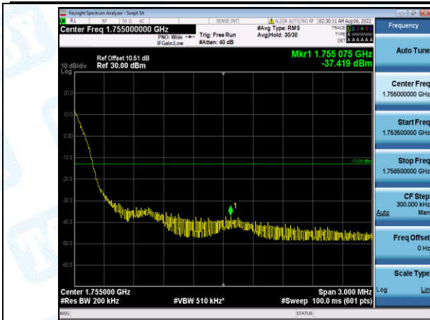
Band4-10MHz-QPSK-20350-1-0-High--37.42-PASS
