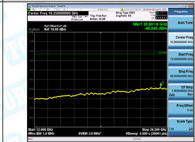
Band12-3MHz-QPSK-23095-1-0-Low-12000-26500--48.04-PASS
