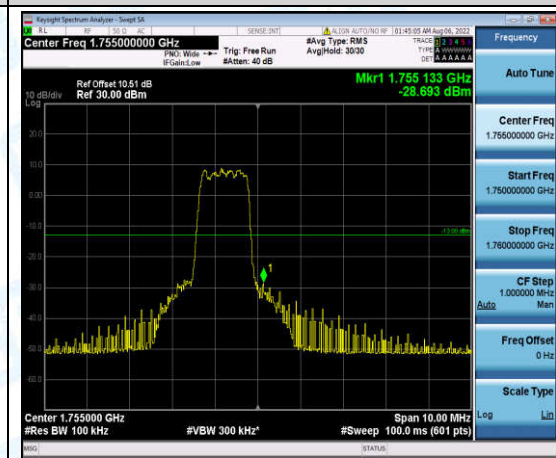
Band4-5MHz-16QAM-20375-6-0-High--28.69-PASS
