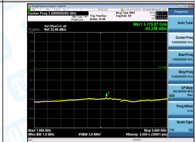
Band12-1.4MHz-QPSK-23173-1-0-High-1000-5000--43.25-PASS
