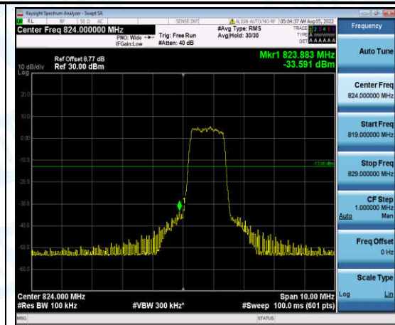
Band5-5MHz-16QAM-20425-6-0-Low--33.59-PASS
