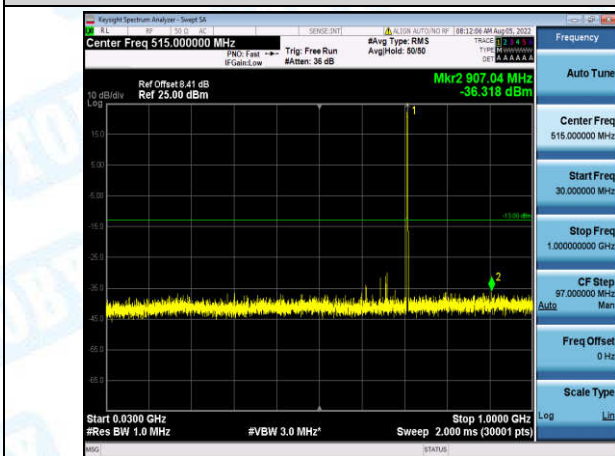
Band12-3MHz-QPSK-23165-1-0-High-30-1000--36.32-PASS
