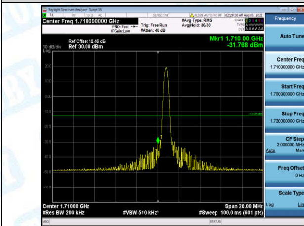
Band4-10MHz-16QAM-20000-1-0-Low--31.77-PASS
