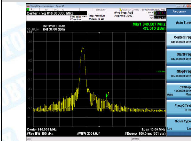
Band5-5MHz-QPSK-20625-1-0-High--39.51-PASS
