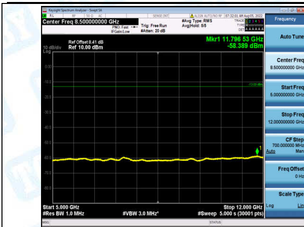
Band12-1.4MHz-16QAM-23173-1-0-High-5000-12000--58.39-PASS
