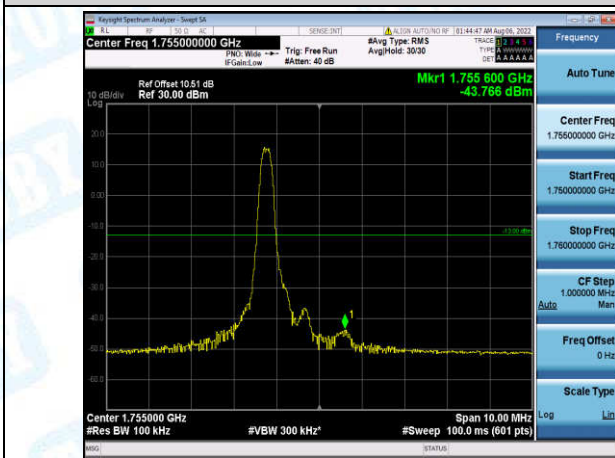
Band4-5MHz-16QAM-20375-1-0-High--43.77-PASS
