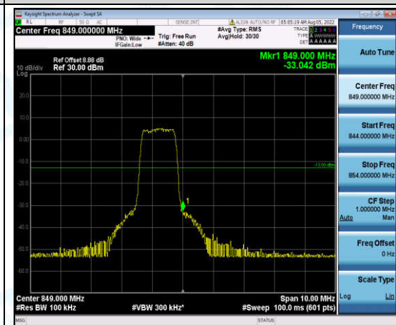
Band5-5MHz-QPSK-20625-6-0-High--33.04-PASS
