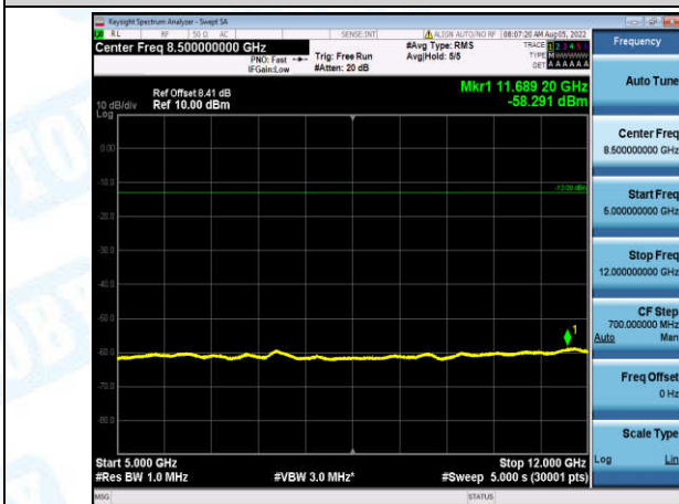
Band12-3MHz-16QAM-23025-1-0-Low-5000-12000--58.29-PASS
