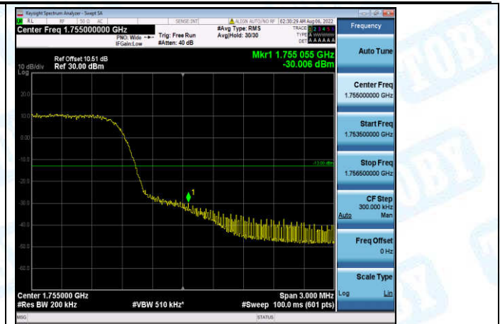
Band4-10MHz-QPSK-20350-6-0-High--30.01-PASS
