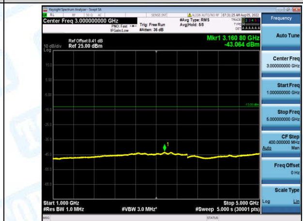
Band12-1.4MHz-16QAM-23173-1-0-High-1000-5000--43.06-PASS
