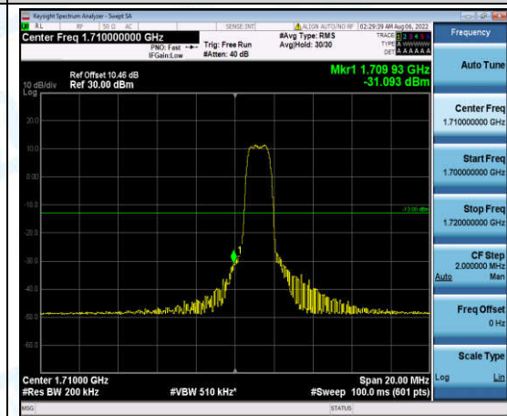
Band4-10MHz-QPSK-20000-6-0-Low--31.09-PASS
