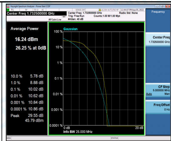
Band4-1.4MHz-QPSK-20175-6-0-Low-10.02-<=13-PASS
