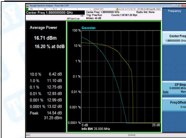
Band2-15MHz-16QAM-18900-1-0-Low-12.75-<=13-PASS
