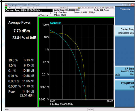
Band5-3MHz-16QAM-20415-6-0-Low-10.36-<=13-PASS
