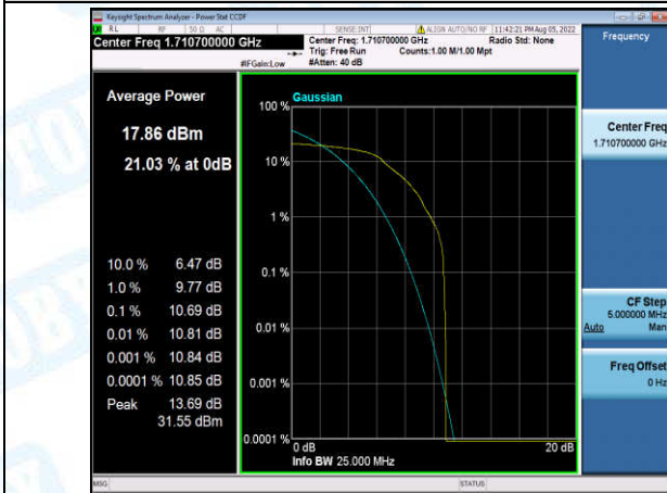
Band4-1.4MHz-QPSK-19957-1-0-Low-10.69-<=13-PASS
