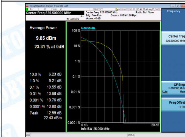
Band5-3MHz-16QAM-20415-1-0-Low-10.55-<=13-PASS
