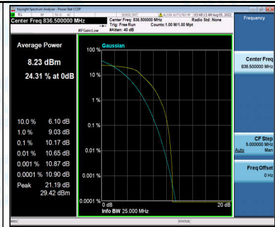
Band5-3MHz-16QAM-20525-6-0-Low-10.17-<=13-PASS
