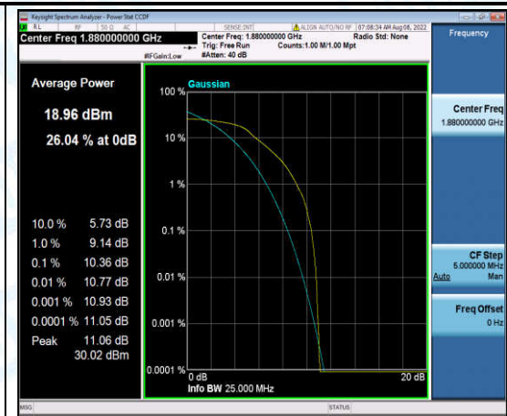
Band2-15MHz-16QAM-18900-6-0-Low-10.36-<=13-PASS
