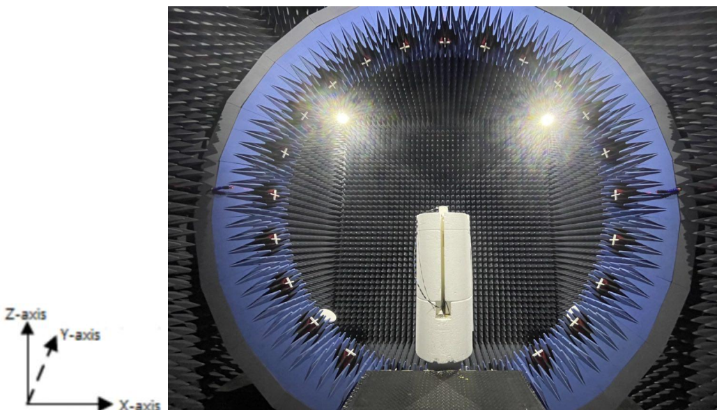
Front view
