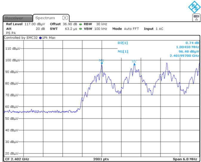
Figure 8.4-4: Carrier frequency separation
