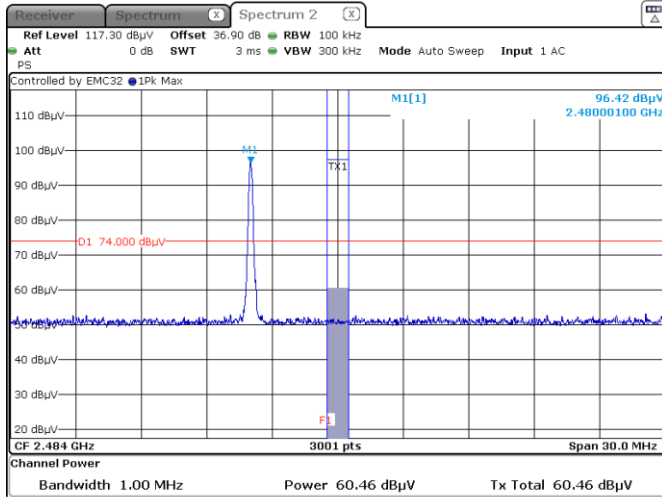
Figure 8.6-10: Band edge spurious emissions at 2483.5 MHz Peak – Hopping OFF
