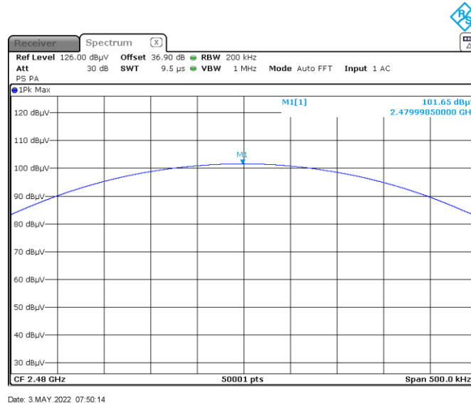
Figure 8.5-3: Output power on high channel
