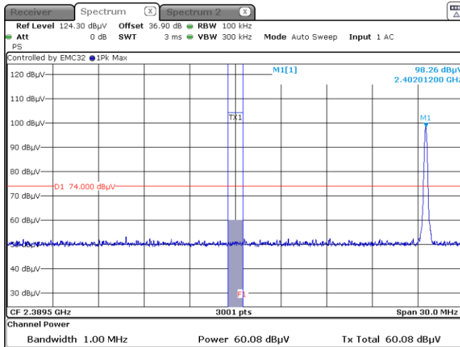
Figure 8.6-8: Band edge spurious emissions at 2390 MHz Peak – Hopping OFF
