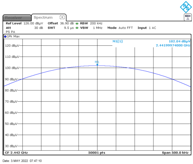
Figure 8.5-2: Output power on mid channel
