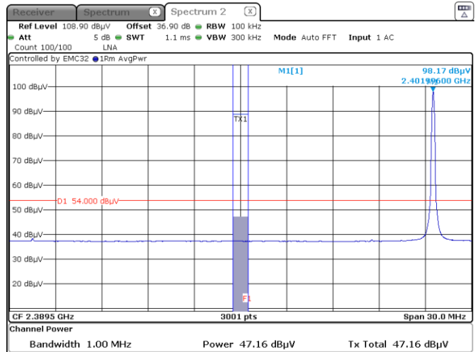
Figure 8.6-9: Band edge spurious emissions at 2390 MHz Average – Hopping OFF
