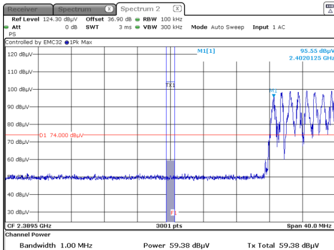
Figure 8.6-12: Band edge spurious emissions at 2390 MHz Peak – Hopping ON
