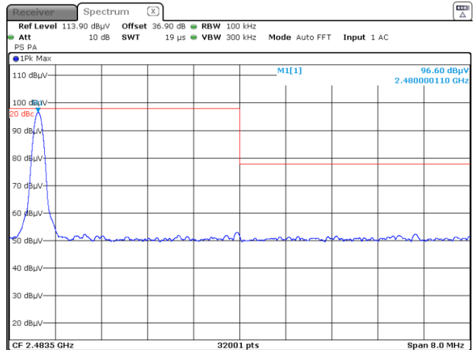
Figure 8.6-18: Non-restricted band edge at 2483.5 MHz, high channel
