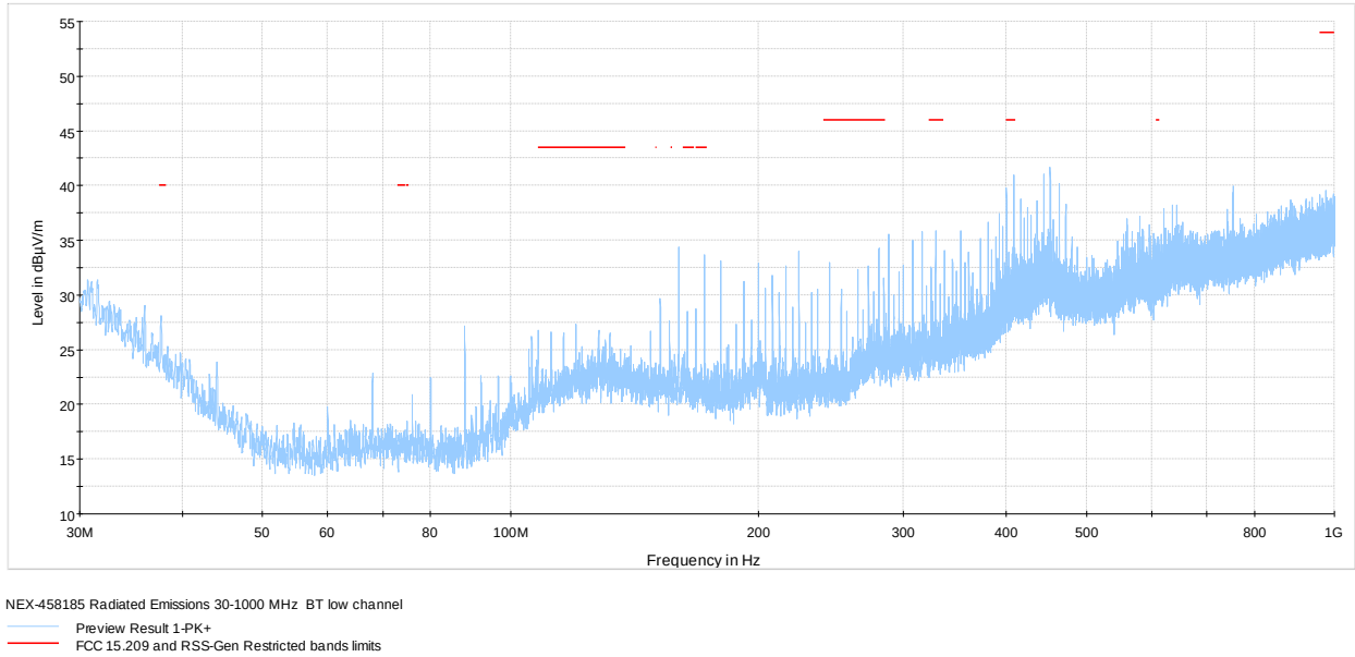
Figure 8.6-1: Radiated spurious emissions 30-1000 MHz low channel
