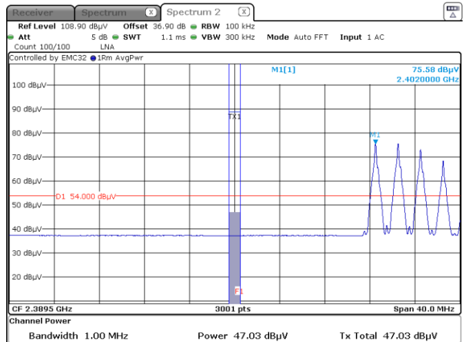
Figure 8.6-13: Band edge spurious emissions at 2390 MHz Average – Hopping ON
