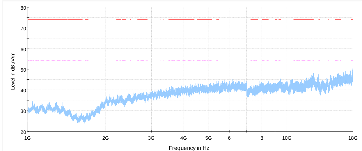
Figure 8.6-5: Radiated spurious emissions 1-18 GHz mid channel
