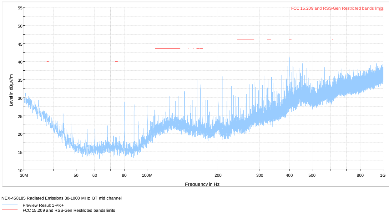
Figure 8.6-2: Radiated spurious emissions 30-1000 MHz mid channel
