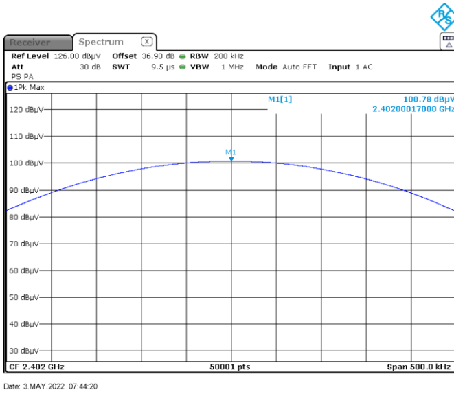
Figure 8.5-1: Output power on low channel
