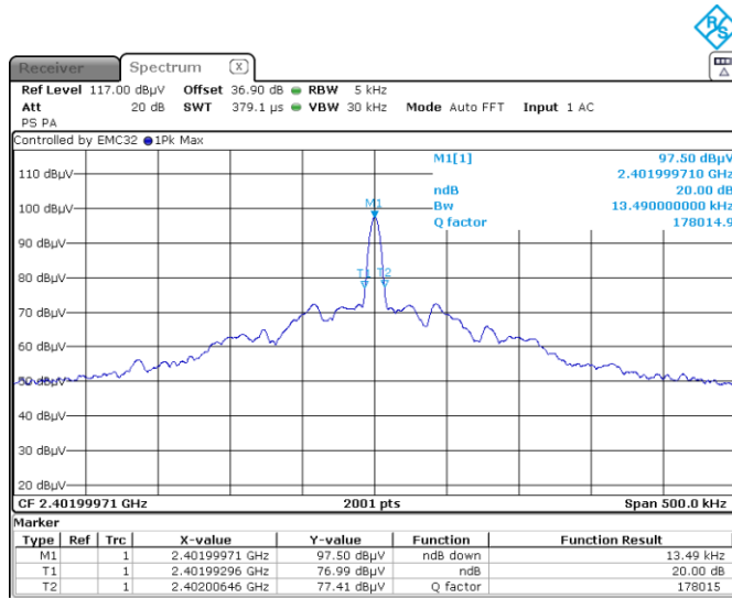
Figure 8.4-1: 20 dB bandwidth on low channel
