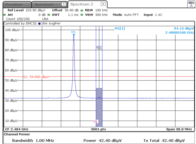
Figure 8.6-11: Band edge spurious emissions at 2483.5 MHz Average – Hopping OFF
