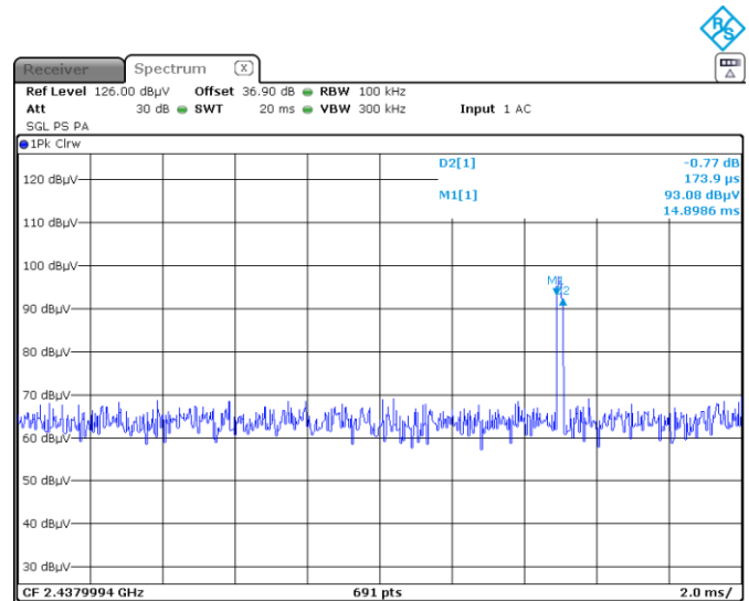
Figure 7.5-6: Dwell time
