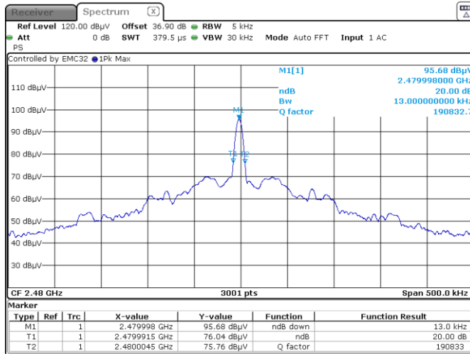
Figure 7.5-3: 20 dB bandwidth on high channel
