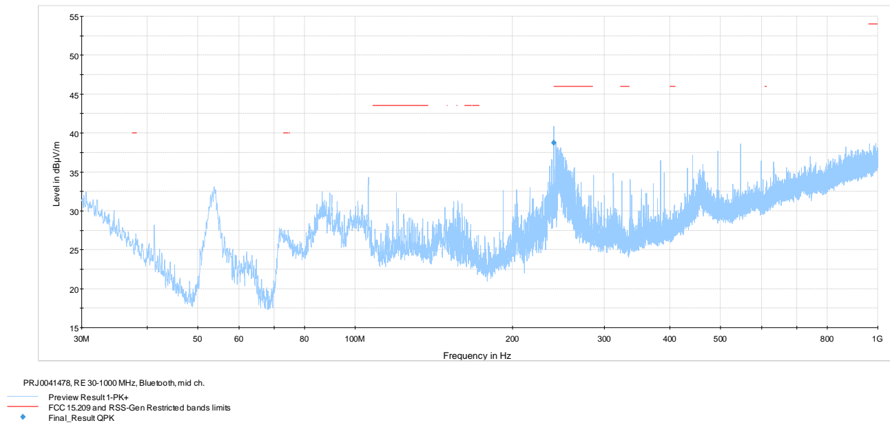
Figure 7.7-2: Radiated spurious emissions 30-1000 MHz mid channel
