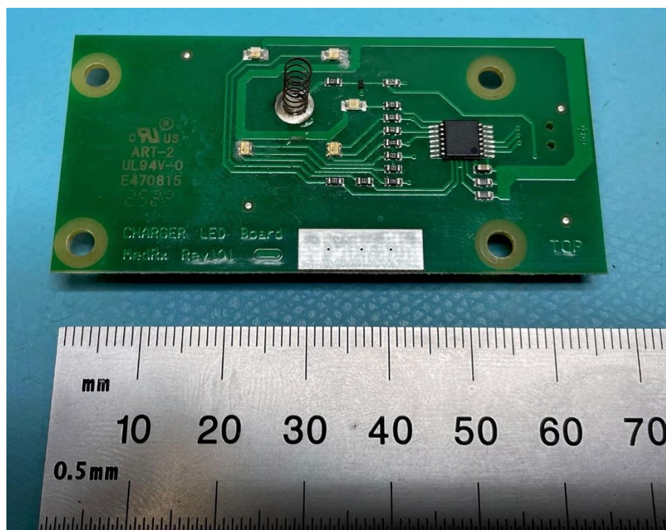
LED Board top view
