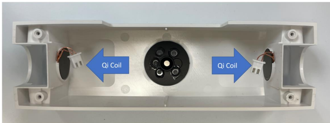
Qi Coil antennas' location
