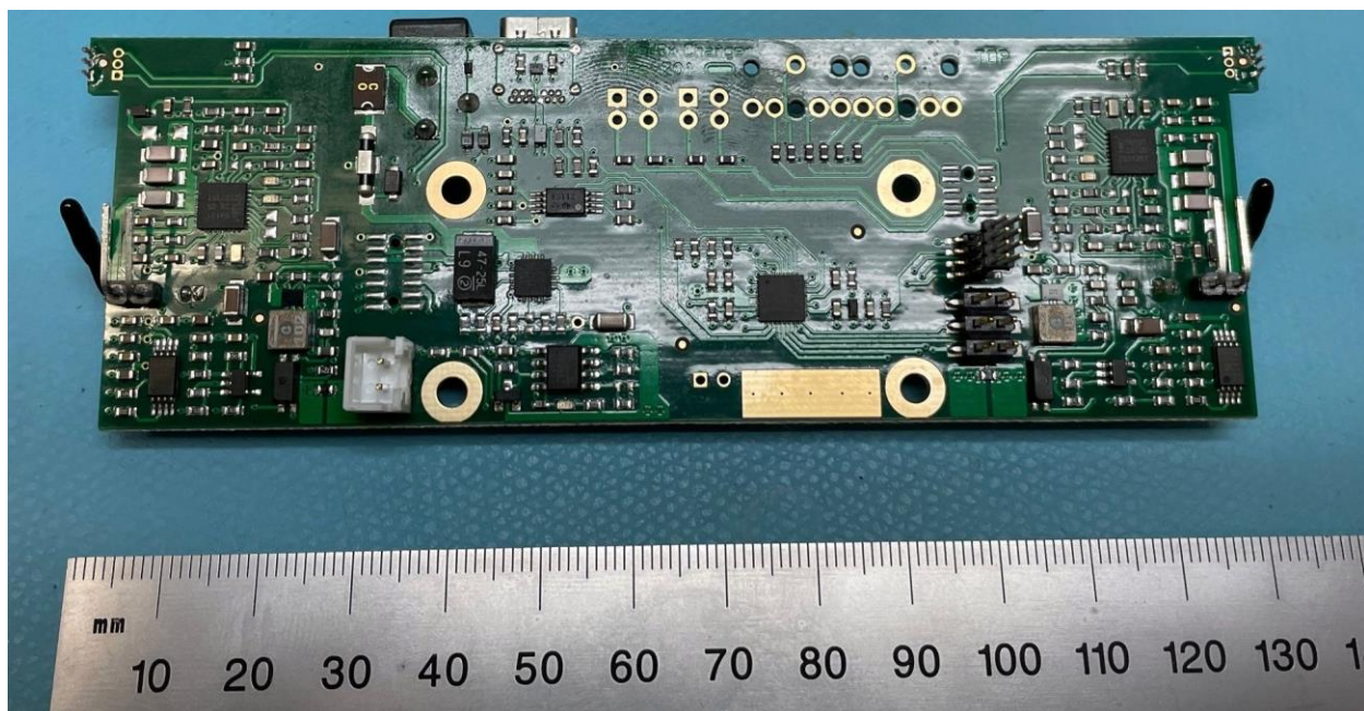
Main PCB top view
