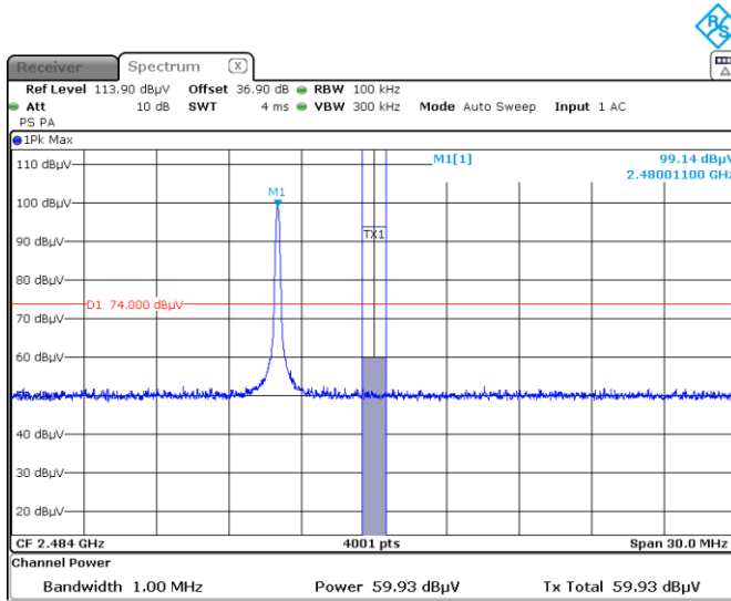
Figure 8.6-10: Band edge spurious emissions at 2483.5 MHz Peak – Hopping OFF
