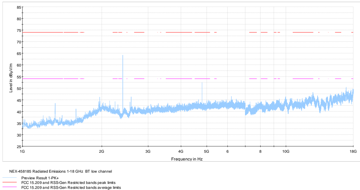
Figure 8.6-4: Radiated spurious emissions 1-18 GHz low channel
