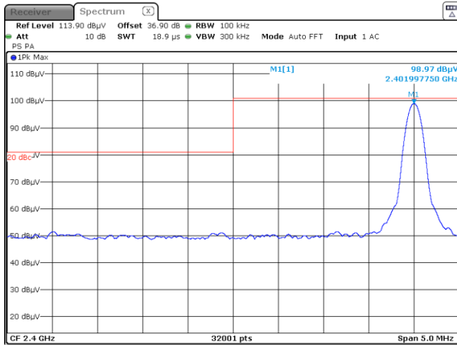
Figure 8.6-16: Non-restricted band edge at 2400 MHz, low channel
