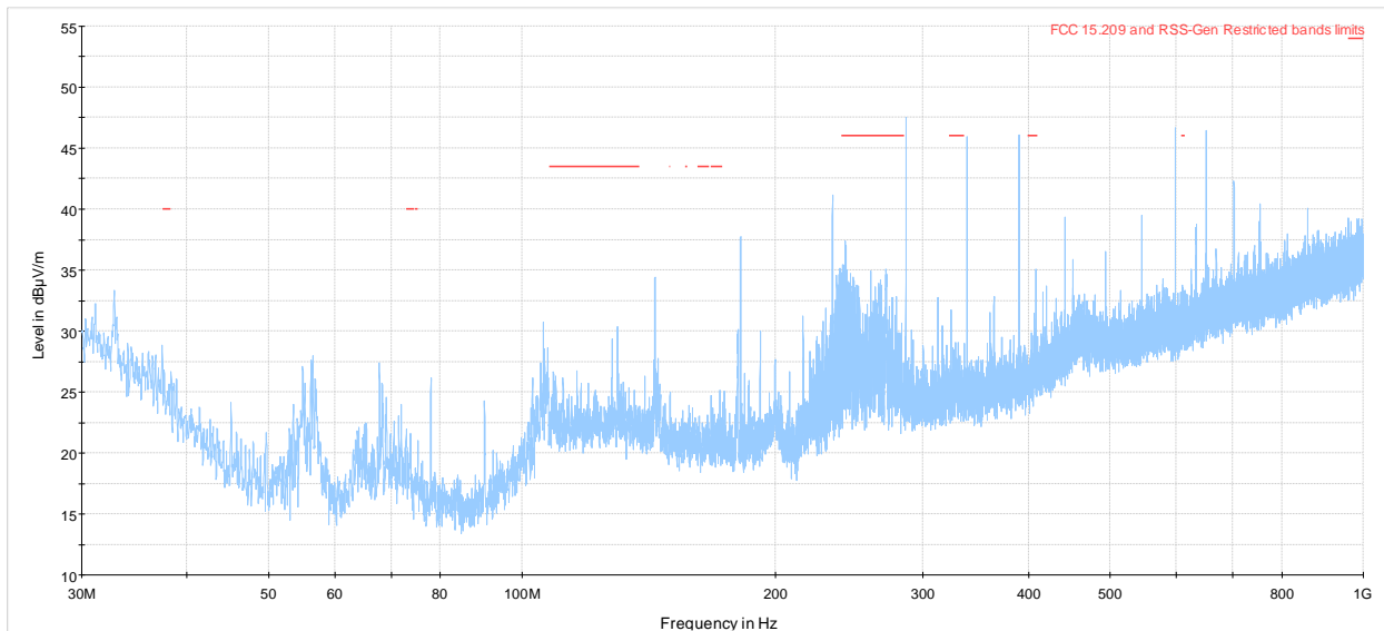
Figure 8.6-1: Radiated spurious emissions 30-1000 MHz low channel
