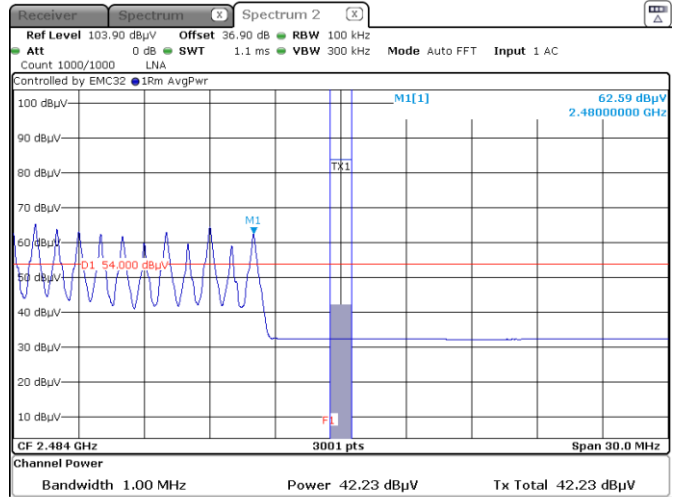
Figure 8.6-15: Band edge spurious emissions at 2483.5 MHz Average – Hopping ON
