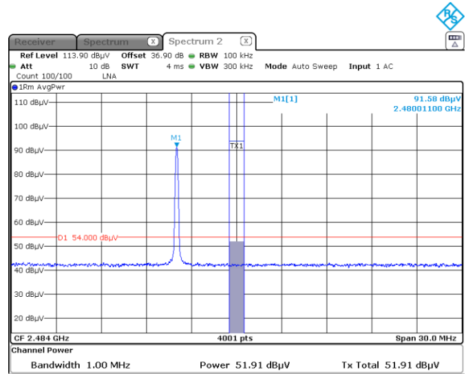
Figure 8.6-11: Band edge spurious emissions at 2483.5 MHz Average – Hopping OFF
