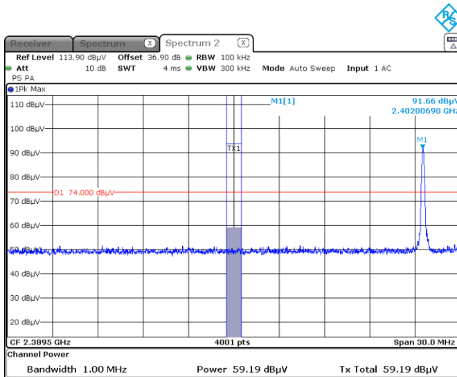
Figure 8.6-8: Band edge spurious emissions at 2390 MHz Peak – Hopping OFF
