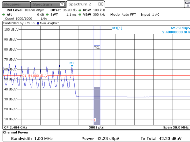
Figure 8.6-14: Band edge spurious emissions at 2483.5 MHz Peak – Hopping ON
