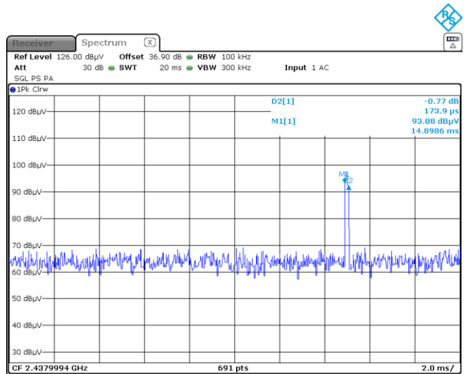
Figure 8.4-6: Dwell time
