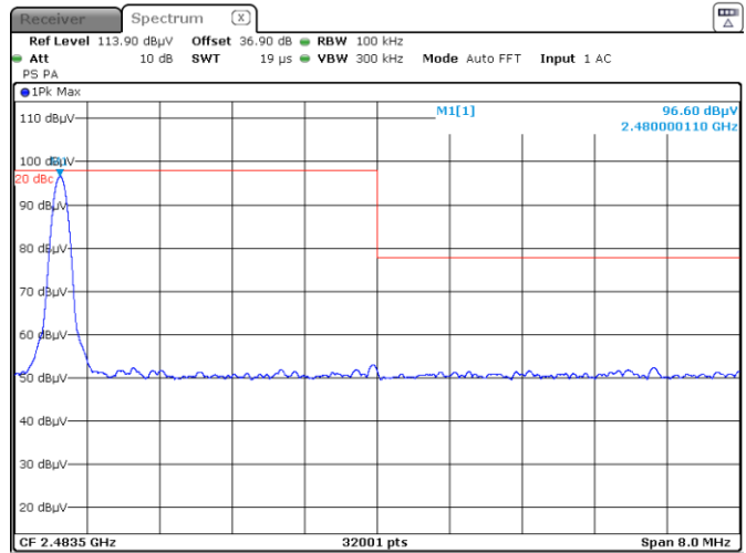
Figure 8.6-18: Non-restricted band edge at 2483.5 MHz, high channel
