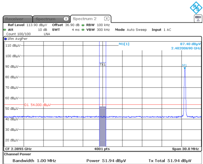
Figure 8.6-9: Band edge spurious emissions at 2390 MHz Average – Hopping OFF
