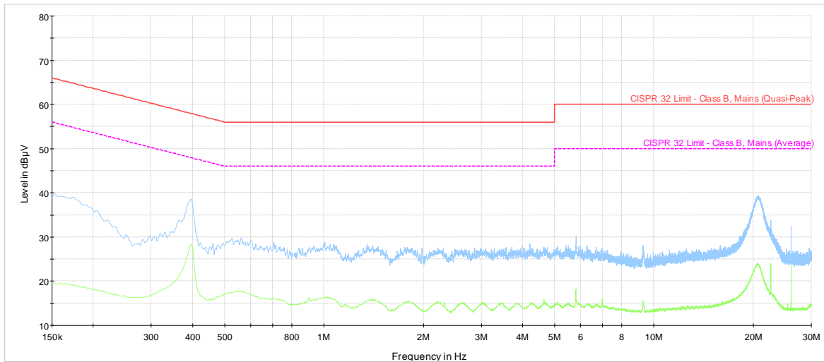
Plot 8.7-1: Conducted emissions on phase line
