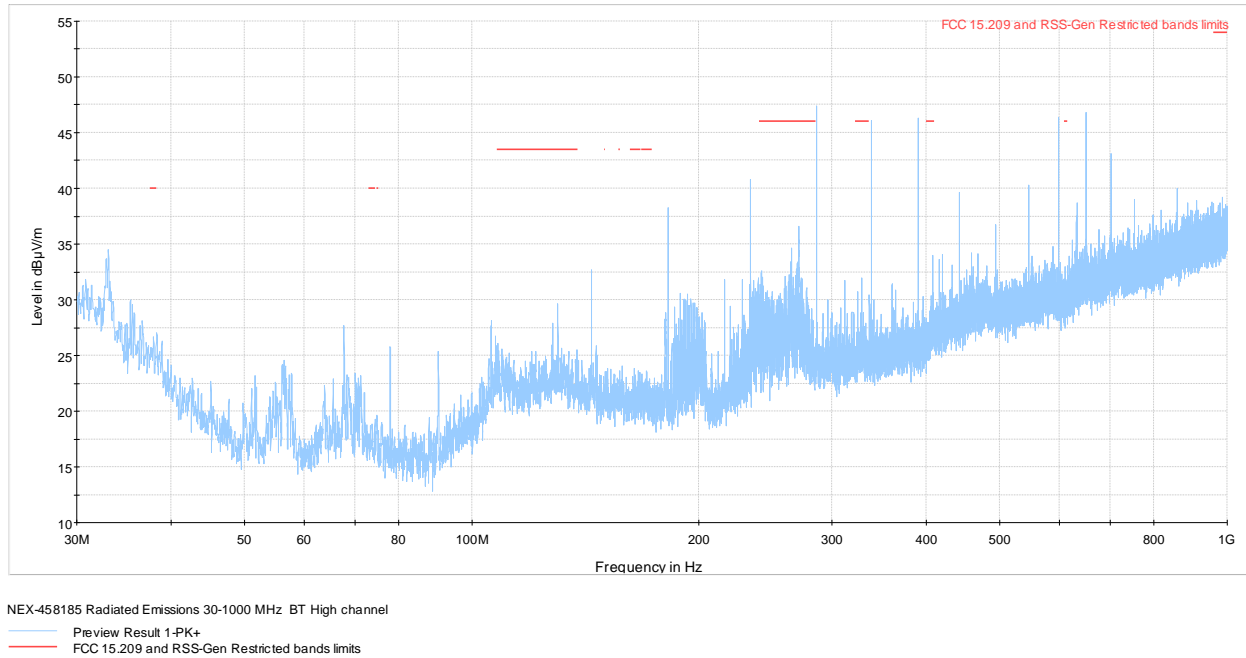
Figure 8.6-3: Radiated spurious emissions 30-1000 MHz high channel
