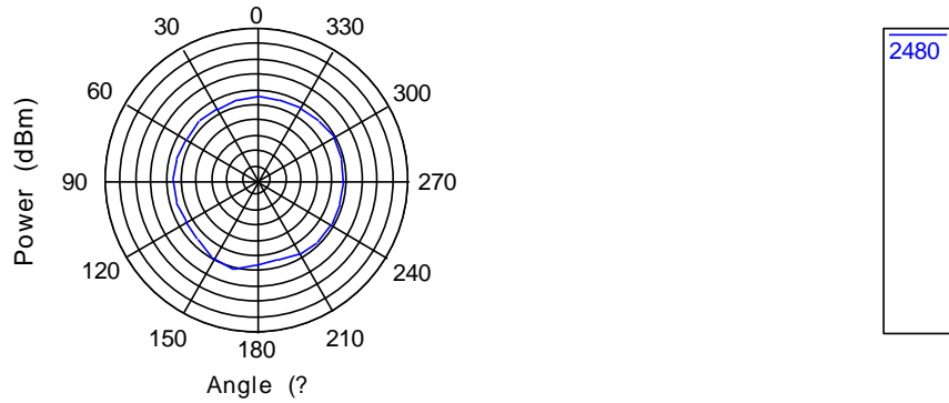
2D(X-Y Plane) RDA5875Y Antenna Gain Free Space-2480MHz
