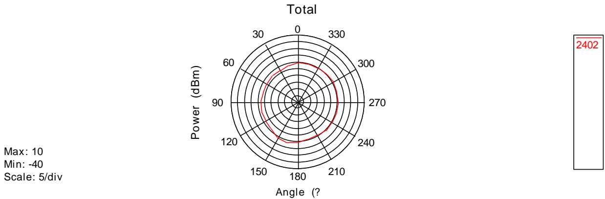
2D(X-Y Plane) RDA5875Y Antenna Gain Free Space-2402MHz
