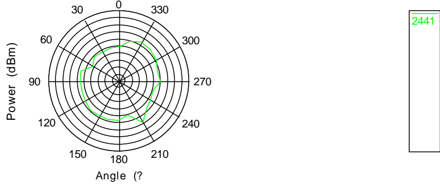
2D(Y-Z Plane) RDA5875Y Antenna Gain Free Space-2441MHz
