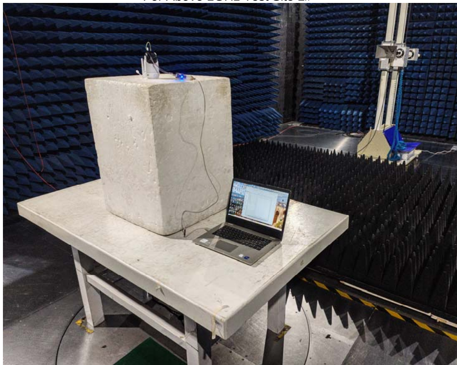
For Above 1GHz Test Site 1#
