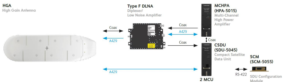
Figure 3-2: AVIATOR 700S SATCOM System
