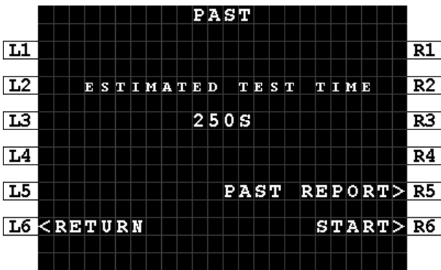
Figure 10-6: MCDU - BITE - PAST
