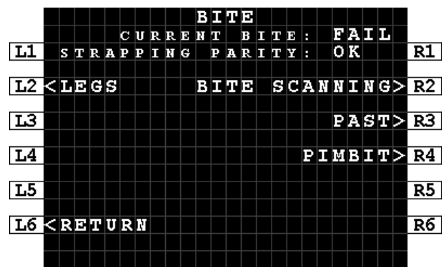
Figure 10-3: MCDU - BITE - FAIL
