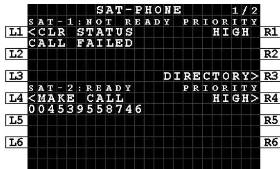
Figure 7-9: MCDU - SAT-PHONE 1/2 - Outgoing Call - Call Failed
