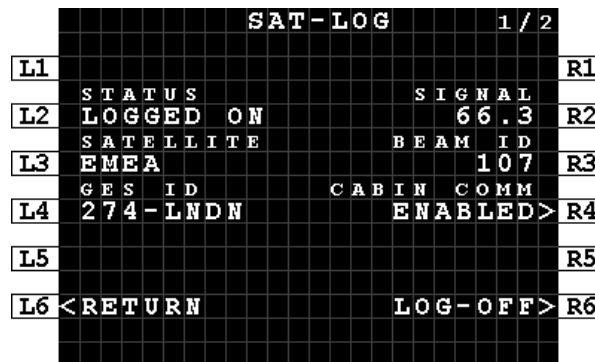
Figure 5-6: MCDU - SAT-LOG 1/2 - Safety Data Available
