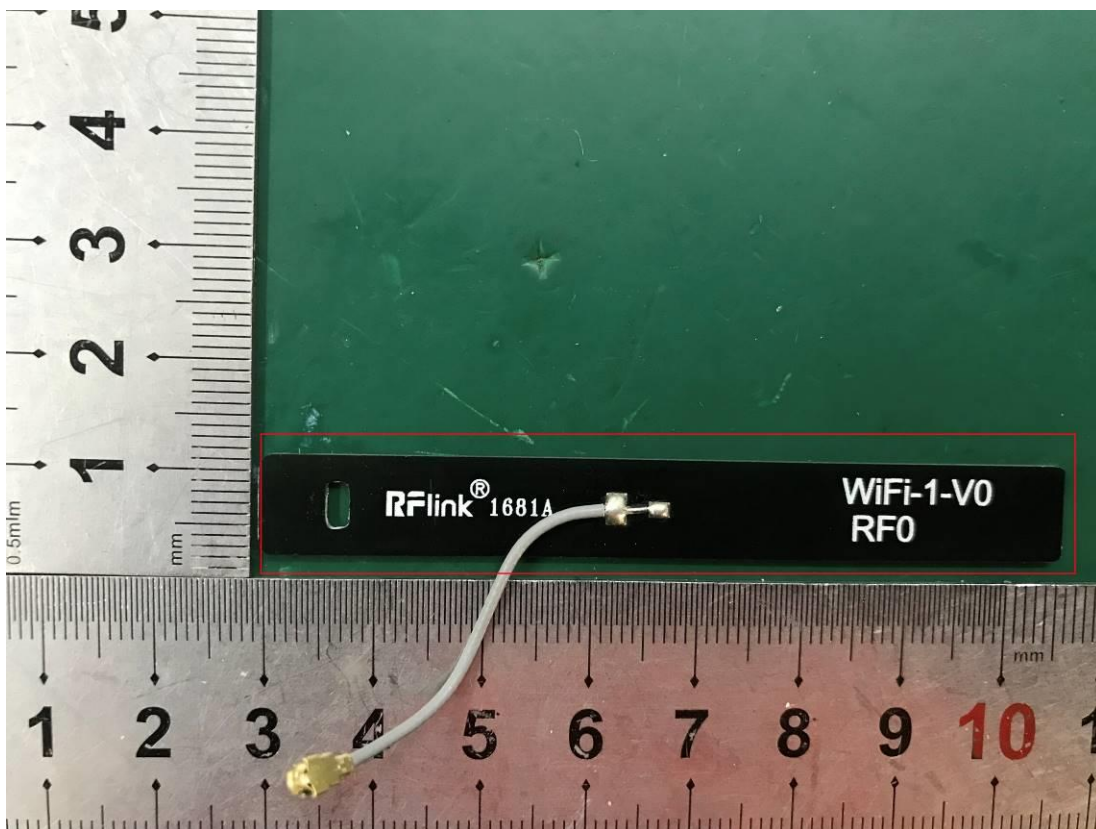
Wi-Fi Antenna 0
