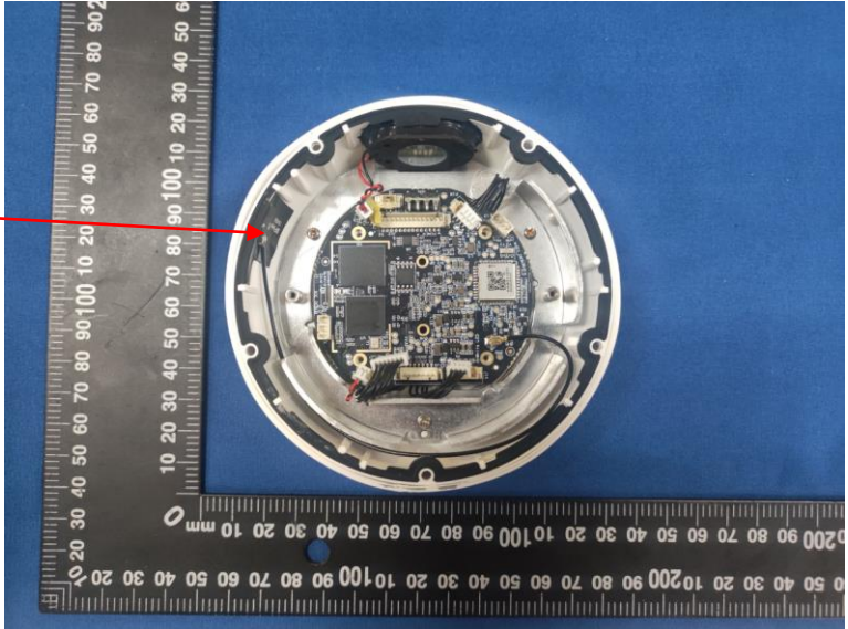
WIFI Antenna
