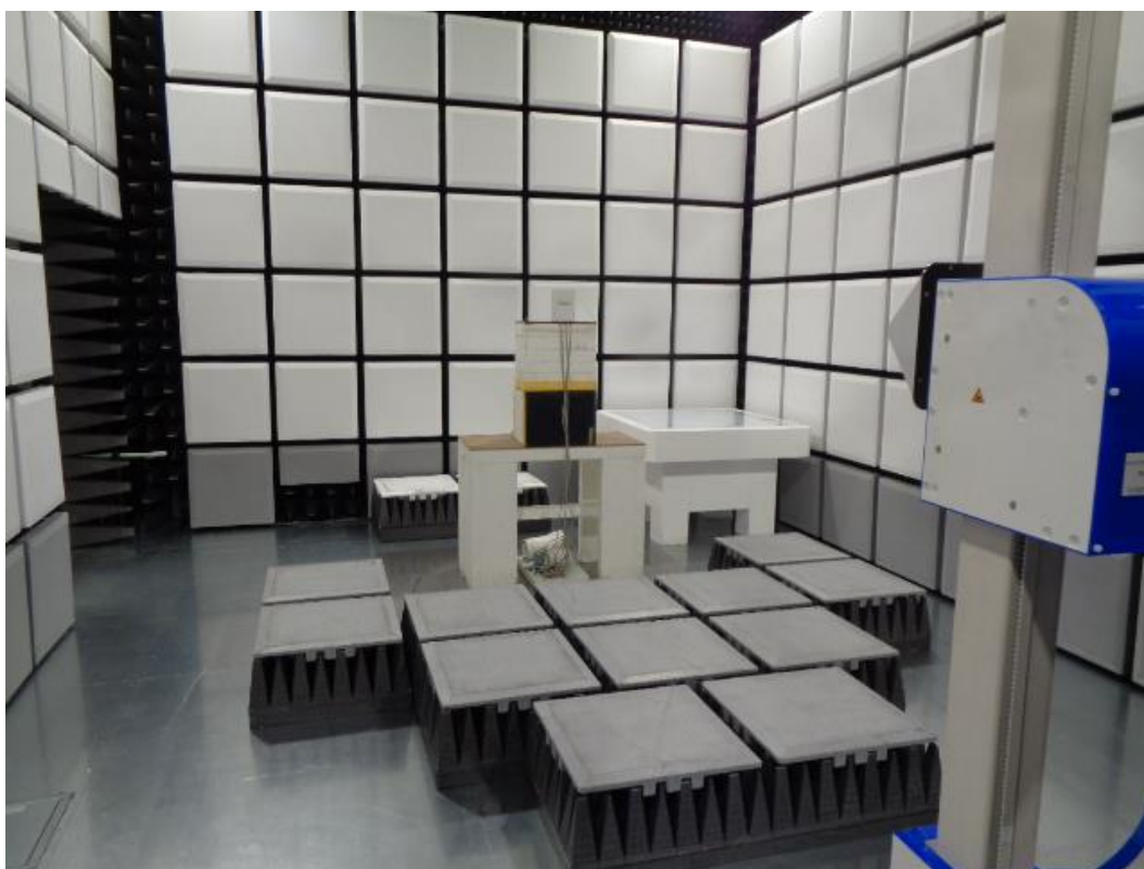
Figure 9.1-2: Radiated emissions set-up for frequencies above 1 GHz
