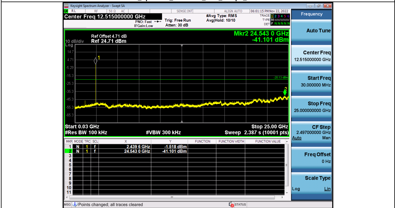
2_Spurious_Emission_BLE_1Mbps_2440
