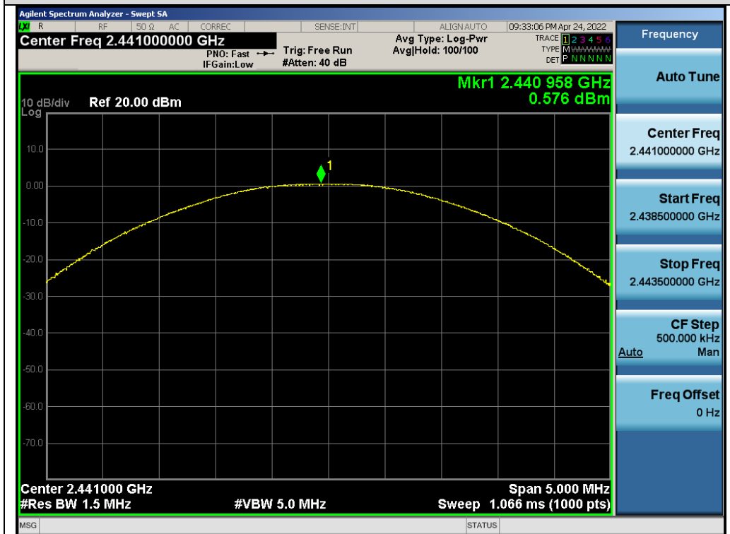
Test_Graph_EDR_ANT1_2441_2Mbps_Peak Power
