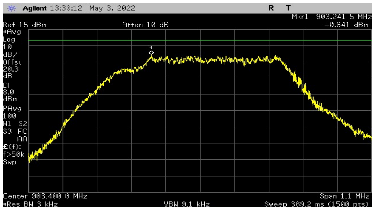
Plot 22 – Power Spectral Density – Lowest Channel
