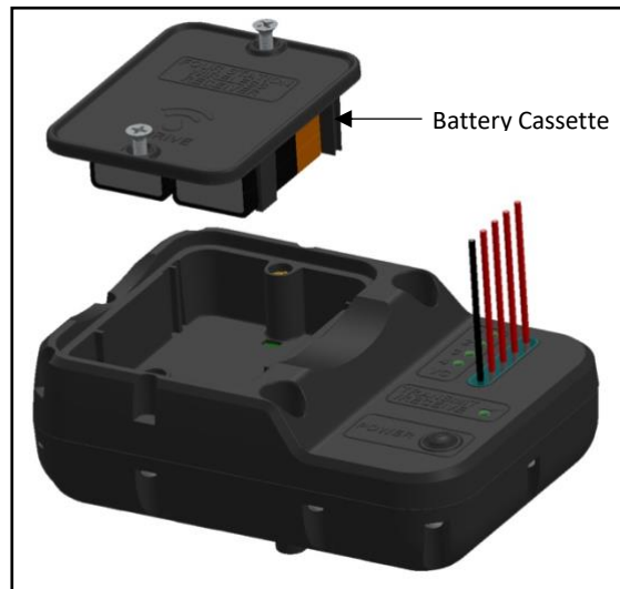
Battery Cassette Figure 14-1
