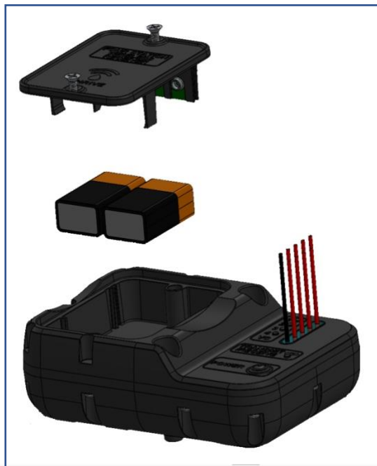
Install the 9-volt Receiver™ Batteries Figure 9-2
