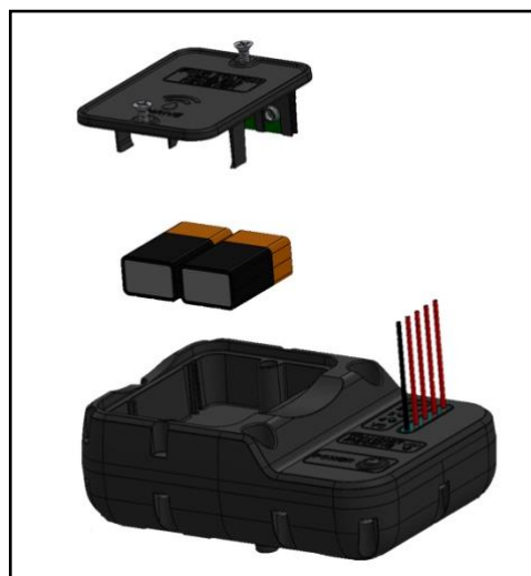
Replace 9-volt Batteries Figure 14-2
