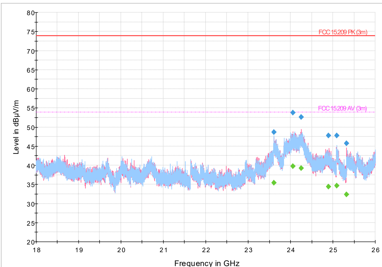
Figure 8.2-7: Radiated spurious emissions, 802.11g, 6 Mbps, 18-26 GHz spectral plot (2437 MHz)
