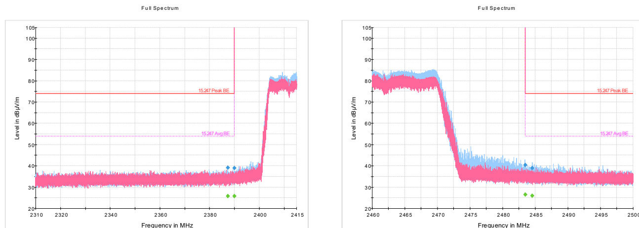
Figure 8.2-1: Radiated emissions, restricted band edge, 802.11g, 6 Mbps
