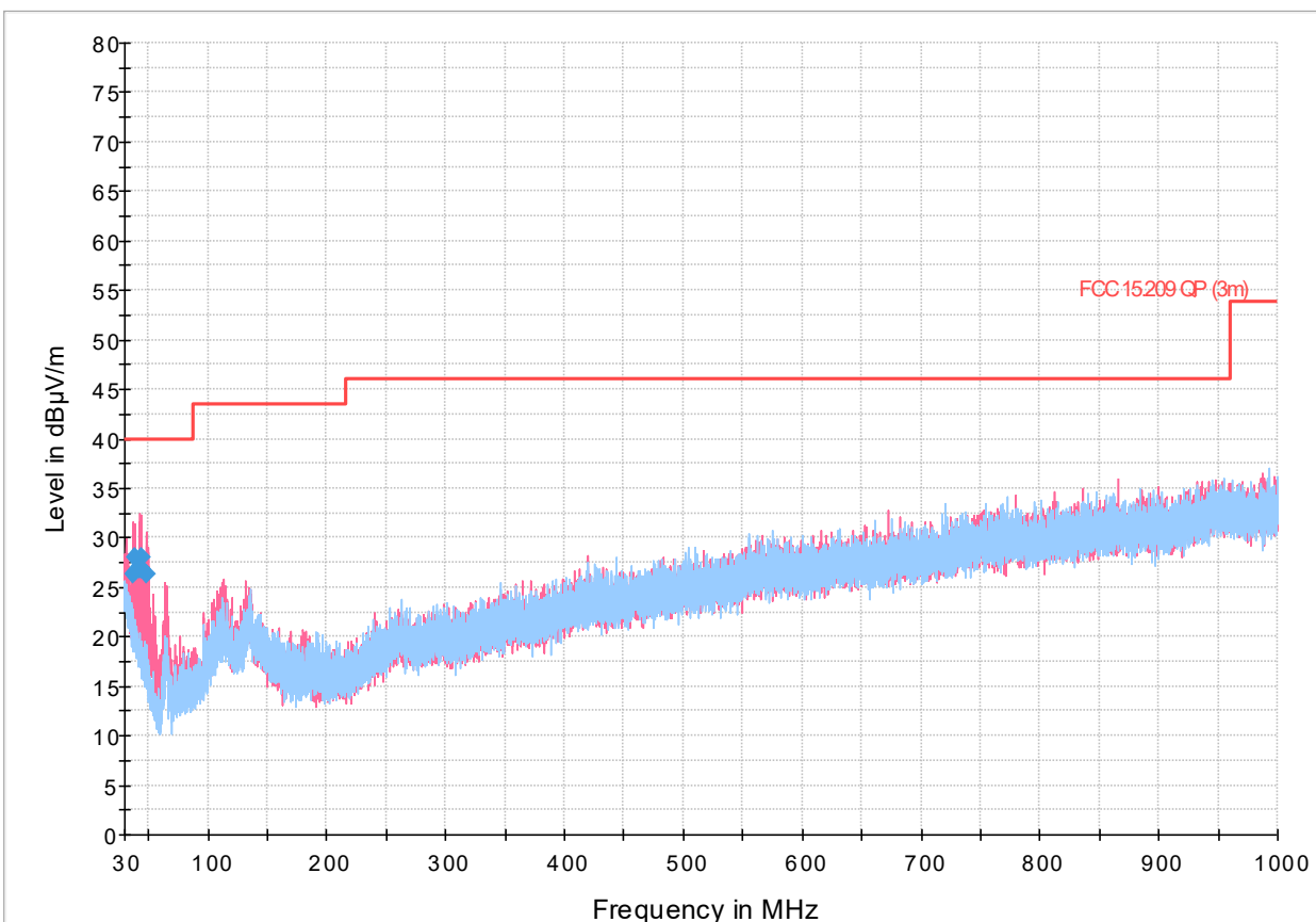
Figure 8.2-2: Radiated spurious emissions, 802.11b, 1 Mbps, 30-1000 MHz spectral plot (2462 MHz)
