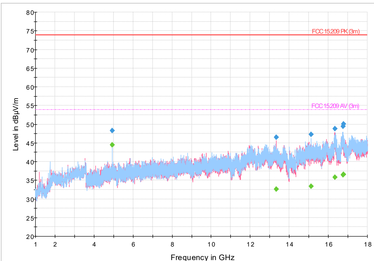
Figure 8.2-3: Radiated spurious emissions, 802.11b, 1 Mbps, 1-18 GHz spectral plot (2462 MHz)
