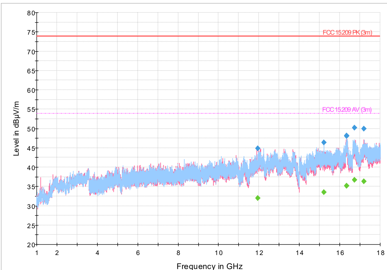
Figure 8.2-6: Radiated spurious emissions, 802.11g, 6 Mbps, 1-18 GHz spectral plot (2437 MHz)
