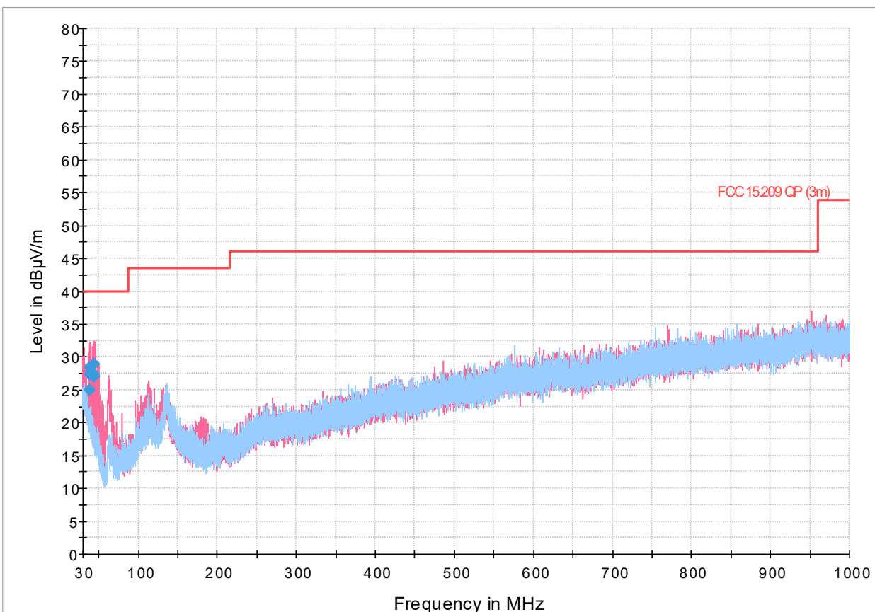
Figure 8.2-8: Radiated spurious emissions, 802.11n-HT20, MSC0, 30-1000 MHz spectral plot (2437 MHz)
