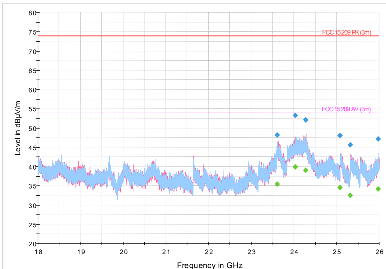
Figure 8.2-10: Radiated spurious emissions, 802.11n-HT20, MSC0, 18-26 GHz spectral plot (2437 MHz)
