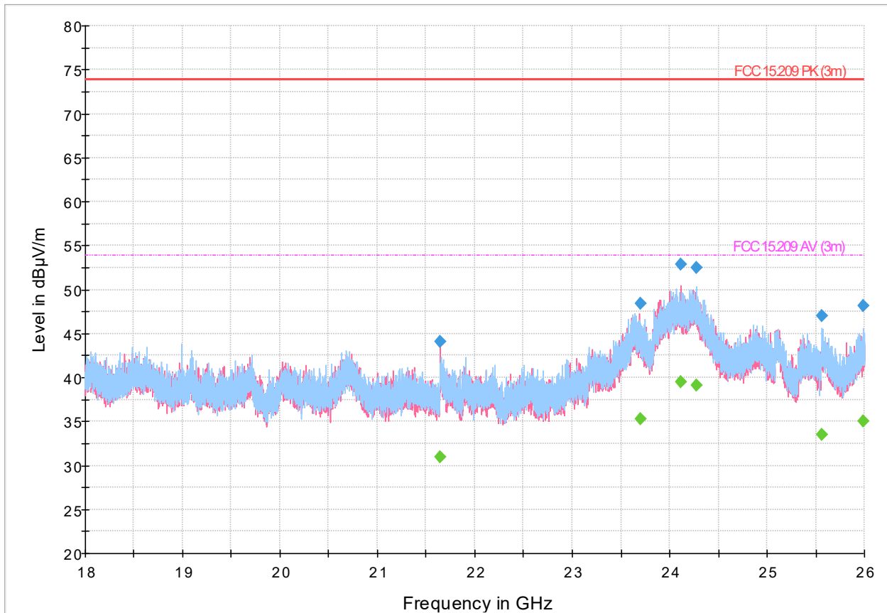
Figure 8.2-4: Radiated spurious emissions, 802.11b, 1 Mbps, 18-26 GHz (2462 MHz) spectral plot
