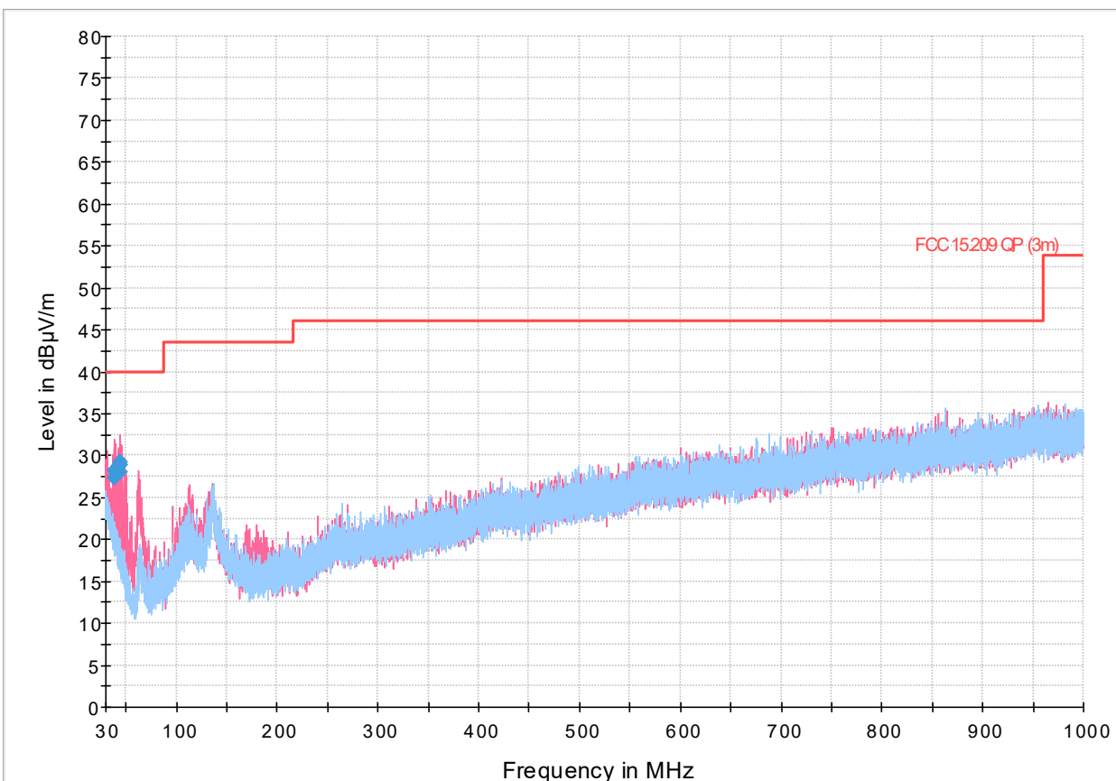
Figure 8.2-5: Radiated spurious emissions, 802.11g, 6 Mbps, 30-1000 MHz spectral plot (2437 MHz)
