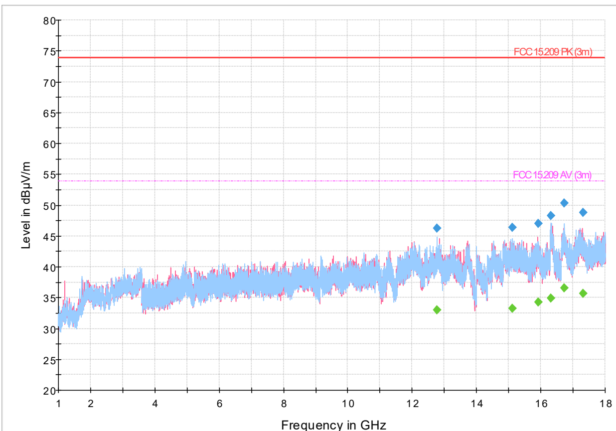
Figure 8.2-9: Radiated spurious emissions, 802.11n-HT20, MSC0, 1-18 GHz spectral plot (2437 MHz)
