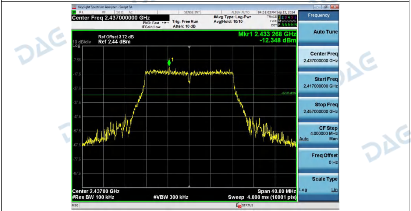
2_Spurious_Emission_NVNT_ANT1_802_11g_2437
