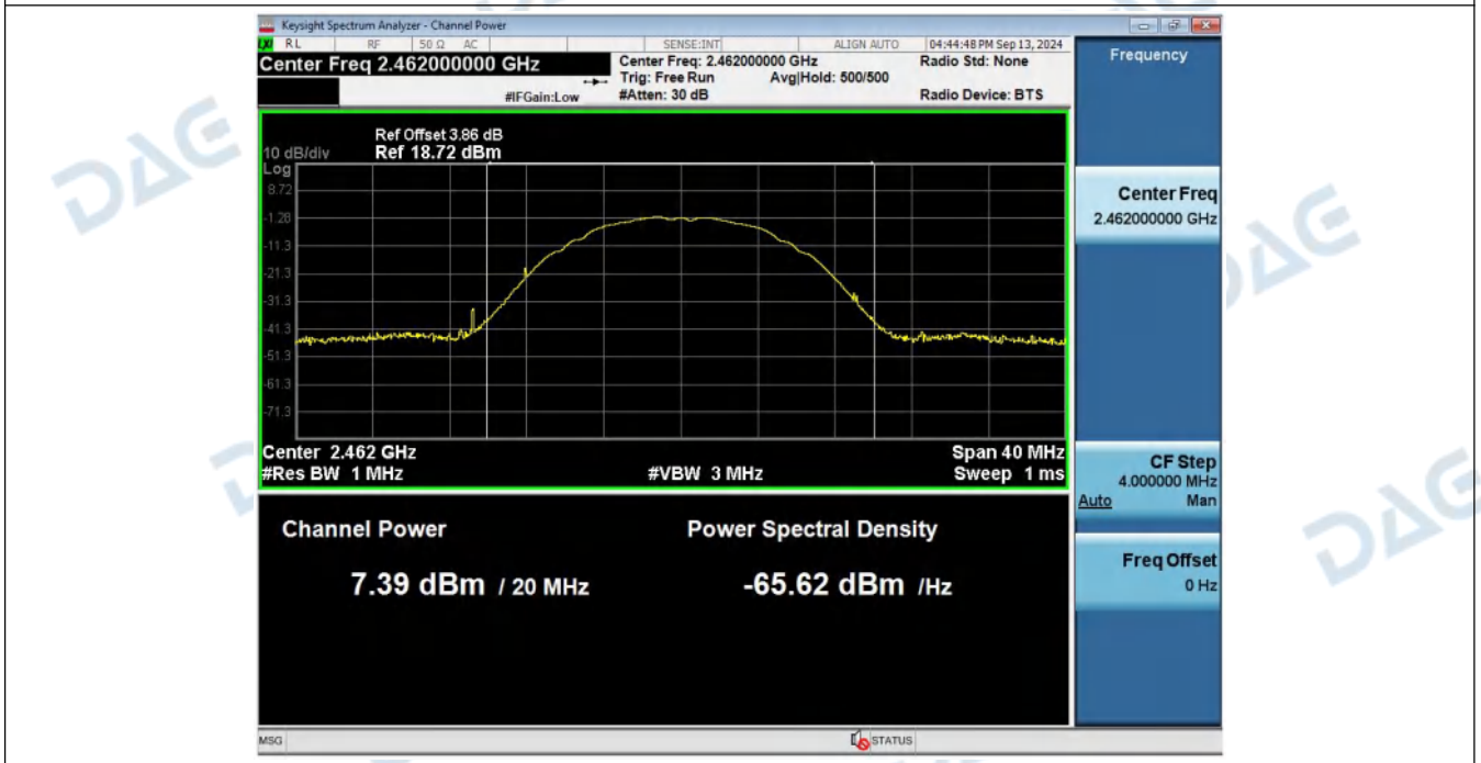
MAX_ Output_Power_NVNT_ANT1_802_11b_2462
