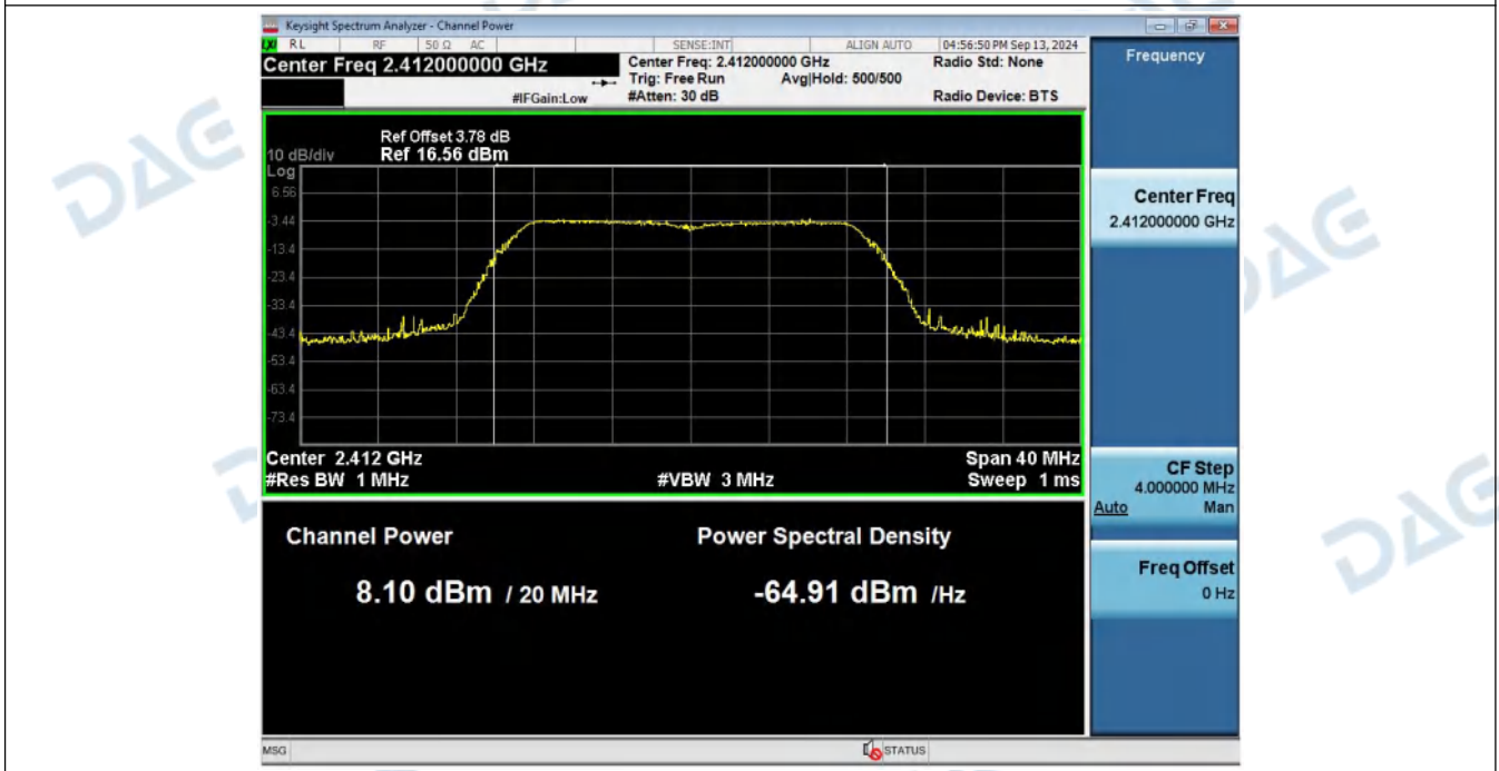
MAX__Output_Power_NVNT_ANT1_802_11n(HT20)_2412
