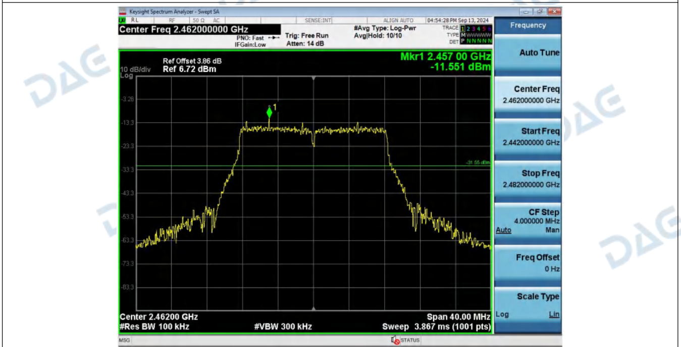
2_Spurious_Emission_NVNT_ANT1_802_11g_2462
