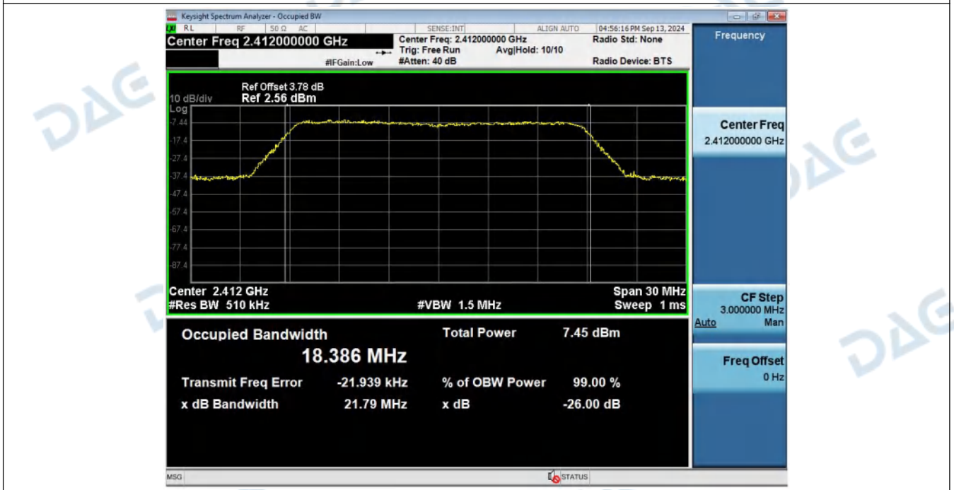
99%_Occupied_Bandwidth_NVNT_ANT1_802_11n(HT20)_2412
