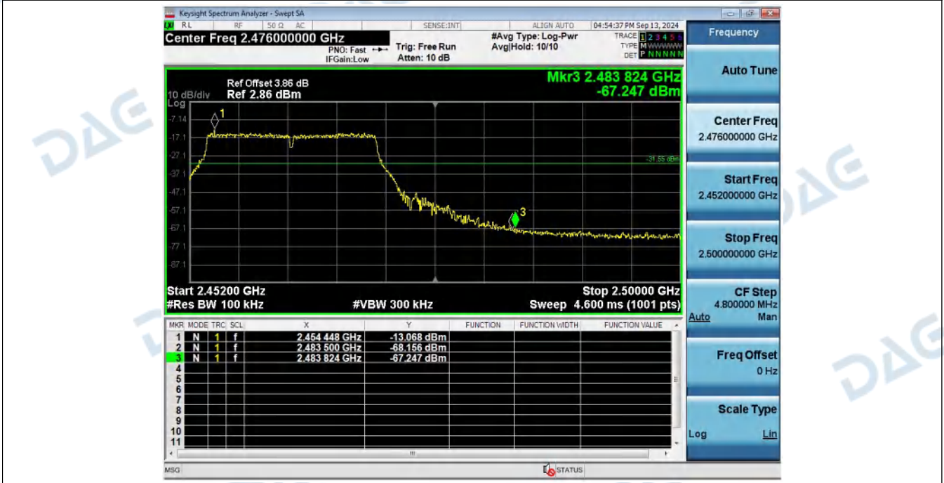
2_Bandedge_NVNT_ANT1_802_11g_2462
