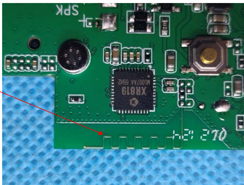
WIFI-PCB Antenna
