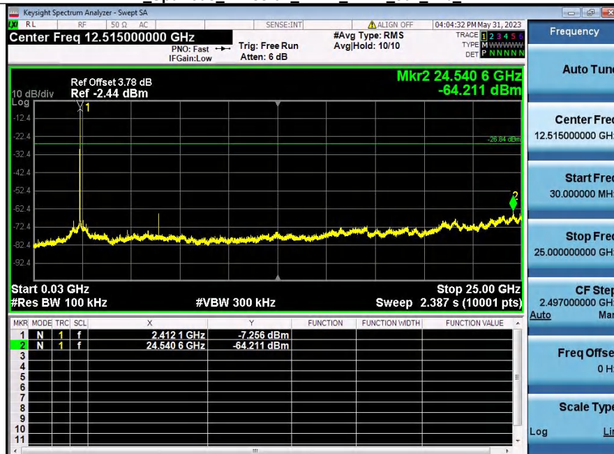
2 Spurious Emission NVNT_ANT1_802_11b_2412
