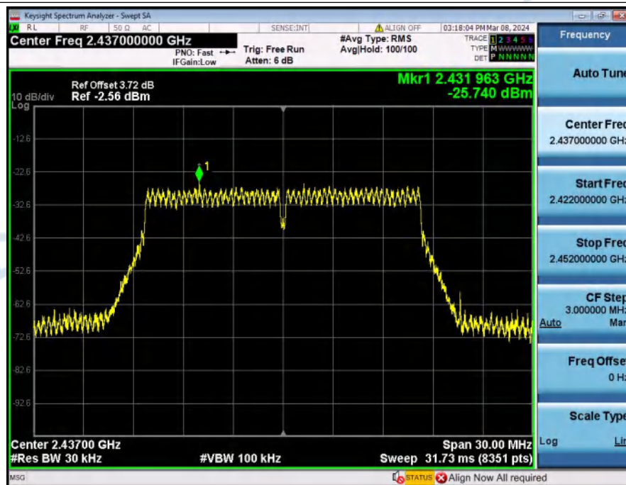
Power Spectral Density_NVNT_ANT1_802_11g_2437
