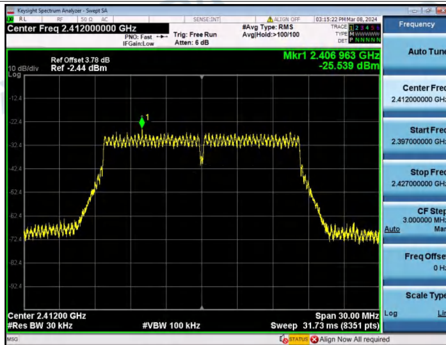
Power Spectral Density_NVNT_ANT1_802_11g_2412
