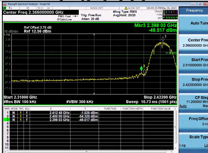
2 Bandedge NVNT ANT1 802 11b 2412
