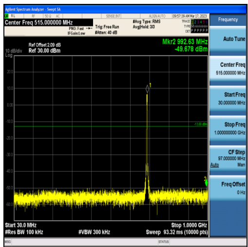
Band71-5MHz-16QAM-133447-25RB#0-Range1:30~1000MHz
