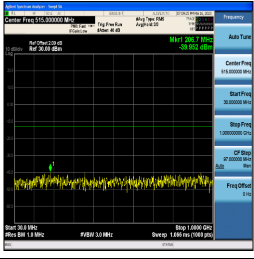
Band25-15MHz-QPSK-26615-75RB#0-Range1:30~1000MHz
