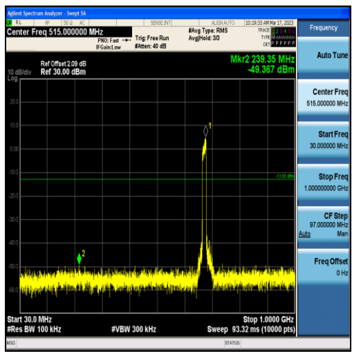
Band71-15MHz-QPSK-133297-75RB#0-Range1:30~1000MHz
