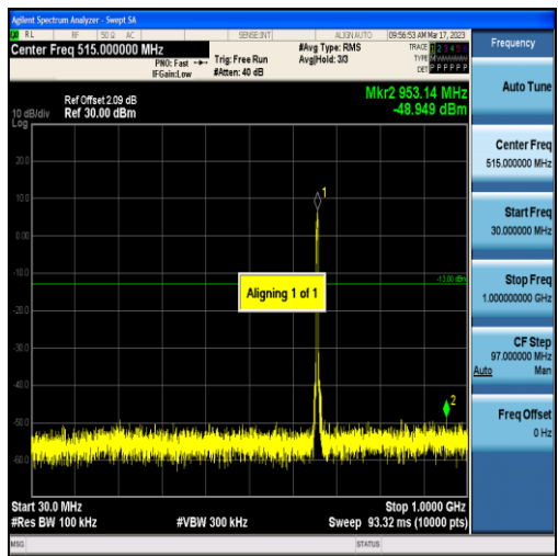
Band71-5MHz-16QAM-133147-25RB#0-Range1:30~1000MHz
