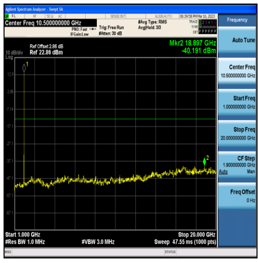
Band25-5MHz-16QAM-26665-25RB#0-Range2:1000~20000MHz
