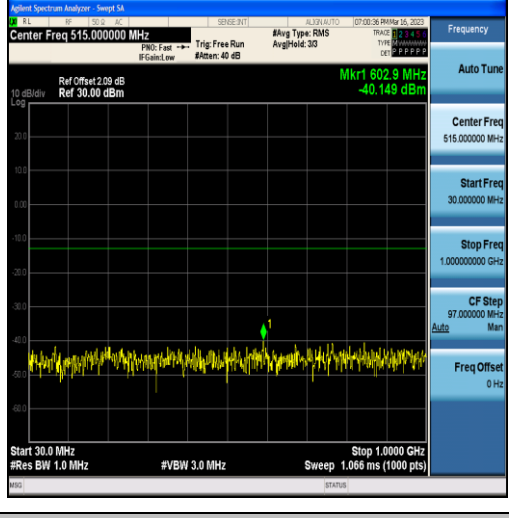
Band25-10MHz-QPSK-26090-50RB#0-Range1:30~1000MHz
