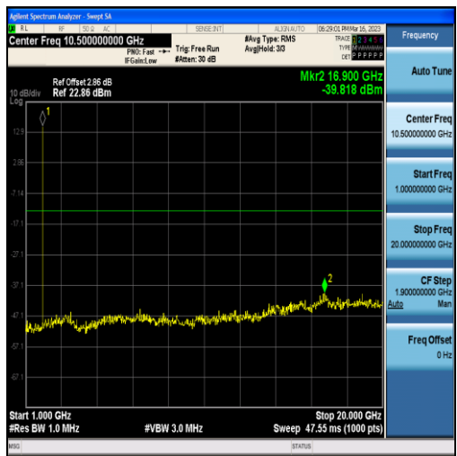
Band25-3MHz-16QAM-26675-15RB#0-Range2:1000~20000MHz
