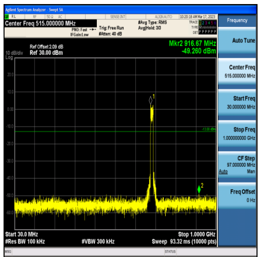
Band71-15MHz-16QAM-133397-75RB#0-Range1:30~1000MHz
