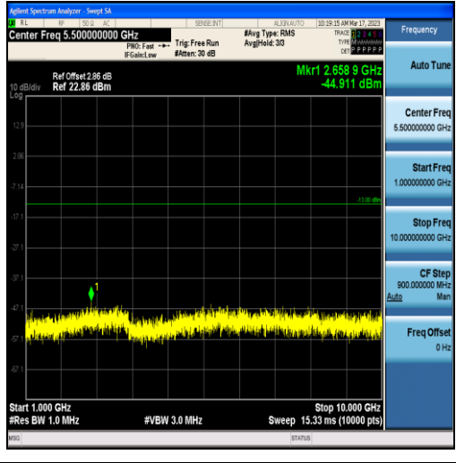
Band71-15MHz-16QAM-133197-75RB#0-Range2:1000~10000MHz
