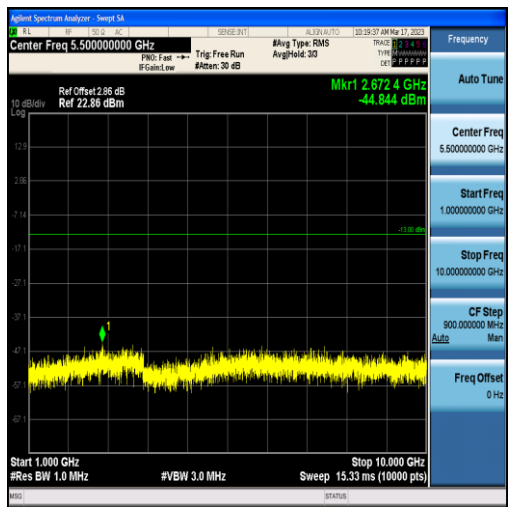
Band71-15MHz-QPSK-133297-75RB#0-Range2:1000~10000MHz
