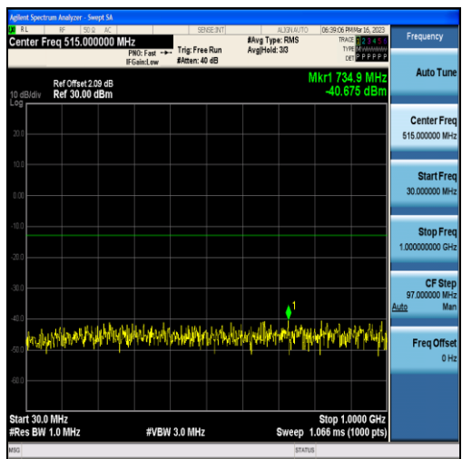
Band25-5MHz-QPSK-26065-25RB#0-Range1:30~1000MHz
