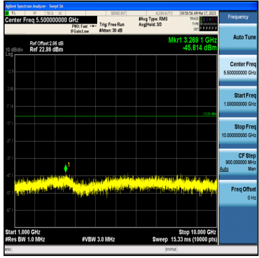
Band71-5MHz-16QAM-133147-25RB#0-Range2:1000~10000MHz
