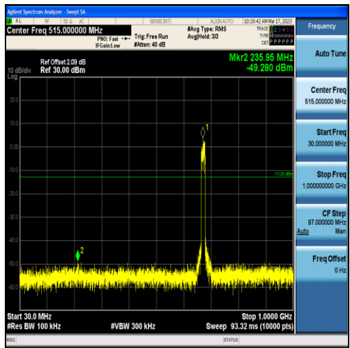
Band71-15MHz-16QAM-133297-75RB#0-Range1:30~1000MHz
