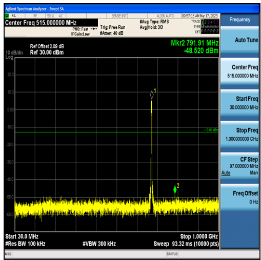
Band71-5MHz-16QAM-133297-25RB#0-Range1:30~1000MHz
