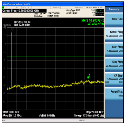
Band25-5MHz-16QAM-26365-25RB#0-Range2:1000~20000MHz
