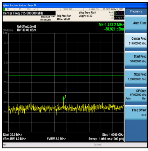
Band25-20MHz-16QAM-26140-100RB#0-Range1:30~1000MHz
