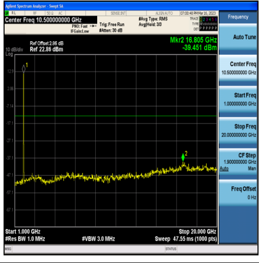
Band25-10MHz-16QAM-26090-50RB#0-Range2:1000~20000MHz
