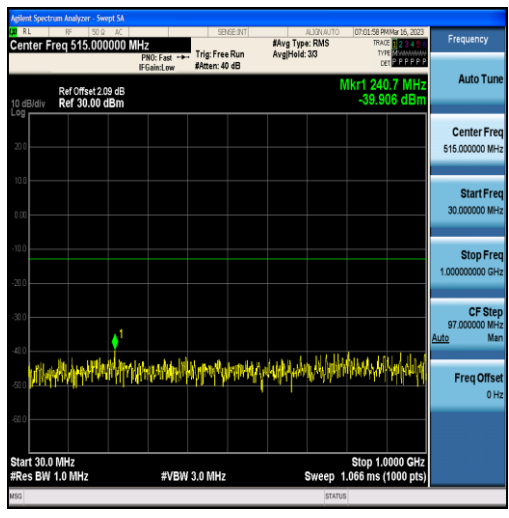
Band25-10MHz-QPSK-26640-50RB#0-Range1:30~1000MHz
