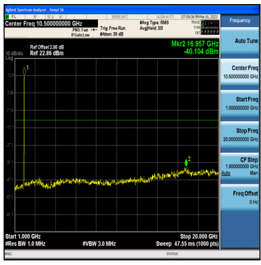
Band25-15MHz-QPSK-26365-75RB#0-Range2:1000~20000MHz
