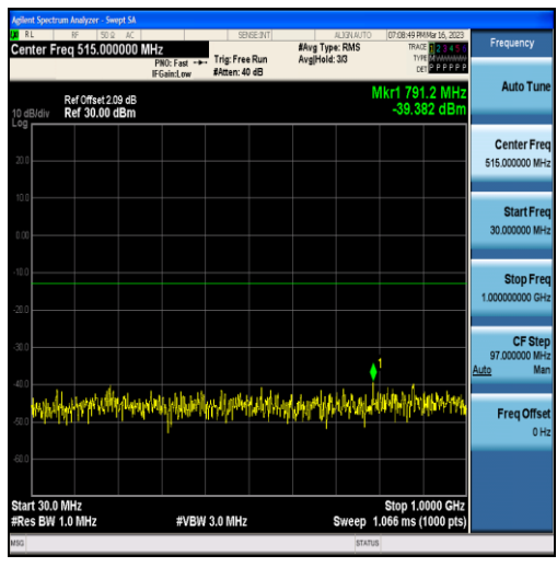
Band25-15MHz-16QAM-26115-75RB#0-Range1:30~1000MHz
