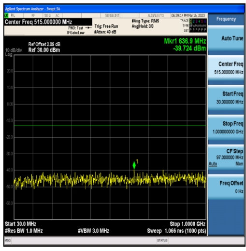
Band25-5MHz-16QAM-26065-25RB#0-Range1:30~1000MHz
