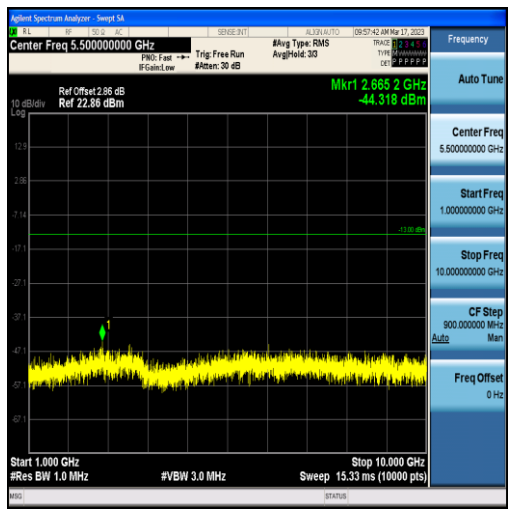
Band71-5MHz-16QAM-133447-25RB#0-Range2:1000~10000MHz
