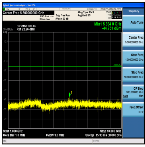
Band71-10MHz-16QAM-133422-50RB#0-Range2:1000~10000MHz
