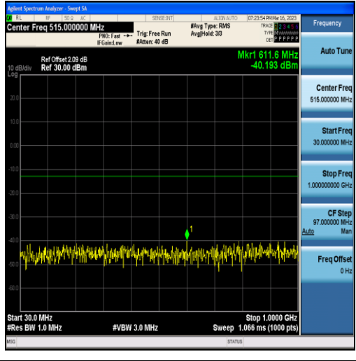
Band25-20MHz-16QAM-26365-100RB#0-Range1:30~1000MHz
