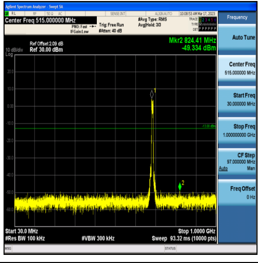
Band71-10MHz-16QAM-133422-50RB#0-Range1:30~1000MHz
