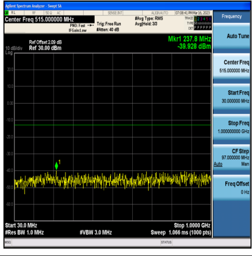
Band25-15MHz-QPSK-26115-75RB#0-Range1:30~1000MHz
