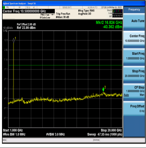
Band25-15MHz-16QAM-26365-75RB#0-Range2:1000~20000MHz
