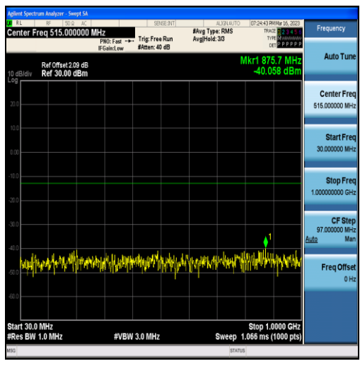
Band25-20MHz-16QAM-26590-100RB#0-Range1:30~1000MHz
