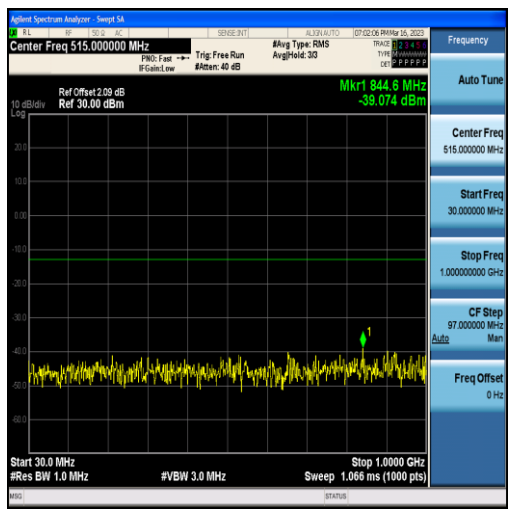
Band25-10MHz-16QAM-26640-50RB#0-Range1:30~1000MHz
