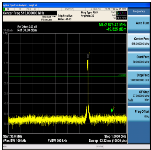
Band71-10MHz-16QAM-133297-50RB#0-Range1:30~1000MHz
