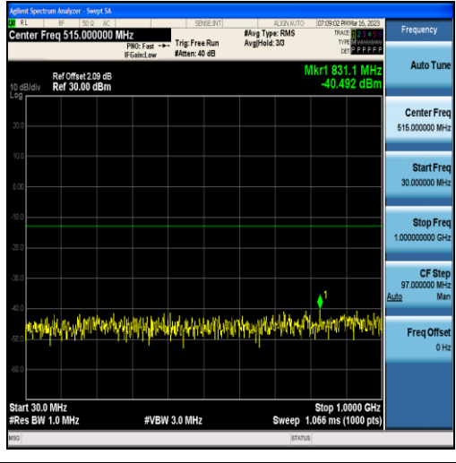
Band25-15MHz-QPSK-26365-75RB#0-Range1:30~1000MHz
