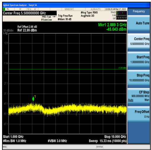
Band71-10MHz-16QAM-133297-50RB#0-Range2:1000~10000MHz
