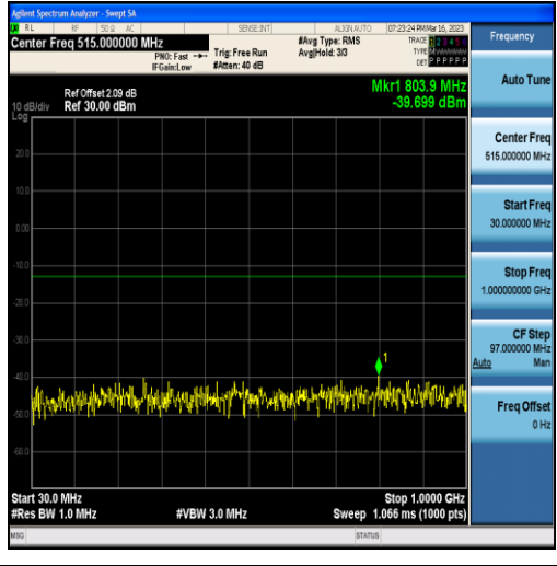
Band25-20MHz-QPSK-26140-100RB#0-Range1:30~1000MHz
