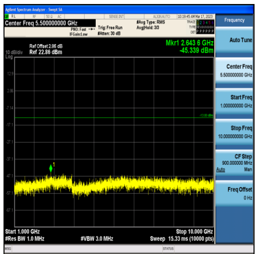
Band71-15MHz-16QAM-133297-75RB#0-Range2:1000~10000MHz
