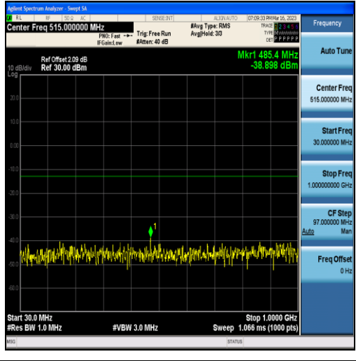
Band25-15MHz-16QAM-26615-75RB#0-Range1:30~1000MHz
