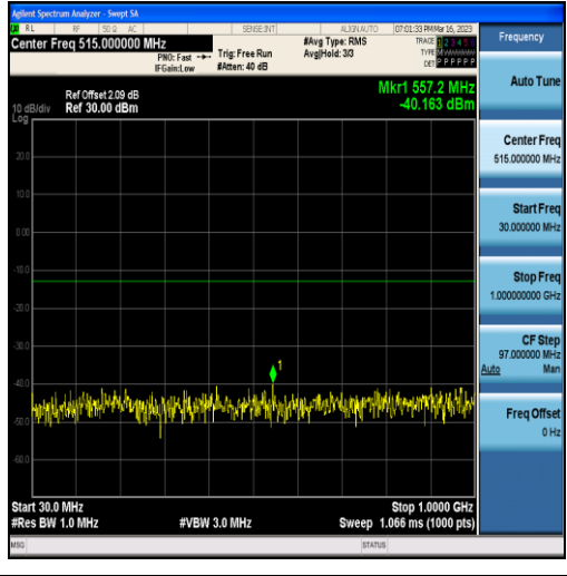
Band25-10MHz-16QAM-26365-50RB#0-Range1:30~1000MHz
