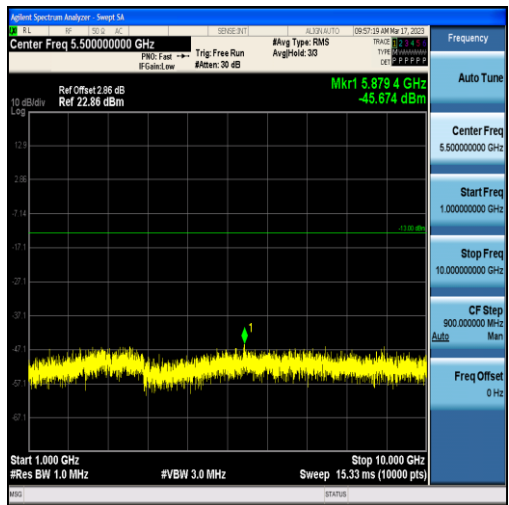
Band71-5MHz-16QAM-133297-25RB#0-Range2:1000~10000MHz
