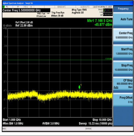
Band71-10MHz-16QAM-133172-50RB#0-Range2:1000~10000MHz
