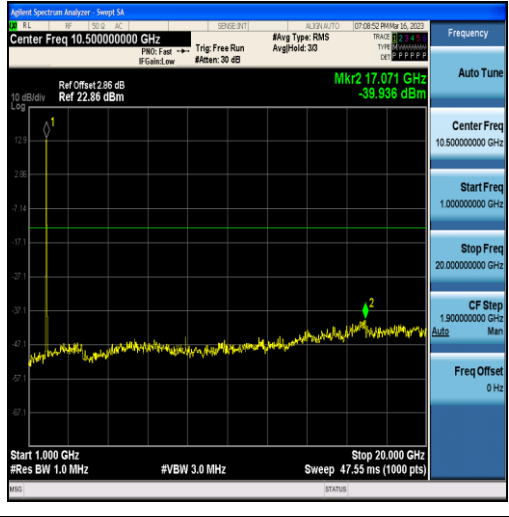
Band25-15MHz-16QAM-26115-75RB#0-Range2:1000~20000MHz
