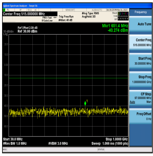
Band25-5MHz-QPSK-26365-25RB#0-Range1:30~1000MHz
