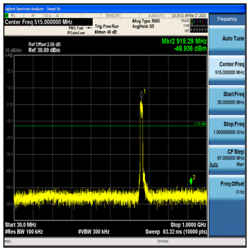
Band71-15MHz-16QAM-133197-75RB#0-Range1:30~1000MHz
