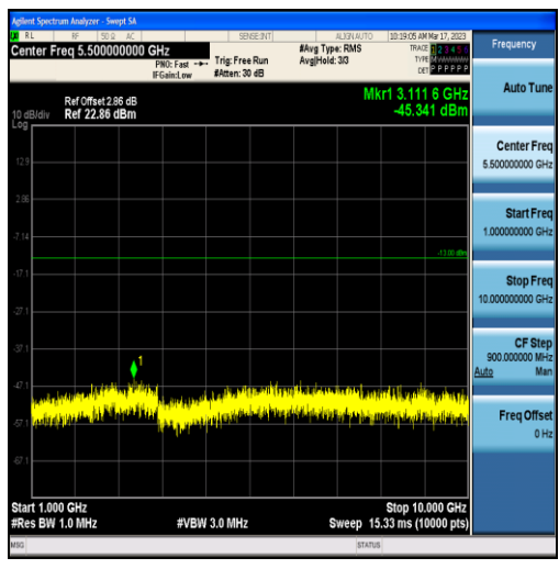
Band71-15MHz-QPSK-133197-75RB#0-Range2:1000~10000MHz
