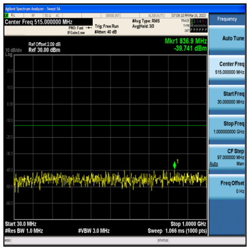
Band25-15MHz-16QAM-26365-75RB#0-Range1:30~1000MHz
