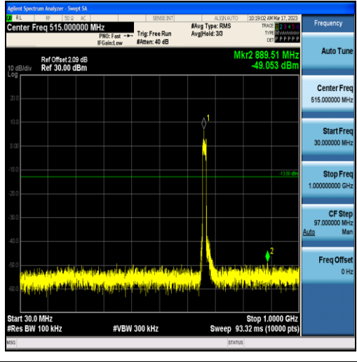
Band71-15MHz-QPSK-133197-75RB#0-Range1:30~1000MHz
