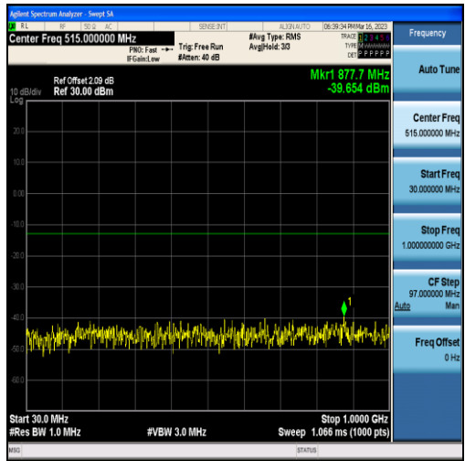
Band25-5MHz-16QAM-26365-25RB#0-Range1:30~1000MHz
