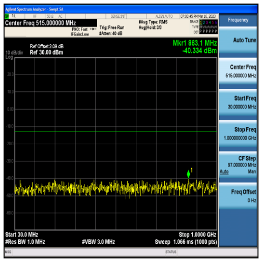
Band25-10MHz-16QAM-26090-50RB#0-Range1:30~1000MHz
