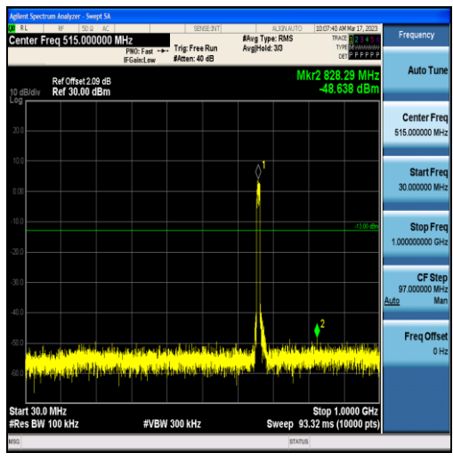
Band71-10MHz-16QAM-133172-50RB#0-Range1:30~1000MHz
