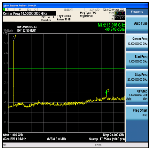
Band25-5MHz-QPSK-26065-25RB#0-Range2:1000~20000MHz
