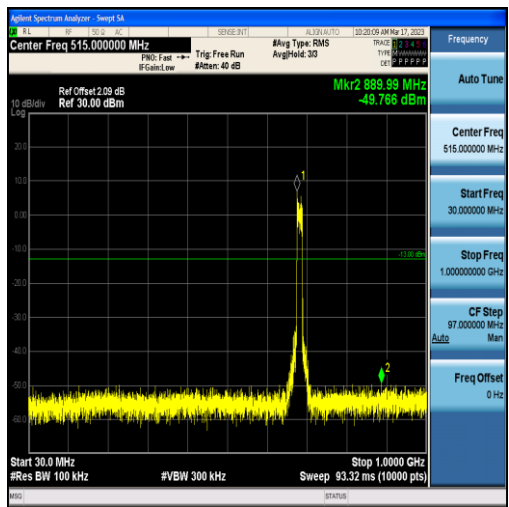
Band71-15MHz-QPSK-133397-75RB#0-Range1:30~1000MHz
