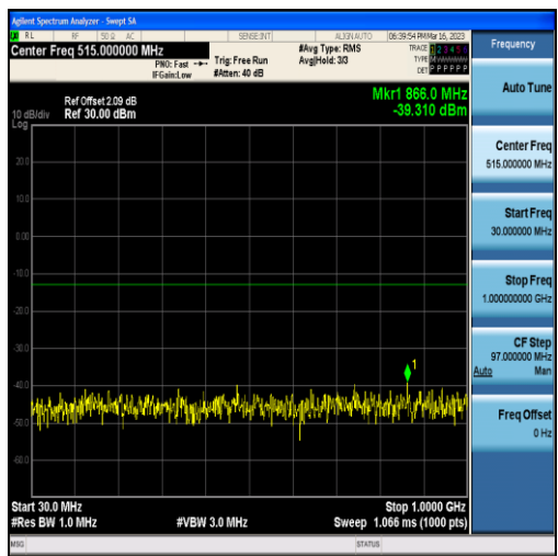
Band25-5MHz-16QAM-26665-25RB#0-Range1:30~1000MHz
