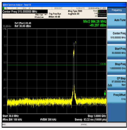
Band71-10MHz-QPSK-133297-50RB#0-Range1:30~1000MHz
