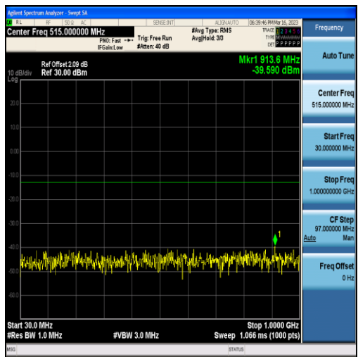
Band25-5MHz-QPSK-26665-25RB#0-Range1:30~1000MHz
