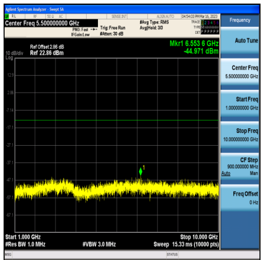
Band12-10MHz-QPSK-23095-50RB#0-Range2:1000~10000MHz
