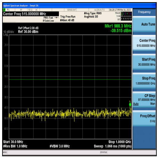
Band25-3MHz-16QAM-26055-15RB#0-Range1:30~1000MHz
