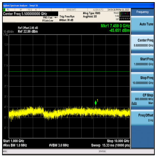
Band12-10MHz-16QAM-23130-50RB#0-Range2:1000~10000MHz
