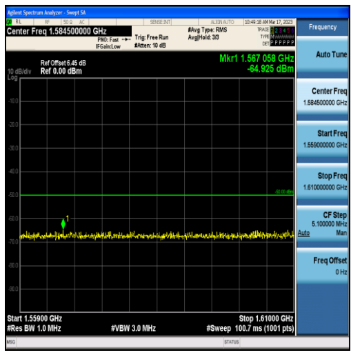
Band13-5MHz-QPSK-23255-25RB#0-Range3:1559~1610MHz
