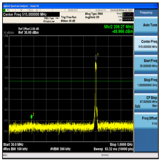
Band12-10MHz-QPSK-23095-50RB#0-Range1:30~1000MHz
