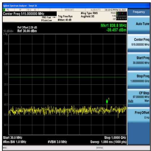
Band25-1.4MHz-16QAM-26683-6RB#0-Range1:30~1000MHz
