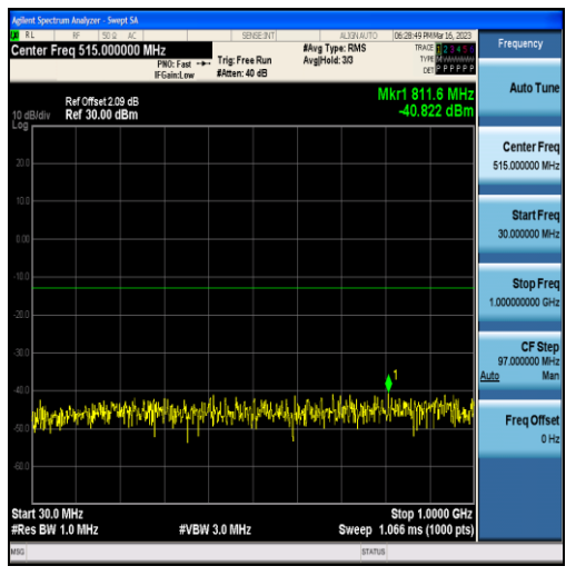
Band25-3MHz-QPSK-26675-15RB#0-Range1:30~1000MHz
