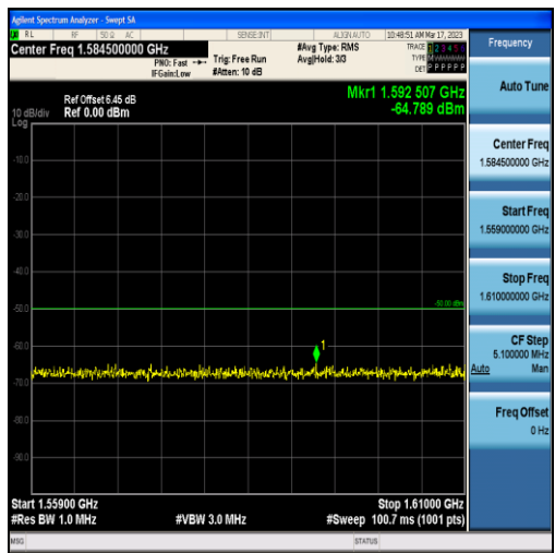
Band13-5MHz-QPSK-23230-25RB#0-Range3:1559~1610MHz
