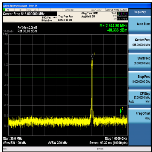
Band17-10MHz-16QAM-23800-50RB#0-Range1:30~1000MHz
