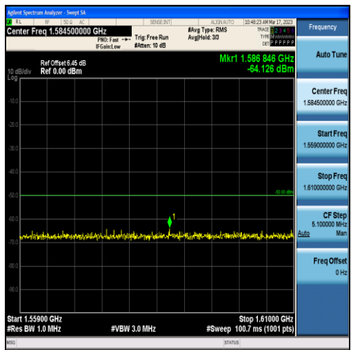
Band13-5MHz-QPSK-23205-25RB#0-Range3:1559~1610MHz
