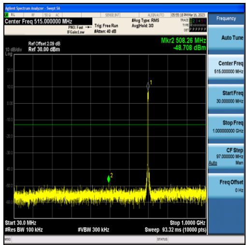
Band17-5MHz-QPSK-23755-25RB#0-Range1:30~1000MHz
