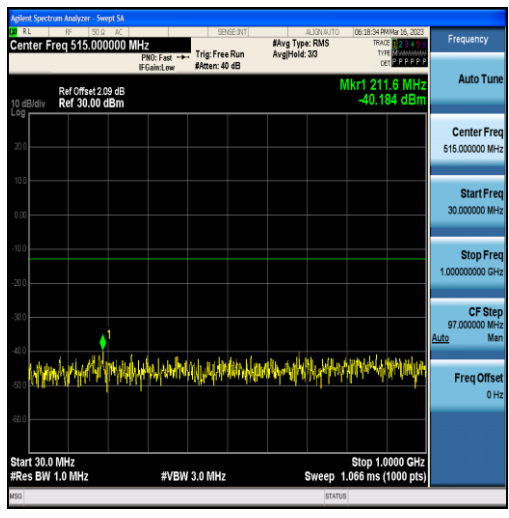
Band25-1.4MHz-QPSK-26683-6RB#0-Range1:30~1000MHz
