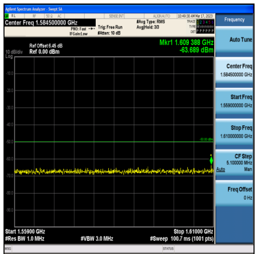
Band13-5MHz-16QAM-23255-25RB#0-Range3:1559~1610MHz
