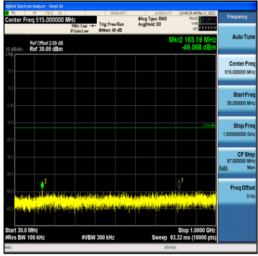
Band13-5MHz-16QAM-23205-25RB#0-Range1:30~1000MHz
