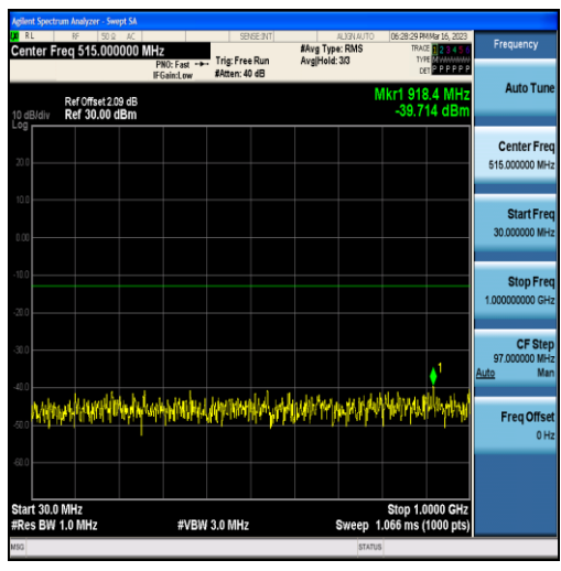
Band25-3MHz-QPSK-26365-15RB#0-Range1:30~1000MHz
