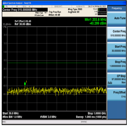
Band25-3MHz-QPSK-26055-15RB#0-Range1:30~1000MHz
