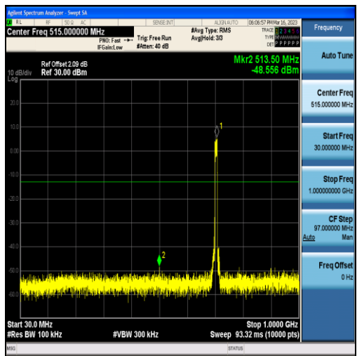
Band17-10MHz-QPSK-23800-50RB#0-Range1:30~1000MHz
