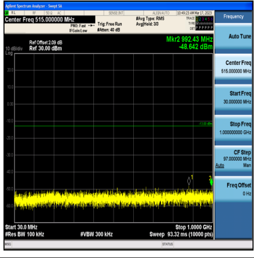
Band13-5MHz-16QAM-23255-25RB#0-Range1:30~1000MHz
