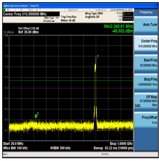
Band12-10MHz-16QAM-23060-50RB#0-Range1:30~1000MHz
