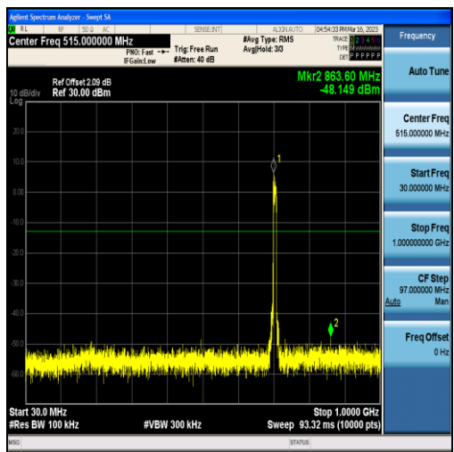
Band12-10MHz-16QAM-23130-50RB#0-Range1:30~1000MHz
