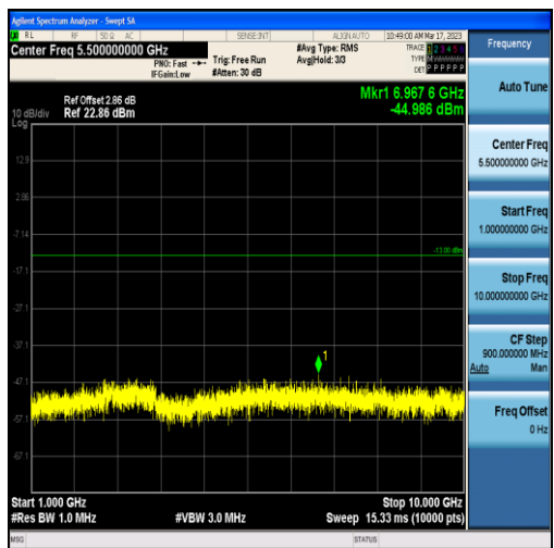
Band13-5MHz-16QAM-23230-25RB#0-Range2:1000~10000MHz
