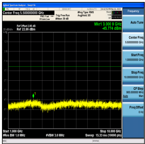
Band12-5MHz-16QAM-23155-25RB#0-Range2:1000~10000MHz
