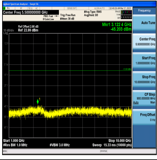
Band13-5MHz-16QAM-23255-25RB#0-Range2:1000~10000MHz
