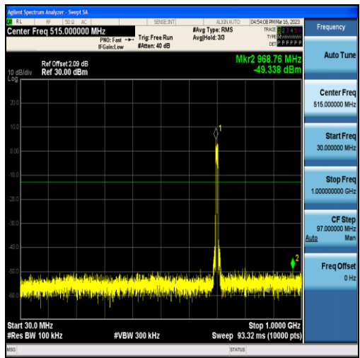
Band12-10MHz-16QAM-23095-50RB#0-Range1:30~1000MHz
