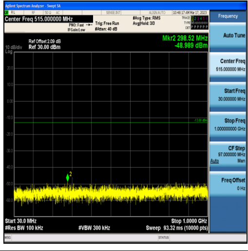
Band13-5MHz-QPSK-23205-25RB#0-Range1:30~1000MHz
