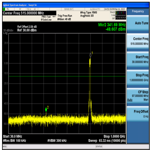
Band12-10MHz-QPSK-23060-50RB#0-Range1:30~1000MHz
