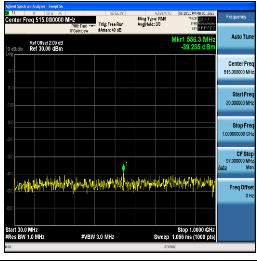
Band25-1.4MHz-16QAM-26365-6RB#0-Range1:30~1000MHz
