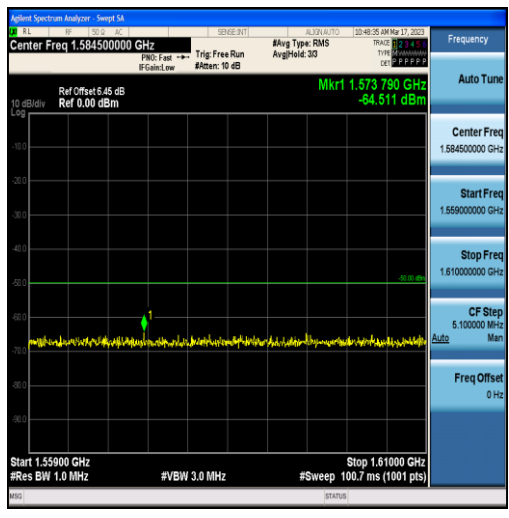
Band13-5MHz-16QAM-23205-25RB#0-Range3:1559~1610MHz
