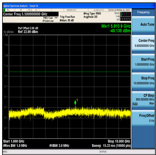
Band12-10MHz-16QAM-23095-50RB#0-Range2:1000~10000MHz
