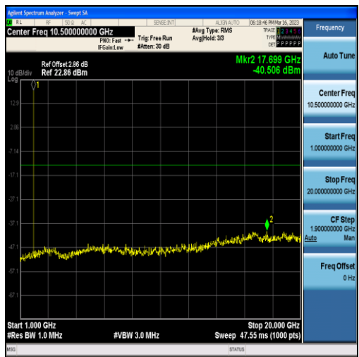
Band25-1.4MHz-16QAM-26683-6RB#0-Range2:1000~20000MHz
