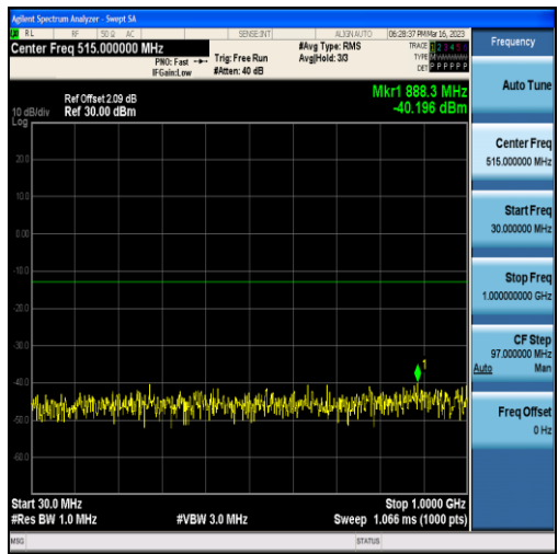
Band25-3MHz-16QAM-26365-15RB#0-Range1:30~1000MHz
