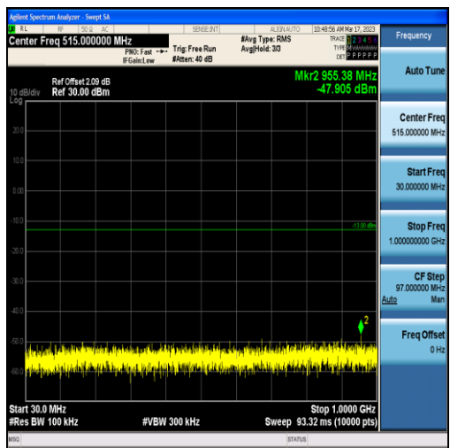
Band13-5MHz-16QAM-23230-25RB#0-Range1:30~1000MHz
