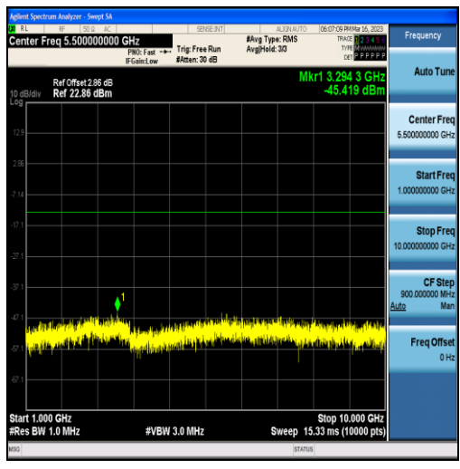
Band17-10MHz-16QAM-23800-50RB#0-Range2:1000~10000MHz
