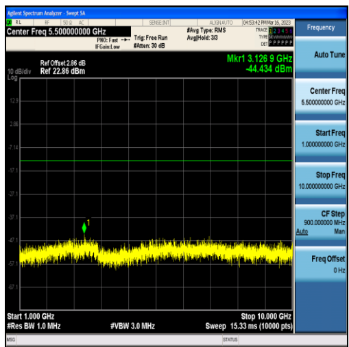
Band12-10MHz-QPSK-23060-50RB#0-Range2:1000~10000MHz
