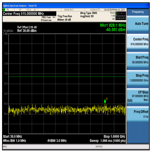
Band25-3MHz-16QAM-26675-15RB#0-Range1:30~1000MHz
