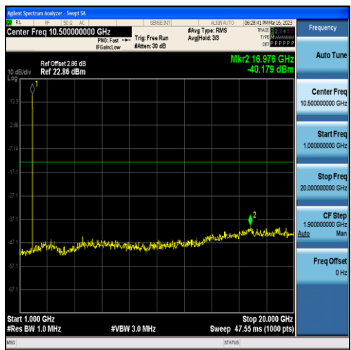
Band25-3MHz-16QAM-26365-15RB#0-Range2:1000~20000MHz
