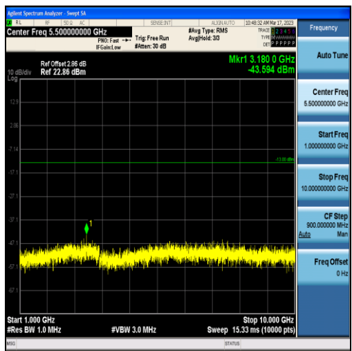
Band13-5MHz-16QAM-23205-25RB#0-Range2:1000~10000MHz
