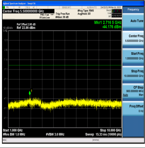
Band12-10MHz-16QAM-23060-50RB#0-Range2:1000~10000MHz
