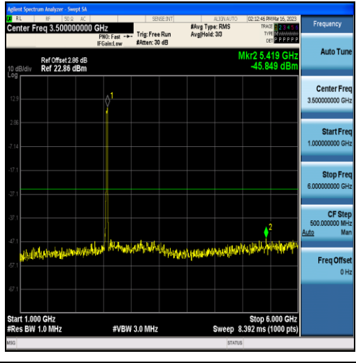
Band7-15MHz-16QAM-21375-75RB#0-Range2:1000~6000MHz
