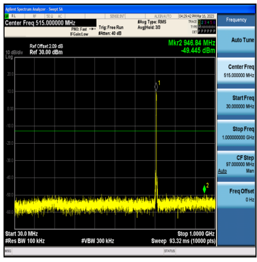
Band12-3MHz-QPSK-23165-15RB#0-Range1:30~1000MHz
