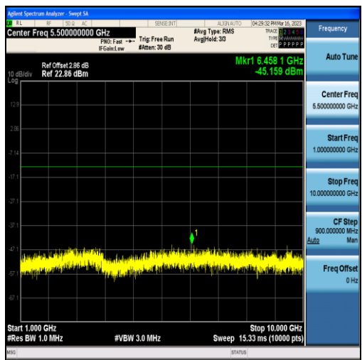
Band12-3MHz-16QAM-23095-15RB#0-Range2:1000~10000MHz
