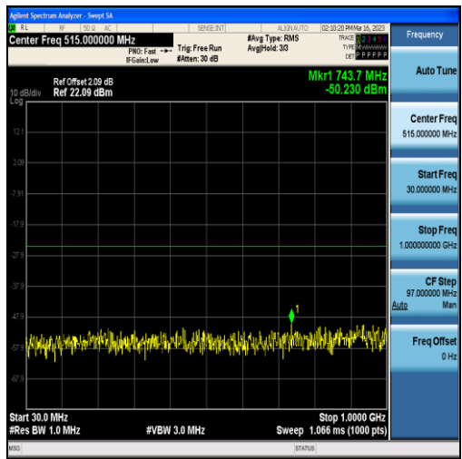
Band7-15MHz-16QAM-20825-75RB#0-Range1:30~1000MHz
