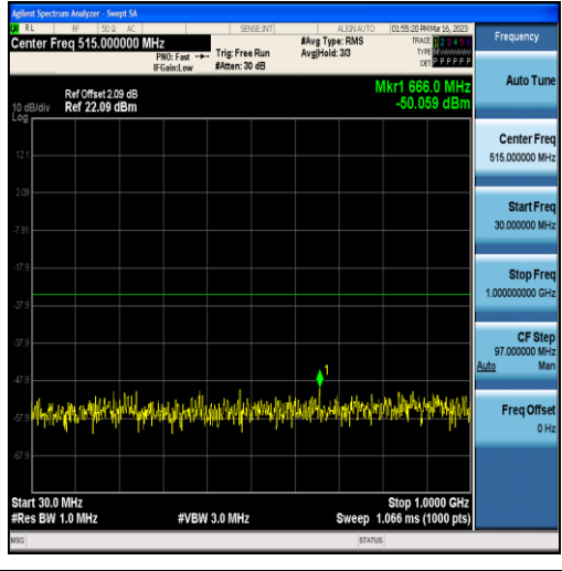
Band7-10MHz-16QAM-21400-50RB#0-Range1:30~1000MHz
