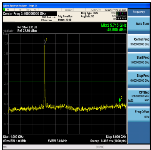
Band7-15MHz-16QAM-21100-75RB#0-Range2:1000~6000MHz
