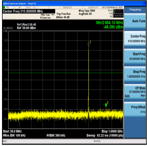
Band12-1.4MHz-16QAM-23095-6RB#0-Range1:30~1000MHz
