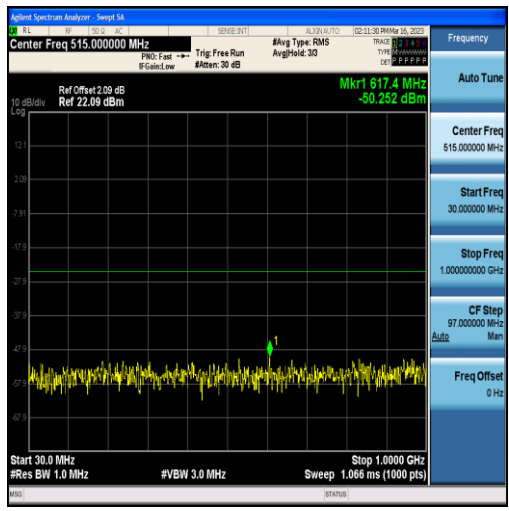
Band7-15MHz-QPSK-21100-75RB#0-Range1:30~1000MHz
