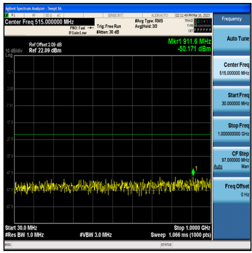
Band7-15MHz-16QAM-21100-75RB#0-Range1:30~1000MHz
