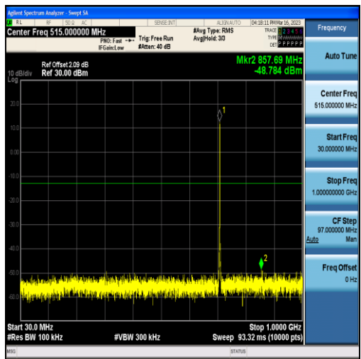
Band12-1.4MHz-QPSK-23173-6RB#0-Range1:30~1000MHz
