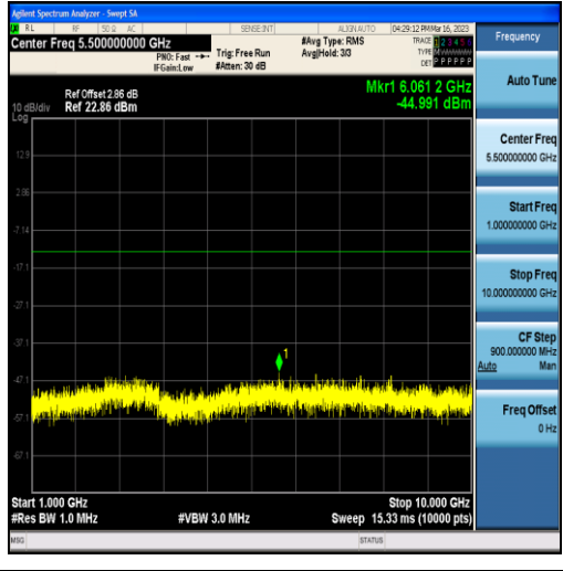
Band12-3MHz-16QAM-23025-15RB#0-Range2:1000~10000MHz
