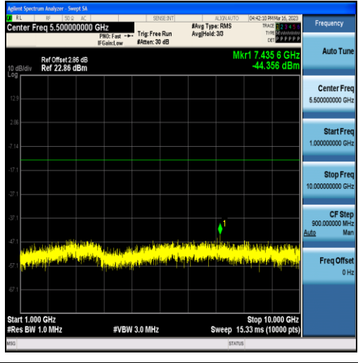
Band12-5MHz-16QAM-23035-25RB#0-Range2:1000~10000MHz
