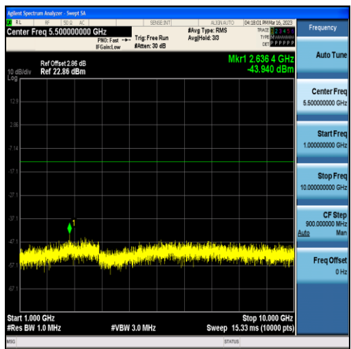
Band12-1.4MHz-16QAM-23095-6RB#0-Range2:1000~10000MHz
