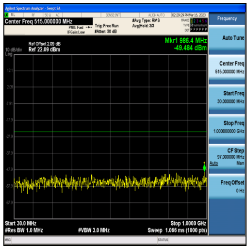
Band7-20MHz-16QAM-20850-100RB#0-Range1:30~1000MHz
