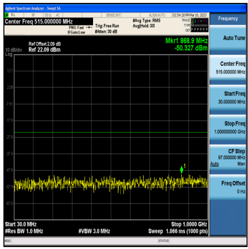
Band7-10MHz-16QAM-21100-50RB#0-Range1:30~1000MHz
