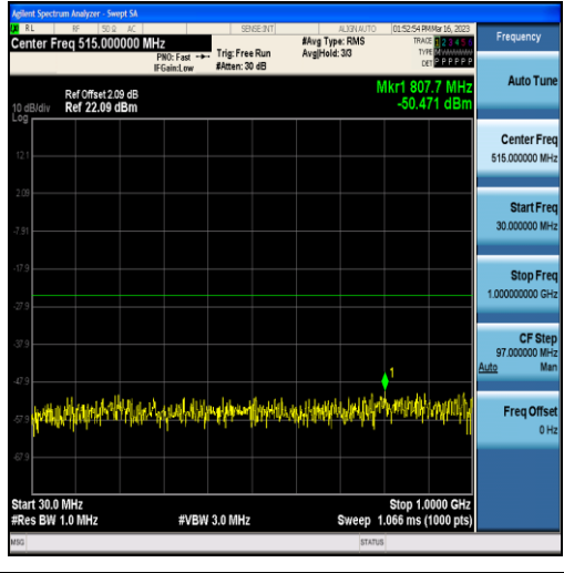
Band7-10MHz-16QAM-20800-50RB#0-Range1:30~1000MHz
