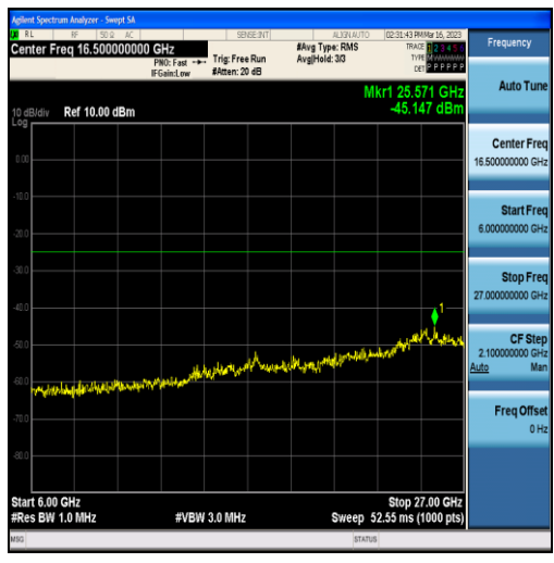
Band7-20MHz-16QAM-21100-100RB#0-Range3:6000~27000MHz
