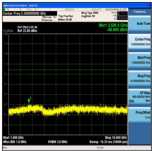
Band12-3MHz-QPSK-23095-15RB#0-Range2:1000~10000MHz
