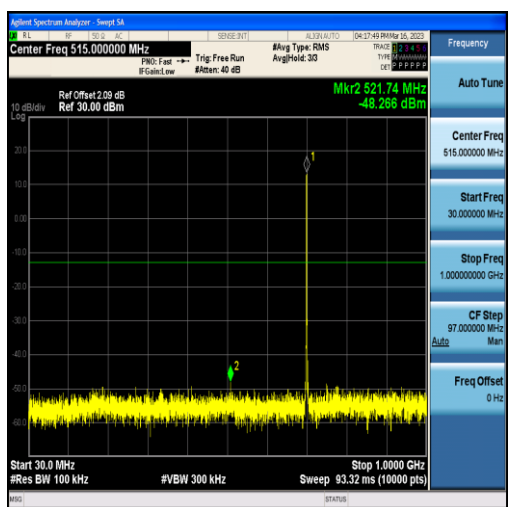
Band12-1.4MHz-QPSK-23095-6RB#0-Range1:30~1000MHz
