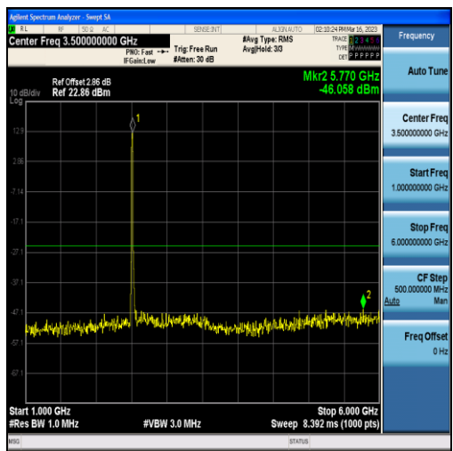
Band7-15MHz-16QAM-20825-75RB#0-Range2:1000~6000MHz
