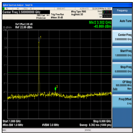
Band7-20MHz-16QAM-20850-100RB#0-Range2:1000~6000MHz
