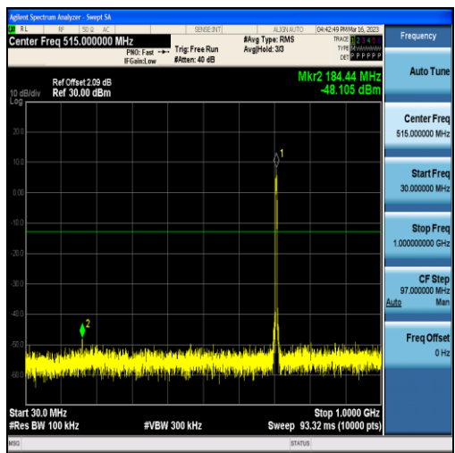
Band12-5MHz-16QAM-23155-25RB#0-Range1:30~1000MHz
