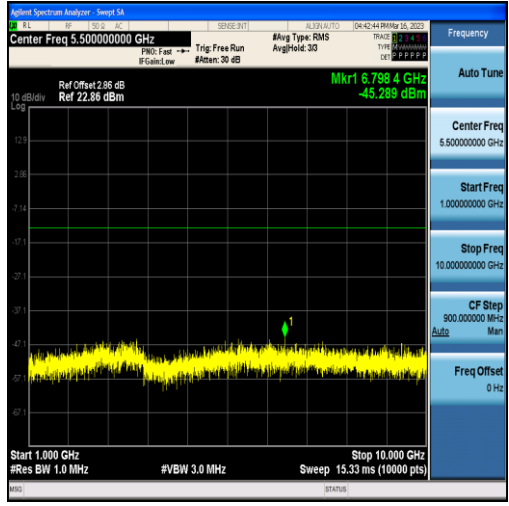
Band12-5MHz-QPSK-23155-25RB#0-Range2:1000~10000MHz
