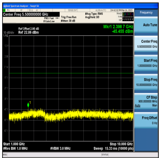
Band12-5MHz-QPSK-23035-25RB#0-Range2:1000~10000MHz
