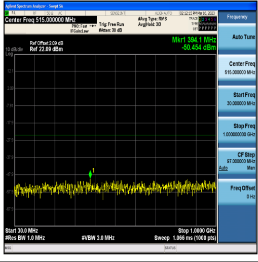
Band7-15MHz-QPSK-21375-75RB#0-Range1:30~1000MHz
