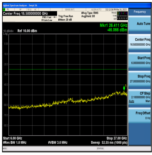
Band7-15MHz-16QAM-21100-75RB#0-Range3:6000~27000MHz
