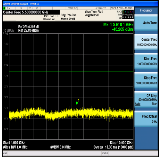
Band12-3MHz-QPSK-23165-15RB#0-Range2:1000~10000MHz
