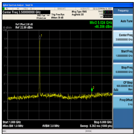
Band7-15MHz-QPSK-21100-75RB#0-Range2:1000~6000MHz
