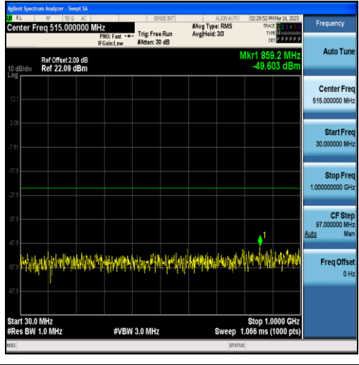
Band7-20MHz-QPSK-21100-100RB#0-Range1:30~1000MHz
