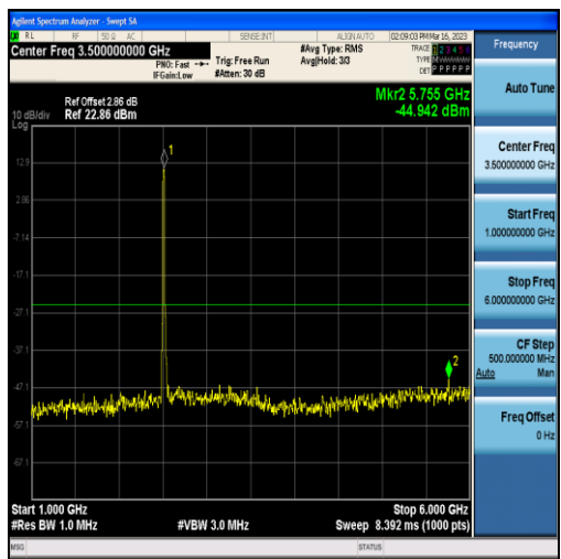
Band7-15MHz-QPSK-20825-75RB#0-Range2:1000~6000MHz
