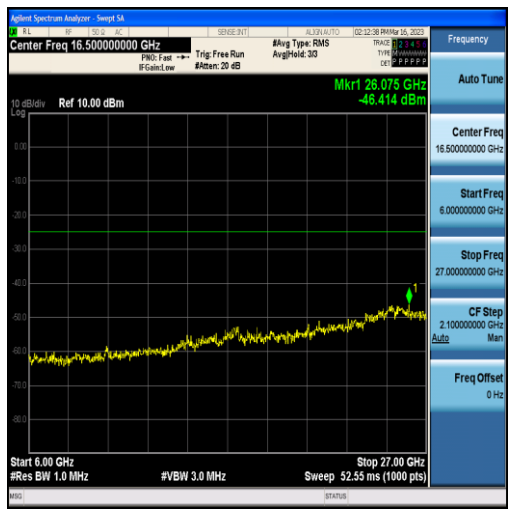
Band7-15MHz-QPSK-21375-75RB#0-Range3:6000~27000MHz
