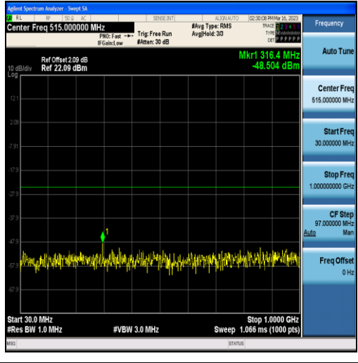
Band7-20MHz-16QAM-21100-100RB#0-Range1:30~1000MHz
