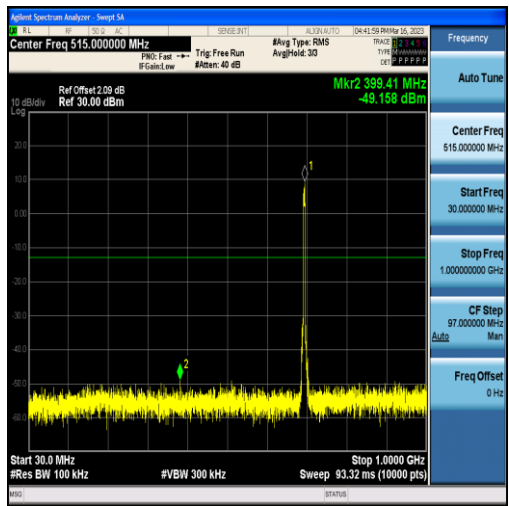
Band12-5MHz-QPSK-23035-25RB#0-Range1:30~1000MHz
