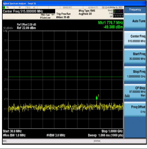
Band7-15MHz-16QAM-21375-75RB#0-Range1:30~1000MHz
