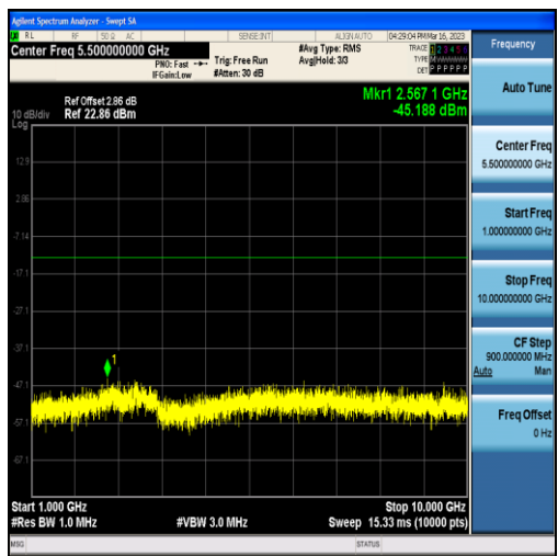
Band12-3MHz-QPSK-23025-15RB#0-Range2:1000~10000MHz
