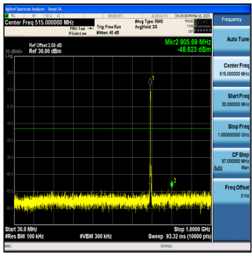
Band12-3MHz-16QAM-23025-15RB#0-Range1:30~1000MHz
