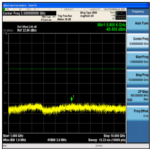
Band12-1.4MHz-QPSK-23095-6RB#0-Range2:1000~10000MHz
