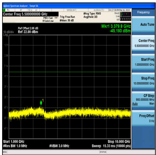
Band12-1.4MHz-16QAM-23017-6RB#0-Range2:1000~10000MHz
