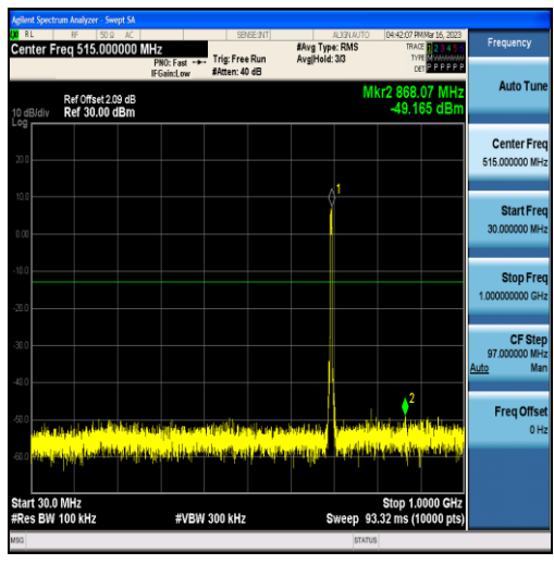
Band12-5MHz-16QAM-23035-25RB#0-Range1:30~1000MHz
