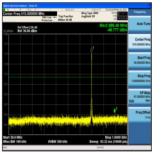
Band12-3MHz-QPSK-23095-15RB#0-Range1:30~1000MHz
