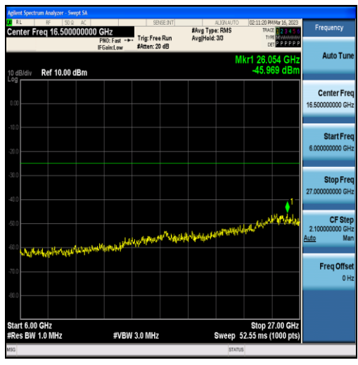
Band7-15MHz-16QAM-20825-75RB#0-Range3:6000~27000MHz
