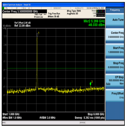
Band7-20MHz-16QAM-21100-100RB#0-Range2:1000~6000MHz
