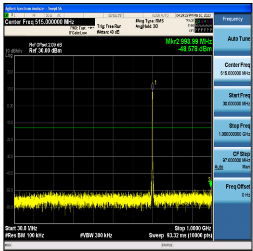
Band12-3MHz-16QAM-23095-15RB#0-Range1:30~1000MHz
