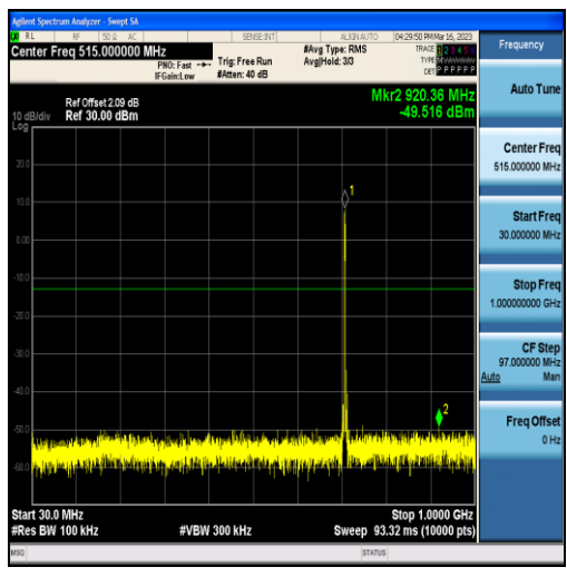
Band12-3MHz-16QAM-23165-15RB#0-Range1:30~1000MHz
