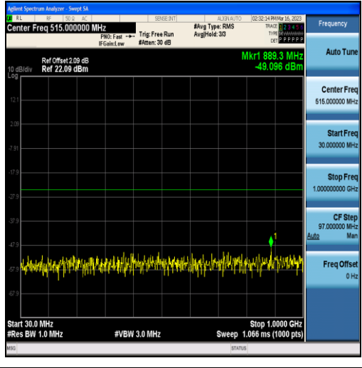
Band7-20MHz-16QAM-21350-100RB#0-Range1:30~1000MHz
