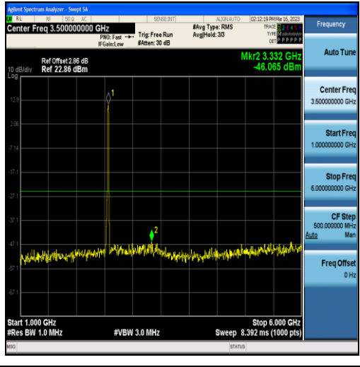
Band7-15MHz-QPSK-21375-75RB#0-Range2:1000~6000MHz
