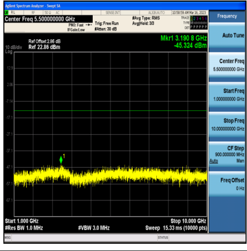
Band5-5MHz-16QAM-20425-25RB#0-Range2:1000~10000MHz
