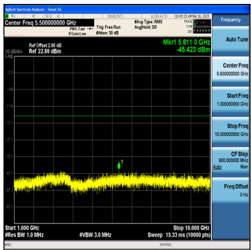
Band5-3MHz-16QAM-20525-15RB#0-Range2:1000~10000MHz
