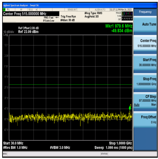
Band7-5MHz-QPSK-21425-25RB#0-Range1:30~1000MHz
