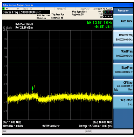
Band5-5MHz-QPSK-20425-25RB#0-Range2:1000~10000MHz
