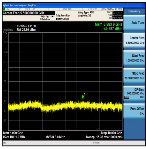
Band5-1.4MHz-QPSK-20525-6RB#0-Range2:1000~10000MHz
