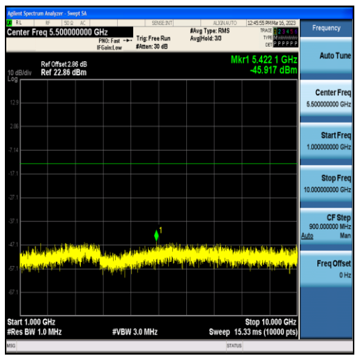
Band5-10MHz-16QAM-20525-50RB#0-Range2:1000~10000MHz
