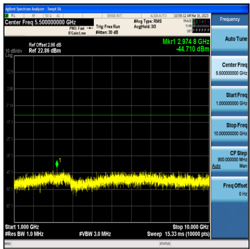
Band5-5MHz-QPSK-20525-25RB#0-Range2:1000~10000MHz
