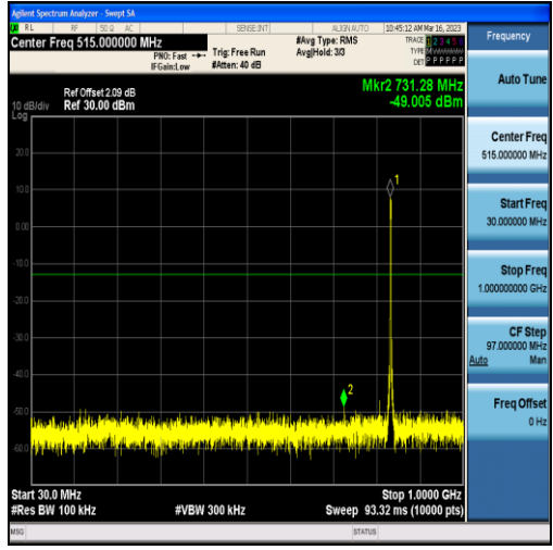
Band5-3MHz-16QAM-20525-15RB#0-Range1:30~1000MHz
