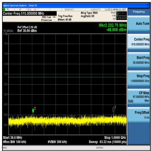
Band5-5MHz-QPSK-20625-25RB#0-Range1:30~1000MHz
