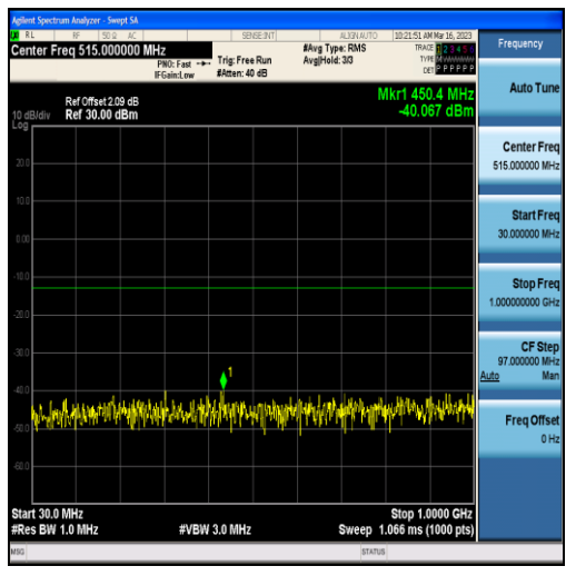
Band4-20MHz-QPSK-20300-100RB#0-Range1:30~1000MHz
