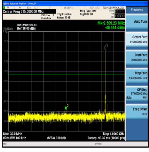
Band5-1.4MHz-16QAM-20525-6RB#0-Range1:30~1000MHz
