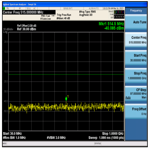
Band4-20MHz-16QAM-20300-100RB#0-Range1:30~1000MHz
