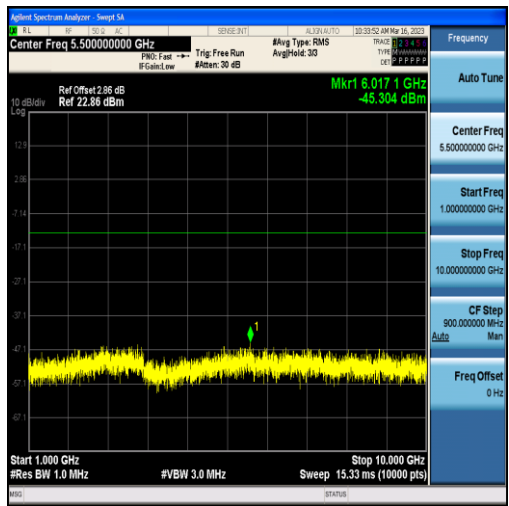
Band5-1.4MHz-16QAM-20407-6RB#0-Range2:1000~10000MHz
