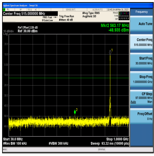
Band5-3MHz-QPSK-20635-15RB#0-Range1:30~1000MHz
