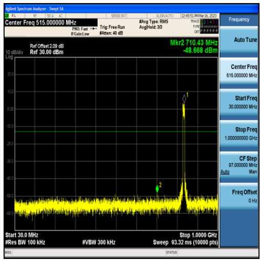
Band5-10MHz-16QAM-20525-50RB#0-Range1:30~1000MHz
