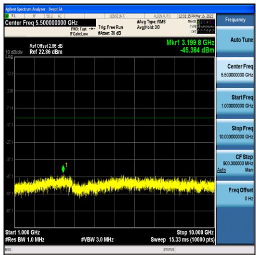
Band5-5MHz-16QAM-20625-25RB#0-Range2:1000~10000MHz
