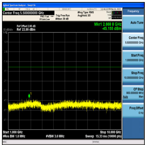
Band5-10MHz-16QAM-20600-50RB#0-Range2:1000~10000MHz
