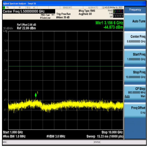
Band5-10MHz-16QAM-20450-50RB#0-Range2:1000~10000MHz
