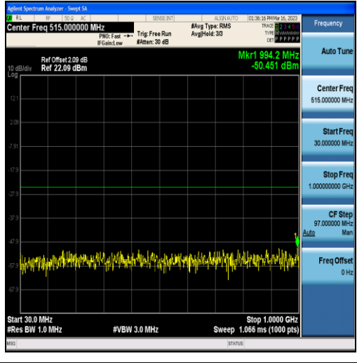
Band7-5MHz-16QAM-20775-25RB#0-Range1:30~1000MHz
