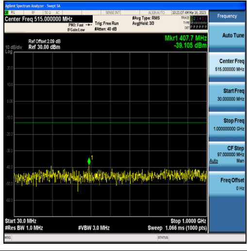
Band4-20MHz-QPSK-20050-100RB#0-Range1:30~1000MHz
