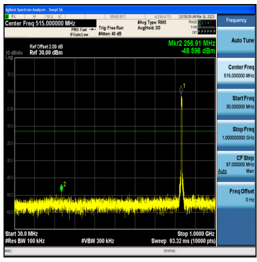
Band5-5MHz-QPSK-20525-25RB#0-Range1:30~1000MHz
