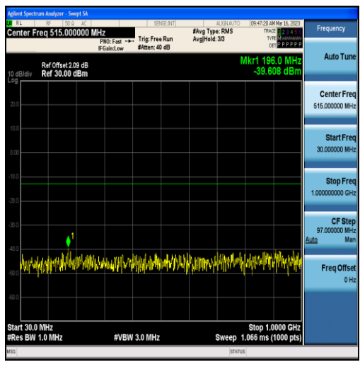
Band4-5MHz-16QAM-20375-25RB#0-Range1:30~1000MHz
