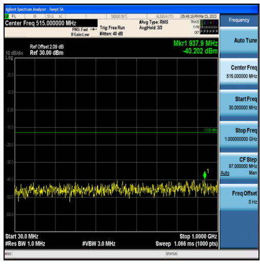
Band2-20MHz-16QAM-18700-100RB#0-Range1:30~1000MHz
