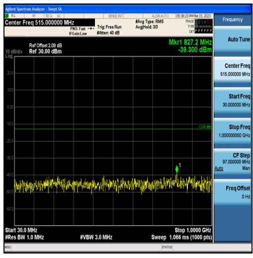
Band2-15MHz-QPSK-19125-75RB#0-Range1:30~1000MHz
