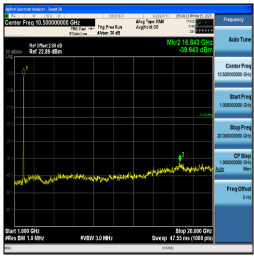
Band2-20MHz-16QAM-19100-100RB#0-Range2:1000~20000MHz
