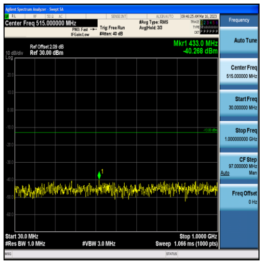
Band4-5MHz-16QAM-19975-25RB#0-Range1:30~1000MHz
