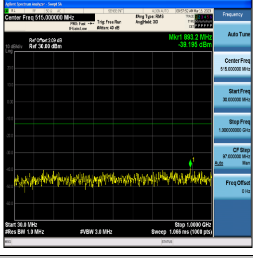
Band4-10MHz-16QAM-20350-50RB#0-Range1:30~1000MHz
