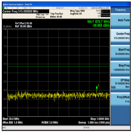
Band4-15MHz-QPSK-20025-75RB#0-Range1:30~1000MHz
