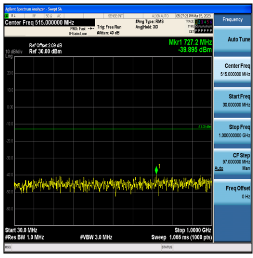
Band2-10MHz-QPSK-19150-50RB#0-Range1:30~1000MHz
