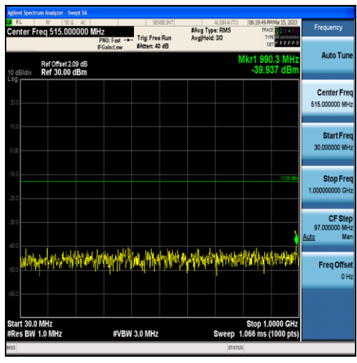
Band4-1.4MHz-16QAM-19957-6RB#0-Range1:30~1000MHz
