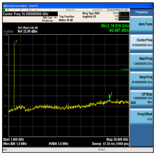
Band2-15MHz-16QAM-18900-75RB#0-Range2:1000~20000MHz
