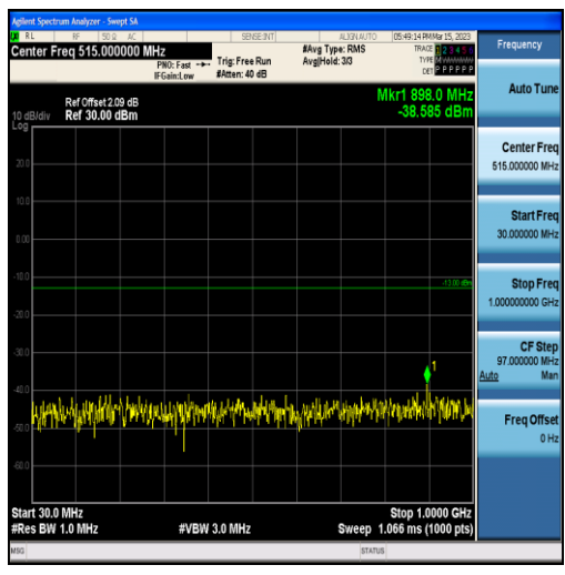
Band2-20MHz-16QAM-19100-100RB#0-Range1:30~1000MHz
