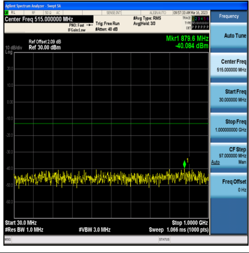
Band4-10MHz-16QAM-20175-50RB#0-Range1:30~1000MHz
