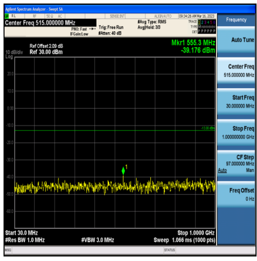
Band4-3MHz-QPSK-20385-15RB#0-Range1:30~1000MHz
