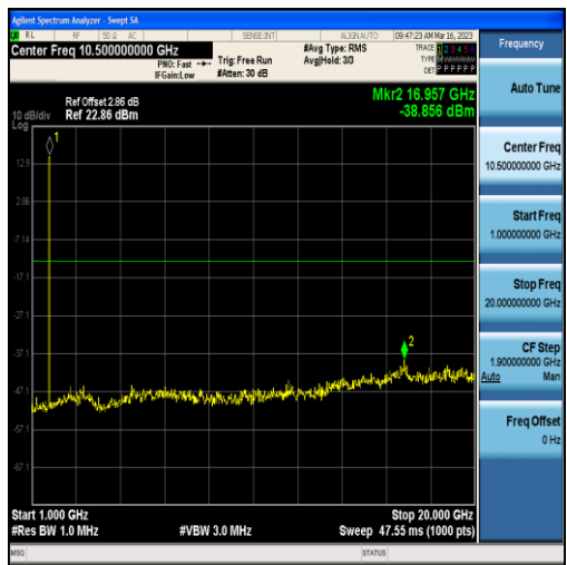
Band4-5MHz-16QAM-20375-25RB#0-Range2:1000~20000MHz
