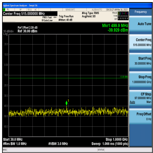
Band4-3MHz-16QAM-19965-15RB#0-Range1:30~1000MHz
