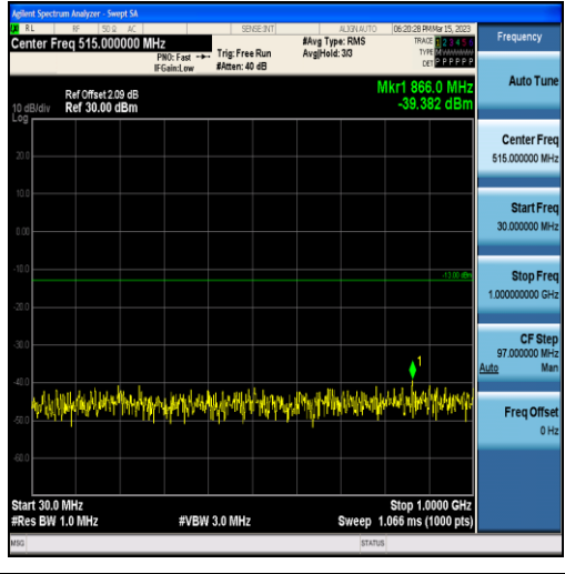
Band4-1.4MHz-16QAM-20175-6RB#0-Range1:30~1000MHz
