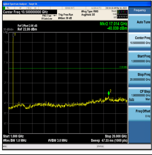
Band4-3MHz-16QAM-20175-15RB#0-Range2:1000~20000MHz
