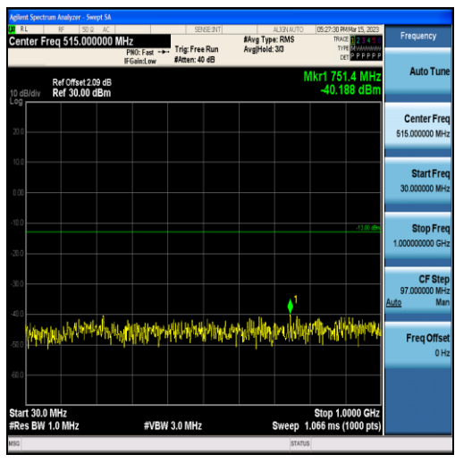
Band2-10MHz-16QAM-19150-50RB#0-Range1:30~1000MHz
