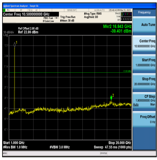
Band2-20MHz-16QAM-18900-100RB#0-Range2:1000~20000MHz
