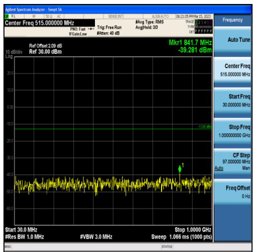
Band4-1.4MHz-16QAM-20393-6RB#0-Range1:30~1000MHz
