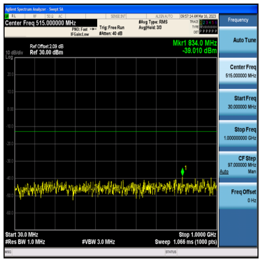
Band4-10MHz-16QAM-20000-50RB#0-Range1:30~1000MHz
