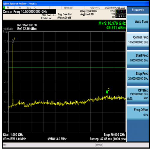
Band4-15MHz-16QAM-20025-75RB#0-Range2:1000~20000MHz
