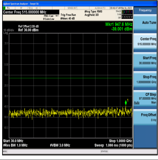
Band4-5MHz-16QAM-20175-25RB#0-Range1:30~1000MHz
