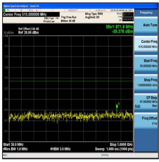
Band4-5MHz-QPSK-20175-25RB#0-Range1:30~1000MHz
