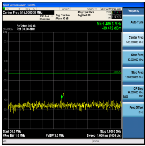
Band2-15MHz-QPSK-18675-75RB#0-Range1:30~1000MHz
