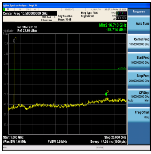
Band2-10MHz-16QAM-19150-50RB#0-Range2:1000~20000MHz
