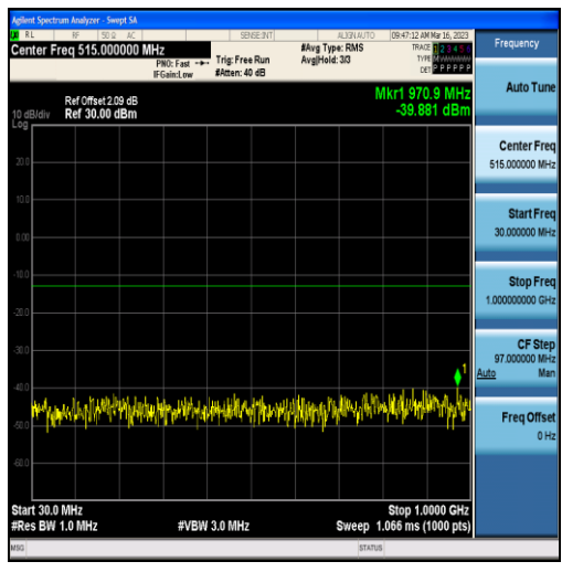
Band4-5MHz-QPSK-20375-25RB#0-Range1:30~1000MHz
