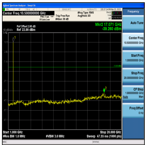
Band2-15MHz-QPSK-18675-75RB#0-Range2:1000~20000MHz
