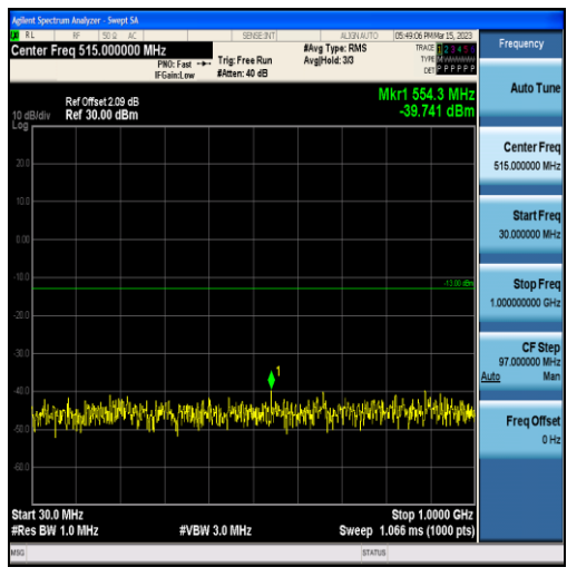
Band2-20MHz-QPSK-19100-100RB#0-Range1:30~1000MHz
