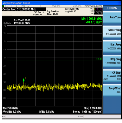
Band4-3MHz-16QAM-20175-15RB#0-Range1:30~1000MHz
