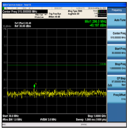
Band4-3MHz-16QAM-20385-15RB#0-Range1:30~1000MHz
