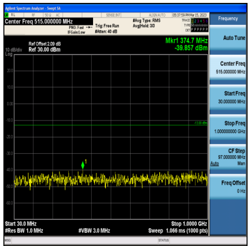
Band2-15MHz-16QAM-18900-75RB#0-Range1:30~1000MHz
