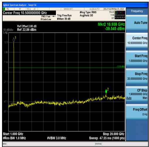
Band2-10MHz-16QAM-18900-50RB#0-Range2:1000~20000MHz
