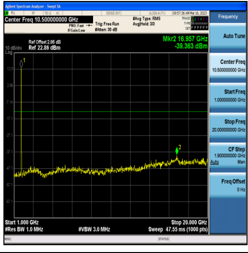
Band4-10MHz-16QAM-20175-50RB#0-Range2:1000~20000MHz
