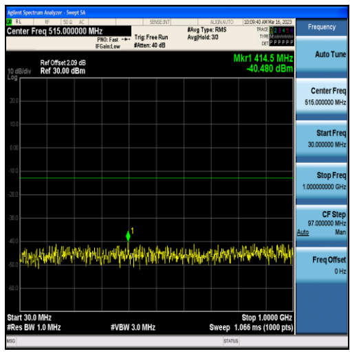
Band4-15MHz-16QAM-20025-75RB#0-Range1:30~1000MHz
