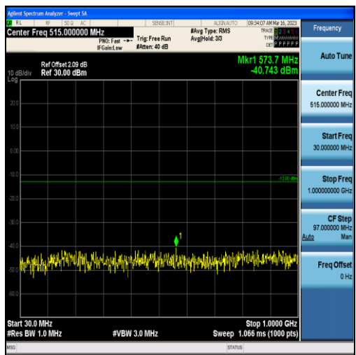
Band4-3MHz-QPSK-20175-15RB#0-Range1:30~1000MHz
