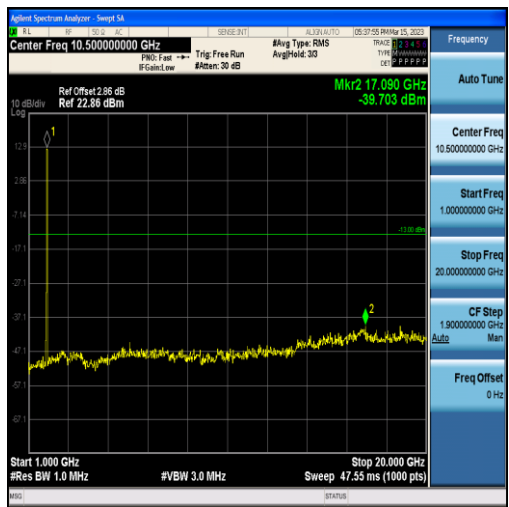
Band2-15MHz-QPSK-18900-75RB#0-Range2:1000~20000MHz
