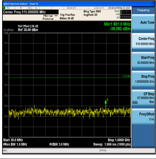
Band2-20MHz-16QAM-18900-100RB#0-Range1:30~1000MHz
