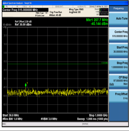
Band4-5MHz-QPSK-19975-25RB#0-Range1:30~1000MHz
