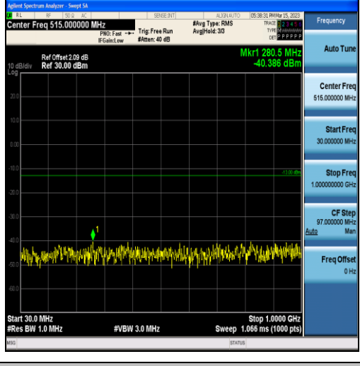
Band2-15MHz-16QAM-19125-75RB#0-Range1:30~1000MHz
