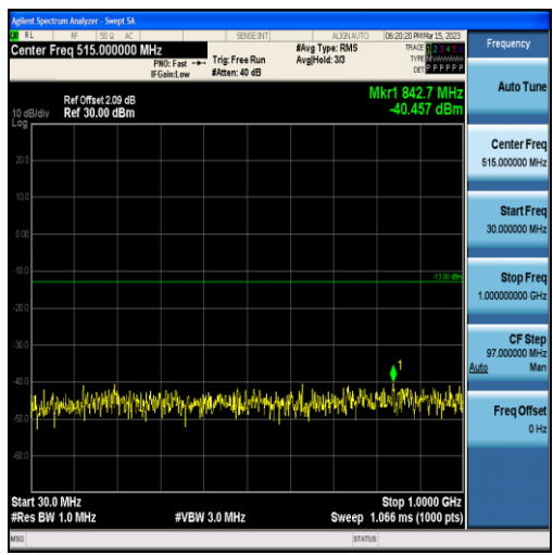
Band4-1.4MHz-QPSK-20175-6RB#0-Range1:30~1000MHz
