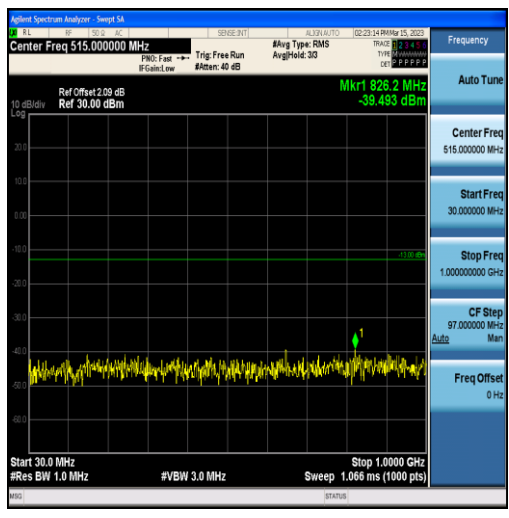
Band2-5MHz-16QAM-19175-25RB#0-Range1:30~1000MHz
