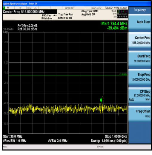
Band2-10MHz-QPSK-18650-50RB#0-Range1:30~1000MHz
