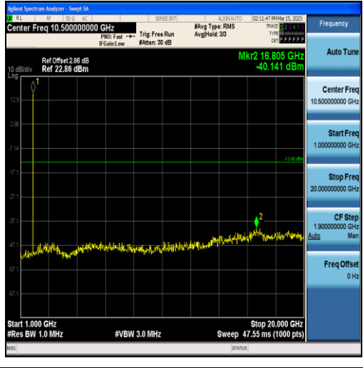
Band2-3MHz-16QAM-18615-15RB#0-Range2:1000~20000MHz
