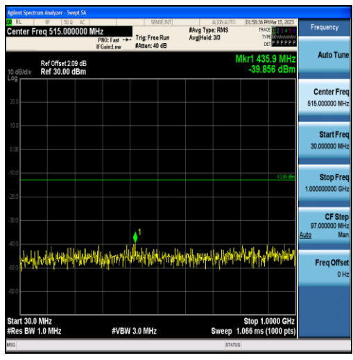
Band2-1.4MHz-QPSK-19193-6RB#0-Range1:30~1000MHz
