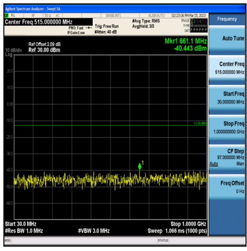
Band2-5MHz-QPSK-19175-25RB#0-Range1:30~1000MHz
