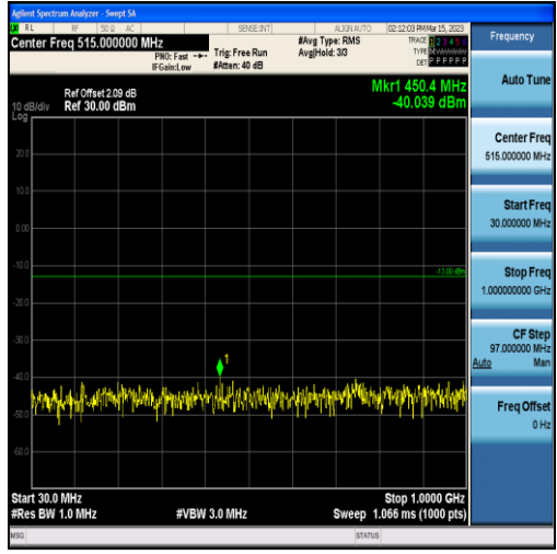
Band2-3MHz-16QAM-18900-15RB#0-Range1:30~1000MHz
