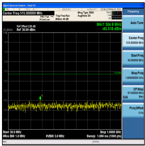
Band2-1.4MHz-QPSK-18900-6RB#0-Range1:30~1000MHz
