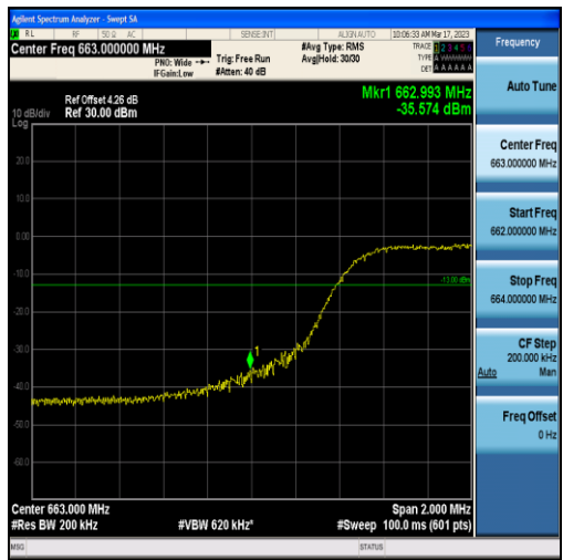
Band71-10MHz-16QAM-133172-50RB#0
