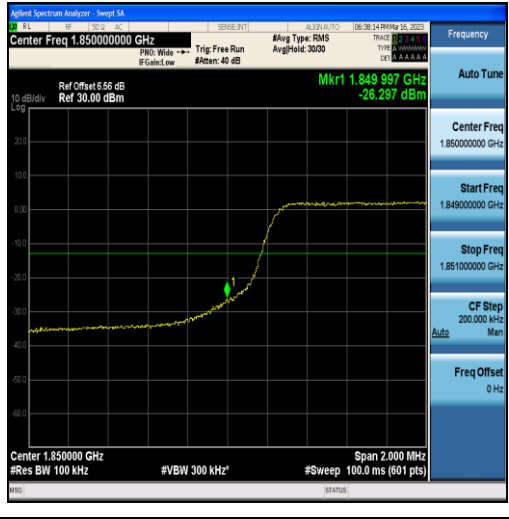
Band25-5MHz-16QAM-26065-25RB#0
