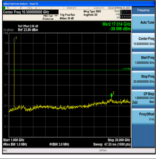
Band2-5MHz-16QAM-18625-25RB#0-Range2:1000~20000MHz
