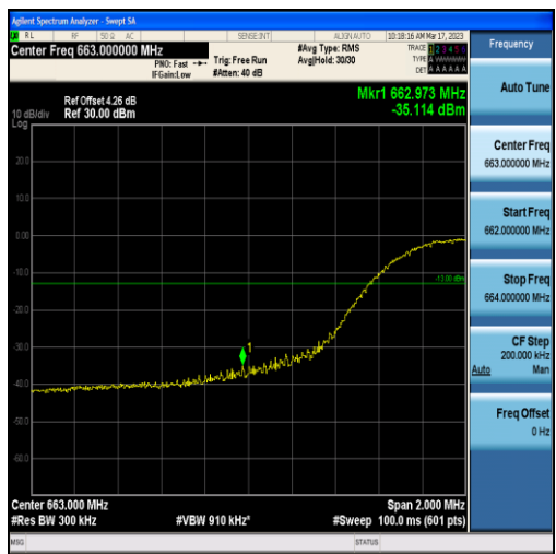
Band71-15MHz-16QAM-133197-75RB#0
