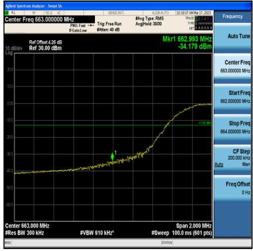
Band71-15MHz-QPSK-133197-75RB#0
