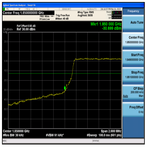
Band25-1.4MHz-16QAM-26047-6RB#0
