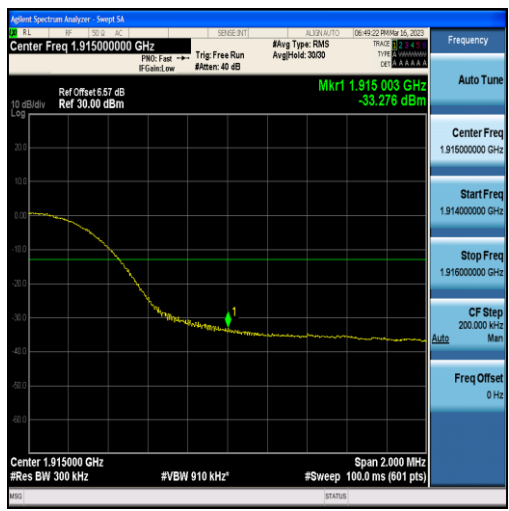
Band25-15MHz-16QAM-26615-75RB#0
