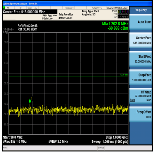
Band2-5MHz-QPSK-18625-25RB#0-Range1:30~1000MHz
