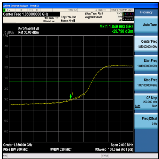
Band25-10MHz-QPSK-26090-50RB#0
