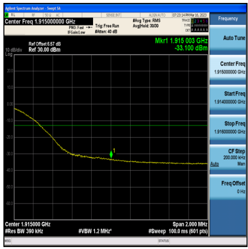
Band25-20MHz-16QAM-26590-100RB#0
