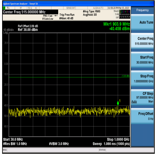
Band2-1.4MHz-16QAM-18900-6RB#0-Range1:30~1000MHz
