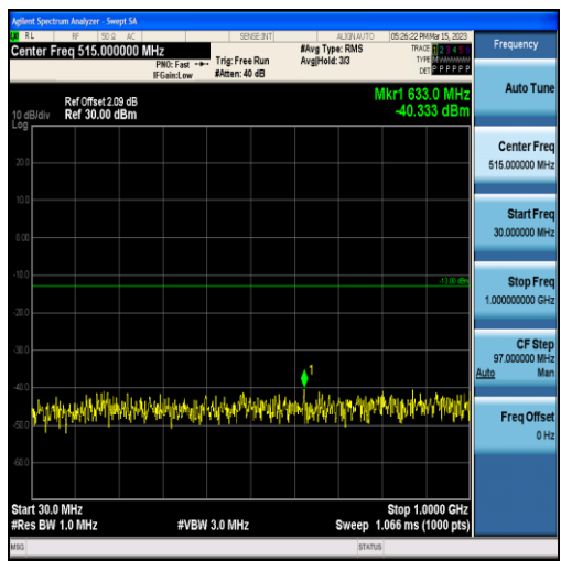
Band2-10MHz-QPSK-18900-50RB#0-Range1:30~1000MHz
