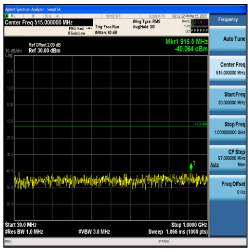
Band2-3MHz-16QAM-19185-15RB#0-Range1:30~1000MHz
