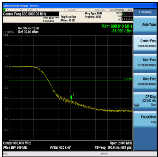
Band71-10MHz-16QAM-133422-50RB#0
