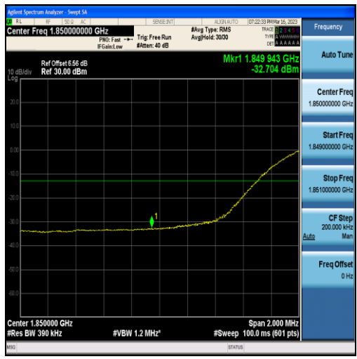
Band25-20MHz-QPSK-26140-100RB#0
