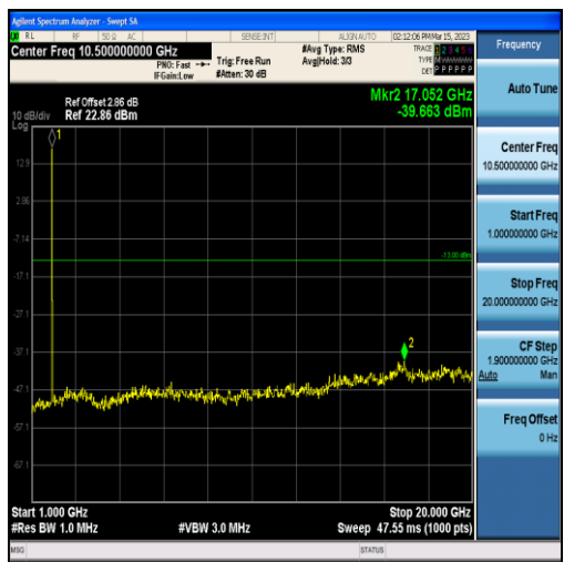
Band2-3MHz-16QAM-18900-15RB#0-Range2:1000~20000MHz
