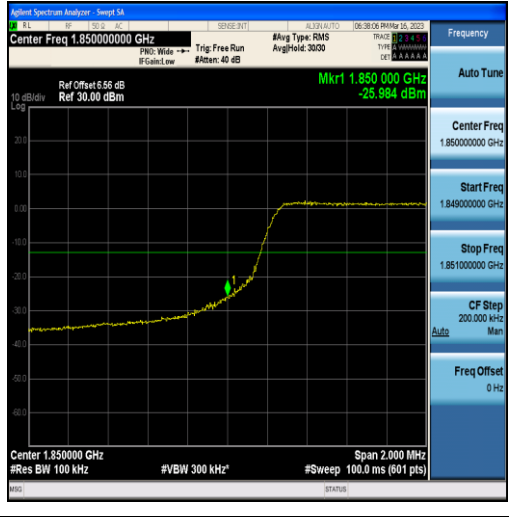
Band25-5MHz-QPSK-26065-25RB#0
