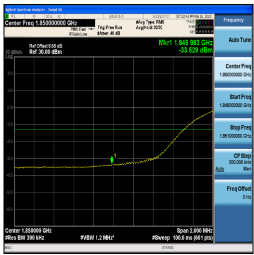
Band25-20MHz-16QAM-26140-100RB#0
