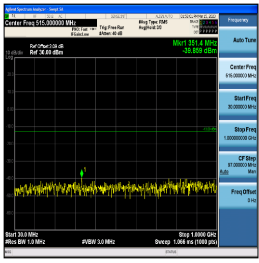
Band2-1.4MHz-16QAM-18607-6RB#0-Range1:30~1000MHz
