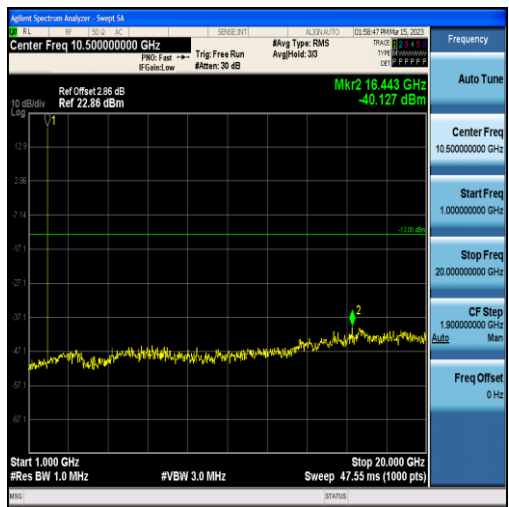
Band2-1.4MHz-16QAM-19193-6RB#0-Range2:1000~20000MHz
