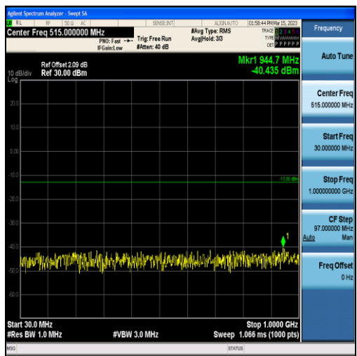
Band2-1.4MHz-16QAM-19193-6RB#0-Range1:30~1000MHz
