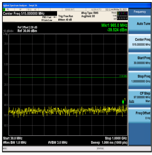
Band2-3MHz-16QAM-18615-15RB#0-Range1:30~1000MHz
