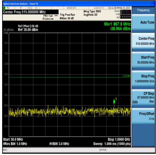
Band2-3MHz-QPSK-18615-15RB#0-Range1:30~1000MHz
