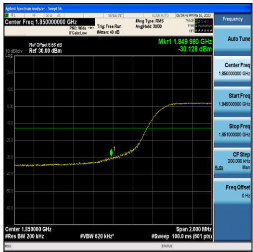
Band25-10MHz-16QAM-26090-50RB#0
