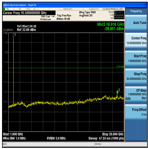
Band2-1.4MHz-16QAM-18607-6RB#0-Range2:1000~20000MHz
