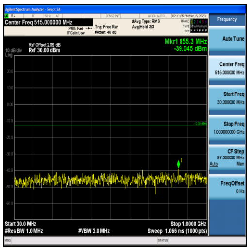
Band2-3MHz-QPSK-18900-15RB#0-Range1:30~1000MHz
