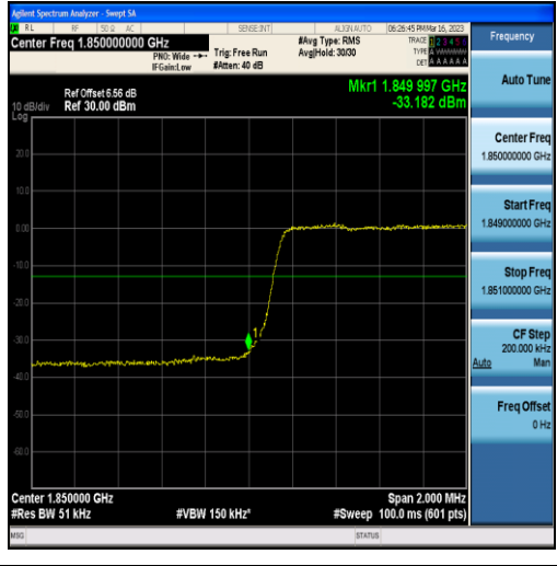
Band25-3MHz-16QAM-26055-15RB#0
