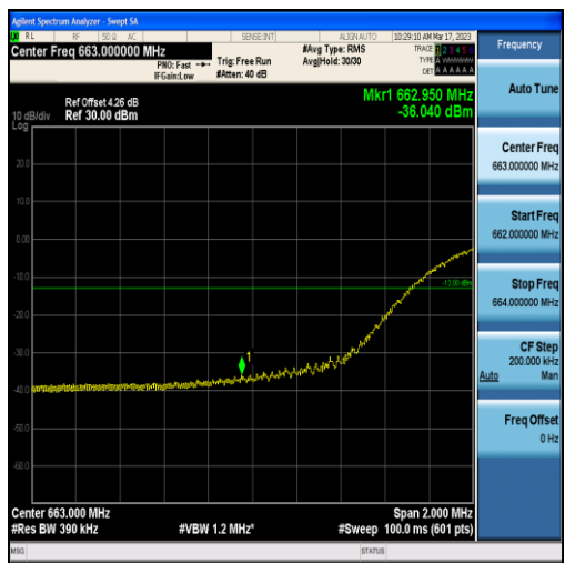
Band71-20MHz-QPSK-133222-100RB#0
