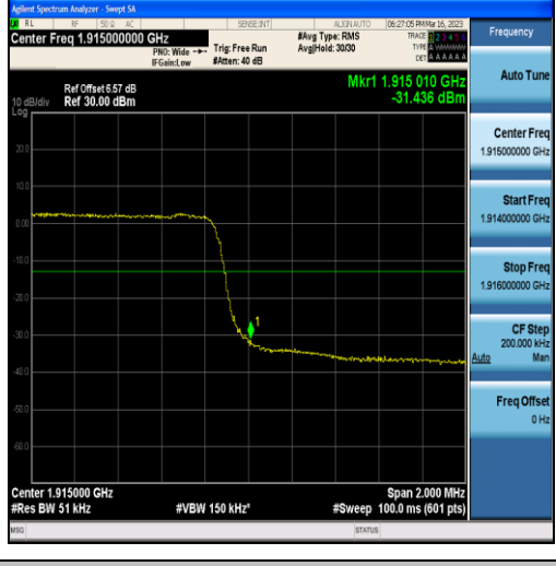
Band25-3MHz-QPSK-26675-15RB#0
