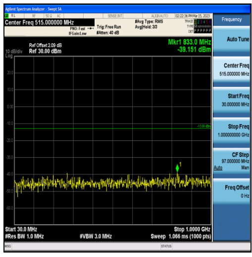
Band2-5MHz-16QAM-18625-25RB#0-Range1:30~1000MHz
