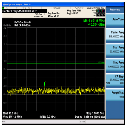
Band2-10MHz-16QAM-18650-50RB#0-Range1:30~1000MHz
