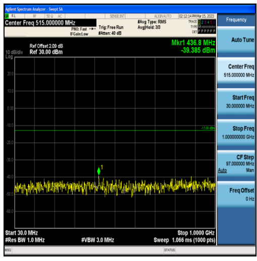
Band2-3MHz-QPSK-19185-15RB#0-Range1:30~1000MHz
