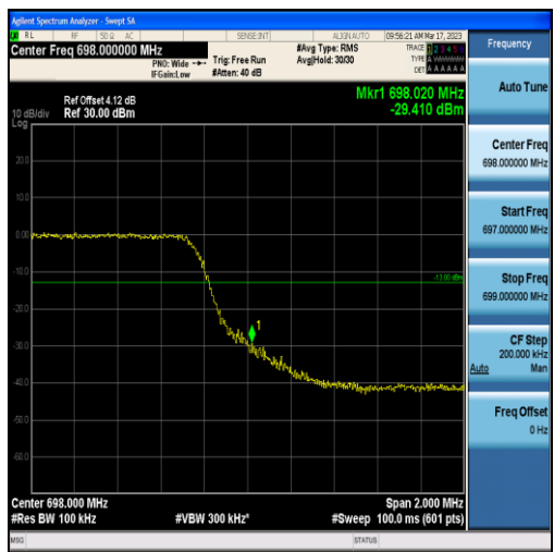
Band71-5MHz-16QAM-133447-25RB#0
