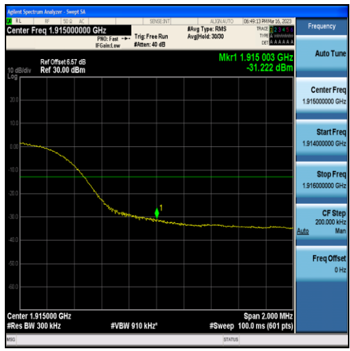
Band25-15MHz-QPSK-26615-75RB#0
