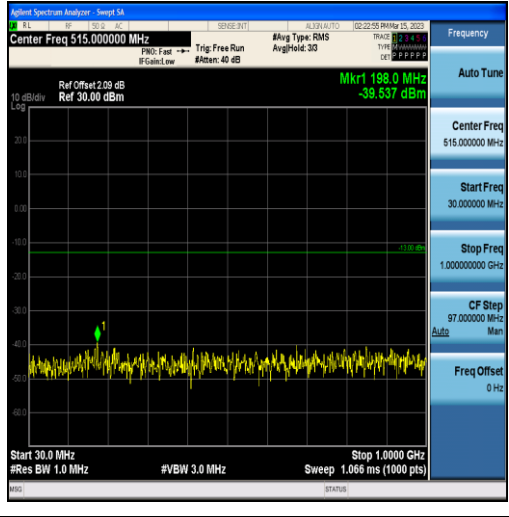
Band2-5MHz-16QAM-18900-25RB#0-Range1:30~1000MHz
