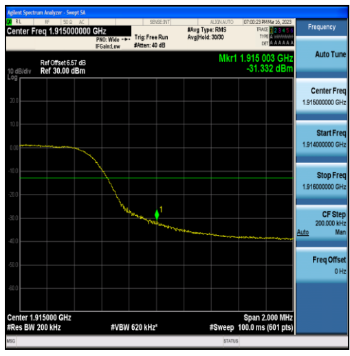
Band25-10MHz-16QAM-26640-50RB#0
