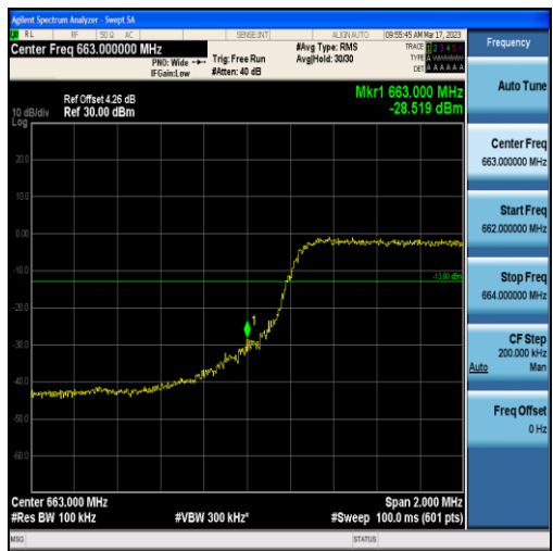
Band71-5MHz-16QAM-133147-25RB#0
