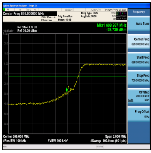
Band12-5MHz-16QAM-23035-25RB#0
