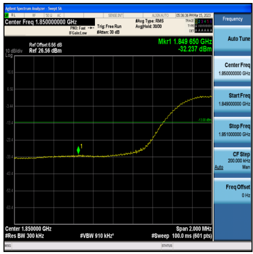
Band2-15MHz-QPSK-18675-75RB#0
