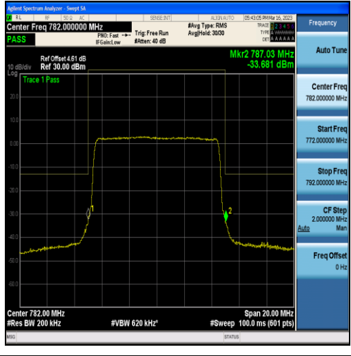
Band13-10MHz-QPSK-23230-50RB#0
