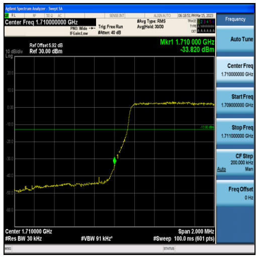
Band4-1.4MHz-16QAM-19957-6RB#0
