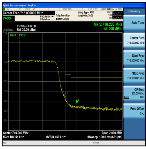
Band12-3MHz-16QAM-23165-15RB#0
