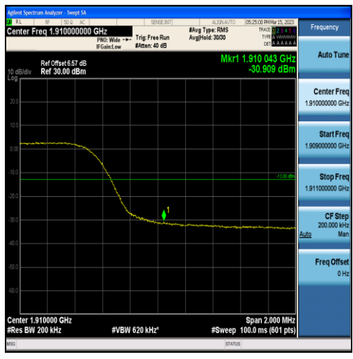
Band2-10MHz-16QAM-19150-50RB#0
