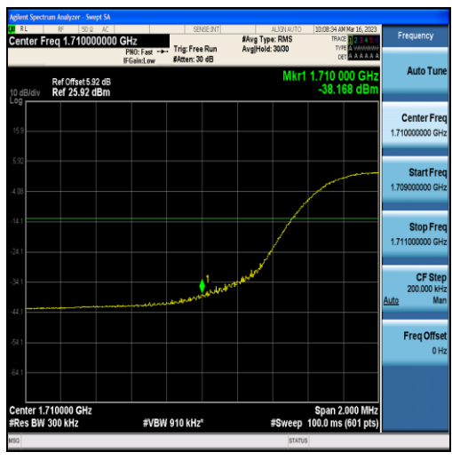
Band4-15MHz-16QAM-20025-75RB#0
