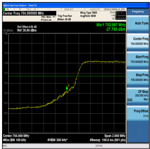
Band17-5MHz-QPSK-23755-25RB#0
