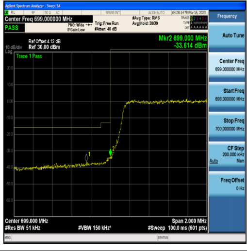
Band12-3MHz-16QAM-23025-15RB#0
