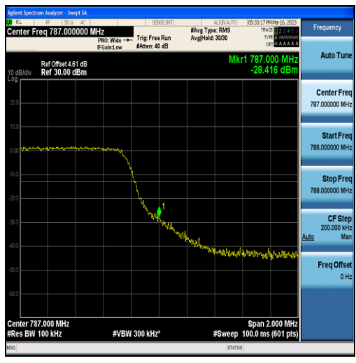
Band13-5MHz-16QAM-23255-25RB#0
