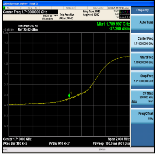
Band4-15MHz-QPSK-20025-75RB#0
