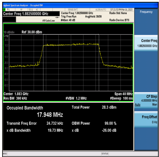
Band25-20MHz-16QAM-26365-100RB#0-17.948
