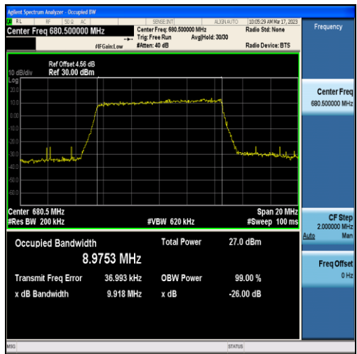
Band71-10MHz-16QAM-133297-50RB#0-8.9753
