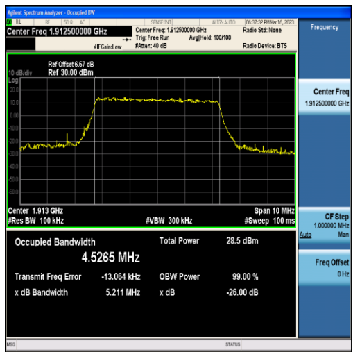
Band25-5MHz-QPSK-26665-25RB#0-4.5265
