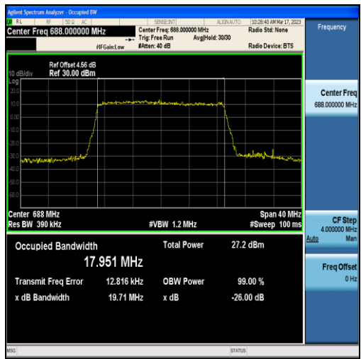
Band71-20MHz-16QAM-133372-100RB#0-17.951
