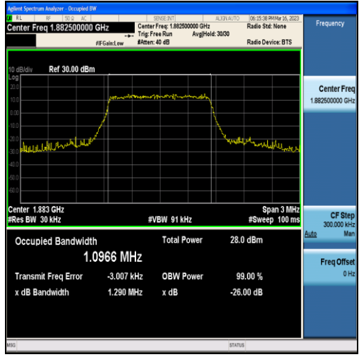
Band25-1.4MHz-QPSK-26365-6RB#0-1.0966
