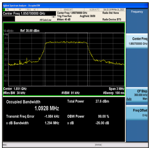
Band25-1.4MHz-QPSK-26047-6RB#0-1.0928
