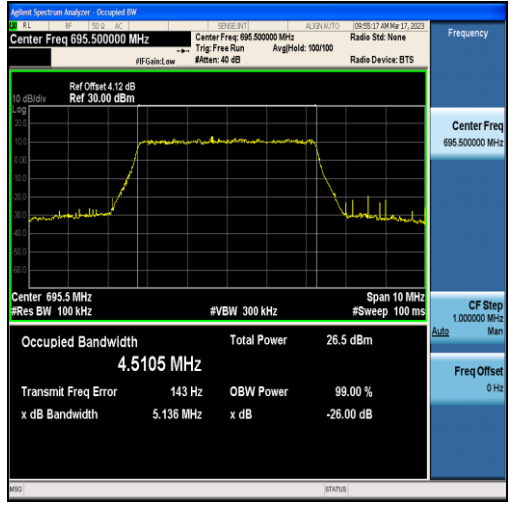
Band71-5MHz-16QAM-133447-25RB#0-4.5105
