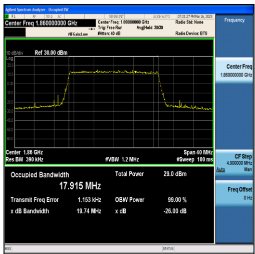
Band25-20MHz-QPSK-26140-100RB#0-17.915
