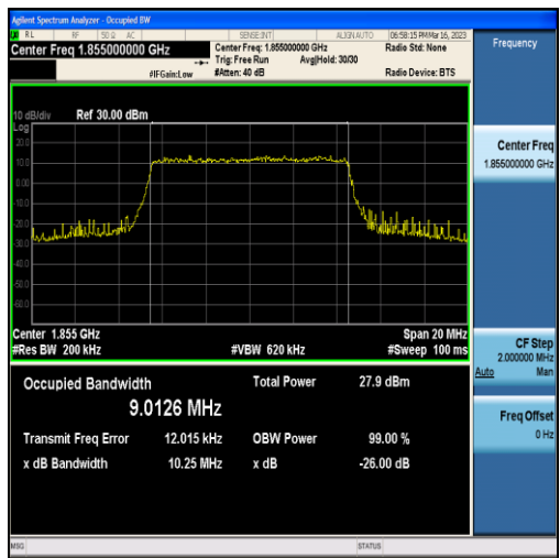
Band25-10MHz-16QAM-26090-50RB#0-9.0126
