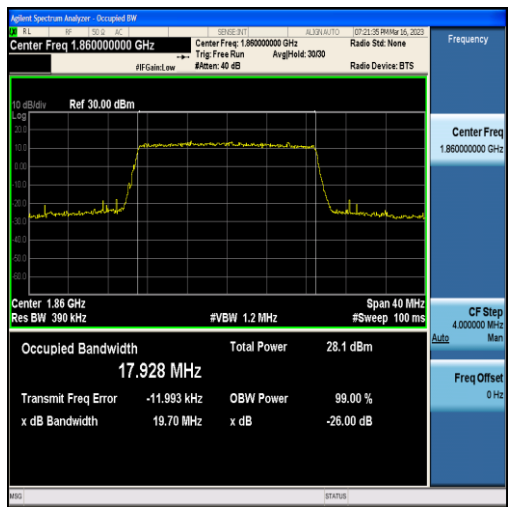
Band25-20MHz-16QAM-26140-100RB#0-17.928
