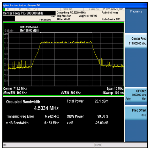
Band17-5MHz-QPSK-23825-25RB#0-4.5034
