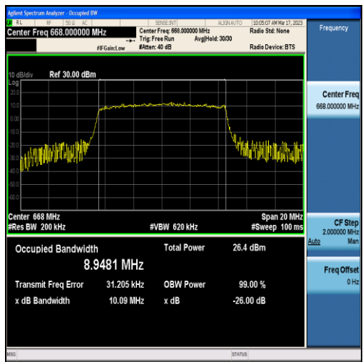
Band71-10MHz-16QAM-133172-50RB#0-8.9481
