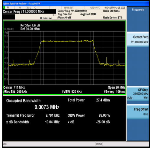
Band17-10MHz-16QAM-23800-50RB#0-9.0073
