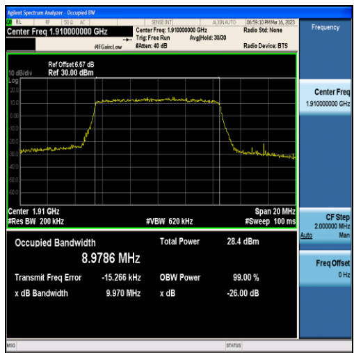
Band25-10MHz-QPSK-26640-50RB#0-8.9786
