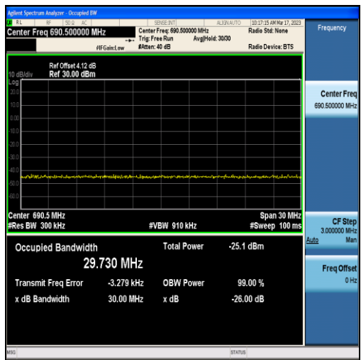
Band71-15MHz-QPSK-133397-75RB#0-29.730
