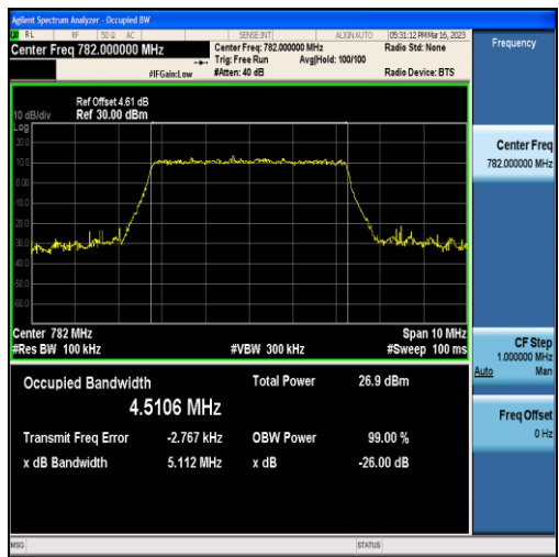
Band13-5MHz-16QAM-23230-25RB#0-4.5106
