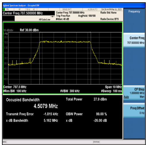
Band12-5MHz-QPSK-23095-25RB#0-4.5079
