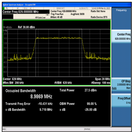
Band5-10MHz-QPSK-20450-50RB#0-8.9869
