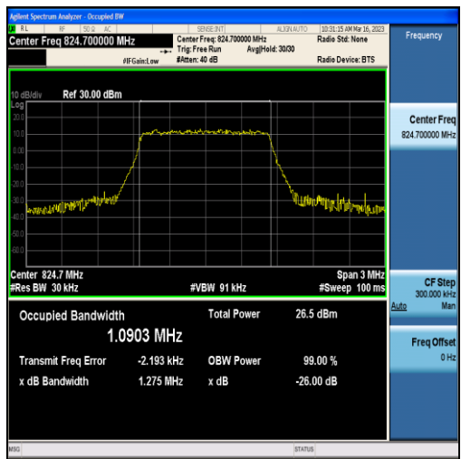
Band5-1.4MHz-QPSK-20407-6RB#0-1.0903
