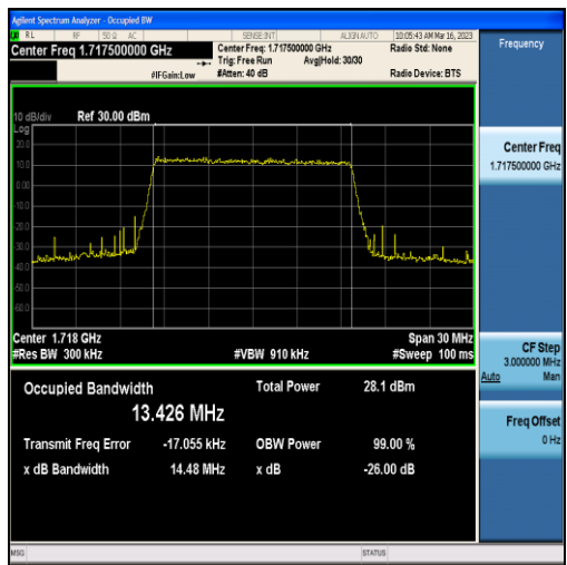
Band4-15MHz-QPSK-20025-75RB#0-13.426
