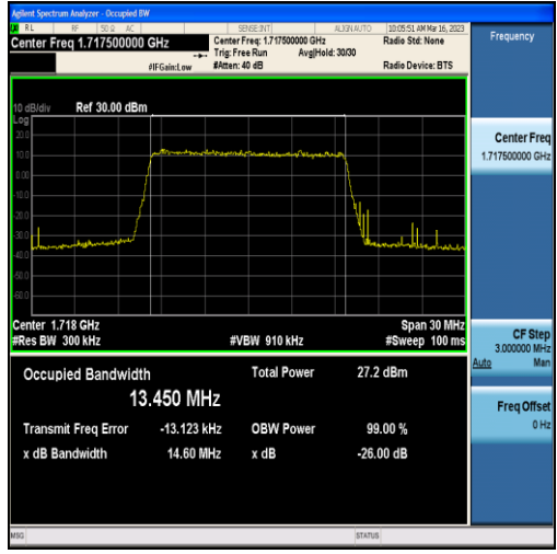
Band4-15MHz-16QAM-20025-75RB#0-13.450
