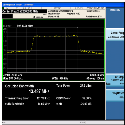
Band7-15MHz-16QAM-21375-75RB#0-13.487
