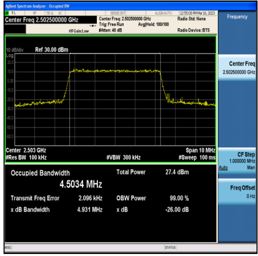
Band7-5MHz-16QAM-20775-25RB#0-4.5034
