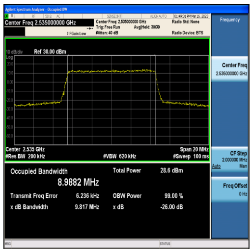
Band7-10MHz-QPSK-21100-50RB#0-8.9882
