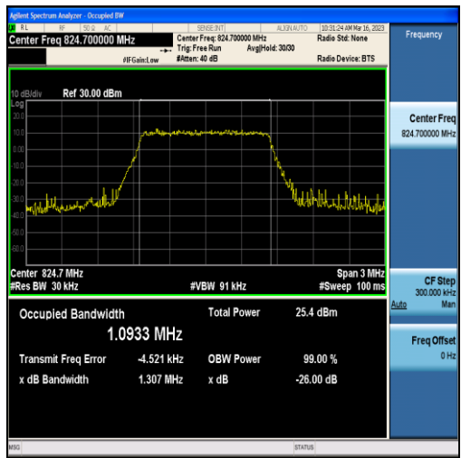
Band5-1.4MHz-16QAM-20407-6RB#0-1.0933
