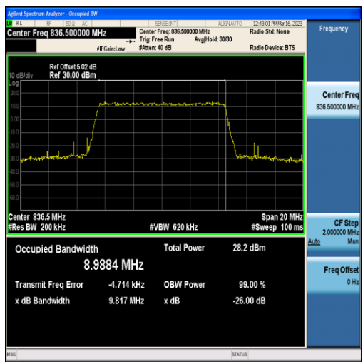
Band5-10MHz-QPSK-20525-50RB#0-8.9884
