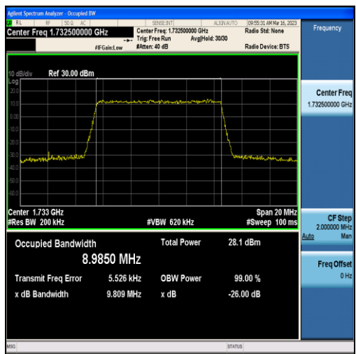
Band4-10MHz-QPSK-20175-50RB#0-8.9850
