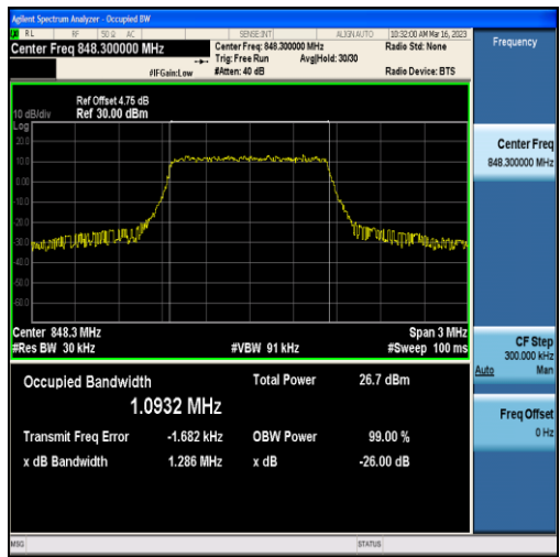
Band5-1.4MHz-QPSK-20643-6RB#0-1.0932
