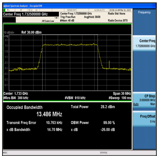
Band4-15MHz-QPSK-20175-75RB#0-13.486
