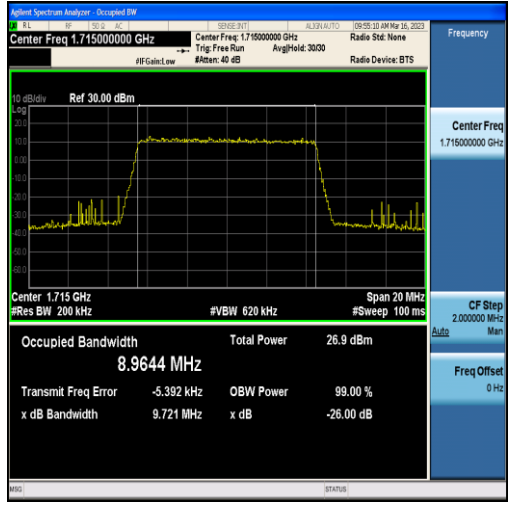
Band4-10MHz-16QAM-20000-50RB#0-8.9644
