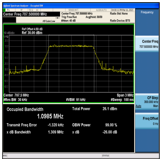
Band12-1.4MHz-16QAM-23095-6RB#0-1.0985
