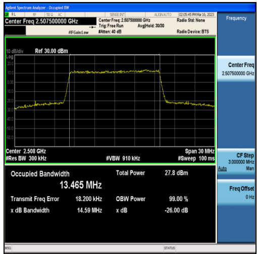
Band7-15MHz-16QAM-20825-75RB#0-13.465
