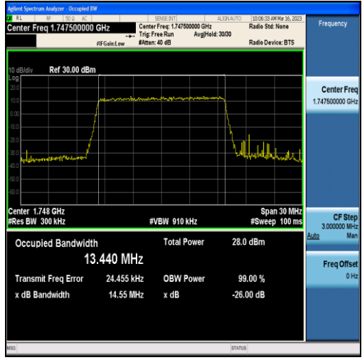
Band4-15MHz-QPSK-20325-75RB#0-13.440
