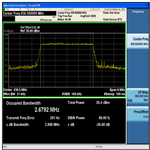
Band5-3MHz-16QAM-20525-15RB#0-2.6792
