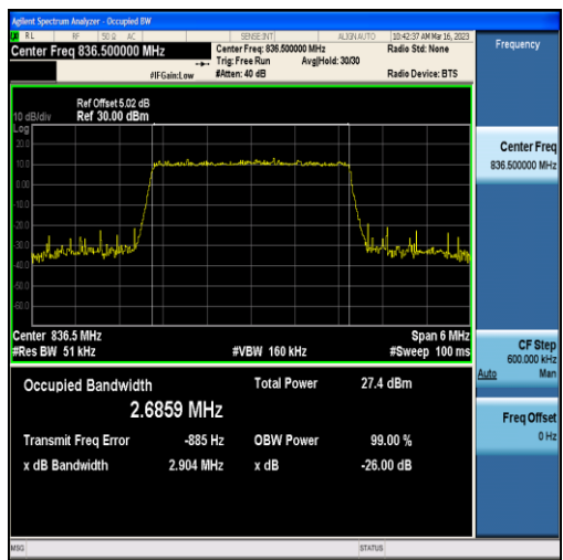
Band5-3MHz-QPSK-20525-15RB#0-2.6859
