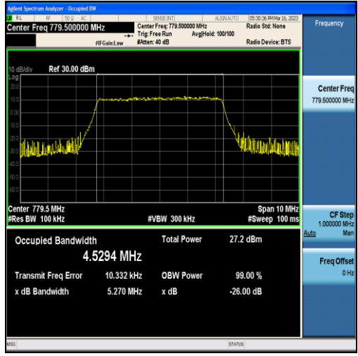
Band13-5MHz-16QAM-23205-25RB#0-4.5294
