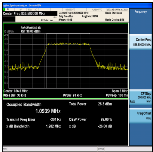
Band5-1.4MHz-16QAM-20525-6RB#0-1.0939
