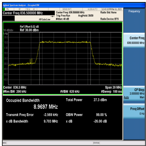
Band5-10MHz-16QAM-20525-50RB#0-8.9697
