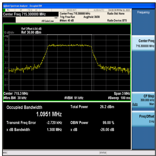
Band12-1.4MHz-16QAM-23173-6RB#0-1.0951
