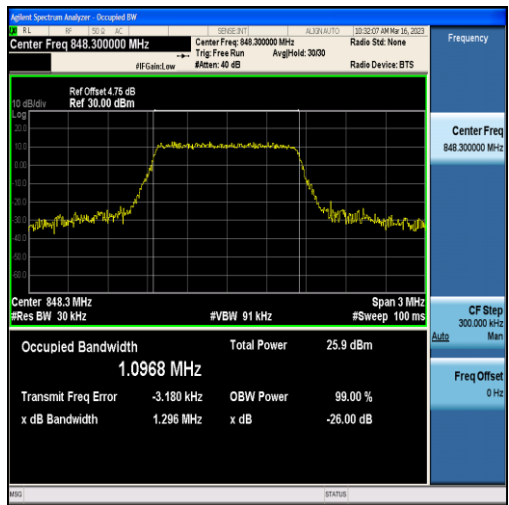
Band5-1.4MHz-16QAM-20643-6RB#0-1.0968
