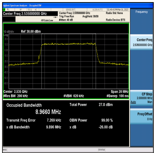
Band7-10MHz-16QAM-21100-50RB#0-8.9660
