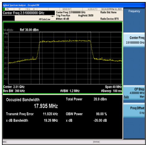
Band7-20MHz-QPSK-20850-100RB#0-17.935
