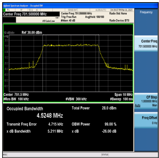
Band12-5MHz-QPSK-23035-25RB#0-4.5248
