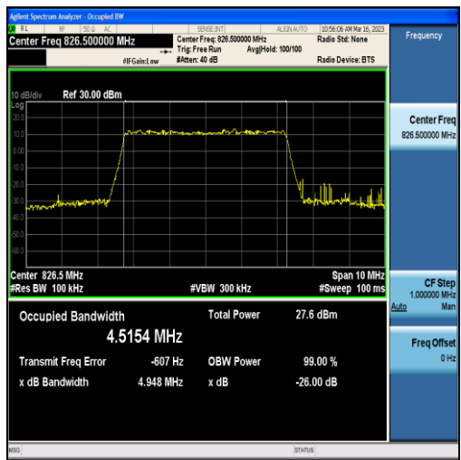
Band5-5MHz-QPSK-20425-25RB#0-4.5154
