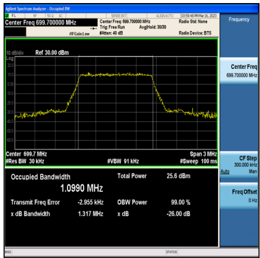
Band12-1.4MHz-16QAM-23017-6RB#0-1.0990
