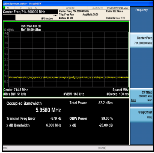
Band12-3MHz-QPSK-23165-15RB#0-5.9580
