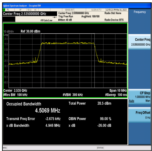
Band7-5MHz-QPSK-21100-25RB#0-4.5069
