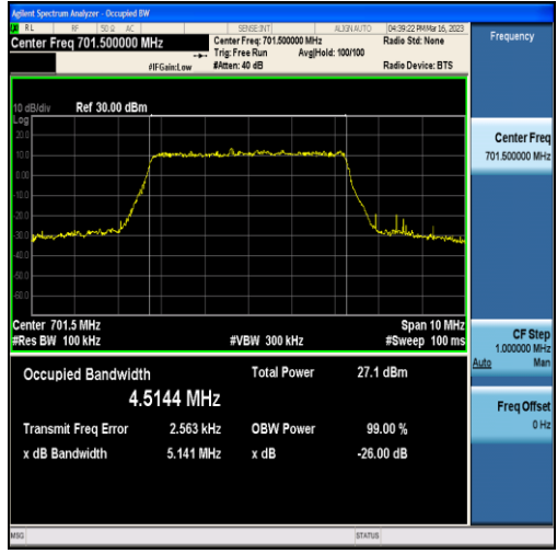
Band12-5MHz-16QAM-23035-25RB#0-4.5144
