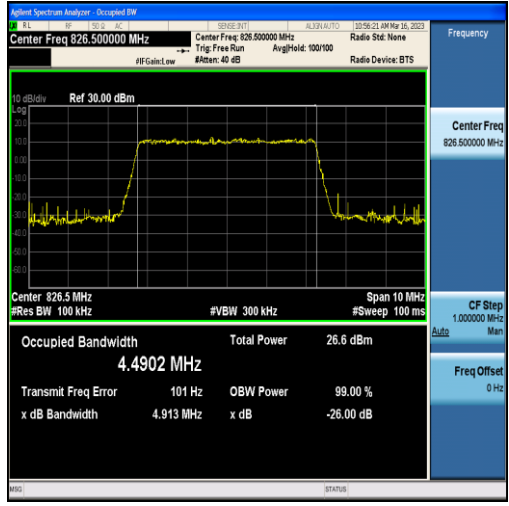
Band5-5MHz-16QAM-20425-25RB#0-4.4902
