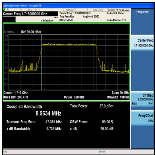
Band4-10MHz-QPSK-20000-50RB#0-8.9634
