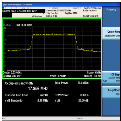
Band7-20MHz-QPSK-21100-100RB#0-17.956
