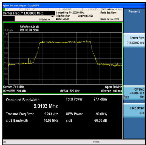
Band12-10MHz-16QAM-23130-50RB#0-9.0193
