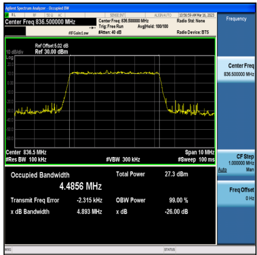
Band5-5MHz-16QAM-20525-25RB#0-4.4856
