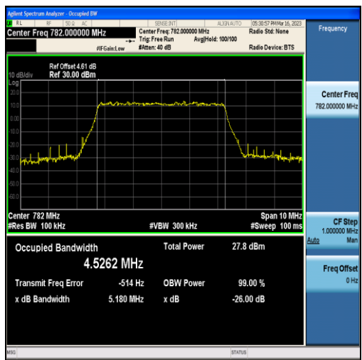
Band13-5MHz-QPSK-23230-25RB#0-4.5262
