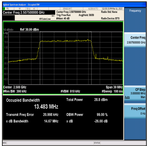
Band7-15MHz-QPSK-20825-75RB#0-13.483
