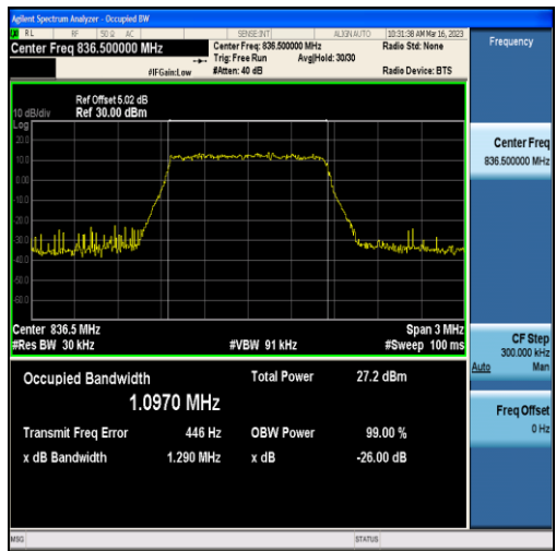
Band5-1.4MHz-QPSK-20525-6RB#0-1.0970
