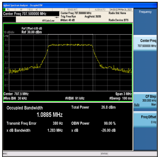
Band12-1.4MHz-QPSK-23095-6RB#0-1.0885
