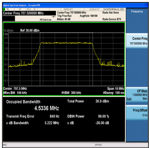
Band12-5MHz-16QAM-23095-25RB#0-4.5336
