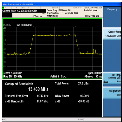
Band4-15MHz-16QAM-20175-75RB#0-13.468
