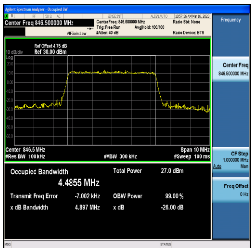
Band5-5MHz-16QAM-20625-25RB#0-4.4855
