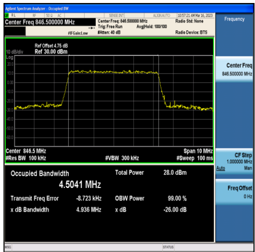
Band5-5MHz-QPSK-20625-25RB#0-4.5041
