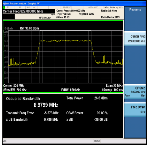
Band5-10MHz-16QAM-20450-50RB#0-8.9799
