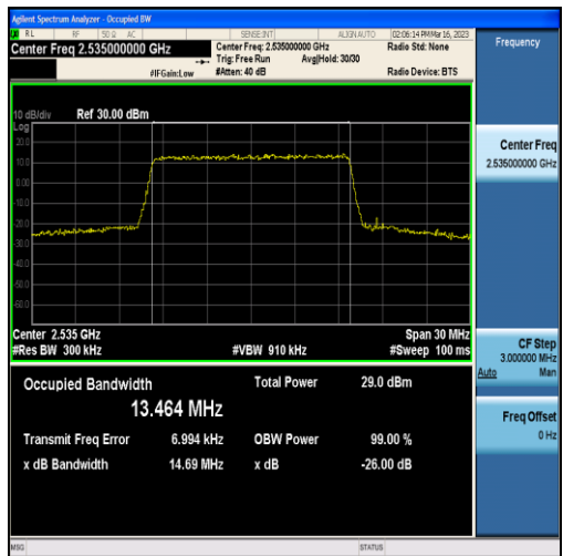
Band7-15MHz-QPSK-21100-75RB#0-13.464
