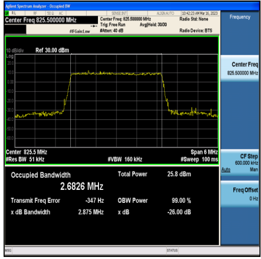
Band5-3MHz-16QAM-20415-15RB#0-2.6826
