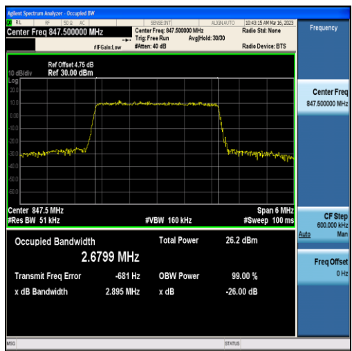
Band5-3MHz-16QAM-20635-15RB#0-2.6799
