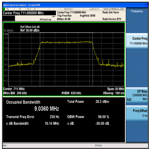
Band12-10MHz-QPSK-23130-50RB#0-9.0360
