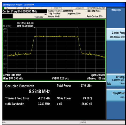
Band5-10MHz-16QAM-20600-50RB#0-8.9648
