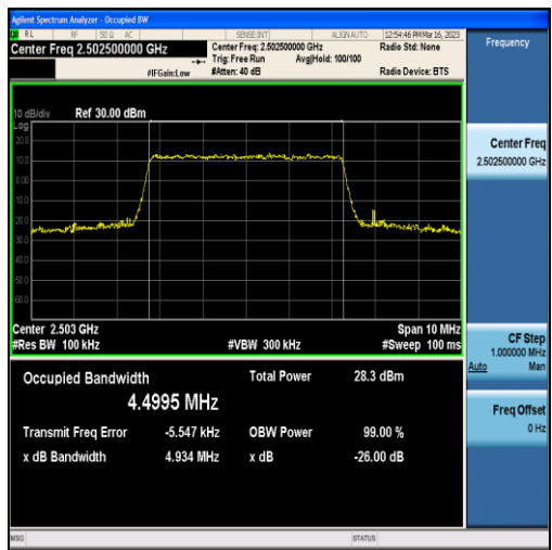
Band7-5MHz-QPSK-20775-25RB#0-4.4995
