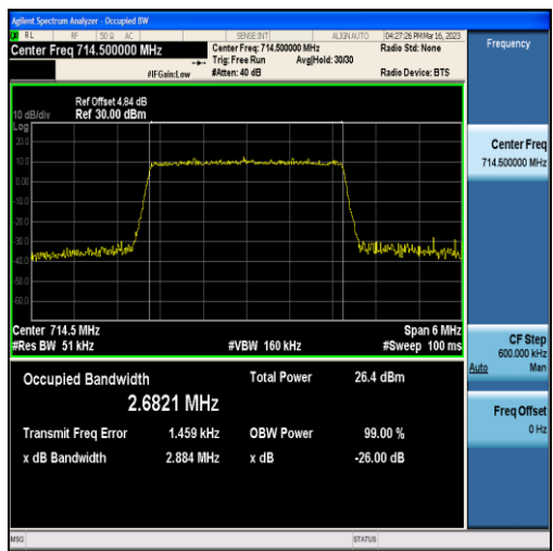
Band12-3MHz-16QAM-23165-15RB#0-2.6821
