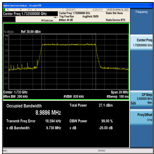
Band4-10MHz-16QAM-20175-50RB#0-8.9886
