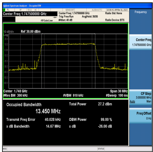
Band4-15MHz-16QAM-20325-75RB#0-13.450
