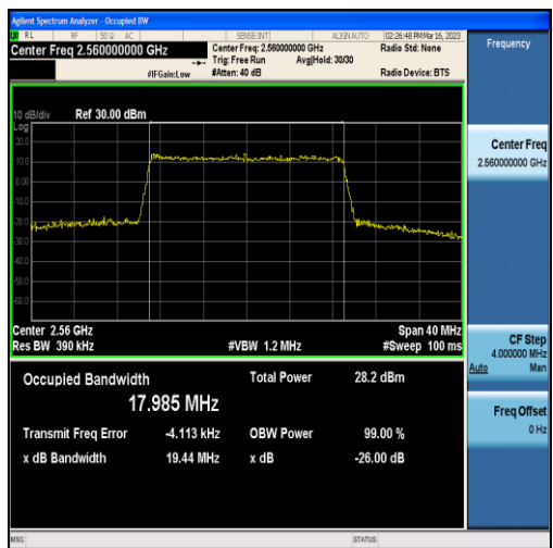
Band7-20MHz-16QAM-21350-100RB#0-17.985
