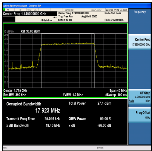
Band4-20MHz-16QAM-20300-100RB#0-17.923
