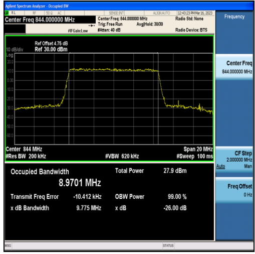
Band5-10MHz-QPSK-20600-50RB#0-8.9701
