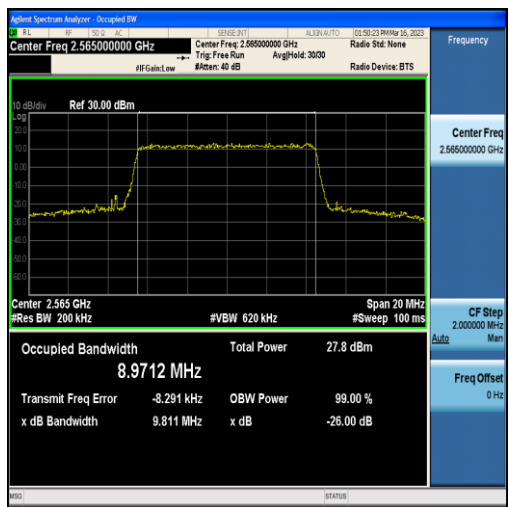
Band7-10MHz-16QAM-21400-50RB#0-8.9712
