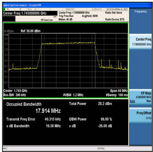
Band4-20MHz-QPSK-20300-100RB#0-17.914
