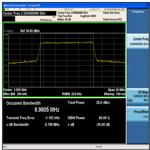
Band7-10MHz-QPSK-20800-50RB#0-8.9805
