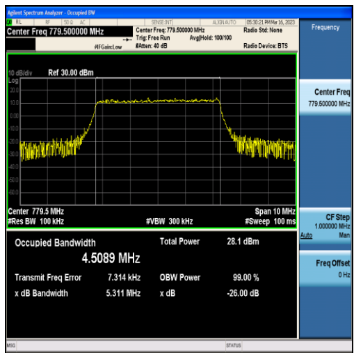
Band13-5MHz-QPSK-23205-25RB#0-4.5089
