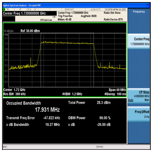
Band4-20MHz-QPSK-20050-100RB#0-17.931
