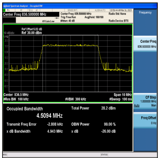
Band5-5MHz-QPSK-20525-25RB#0-4.5094
