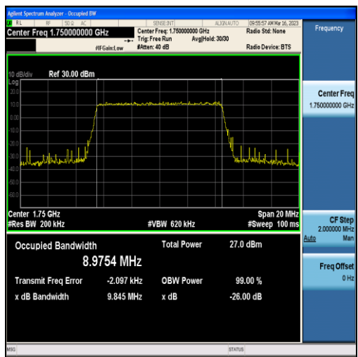
Band4-10MHz-16QAM-20350-50RB#0-8.9754
