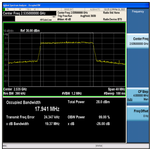
Band7-20MHz-16QAM-21100-100RB#0-17.941
