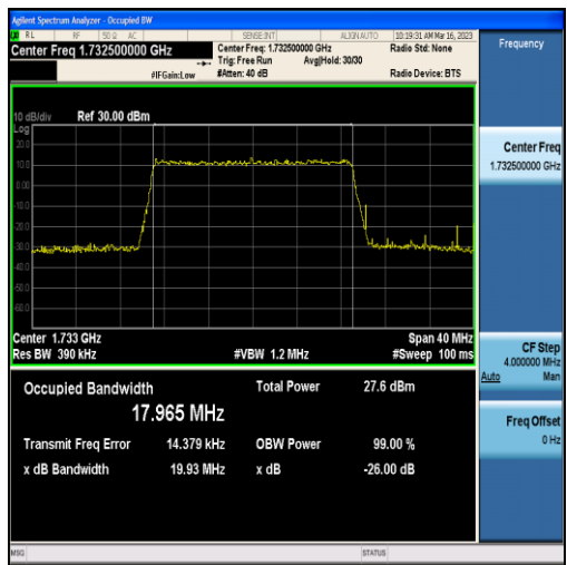
Band4-20MHz-16QAM-20175-100RB#0-17.965
