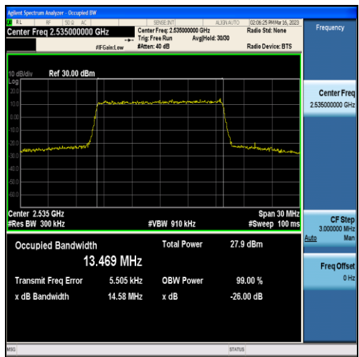
Band7-15MHz-16QAM-21100-75RB#0-13.469
