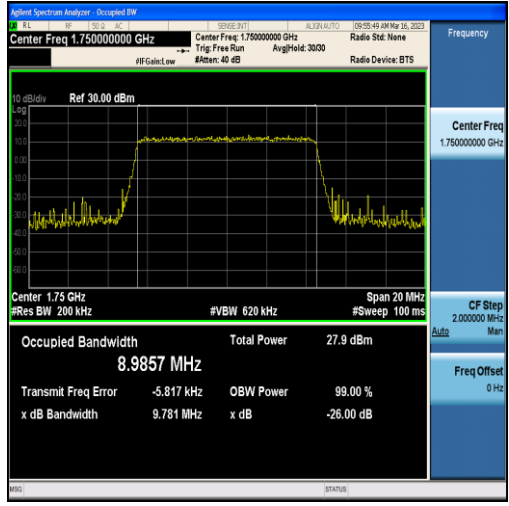
Band4-10MHz-QPSK-20350-50RB#0-8.9857
