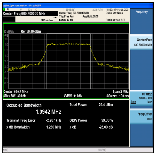
Band12-1.4MHz-QPSK-23017-6RB#0-1.0942
