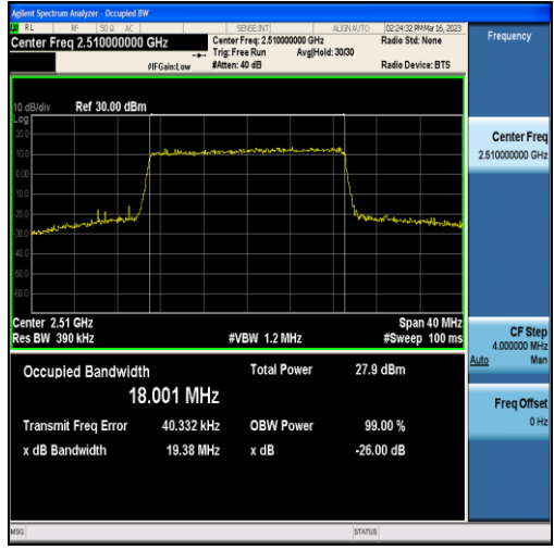
Band7-20MHz-16QAM-20850-100RB#0-18.001
