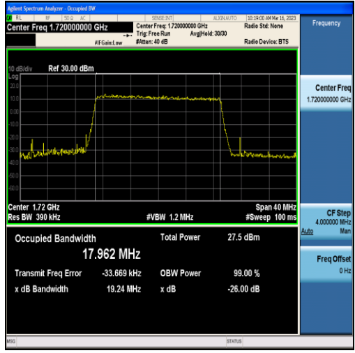
Band4-20MHz-16QAM-20050-100RB#0-17.962
