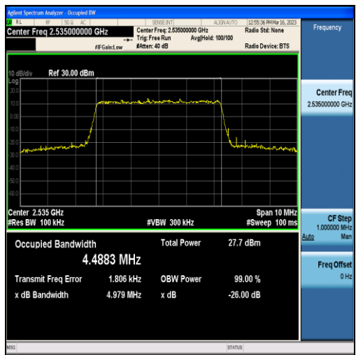
Band7-5MHz-16QAM-21100-25RB#0-4.4883
