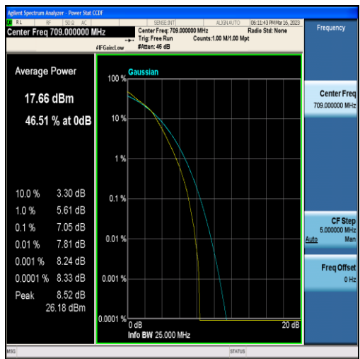
Band17-10MHz-16QAM-23780-50RB#0
