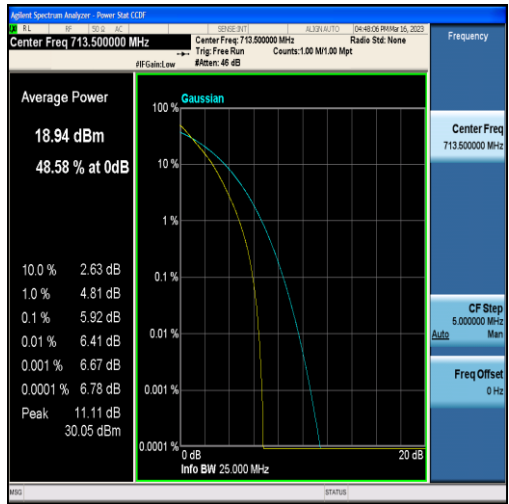
Band12-5MHz-QPSK-23155-25RB#0
