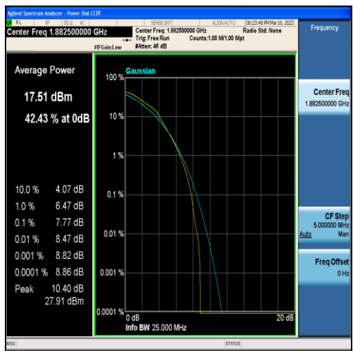
Band25-1.4MHz-16QAM-26365-6RB#0
