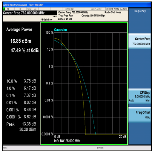
Band13-10MHz-QPSK-23230-50RB#0
