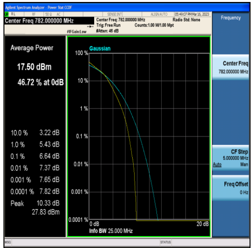
Band13-10MHz-16QAM-23230-50RB#0
