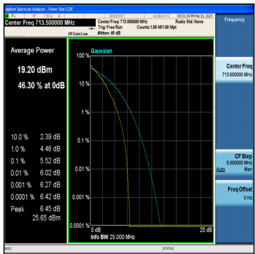
Band17-5MHz-QPSK-23825-25RB#0
