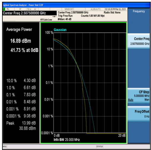
Band7-15MHz-16QAM-20825-75RB#0
