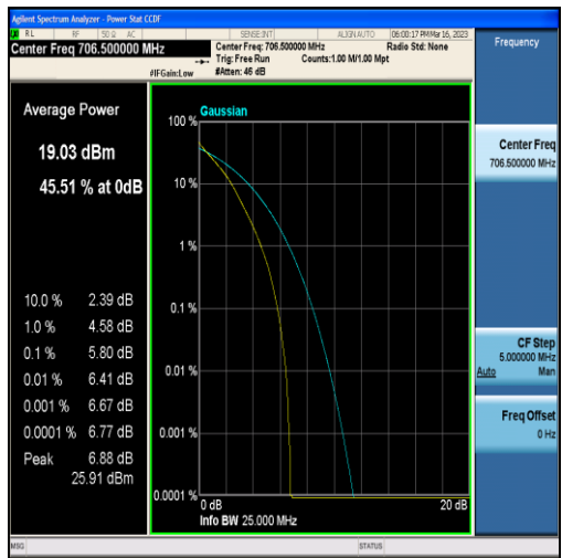
Band17-5MHz-QPSK-23755-25RB#0
