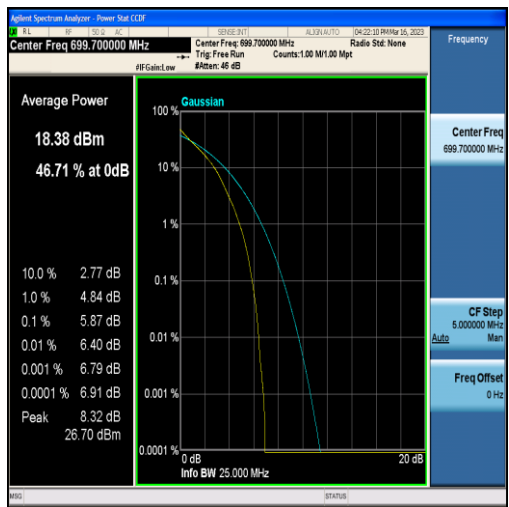
Band12-1.4MHz-QPSK-23017-6RB#0
