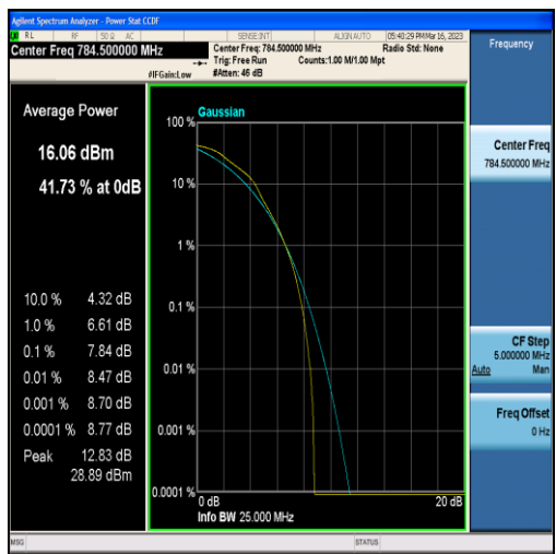
Band13-5MHz-16QAM-23255-25RB#0
