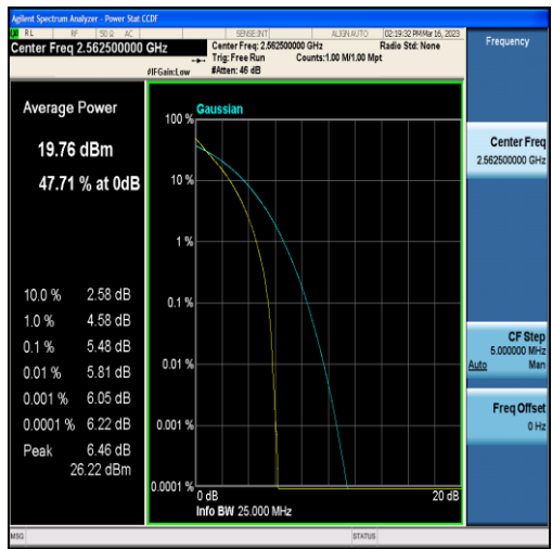
Band7-15MHz-QPSK-21375-75RB#0
