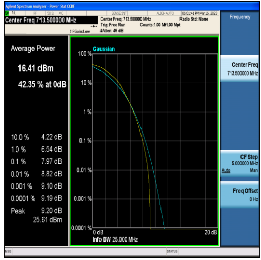
Band17-5MHz-16QAM-23825-25RB#0
