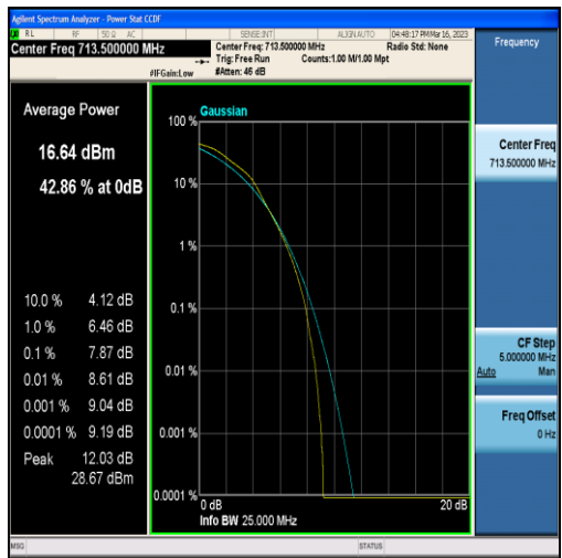
Band12-5MHz-16QAM-23155-25RB#0
