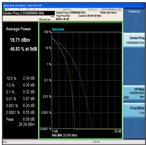
Band7-20MHz-QPSK-21100-100RB#0
