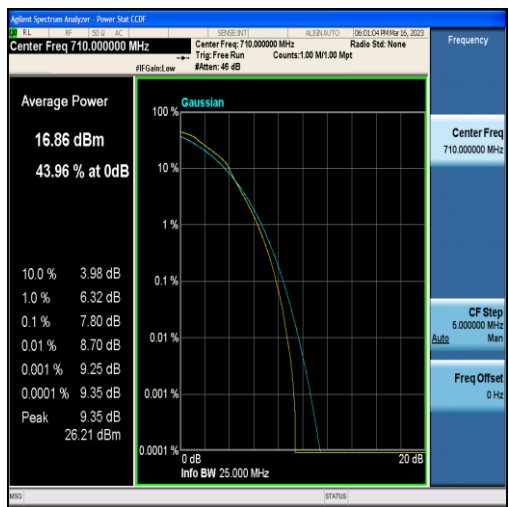
Band17-5MHz-16QAM-23790-25RB#0
