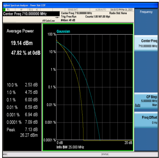
Band17-5MHz-QPSK-23790-25RB#0
