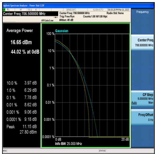
Band17-5MHz-16QAM-23755-25RB#0
