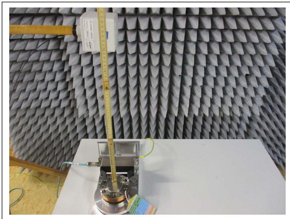
Photograph A1-2: SETUP B (distance from surface of EUT to surface of probe)
