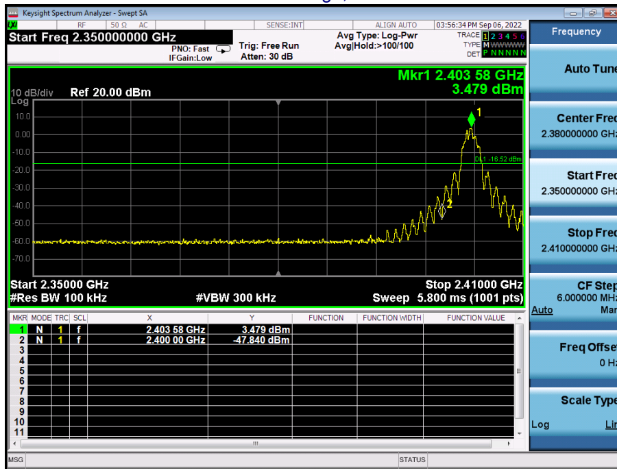
FSK: Band Edge, Left Side
