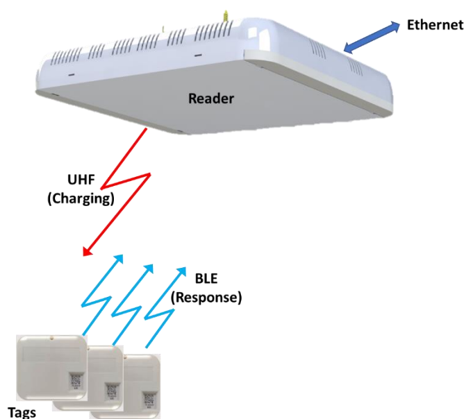
Figure 2 - Reader's functionality
