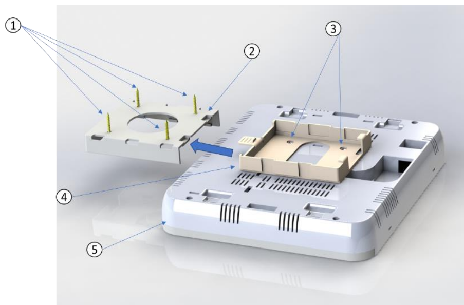
Figure 7 - Fixed mounting kit – Installation illustration
