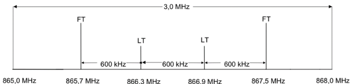
Figure 10 - EN 302 308 Lower band designated frequencies
