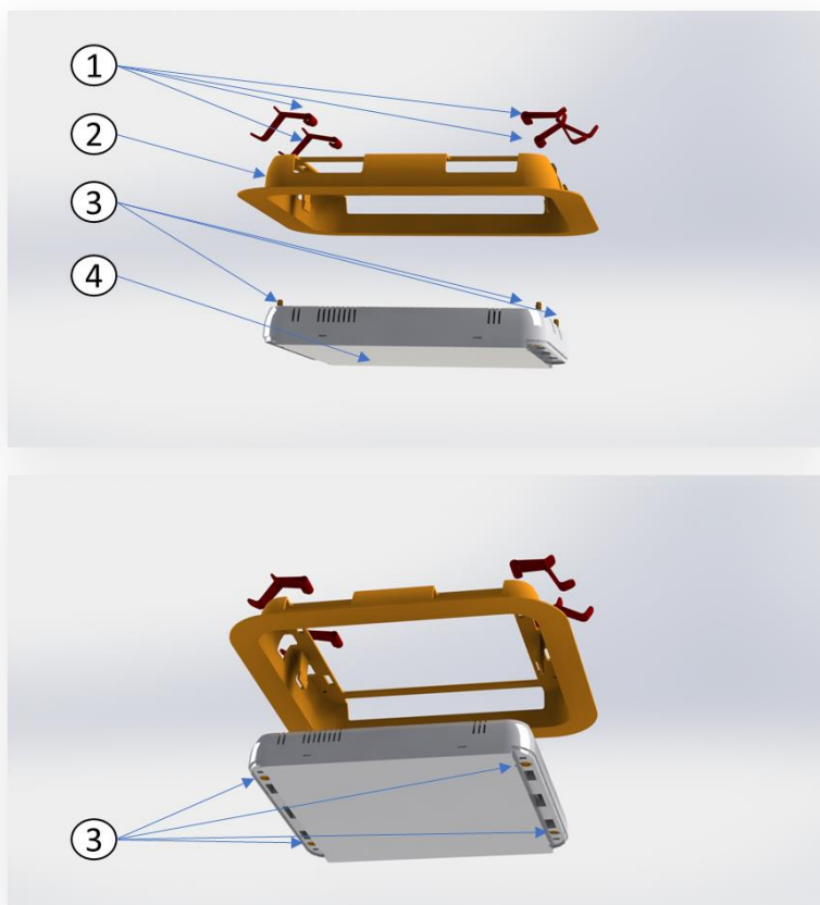
Figure 9 - Flush mounting kit – Installation illustration
