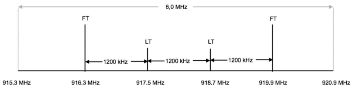
Figure 11 - EN 302 308 Upper band designated frequencies
