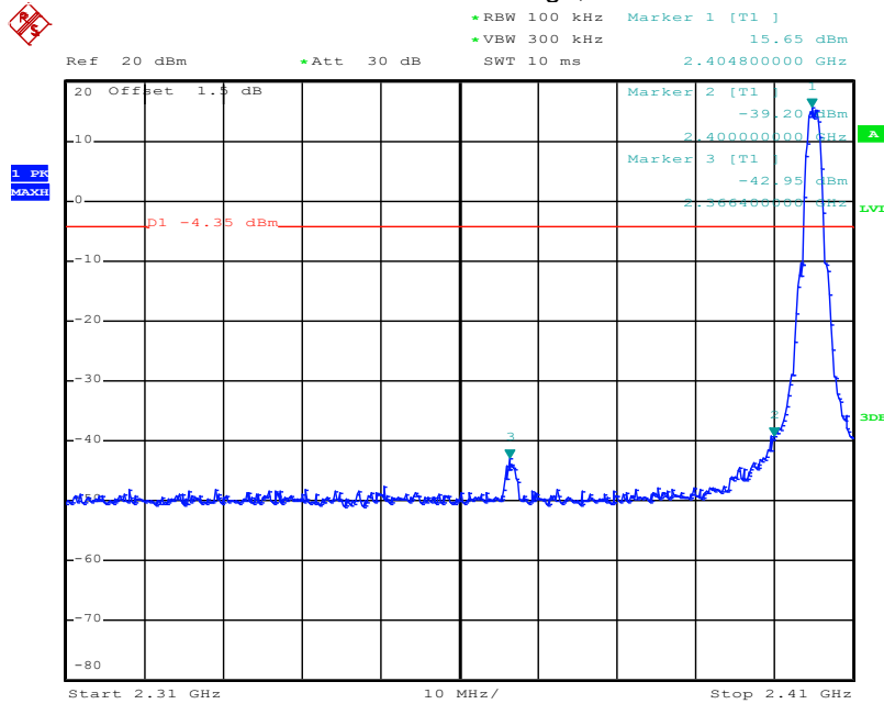
OQPSK: Band Edge, Left Side
