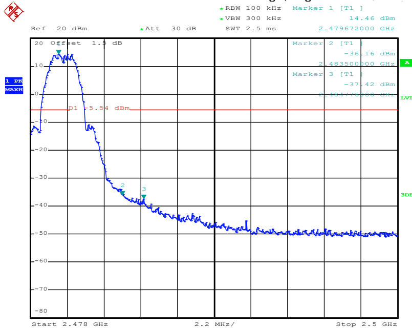
OQPSK: Band Edge, Right Side
