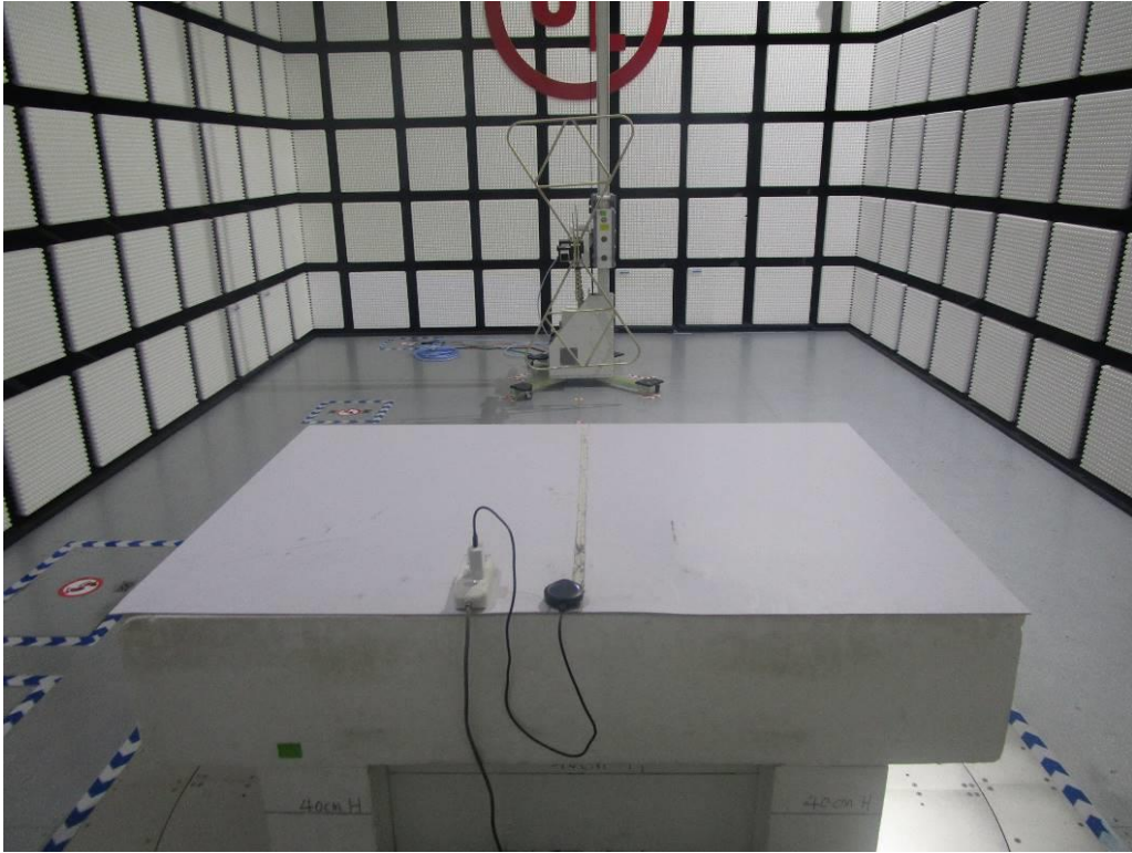
Radiated Emissions up to 1 GHz
