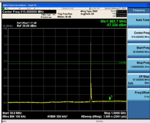
Band12_10MHz_16QAM_23130_1RB#0_30~1000_30~10
