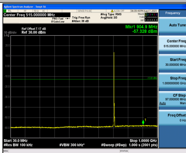
Band12_3MHz_QPSK_23165_1RB#0_30~1000_30~1000
