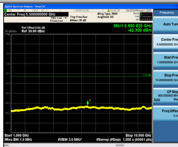
Band12_5MHz_QPSK_23095_1RB#0_1000~10000_1000~10000
