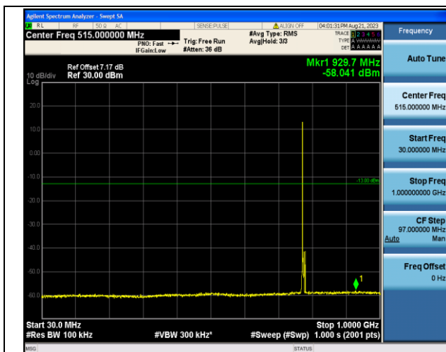
Band13_5MHz_QPSK_23205_1RB#0_30~1000_30~1000
