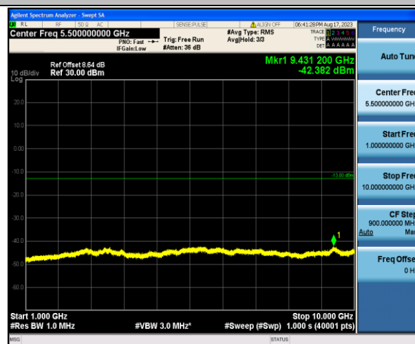
Band12_10MHz_16QAM_23060_1RB#0_1000~10000_1000~100
