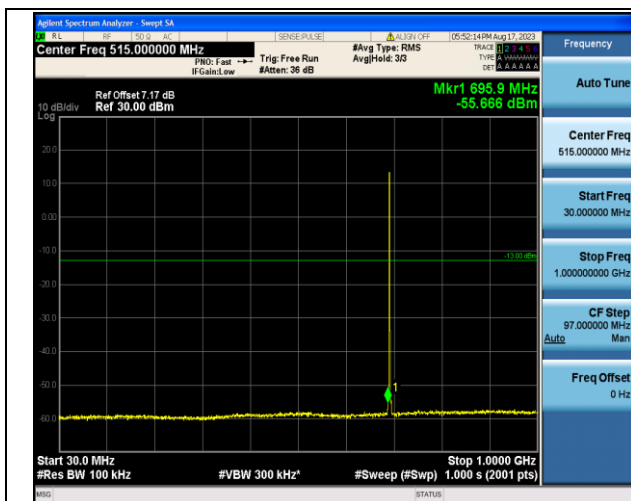
Band12_1.4MHz_QPSK_23017_1RB#0_30~1000_30~100
