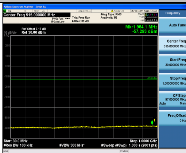
Band4_20MHz_16QAM_20300_1RB#0_30~1000_30~100
