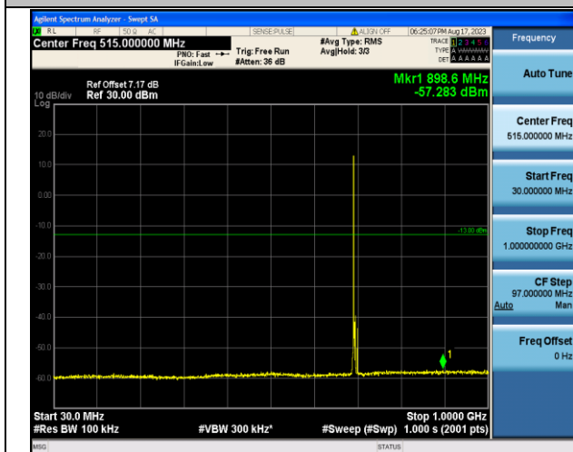
Band12_5MHz_16QAM_23035_1RB#0_30~1000_30~1000
