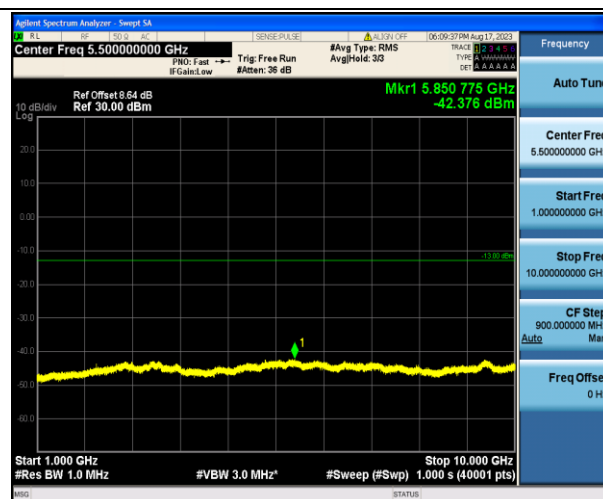
Band12_3MHz_16QAM_23095_1RB#0_1000~10000_1000~1000
