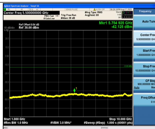
Band12_5MHz_16QAM_23095_1RB#0_1000~10000_1000~1000
