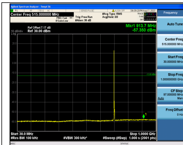
Band12_3MHz_16QAM_23095_1RB#0_30~1000_30~100
