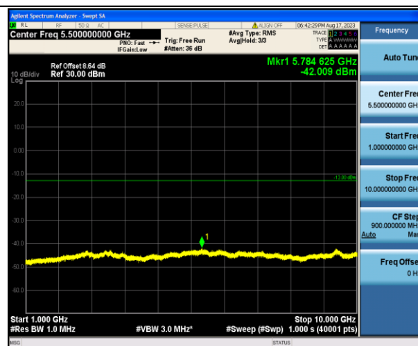
Band12_10MHz_16QAM_23095_1RB#0_1000~10000_1000~100
