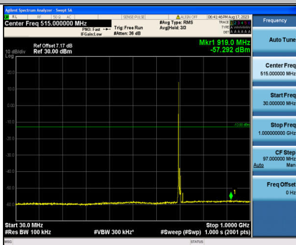
Band12_10MHz_QPSK_23095_1RB#0_30~1000_30~100
