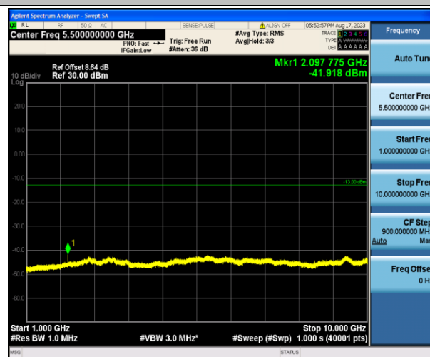
Band12_1.4MHz_16QAM_23017_1RB#0_1000~10000_1000~10
