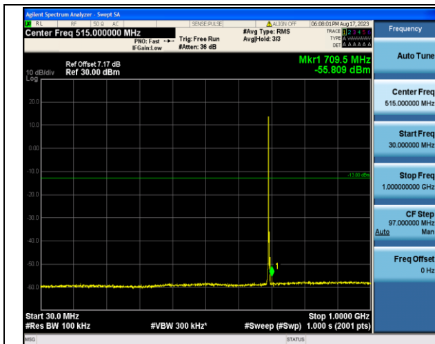
Band12_3MHz_QPSK_23025_1RB#0_30~1000_30~1000
