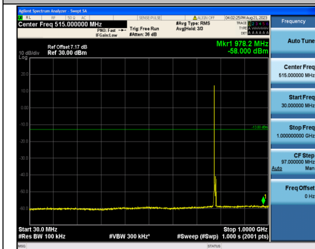
Band13_5MHz_QPSK_23230_1RB#0_30~1000_30~1000
