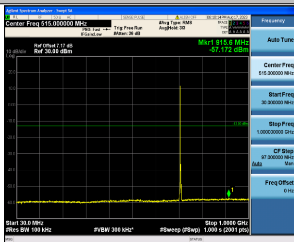
Band12_3MHz_16QAM_23165_1RB#0_30~1000_30~100
