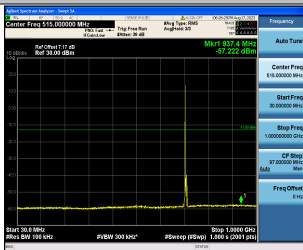
Band12_5MHz_QPSK_23155_1RB#0_30~1000_30~1000
