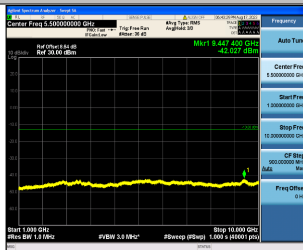
Band12_10MHz_16QAM_23130_1RB#0_1000~10000_1000~100
