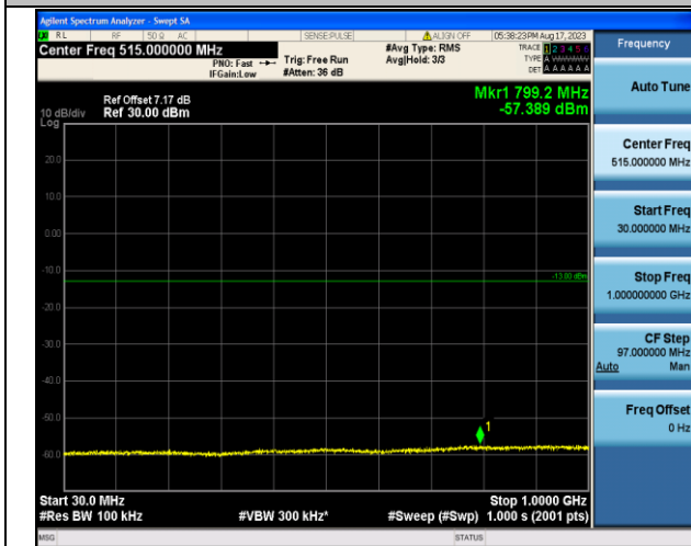
Band4_20MHz_QPSK_20050_1RB#0_30~1000_30~1000
