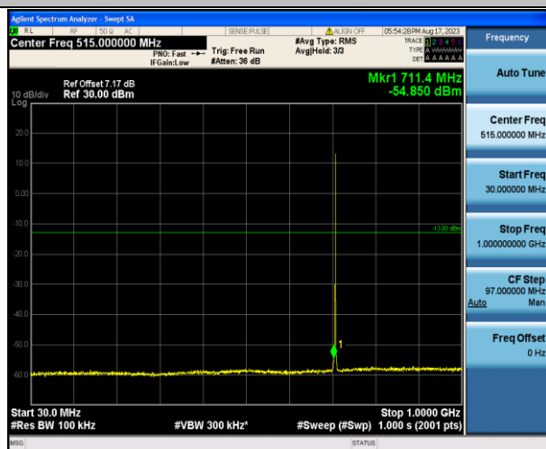
Band12_1.4MHz_16QAM_23173_1RB#0_30~1000_30~1000
