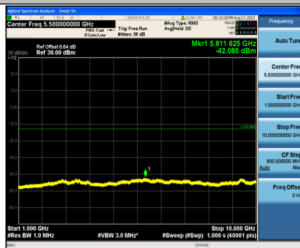
Band12_3MHz_16QAM_23165_1RB#0_1000~10000_1000~1000
