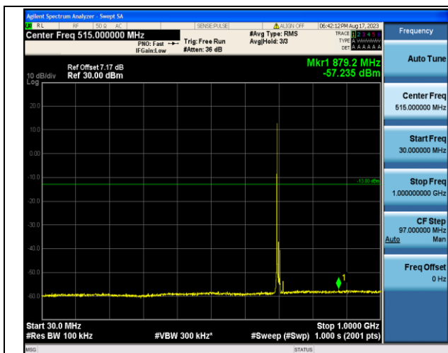
Band12_10MHz_16QAM_23095_1RB#0_30~1000_30~10
