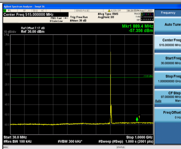
Band12_5MHz_16QAM_23155_1RB#0_30~1000_30~100
