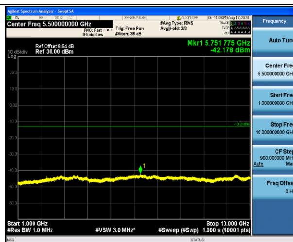
Band12_10MHz_QPSK_23060_1RB#0_1000~10000_1000~1000
