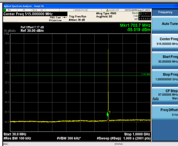
Band12_1.4MHz_QPSK_23095_1RB#0_30~1000_30~100
