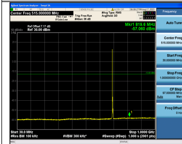
Band12_3MHz_16QAM_23025_1RB#0_30~1000_30~1000
