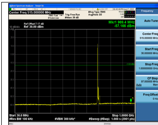
Band12_10MHz_QPSK_23060_1RB#0_30~1000_30~100
