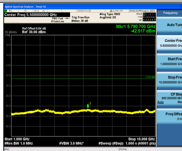
Band13_5MHz_QPSK_23230_1RB#0_1000~10000_1000~10000
