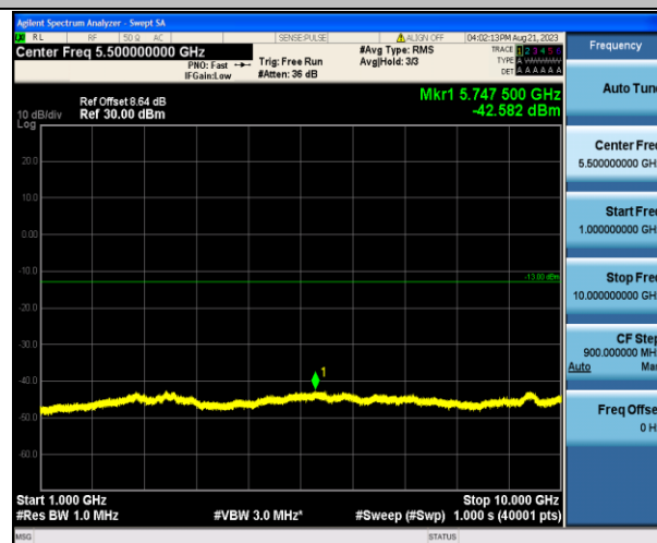
Band13_5MHz_16QAM_23205_1RB#0_1000~10000_1000~10000
