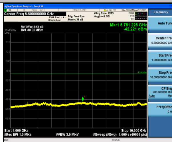
Band12_10MHz_QPSK_23130_1RB#0_1000~10000_1000~1000
