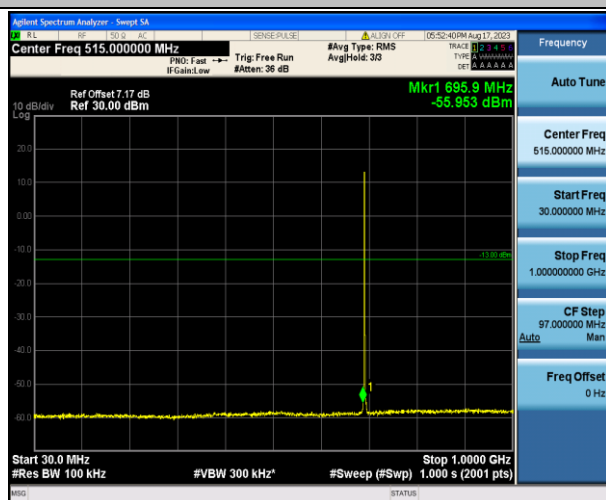
Band12_1.4MHz_16QAM_23017_1RB#0_30~1000_30~1
