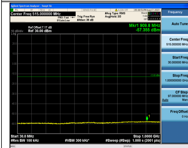
Band4_20MHz_QPSK_20175_1RB#0_30~1000_30~1000
