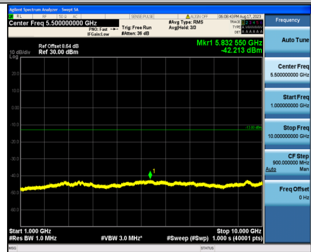
Band12_3MHz_16QAM_23025_1RB#0_1000~10000_1000~10000
