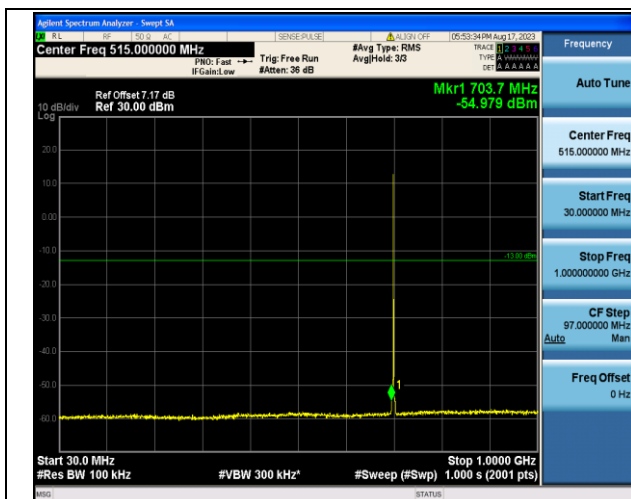
Band12_1.4MHz_16QAM_23095_1RB#0_30~1000_30~1000
