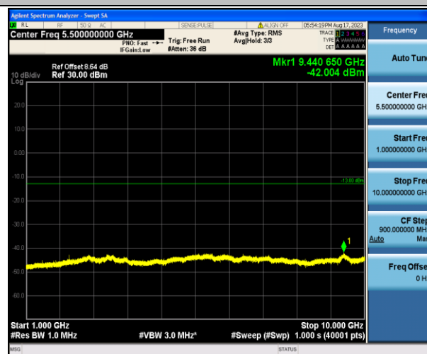
Band12_1.4MHz_QPSK_23173_1RB#0_1000~10000_1000~1000
