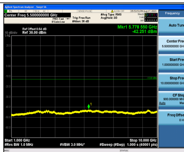
Band12_1.4MHz_16QAM_23095_1RB#0_1000~10000_1000~10000
