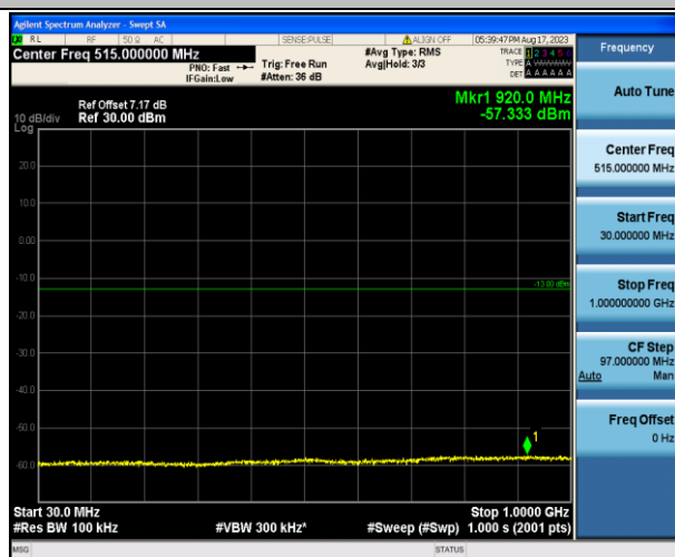
Band4_20MHz_QPSK_20300_1RB#0_30~1000_30~1000
