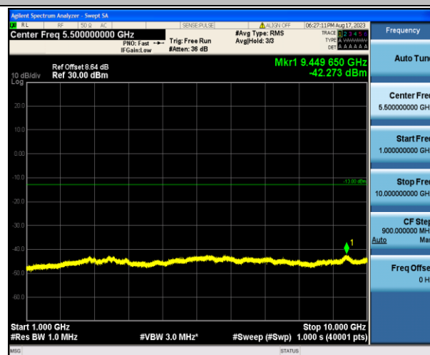
Band12_5MHz_16QAM_23155_1RB#0_1000~10000_1000~1000
