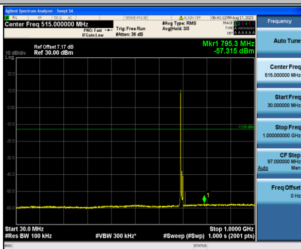
Band12_10MHz_16QAM_23060_1RB#0_30~1000_30~10
