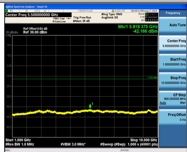
Band12_3MHz_QPSK_23095_1RB#0_1000~10000_1000~10000
