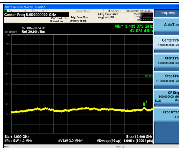
Band13_5MHz_QPSK_23205_1RB#0_1000~10000_1000~10000
