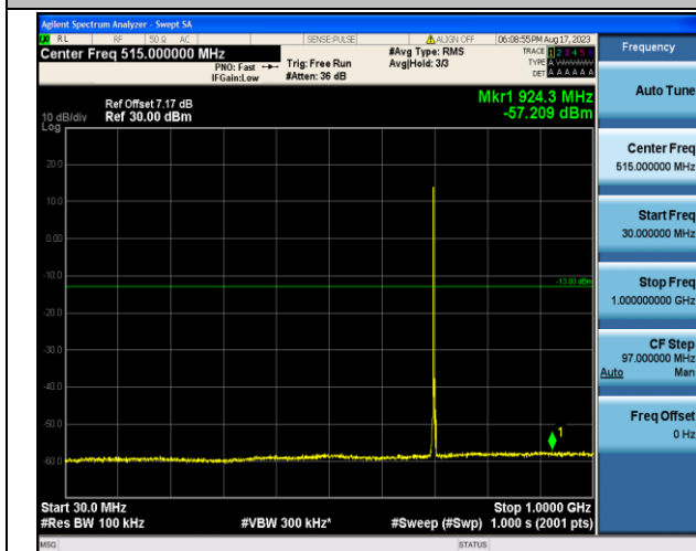
Band12_3MHz_QPSK_23095_1RB#0_30~1000_30~1000
