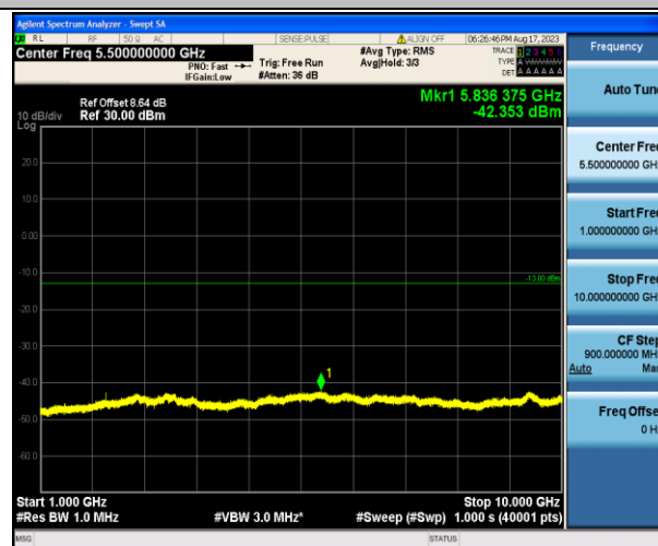
Band12_5MHz_QPSK_23155_1RB#0_1000~10000_1000~10000
