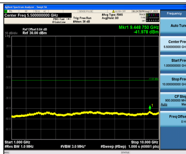
Band12_5MHz_QPSK_23035_1RB#0_1000~10000_1000~10000
