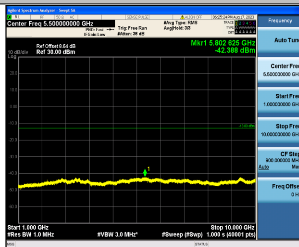
Band12_5MHz_16QAM_23035_1RB#0_1000~10000_1000~10000
