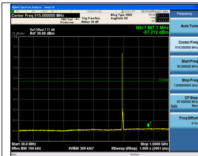
Band12_5MHz_QPSK_23035_1RB#0_30~1000_30~1000
