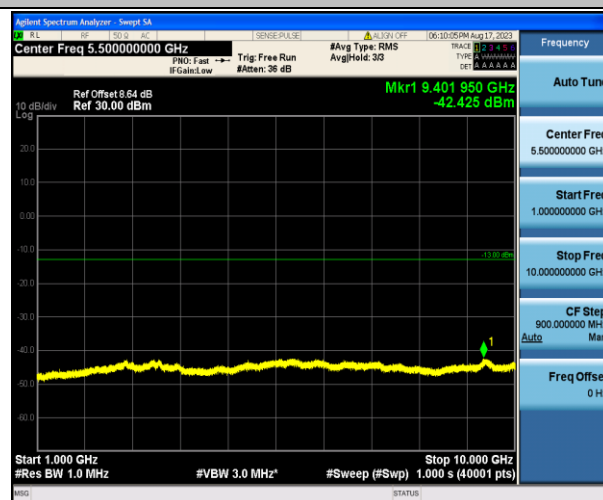
Band12_3MHz_QPSK_23165_1RB#0_1000~10000_1000~10000
