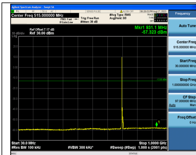
Band12_5MHz_16QAM_23095_1RB#0_30~1000_30~100
