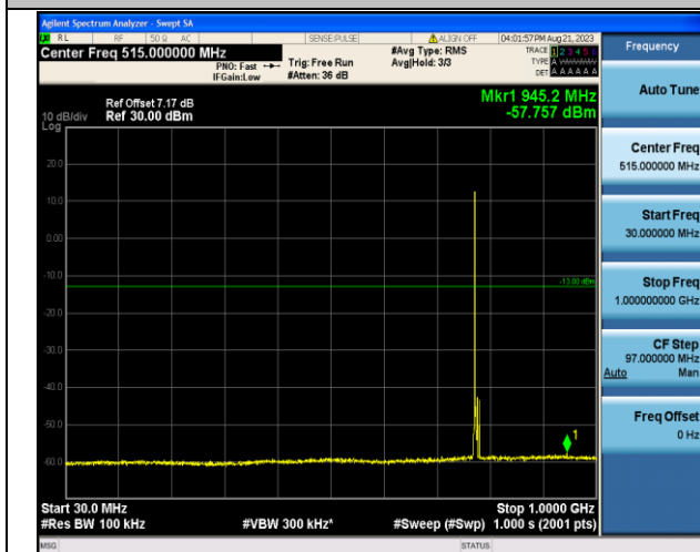
Band13_5MHz_16QAM_23205_1RB#0_30~1000_30~1000
