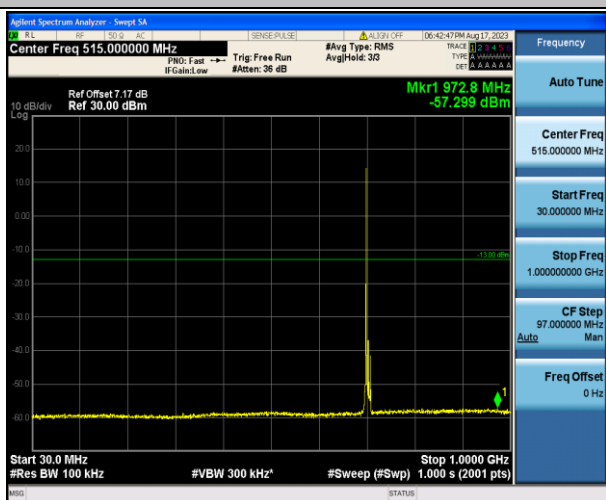
Band12_10MHz_QPSK_23130_1RB#0_30~1000_30~100
