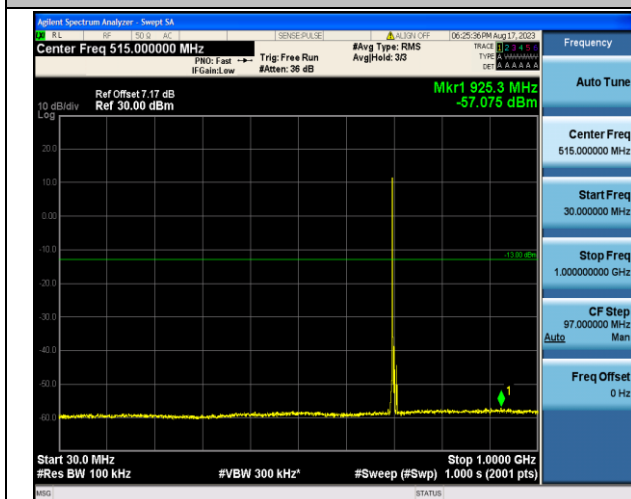
Band12_5MHz_QPSK_23095_1RB#0_30~1000_30~1000
