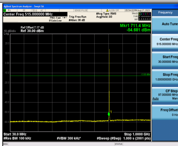
Band12_1.4MHz_QPSK_23173_1RB#0_30~1000_30~1000
